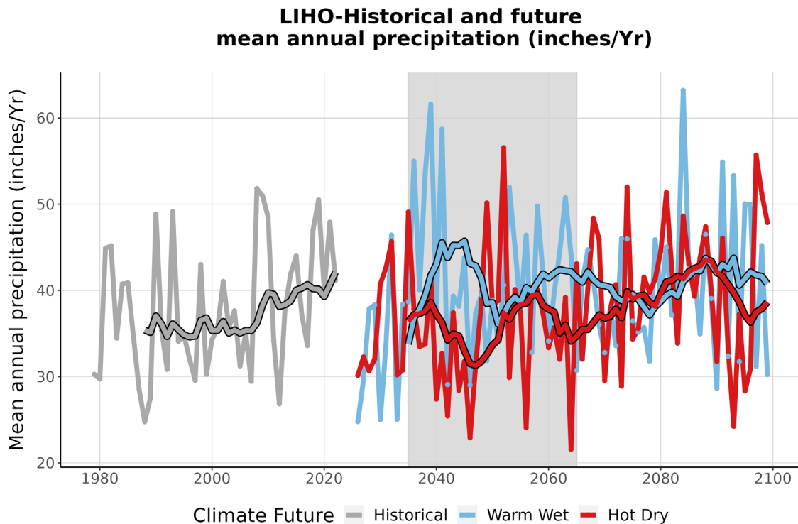
Figure 4. This graph compares observed average annual precipitation at LIHO (inches/year) (1979-2022) with projected average annual precipitation for the two climate futures over the period 2023-2099. The historically observed data is shown in gray, the Warm Wet climate future in blue, and the Hot Dry climate future in red. The smooth line running through each projection is the 10-year running average for historical observations and future projections. The gray-shaded area represents the time period that was averaged (2035-2065) to summarize future projections for the year 2050 (Appendix 1).
