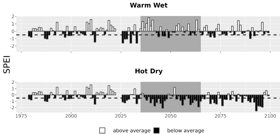
Figure 7. Drought metrics for LIHO. Drought index (SPEI; units = standard deviations from historical) timeseries for each climate future. Below-average SPEI (black bars) indicates dry conditions. The dotted line (SPEI = -0.5) indicates drought conditions.
