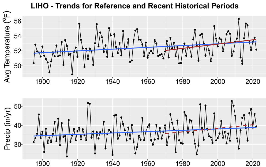
Figure 1. Historical trends in annual average temperature (upper plot) and annual total precipitation (lower plot) for LIHO from 1895-2022. Black points show yearly values while blue lines are linear regressions for the entire period record and red lines for 1970-2022 trends. Solid lines are significant trends (i.e., p < 0.05 ); dashed lines are not statistically significant.
