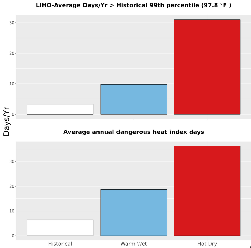
Figure 5. The upper bar graph represents the average number of days annually with temperatures greater than the historical 99th percentile (97.8 °F) historically (1979-2012) and for the two climate futures (2050). The bottom bar graph represents the average annual number of dangerous heat index days historically and for the two climate futures. Dangerous heat index days are days that exceed 105 °F.
