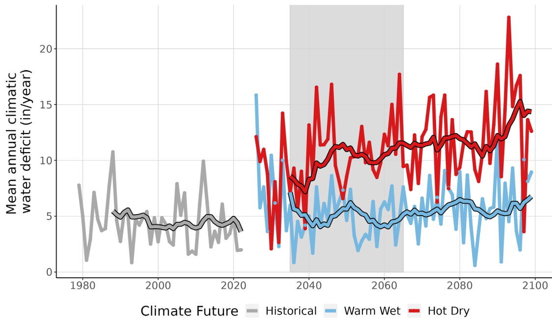
Figure 9. This line graph compares observed climatic water deficit at LIHO (inches/year) (1979-2022) with projected climatic water deficit for the two climate futures over the period 2023-2099. The historical observation data is shown in gray, the Warm Wet climate future in blue, and the Hot Dry climate future in red. The smooth line running through each projection is the 10-year running average for historical observations and future projections. Gray-shaded area represents the time period that was averaged (2035-2065) to summarize future projections for the year 2050.
