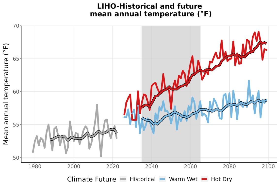
Figure 3. This graph compares observed average annual temperature at LIHO (°F) (1979-2022) with projected average annual temperature for the two climate futures over the period 2023-2099. The historically observed data
