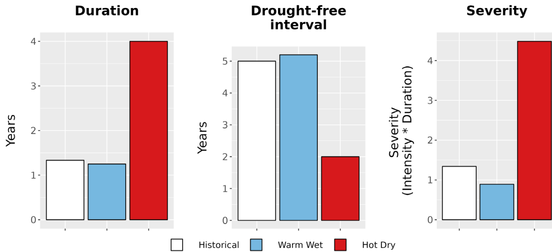
Figure 8. Drought metrics for LIHO. (Left) Average drought duration (years) historically (1979-2012) and under each climate future. (Middle) Average drought return interval (years), indicating the expected amount of time between periods of drought, historically and under each climate future. (Right) Average drought severity, a measure of drought intensity multiplied by duration, historically and under each climate future.
