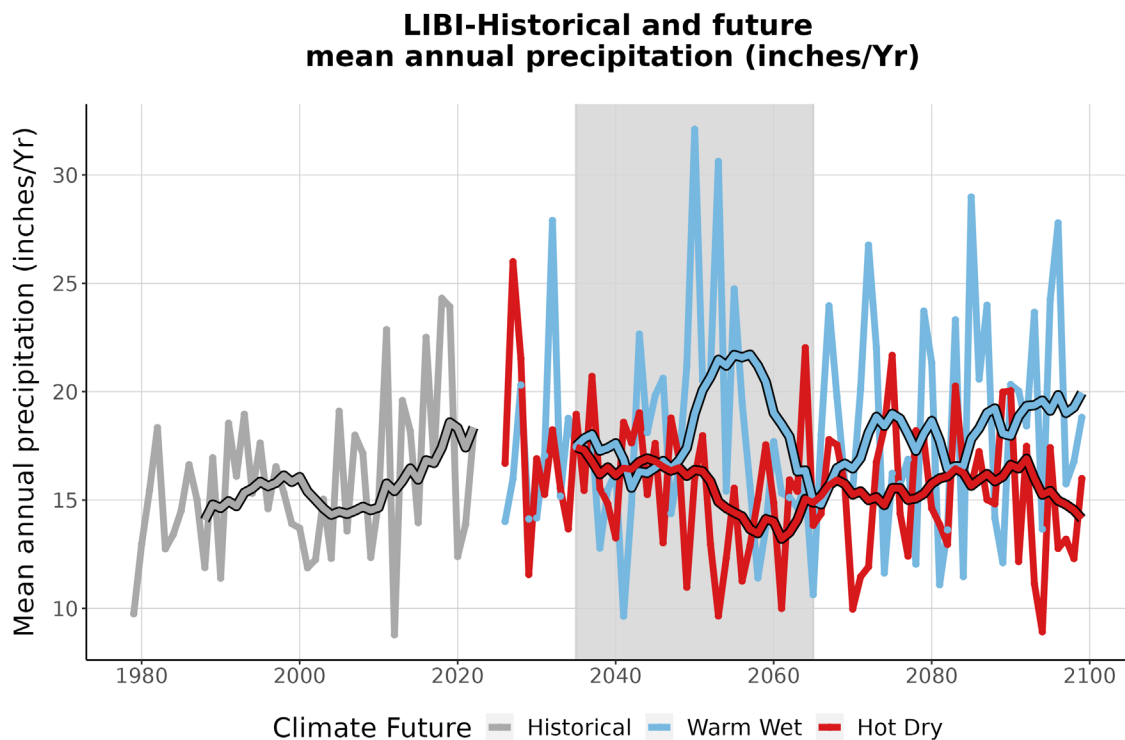
Figure 4. This graph compares observed average annual precipitation at LIBI (inches/year) (1979-2022) with projected average annual precipitation for the two climate futures over the period 2023-2099. The historically observed data is shown in gray, the Warm Wet climate future in blue, and the Hot Dry climate future in red. The smooth line running through each projection is the 10-year running average for historical observations and future projections. The gray-shaded area represents the time period that was averaged (2035-2065) to summarize future projections for the year 2050 (Appendix 1).
