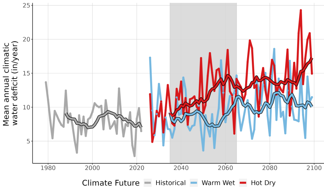
Figure 9. This line graph compares observed climatic water deficit at LIBI (inches/year) (1979-2022) with projected climatic water deficit for the two climate futures over the period 2023-2099. The historical observation data is shown in gray, the Warm Wet climate future in blue, and the Hot Dry climate future in red. The smooth line running through each projection is the 10-year running average for historical observations and future projections. Gray-shaded area represents the time period that was averaged (2035-2065) to summarize future projections for the year 2050.
