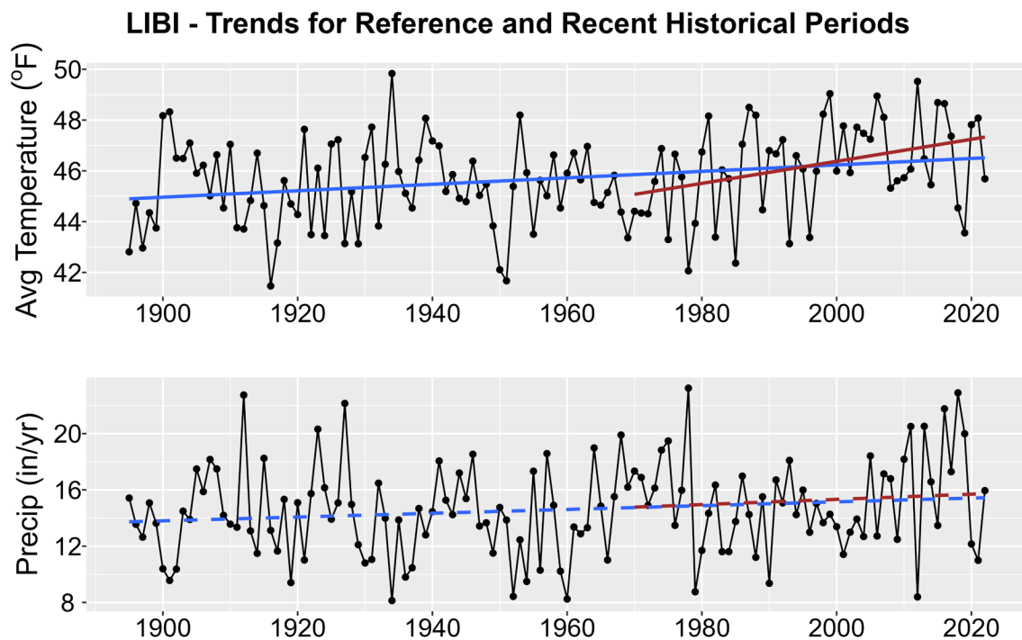
Figure 1. Historical trends in annual average temperature (upper plot) and annual total precipitation (lower plot) for LIBI from 1895-2022. Black points show yearly values while blue lines are linear regressions for the entire period record and red lines for 1970-2022 trends. Solid lines are significant trends (i.e., p < 0.05 ); dashed lines are not statistically significant.
