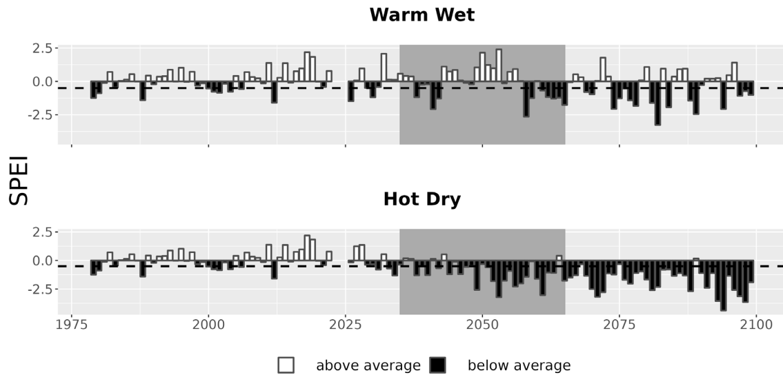
Figure 7. Drought metrics for LIBI. Drought index (SPEI; units = standard deviations from historical) timeseries for each climate future. Below-average SPEI (black bars) indicates dry conditions. The dotted line (SPEI = -0.5) indicates drought conditions.
