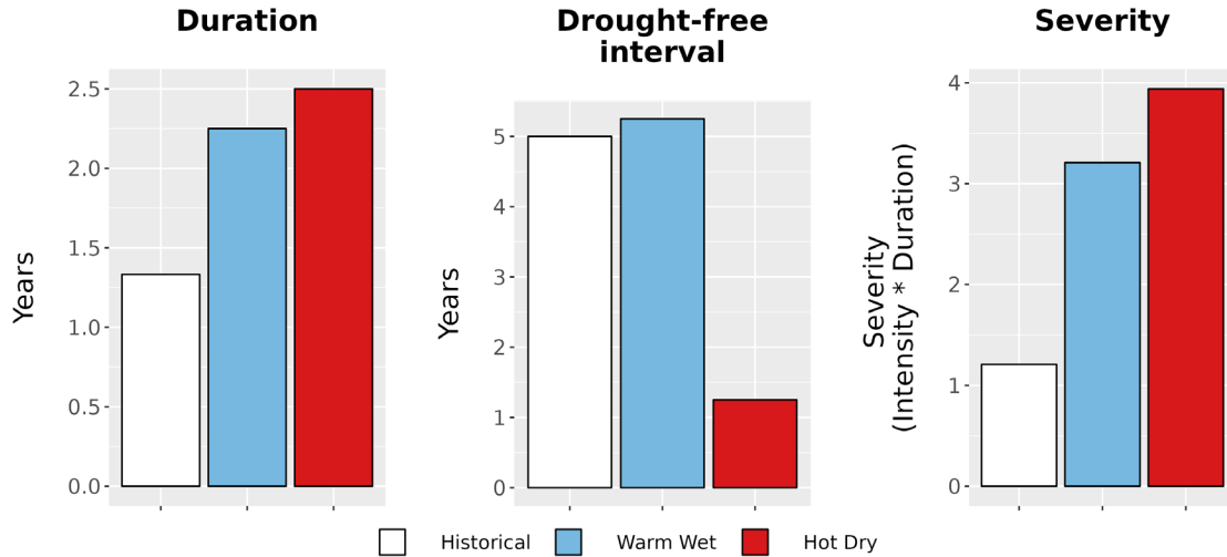
Figure 8. Drought metrics for LIBI. (Left) Average drought duration (years) historically (1979-2012) and under each climate future. (Middle) Average drought return interval (years), indicating the expected amount of time between periods of drought, historically and under each climate future. (Right) Average drought severity, a measure of drought intensity multiplied by duration, historically and under each climate future.
