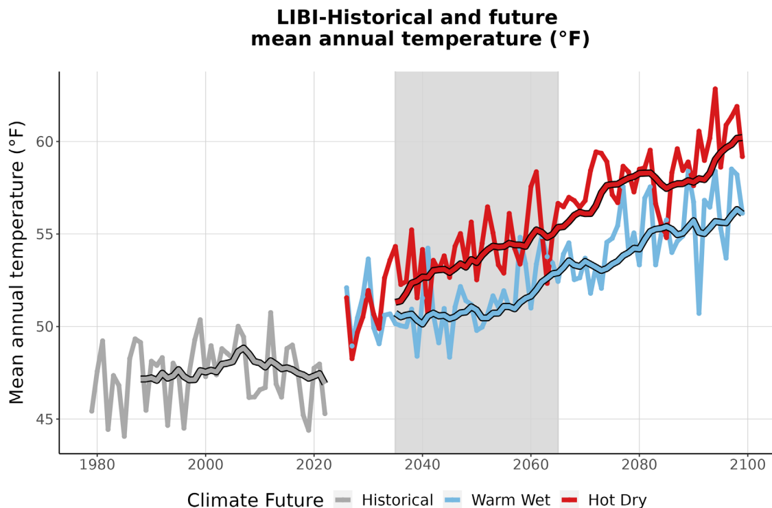
Figure 3. This graph compares observed average annual temperature at LIBI (°F) (1979-2022) with projected average annual temperature for the two climate futures over the period 2023-2099. The historically observed data
