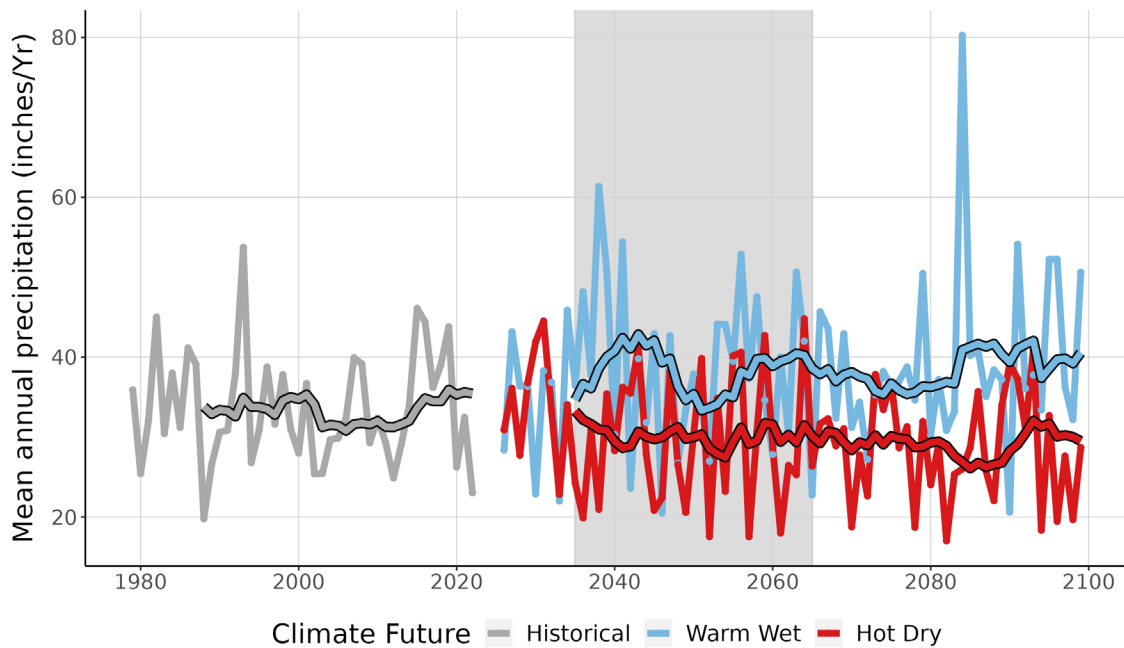
Figure 4. This graph compares observed average annual precipitation at LECL (inches/year) (1979-2022) with projected average annual precipitation for the two climate futures over the period 2023-2099. The historically observed data is shown in gray, the Warm Wet climate future in blue, and the Hot Dry climate future in red. The smooth line running through each projection is the 10-year running average for historical observations and future projections. The gray-shaded area represents the time period that was averaged (2035-2065) to summarize future projections for the year 2050 (Appendix 1).
