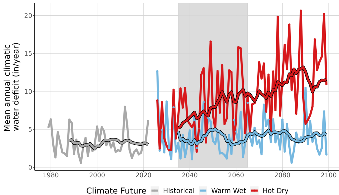
Figure 9. This line graph compares observed climatic water deficit at LECL (inches/year) (1979-2022) with projected climatic water deficit for the two climate futures over the period 2023-2099. The historical observation data is shown in gray, the Warm Wet climate future in blue, and the Hot Dry climate future in red. The smooth line running through each projection is the 10-year running average for historical observations and future projections. Gray-shaded area represents the time period that was averaged (2035-2065) to summarize future projections for the year 2050.
