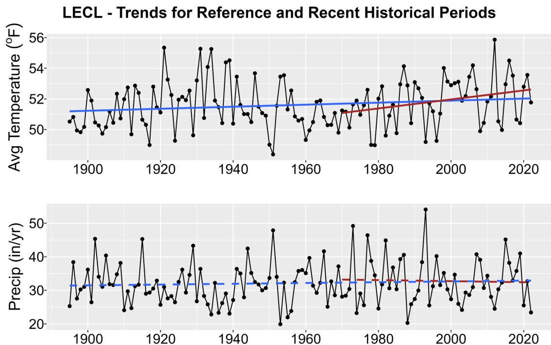
Figure 1. Historical trends in annual average temperature (upper plot) and annual total precipitation (lower plot) for LECL from 1895-2022. Black points show yearly values while blue lines are linear regressions for the entire period record and red lines for 1970-2022 trends. Solid lines are significant trends (i.e., p < 0.05 ); dashed lines are not statistically significant.
