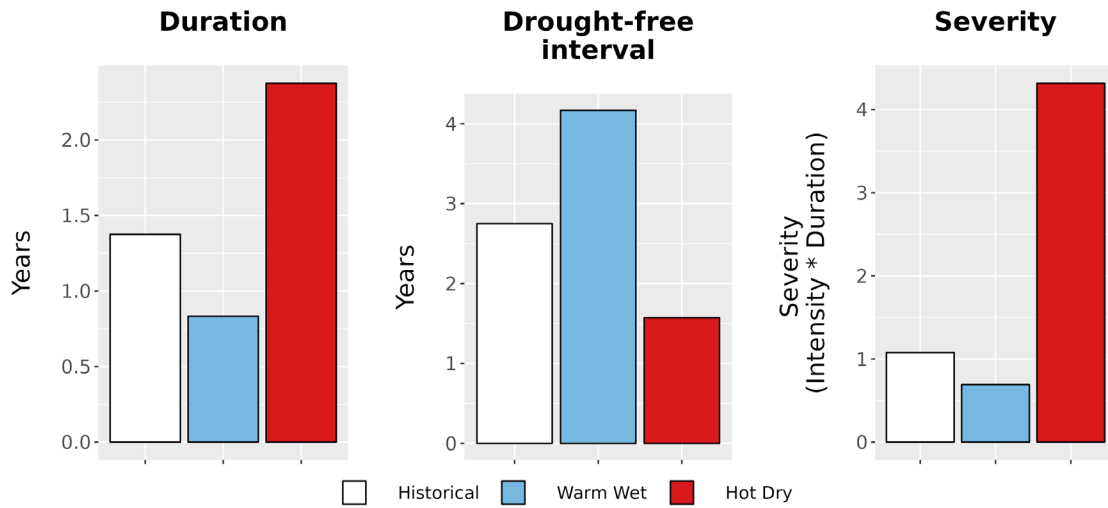
Figure 8. Drought metrics for LECL. (Left) Average drought duration (years) historically (1979-2012) and under each climate future. (Middle) Average drought return interval (years), indicating the expected amount of time between periods of drought, historically and under each climate future. (Right) Average drought severity, a measure of drought intensity multiplied by duration, historically and under each climate future.
