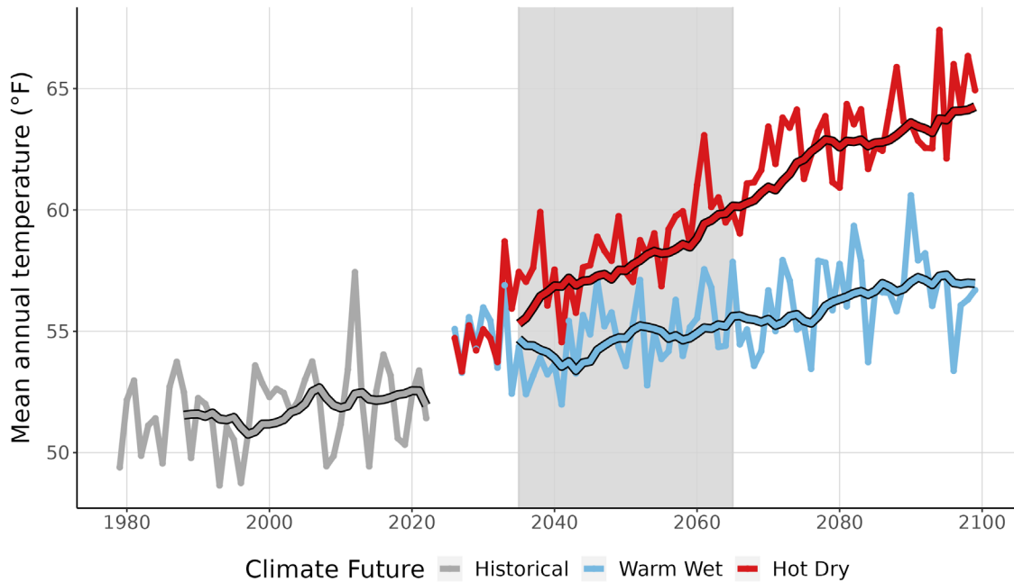
Figure 3. This graph compares observed average annual temperature at LECL (°F) (1979-2022) with projected average annual temperature for the two climate futures over the period 2023-2099. The historically observed data is shown in gray, the Warm Wet climate future in blue, and the Hot Dry climate future in red. The smooth line running through each projection is the 10-year running average for historical observations and future projections. Gray-shaded area represents the time period that was averaged (2035-2065) to summarize future projections for the year 2050 (Appendix 1).
