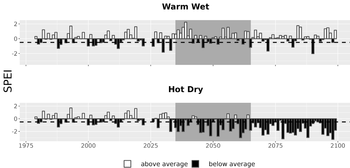
Figure 7. Drought metrics for LECL. Drought index (SPEI; units = standard deviations from historical) timeseries for each climate future. Below-average SPEI (black bars) indicates dry conditions. The dotted line (SPEI = -0.5) indicates drought conditions.
