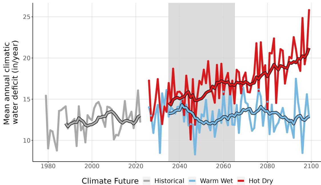
Figure 9. This line graph compares observed climatic water deficit at LARO (inches/year) (1979-2022) with projected climatic water deficit for the two climate futures over the period 2023-2099. The historical observation data is shown in gray, the Warm Wet climate future in blue, and the Hot Dry climate future in red. The smooth line running through each projection is the 10-year running average for historical observations and future projections. Gray-shaded area represents the time period that was averaged (2035-2065) to summarize future projections for the year 2050.
