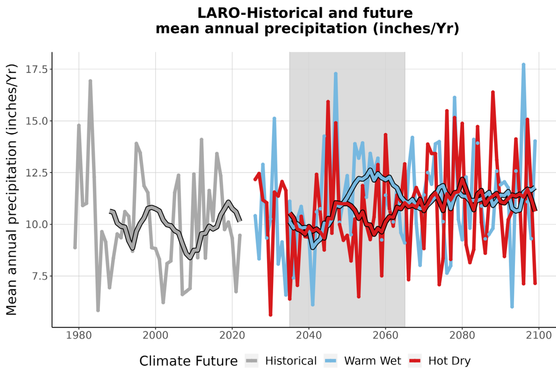
Figure 4. This graph compares observed average annual precipitation at LARO (inches/year) (1979-2022) with projected average annual precipitation for the two climate futures over the period 2023-2099. The historically observed data is shown in gray, the Warm Wet climate future in blue, and the Hot Dry climate future in red. The smooth line running through each projection is the 10-year running average for historical observations and future projections. The gray-shaded area represents the time period that was averaged (2035-2065) to summarize future projections for the year 2050 (Appendix 1).
