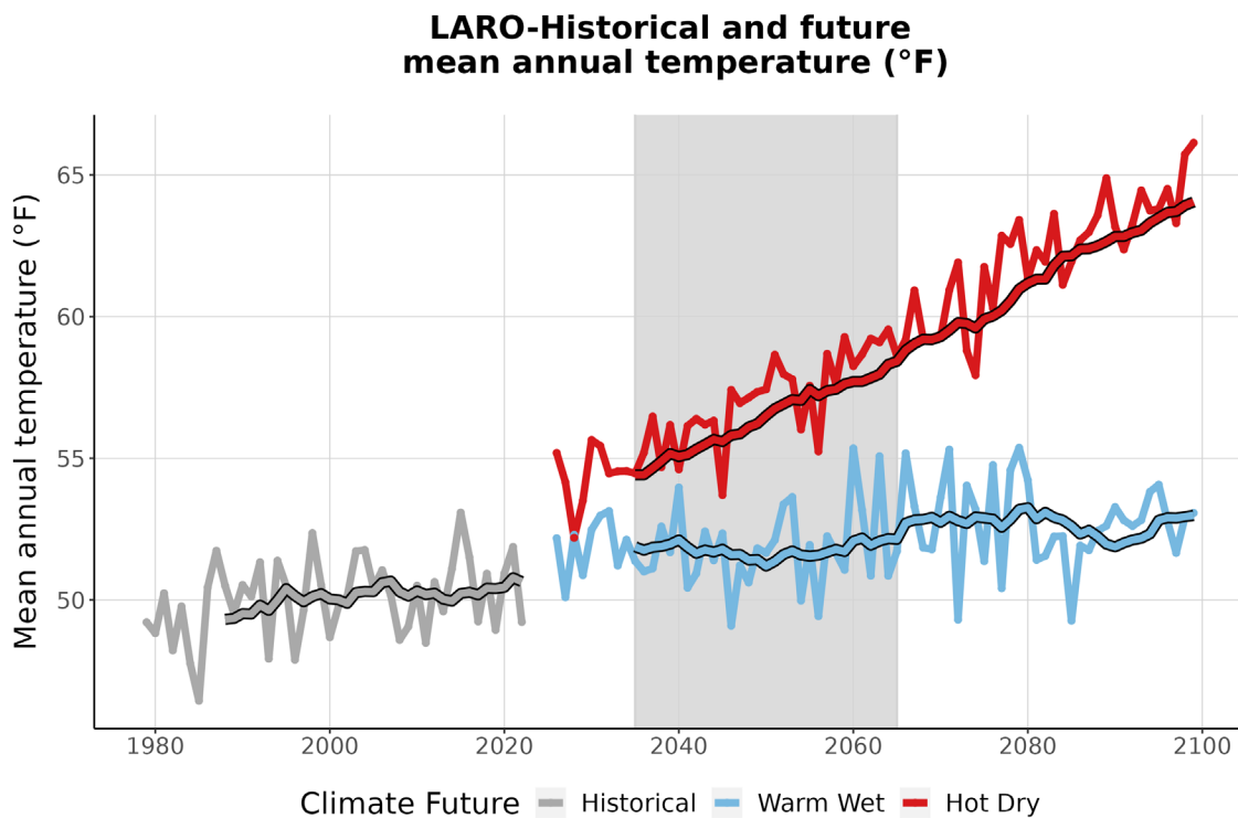
Figure 3. This graph compares observed average annual temperature at LARO (°F) (1979-2022) with projected average annual temperature for the two climate futures over the period 2023-2099. The historically observed data is shown in gray, the Warm Wet climate future in blue, and the Hot Dry climate future in red. The smooth line
