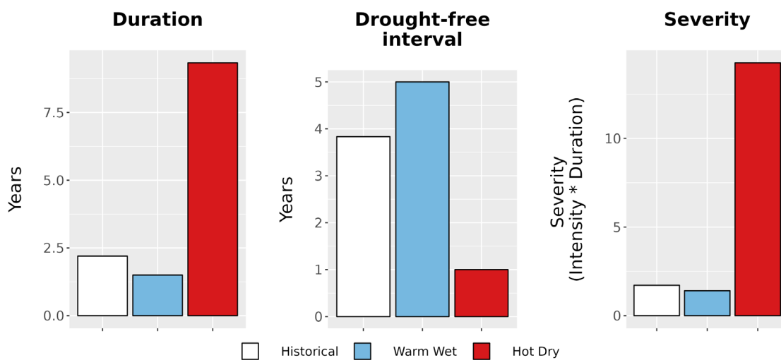
Figure 8. Drought metrics for LARO. (Left) Average drought duration (years) historically (1979-2012) and under each climate future. (Middle) Average drought return interval (years), indicating the expected amount of time between periods of drought, historically and under each climate future. (Right) Average drought severity, a measure of drought intensity multiplied by duration, historically and under each climate future.
