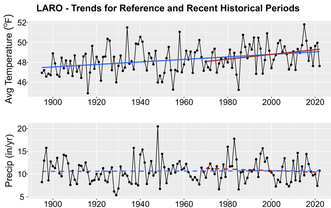
Figure 1. Historical trends in annual average temperature (upper plot) and annual total precipitation (lower plot) for LARO from 1895-2022. Black points show yearly values while blue lines are linear regressions for the entire period record and red lines for 1970-2022 trends. Solid lines are significant trends (i.e., p < 0.05 ); dashed lines are not statistically significant.
