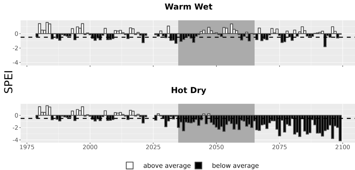
Figure 7. Drought metrics for LARO. Drought index (SPEI; units = standard deviations from historical) timeseries for each climate future. Below-average SPEI (black bars) indicates dry conditions. The dotted line (SPEI = -0.5) indicates drought conditions.
