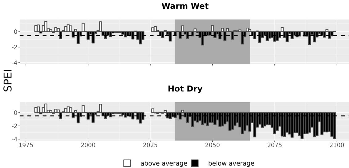
Figure 7. Drought metrics for LAKE. Drought index (SPEI; units = standard deviations from historical) timeseries for each climate future. Below-average SPEI (black bars) indicates dry conditions. The dotted line (SPEI = -0.5) indicates drought conditions.
