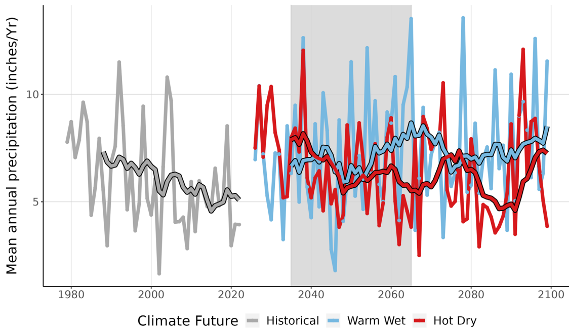
Figure 4. This graph compares observed average annual precipitation at LAKE (inches/year) (1979-2022) with projected average annual precipitation for the two climate futures over the period 2023-2099. The historically observed data is shown in gray, the Warm Wet climate future in blue, and the Hot Dry climate future in red. The smooth line running through each projection is the 10-year running average for historical observations and future projections. The gray-shaded area represents the time period that was averaged (2035-2065) to summarize future projections for the year 2050 (Appendix 1).
