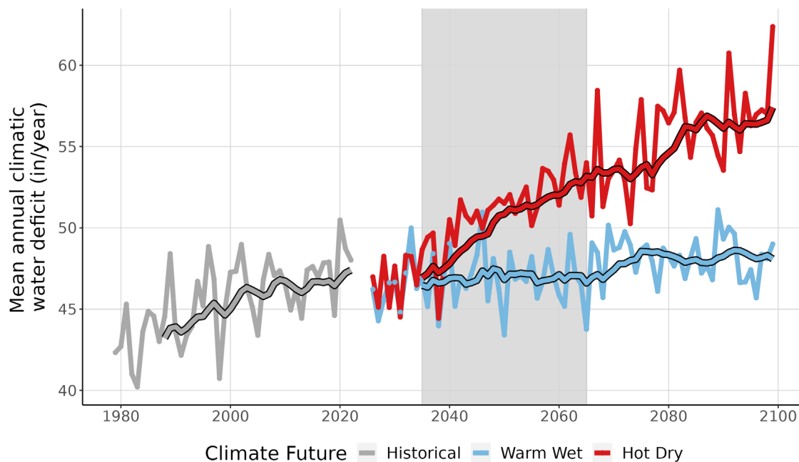
Figure 9. This line graph compares observed climatic water deficit at LAKE (inches/year) (1979-2022) with projected climatic water deficit for the two climate futures over the period 2023-2099. The historical observation data is shown in gray, the Warm Wet climate future in blue, and the Hot Dry climate future in red. The smooth line running through each projection is the 10-year running average for historical observations and future projections. Gray-shaded area represents the time period that was averaged (2035-2065) to summarize future projections for the year 2050.
