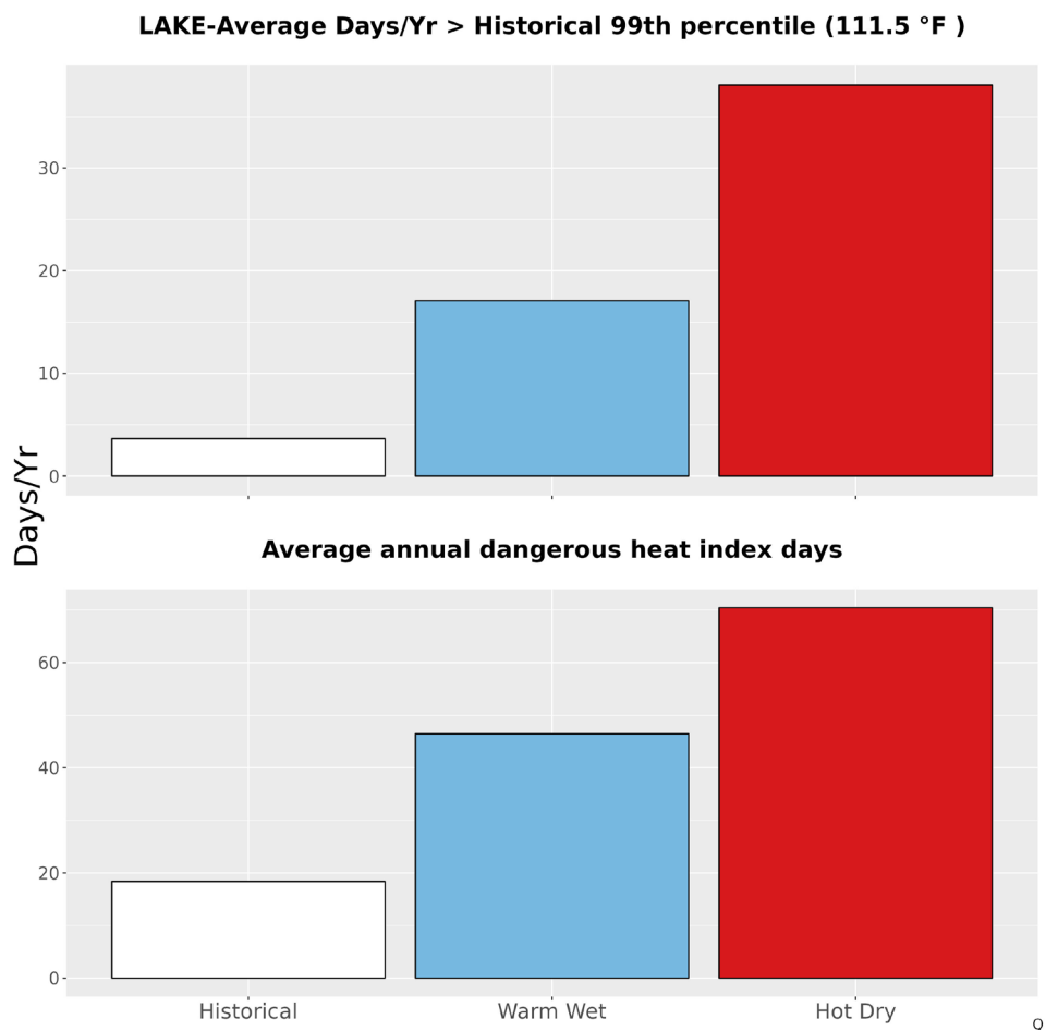
Figure 5. The upper bar graph represents the average number of days annually with temperatures greater than the historical 99th percentile (111.5 °F) historically (1979-2012) and for the two climate futures (2050). The bottom bar graph represents the average annual number of dangerous heat index days historically and for the two climate futures. Dangerous heat index days are days that exceed 105 °F.
