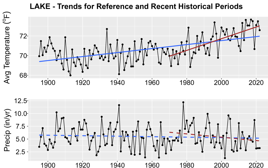
Figure 1. Historical trends in annual average temperature (upper plot) and annual total precipitation (lower plot) for LAKE from 1895-2022. Black points show yearly values while blue lines are linear regressions for the entire period record and red lines for 1970-2022 trends. Solid lines are significant trends (i.e., p < 0.05 ); dashed lines are not statistically significant.
