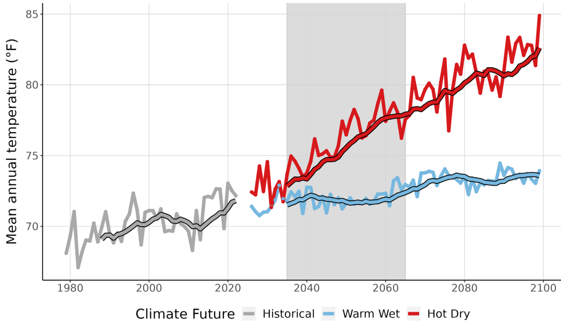
Figure 3. This graph compares observed average annual temperature at LAKE (°F) (1979-2022) with projected average annual temperature for the two climate futures over the period 2023-2099. The historically observed data is shown in gray, the Warm Wet climate future in blue, and the Hot Dry climate future in red. The smooth line running through each projection is the 10-year running average for historical observations and future projections. Gray-shaded area represents the time period that was averaged (2035-2065) to summarize future projections for the year 2050 (Appendix 1).
