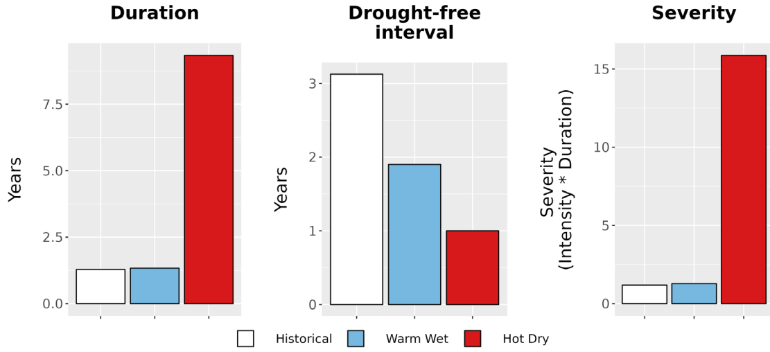
Figure 8. Drought metrics for LAKE. (Left) Average drought duration (years) historically (1979-2012) and under each climate future. (Middle) Average drought return interval (years), indicating the expected amount of time between periods of drought, historically and under each climate future. (Right) Average drought severity, a measure of drought intensity multiplied by duration, historically and under each climate future.
