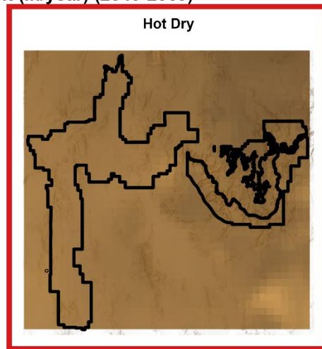
Figure A3. (Top) Map showing average annual climatic water deficit for the historical period (inches/year) and (bottom) change in average annual climatic water deficit for the two climate futures. Legends are located below each set of maps as a continuous color gradient. Gridded data is extracted from Hegewisch, K.C. and J.T. Abatzoglou, 'Climate Mapper' web tool. Climate Toolbox ( https://climatetoolbox.org/ ) accessed on 6/3/2024.
