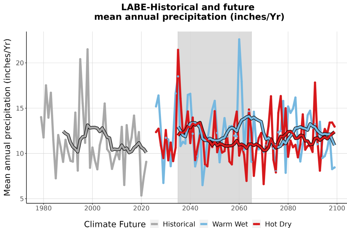
Figure 4. This graph compares observed average annual precipitation at LABE (inches/year) (1979-2022) with projected average annual precipitation for the two climate futures over the period 2023-2099. The historically observed data is shown in gray, the Warm Wet climate future in blue, and the Hot Dry climate future in red. The smooth line running through each projection is the 10-year running average for historical observations and future projections. The gray-shaded area represents the time period that was averaged (2035-2065) to summarize future projections for the year 2050 (Appendix 1).
