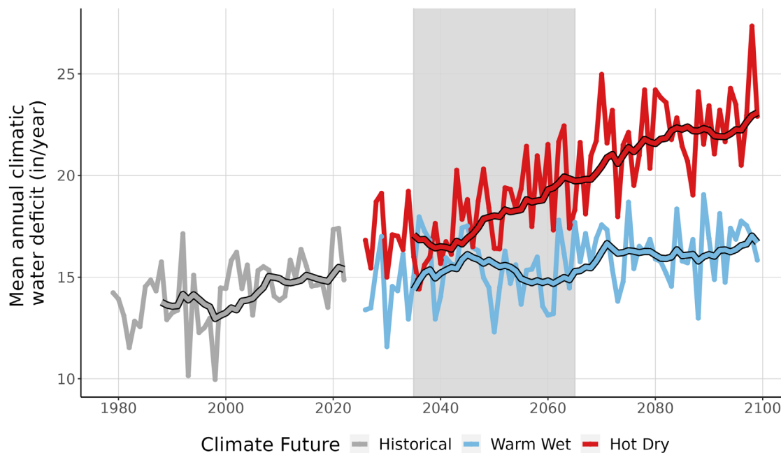
Figure 9. This line graph compares observed climatic water deficit at LABE (inches/year) (1979-2022) with projected climatic water deficit for the two climate futures over the period 2023-2099. The historical observation data is shown in gray, the Warm Wet climate future in blue, and the Hot Dry climate future in red. The smooth line running through each projection is the 10-year running average for historical observations and future projections. Gray-shaded area represents the time period that was averaged (2035-2065) to summarize future projections for the year 2050.
