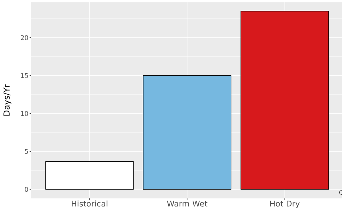
Figure 5. Metrics of extreme temperature at LABE. The bar graph represents the average number of days annually with temperatures greater than the historical 99th percentile (94.7 °F) historically (1979-2012) and for the two climate futures (2050).
