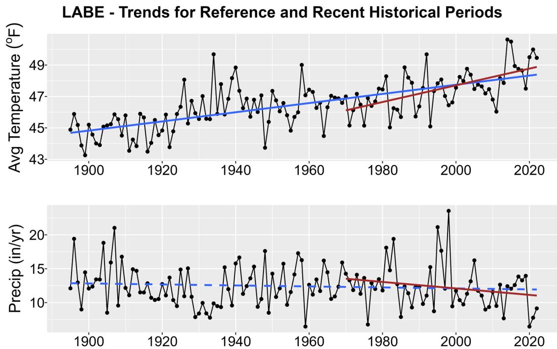
Figure 1. Historical trends in annual average temperature (upper plot) and annual total precipitation (lower plot) for LABE from 1895-2022. Black points show yearly values while blue lines are linear regressions for the entire period record and red lines for 1970-2022 trends. Solid lines are significant trends (i.e., p < 0.05 ); dashed lines are not statistically significant.
