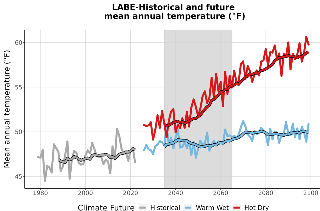
Figure 3. This graph compares observed average annual temperature at LABE (°F) (1979-2022) with projected average annual temperature for the two climate futures over the period 2023-2099. The historically observed data
