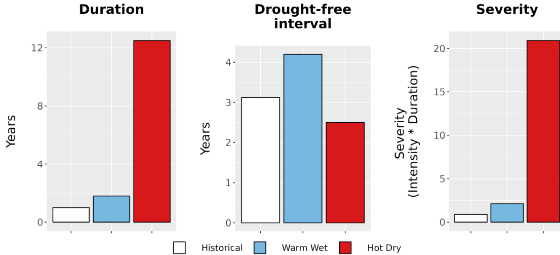
Figure 8. Drought metrics for LABE. (Left) Average drought duration (years) historically (1979-2012) and under each climate future. (Middle) Average drought return interval (years), indicating the expected amount of time between periods of drought, historically and under each climate future. (Right) Average drought severity, a measure of drought intensity multiplied by duration, historically and under each climate future.
