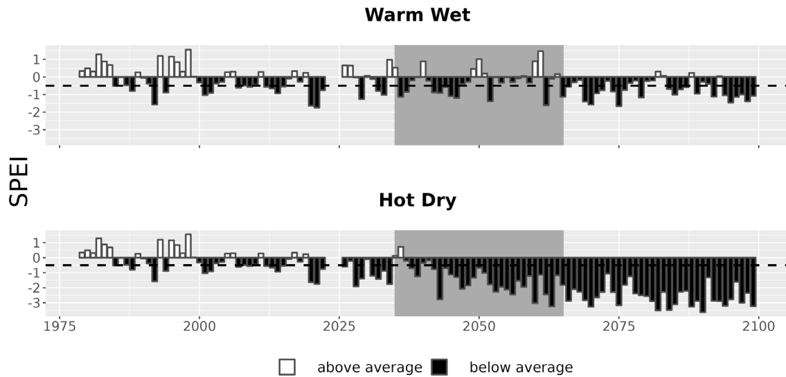
Figure 7. Drought metrics for LABE. Drought index (SPEI; units = standard deviations from historical) timeseries for each climate future. Below-average SPEI (black bars) indicates dry conditions. The dotted line (SPEI = -0.5) indicates drought conditions.
