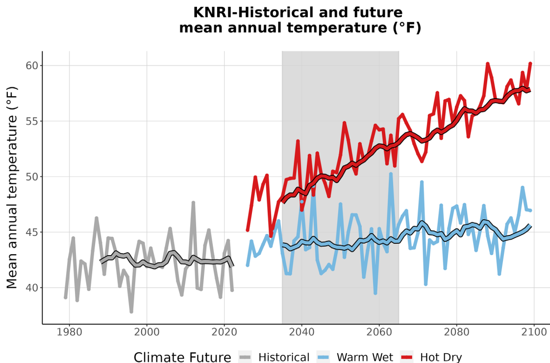
Figure 3. This graph compares observed average annual temperature at KNRI (°F) (1979-2022) with projected average annual temperature for the two climate futures over the period 2023-2099. The historically observed data
