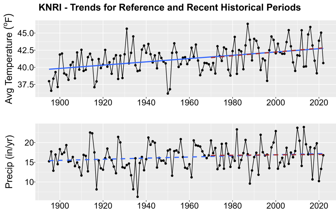
Figure 1. Historical trends in annual average temperature (upper plot) and annual total precipitation (lower plot) for KNRI from 1895-2022. Black points show yearly values while blue lines are linear regressions for the entire period record and red lines for 1970-2022 trends. Solid lines are significant trends (i.e., p < 0.05 ); dashed lines are not statistically significant.
