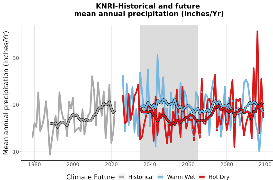
Figure 4. This graph compares observed average annual precipitation at KNRI (inches/year) (1979-2022) with projected average annual precipitation for the two climate futures over the period 2023-2099. The historically observed data is shown in gray, the Warm Wet climate future in blue, and the Hot Dry climate future in red. The smooth line running through each projection is the 10-year running average for historical observations and future projections. The gray-shaded area represents the time period that was averaged (2035-2065) to summarize future projections for the year 2050 (Appendix 1).
