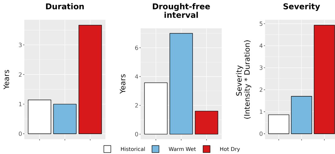
Figure 8. Drought metrics for KNRI. (Left) Average drought duration (years) historically (1979-2012) and under each climate future. (Middle) Average drought return interval (years), indicating the expected amount of time between periods of drought, historically and under each climate future. (Right) Average drought severity, a measure of drought intensity multiplied by duration, historically and under each climate future.
