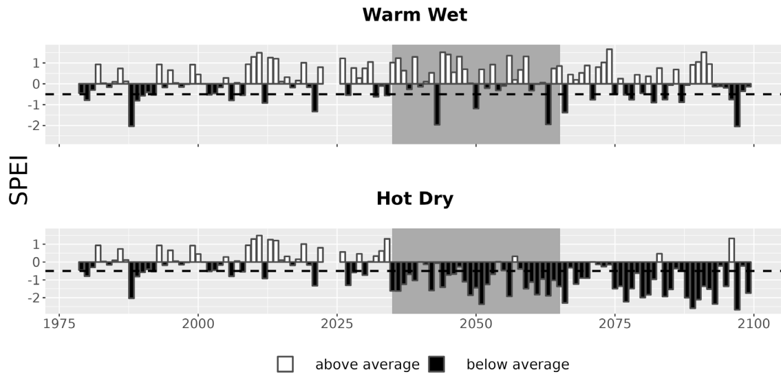
Figure 7. Drought metrics for KNRI. Drought index (SPEI; units = standard deviations from historical) timeseries for each climate future. Below-average SPEI (black bars) indicates dry conditions. The dotted line (SPEI = -0.5) indicates drought conditions.
