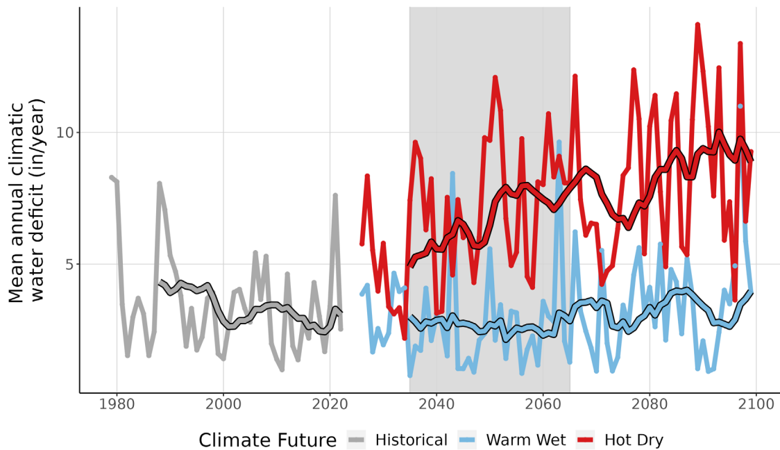
Figure 9. This line graph compares observed climatic water deficit at KNRI (inches/year) (1979-2022) with projected climatic water deficit for the two climate futures over the period 2023-2099. The historical observation data is shown in gray, the Warm Wet climate future in blue, and the Hot Dry climate future in red. The smooth line running through each projection is the 10-year running average for historical observations and future projections. Gray-shaded area represents the time period that was averaged (2035-2065) to summarize future projections for the year 2050.
