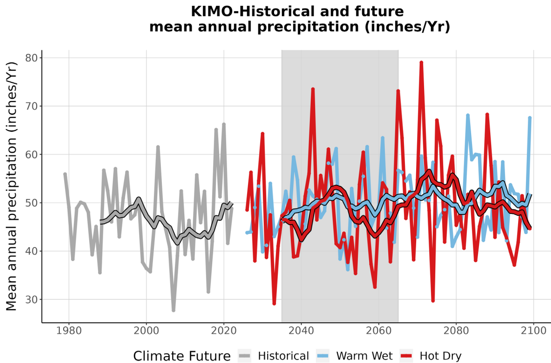
Figure 4. This graph compares observed average annual precipitation at KIMO (inches/year) (1979-2022) with projected average annual precipitation for the two climate futures over the period 2023-2099. The historically observed data is shown in gray, the Warm Wet climate future in blue, and the Hot Dry climate future in red. The smooth line running through each projection is the 10-year running average for historical observations and future projections. The gray-shaded area represents the time period that was averaged (2035-2065) to summarize future projections for the year 2050 (Appendix 1).
