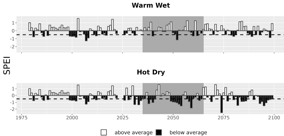
Figure 7. Drought metrics for KIMO. Drought index (SPEI; units = standard deviations from historical) timeseries for each climate future. Below-average SPEI (black bars) indicates dry conditions. The dotted line (SPEI = -0.5) indicates drought conditions.
