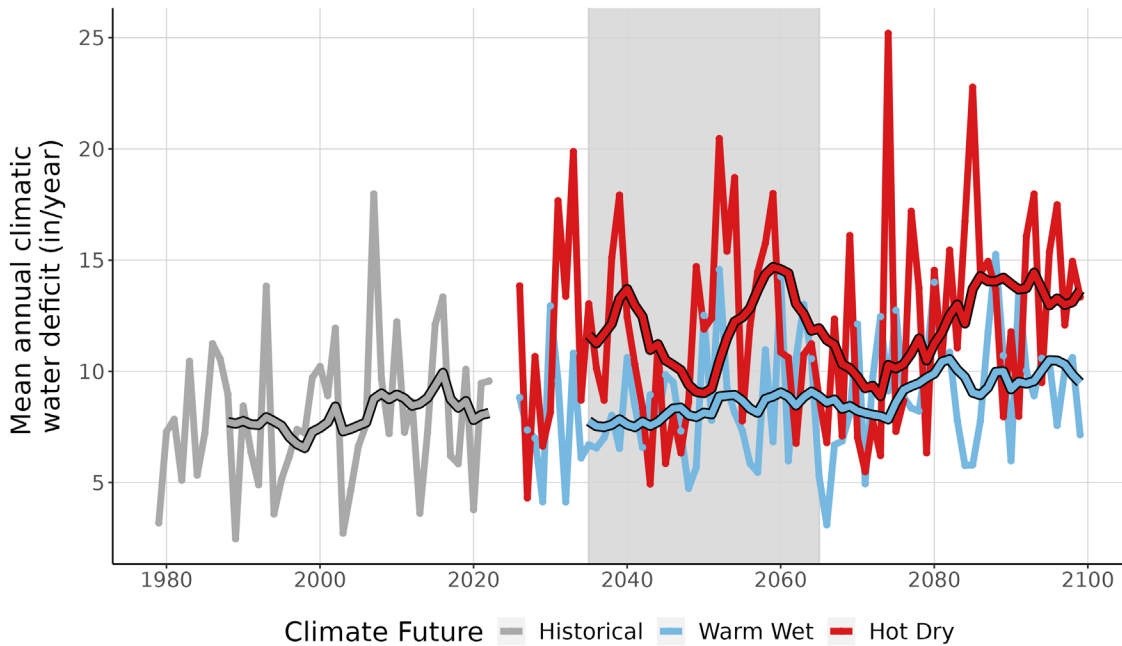
Figure 9. This line graph compares observed climatic water deficit at KIMO (inches/year) (1979-2022) with projected climatic water deficit for the two climate futures over the period 2023-2099. The historical observation data is shown in gray, the Warm Wet climate future in blue, and the Hot Dry climate future in red. The smooth line running through each projection is the 10-year running average for historical observations and future projections. Gray-shaded area represents the time period that was averaged (2035-2065) to summarize future projections for the year 2050.
