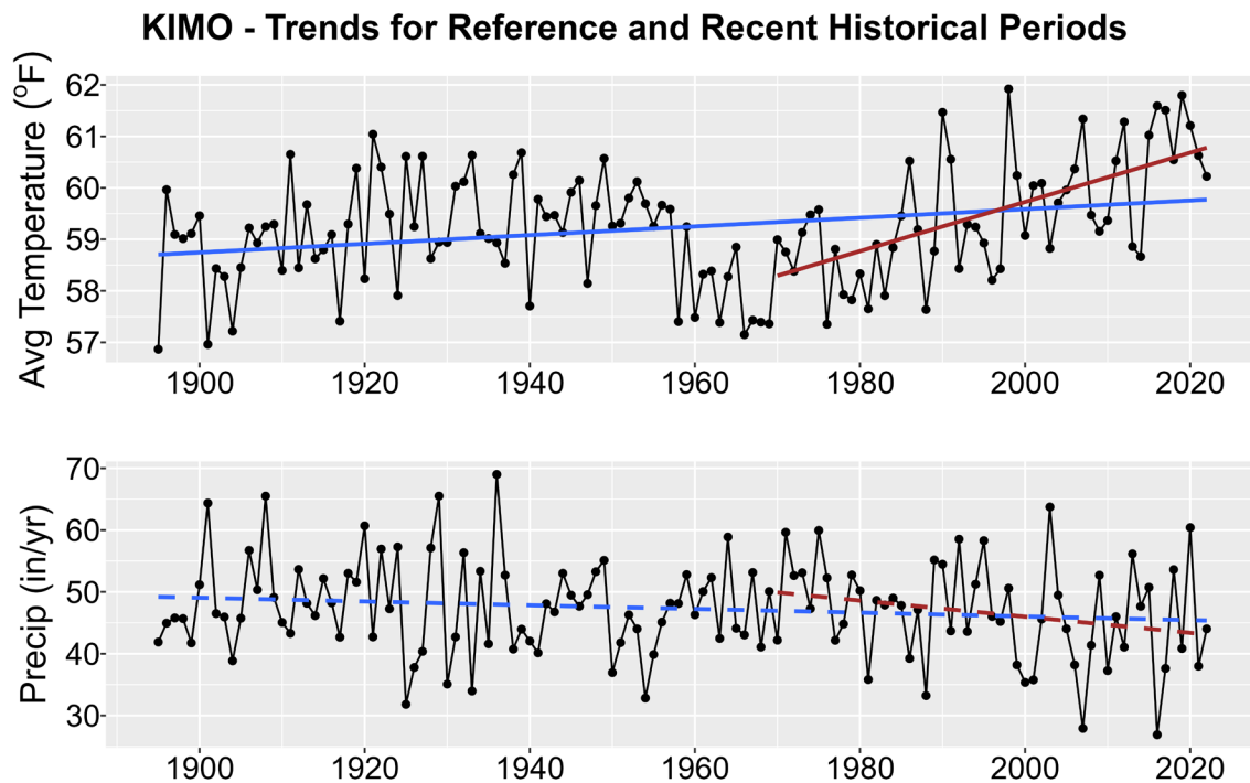
Figure 1. Historical trends in annual average temperature (upper plot) and annual total precipitation (lower plot) for KIMO from 1895-2022. Black points show yearly values while blue lines are linear regressions for the entire period record and red lines for 1970-2022 trends. Solid lines are significant trends (i.e., p < 0.05 ); dashed lines are not statistically significant.
