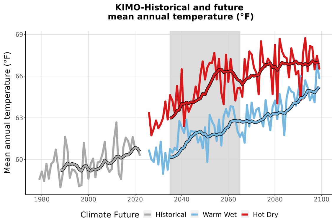
Figure 3. This graph compares observed average annual temperature at KIMO (°F) (1979-2022) with projected average annual temperature for the two climate futures over the period 2023-2099. The historically observed data
