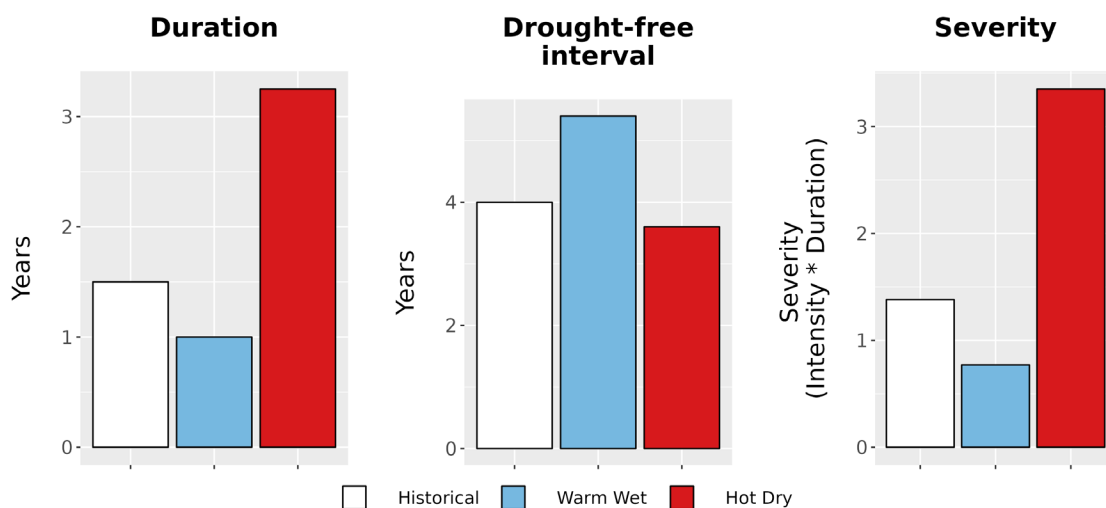
Figure 8. Drought metrics for KIMO. (Left) Average drought duration (years) historically (1979-2012) and under each climate future. (Middle) Average drought return interval (years), indicating the expected amount of time between periods of drought, historically and under each climate future. (Right) Average drought severity, a measure of drought intensity multiplied by duration, historically and under each climate future.
