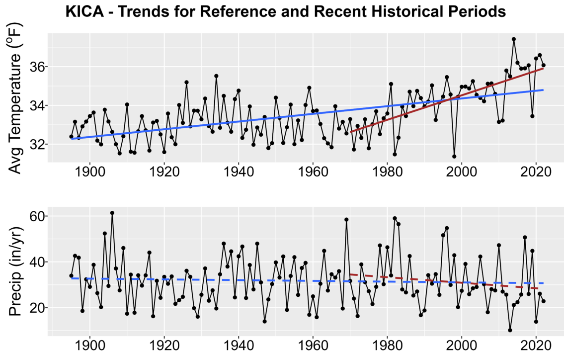
Figure 1. Historical trends in annual average temperature (upper plot) and annual total precipitation (lower plot) for KICA from 1895-2022. Black points show yearly values while blue lines are linear regressions for the entire period record and red lines for 1970-2022 trends. Solid lines are significant trends (i.e., p < 0.05 ); dashed lines are not statistically significant.
