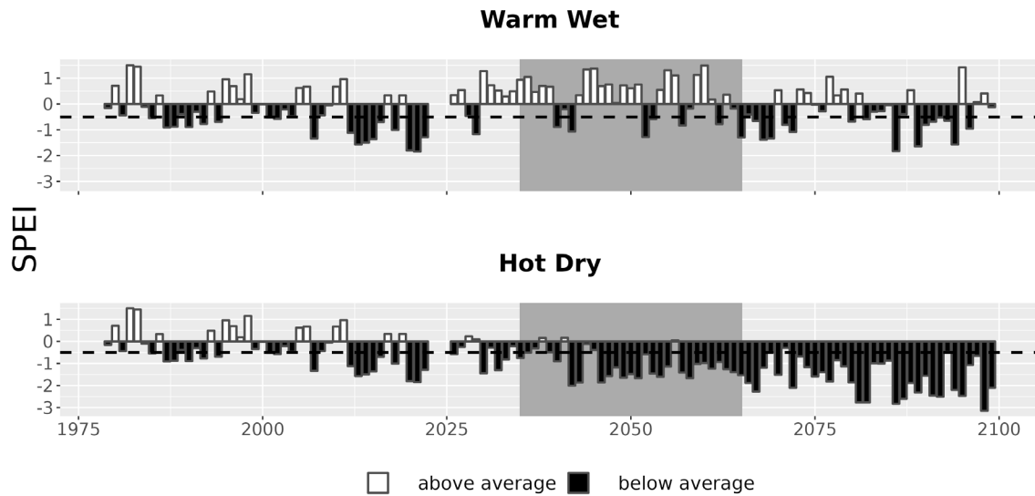
Figure 7. Drought metrics for KICA. Drought index (SPEI; units = standard deviations from historical) timeseries for each climate future. Below-average SPEI (black bars) indicates dry conditions. The dotted line (SPEI = -0.5) indicates drought conditions.
