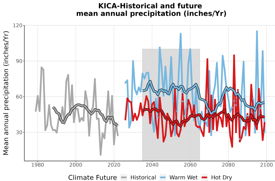
Figure 4. This graph compares observed average annual precipitation at KICA (inches/year) (1979-2022) with projected average annual precipitation for the two climate futures over the period 2023-2099. The historically observed data is shown in gray, the Warm Wet climate future in blue, and the Hot Dry climate future in red. The smooth line running through each projection is the 10-year running average for historical observations and future projections. The gray-shaded area represents the time period that was averaged (2035-2065) to summarize future projections for the year 2050 (Appendix 1).
