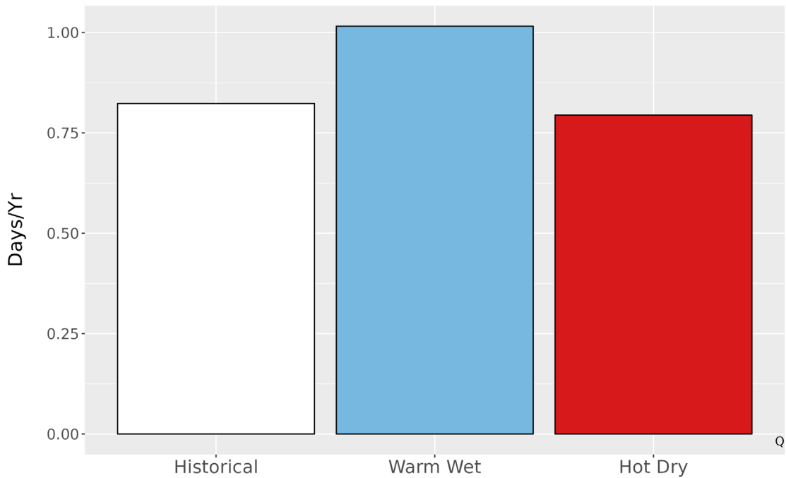
Figure 6. Average number of days annually with precipitation exceeding the 99th percentile (4.4 in.) of precipitation from the historical period 1979-2012 and for each climate future.
