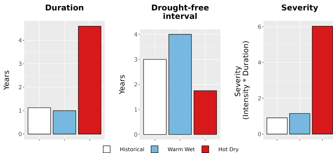
Figure 8. Drought metrics for KICA. (Left) Average drought duration (years) historically (1979-2012) and under each climate future. (Middle) Average drought return interval (years), indicating the expected amount of time between periods of drought, historically and under each climate future. (Right) Average drought severity, a measure of drought intensity multiplied by duration, historically and under each climate future.
