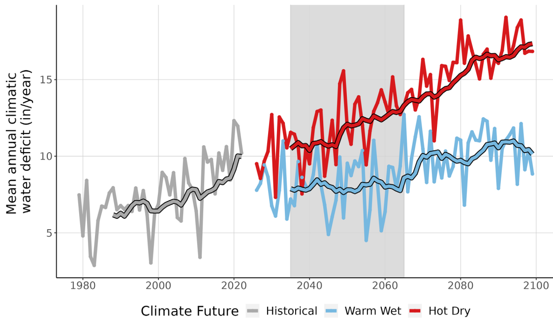
Figure 9. This line graph compares observed climatic water deficit at KICA (inches/year) (1979-2022) with projected climatic water deficit for the two climate futures over the period 2023-2099. The historical observation data is shown in gray, the Warm Wet climate future in blue, and the Hot Dry climate future in red. The smooth line running through each projection is the 10-year running average for historical observations and future projections. Gray-shaded area represents the time period that was averaged (2035-2065) to summarize future projections for the year 2050.
