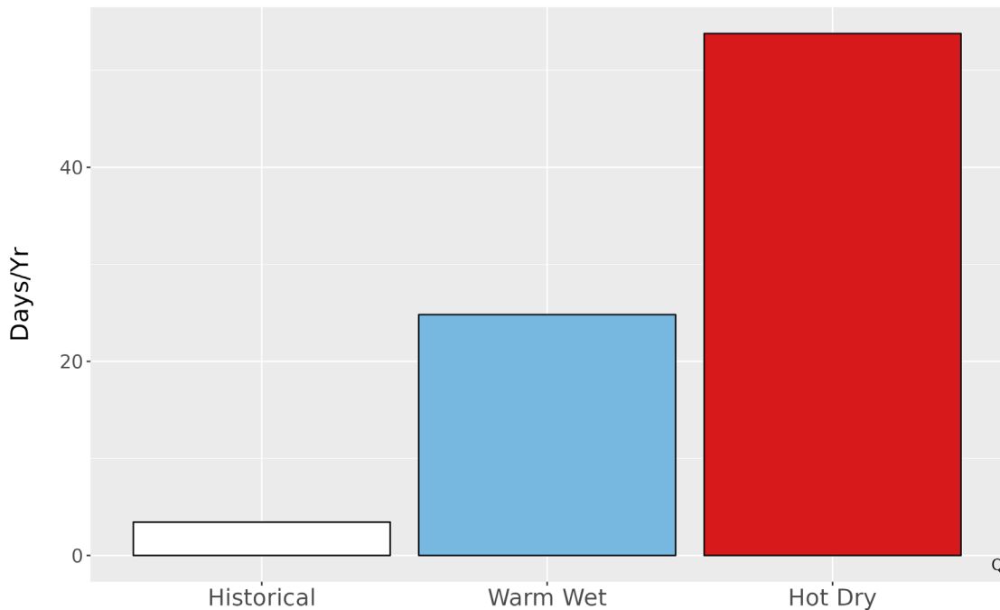
Figure 5. Metrics of extreme temperature at KICA. The bar graph represents the average number of days annually with temperatures greater than the historical 99th percentile (67.9 °F) historically (1979-2012) and for the two climate futures (2050).
