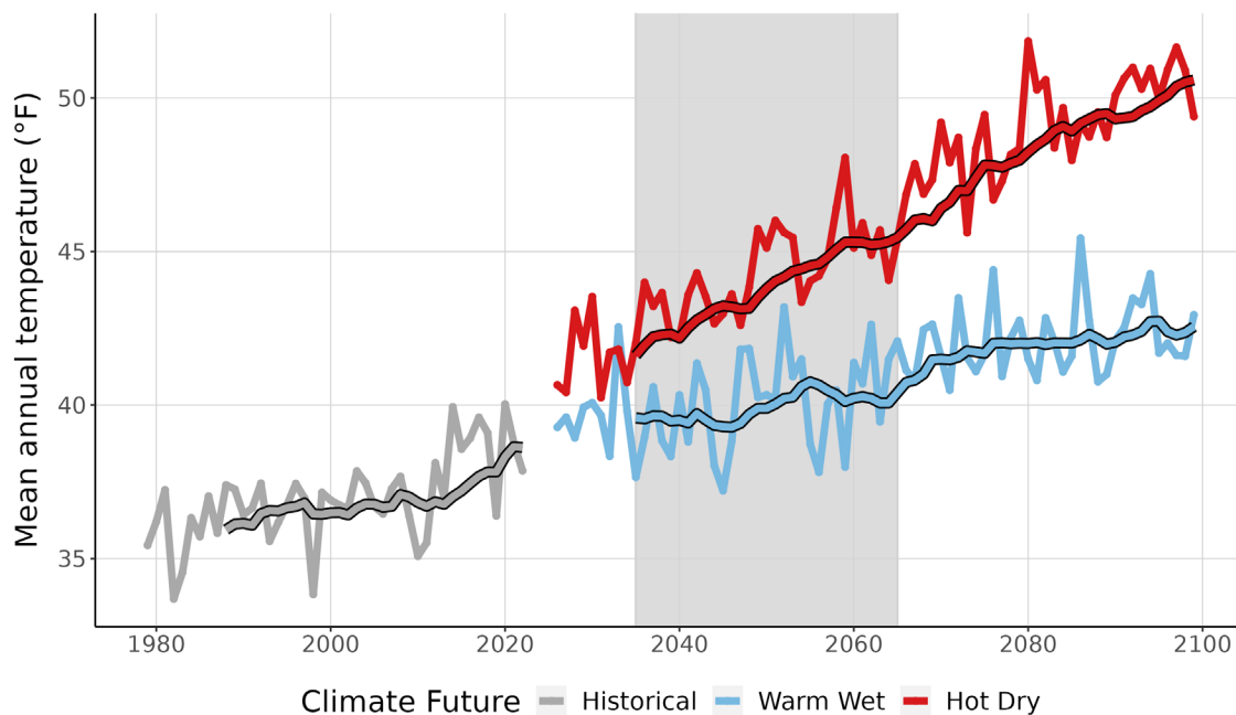
Figure 3. This graph compares observed average annual temperature at KICA (°F) (1979-2022) with projected average annual temperature for the two climate futures over the period 2023-2099. The historically observed data is shown in gray, the Warm Wet climate future in blue, and the Hot Dry climate future in red. The smooth line running through each projection is the 10-year running average for historical observations and future projections. Gray-shaded area represents the time period that was averaged (2035-2065) to summarize future projections for the year 2050 (Appendix 1).
