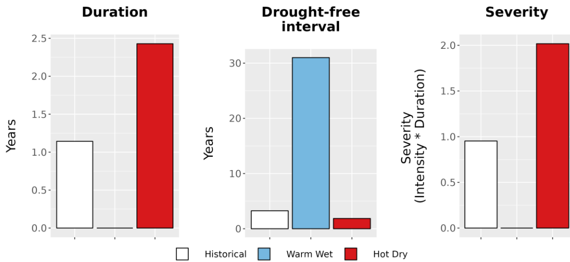
Figure 8. Drought metrics for KEWE. (Left) Average drought duration (years) historically (1979-2012) and under each climate future. (Middle) Average drought return interval (years), indicating the expected amount of time between periods of drought, historically and under each climate future. (Right) Average drought severity, a measure of drought intensity multiplied by duration, historically and under each climate future.
