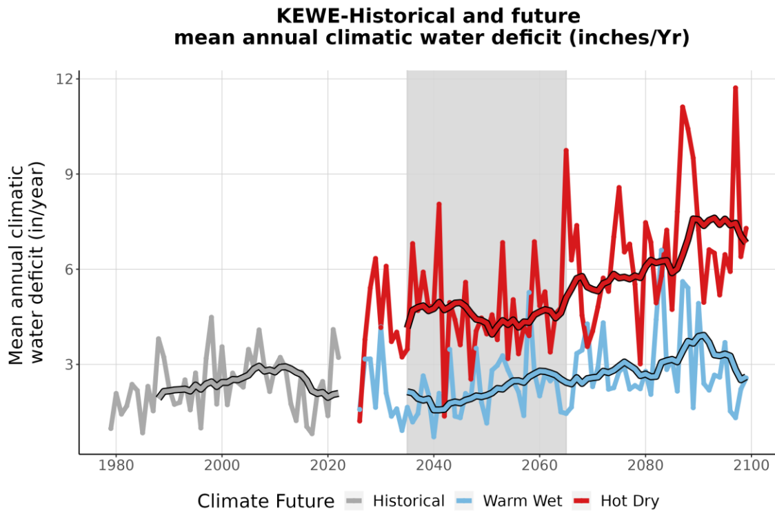
Figure 9. This line graph compares observed climatic water deficit at KEWE (inches/year) (1979-2022) with projected climatic water deficit for the two climate futures over the period 2023-2099. The historical observation data is shown in gray, the Warm Wet climate future in blue, and the Hot Dry climate future in red. The smooth line running through each projection is the 10-year running average for historical observations and future projections. Gray-shaded area represents the time period that was averaged (2035-2065) to summarize future projections for the year 2050.
