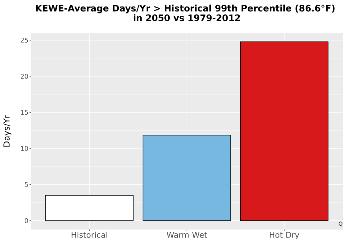
Figure 5. Metrics of extreme temperature at KEWE. The bar graph represents the average number of days annually with temperatures greater than the historical 99th percentile (86.6 °F) historically (1979-2012) and for the two climate futures (2050).
