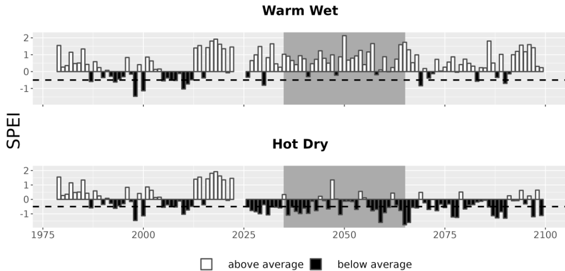
Figure 7. Drought metrics for KEWE. Drought index (SPEI; units = standard deviations from historical) timeseries for each climate future. Below-average SPEI (black bars) indicates dry conditions. The dotted line (SPEI = -0.5) indicates drought conditions.
