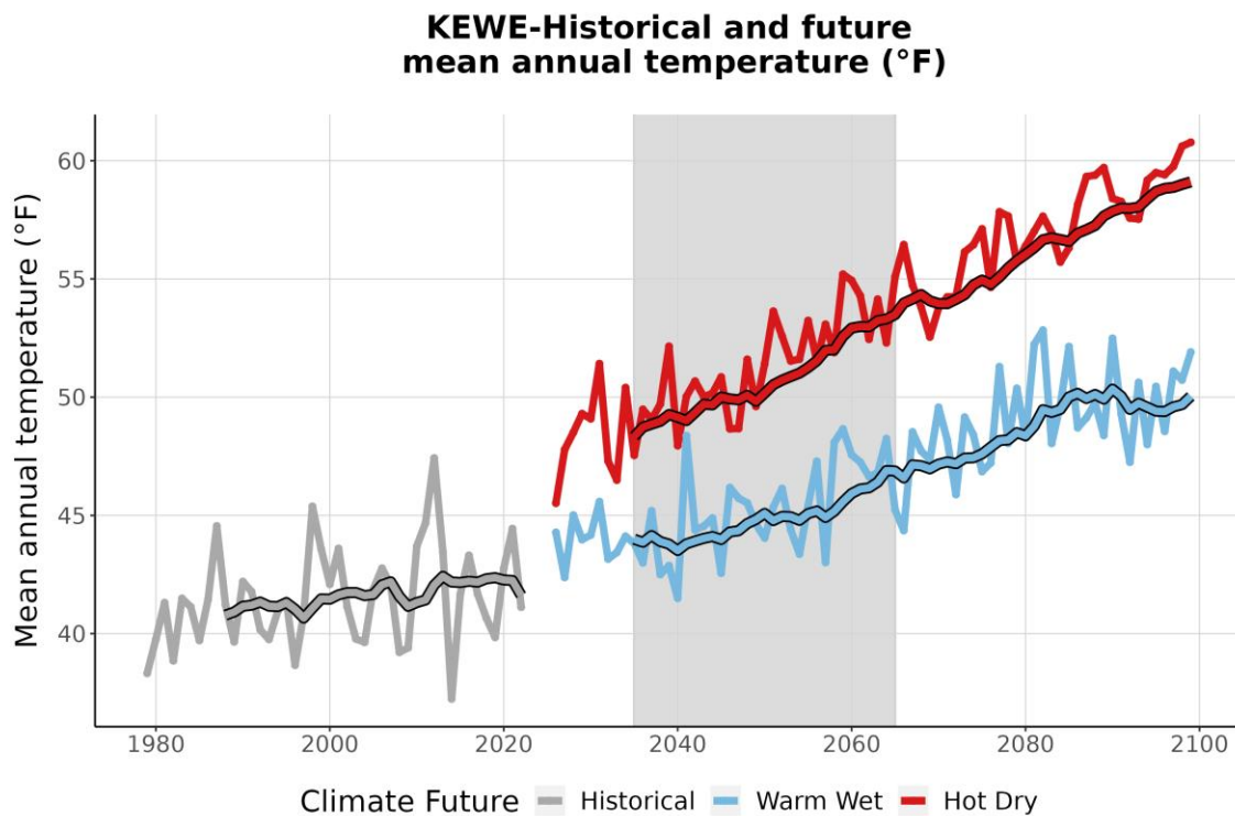
Figure 3. This graph compares observed average annual temperature at KEWE (°F) (1979-2022) with projected average annual temperature for the two climate futures over the period 2023-2099. The historically observed data is shown in gray, the Warm Wet climate future in blue, and the Hot Dry climate future in red. The smooth line
