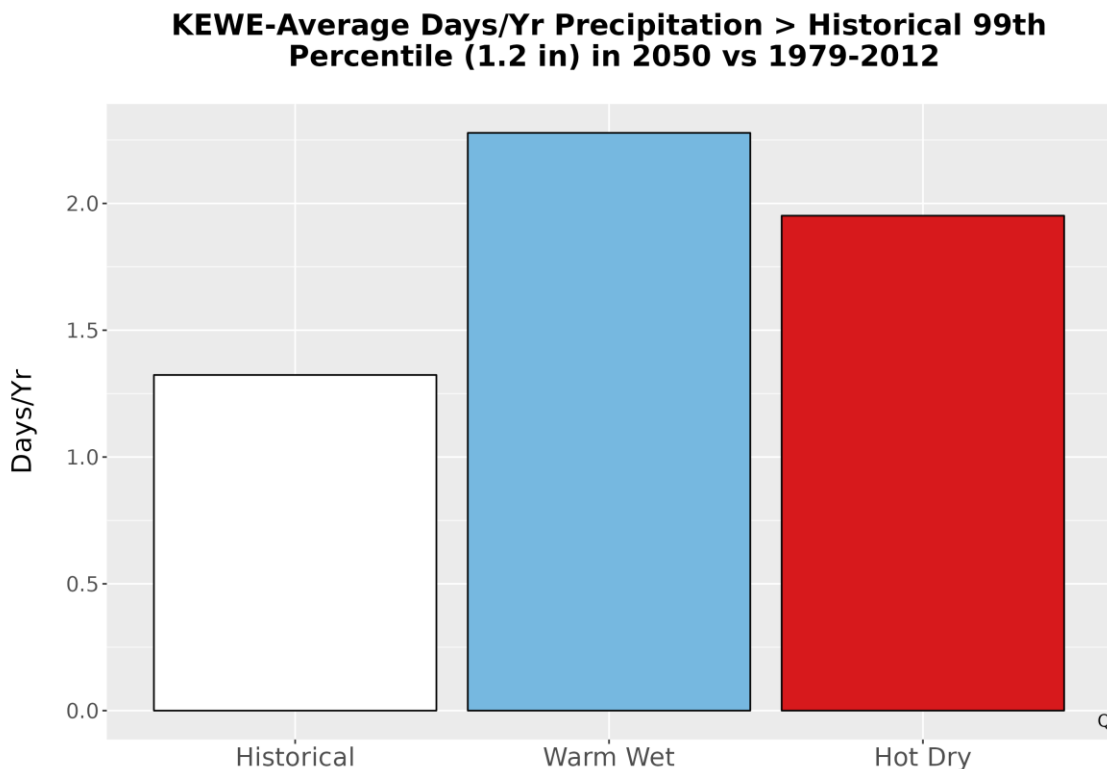
Figure 6. Average number of days annually with precipitation exceeding the 99th percentile (1.2 in.) of precipitation from the historical period 1979-2012 and for each climate future.
