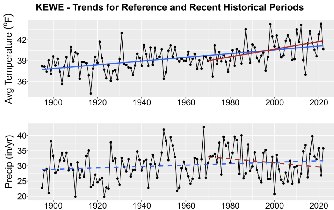
Figure 1. Historical trends in annual average temperature (upper plot) and annual total precipitation (lower plot) for KEWE from 1895-2022. Black points show yearly values while blue lines are linear regressions for the entire period record and red lines for 1970-2022 trends. Solid lines are significant trends (i.e., p < 0.05 ); dashed lines are not statistically significant.
