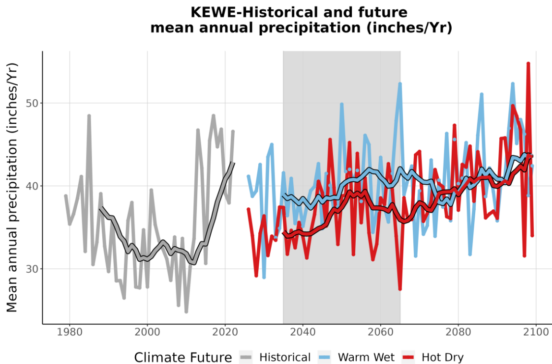
Figure 4. This graph compares observed average annual precipitation at KEWE (inches/year) (1979-2022) with projected average annual precipitation for the two climate futures over the period 2023-2099. The historically observed data is shown in gray, the Warm Wet climate future in blue, and the Hot Dry climate future in red. The smooth line running through each projection is the 10-year running average for historical observations and future projections. The gray-shaded area represents the time period that was averaged (2035-2065) to summarize future projections for the year 2050 (Appendix 1).
