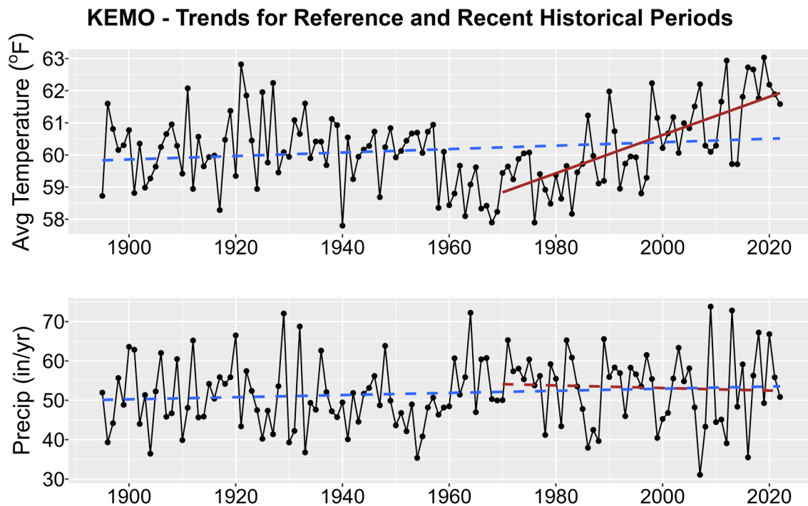
Figure 1. Historical trends in annual average temperature (upper plot) and annual total precipitation (lower plot) for KEMO from 1895-2022. Black points show yearly values while blue lines are linear regressions for the entire period record and red lines for 1970-2022 trends. Solid lines are significant trends (i.e., p < 0.05 ); dashed lines are not statistically significant.
