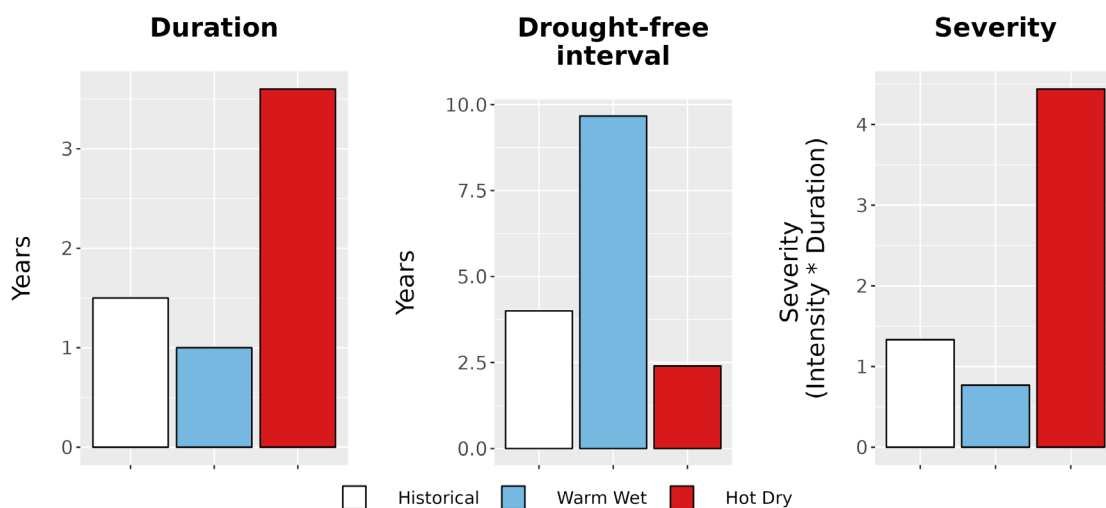
Figure 8. Drought metrics for KEMO. (Left) Average drought duration (years) historically (1979-2012) and under each climate future. (Middle) Average drought return interval (years), indicating the expected amount of time between periods of drought, historically and under each climate future. (Right) Average drought severity, a measure of drought intensity multiplied by duration, historically and under each climate future.
