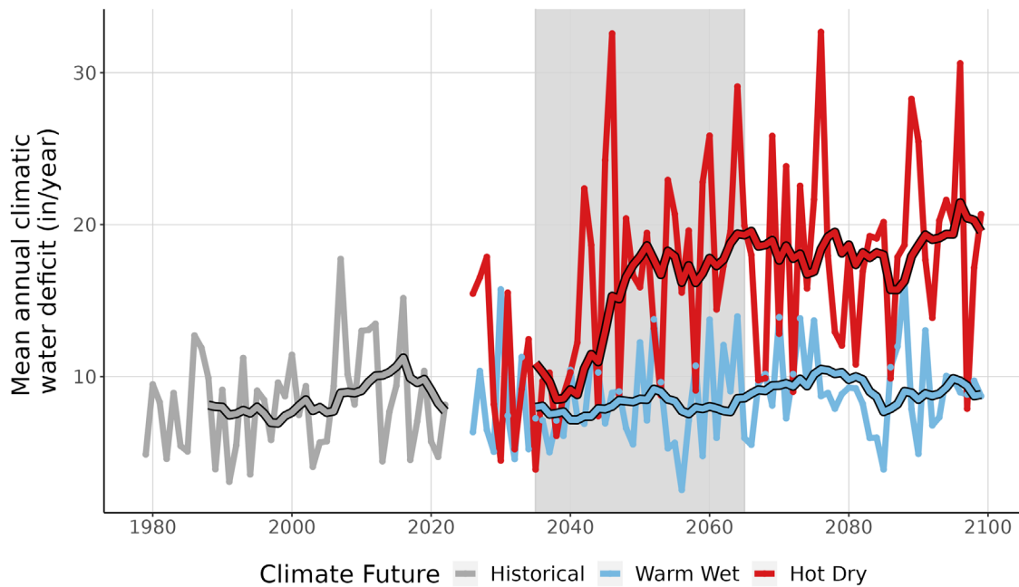
Figure 9. This line graph compares observed climatic water deficit at KEMO (inches/year) (1979-2022) with projected climatic water deficit for the two climate futures over the period 2023-2099. The historical observation data is shown in gray, the Warm Wet climate future in blue, and the Hot Dry climate future in red. The smooth line running through each projection is the 10-year running average for historical observations and future projections. Gray-shaded area represents the time period that was averaged (2035-2065) to summarize future projections for the year 2050.
