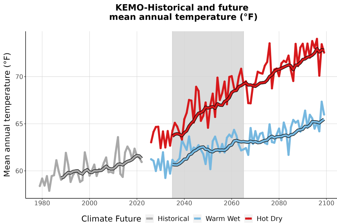
Figure 3. This graph compares observed average annual temperature at KEMO (°F) (1979-2022) with projected average annual temperature for the two climate futures over the period 2023-2099. The historically observed data
