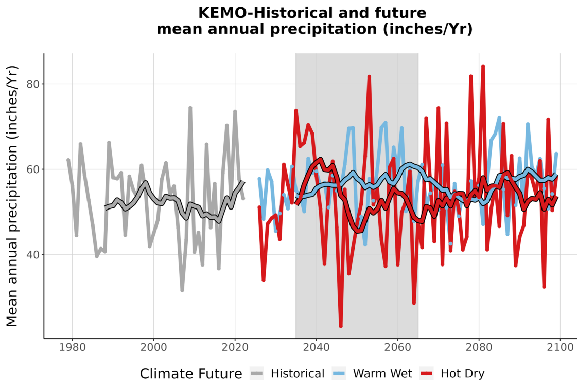
Figure 4. This graph compares observed average annual precipitation at KEMO (inches/year) (1979-2022) with projected average annual precipitation for the two climate futures over the period 2023-2099. The historically observed data is shown in gray, the Warm Wet climate future in blue, and the Hot Dry climate future in red. The smooth line running through each projection is the 10-year running average for historical observations and future projections. The gray-shaded area represents the time period that was averaged (2035-2065) to summarize future projections for the year 2050 (Appendix 1).
