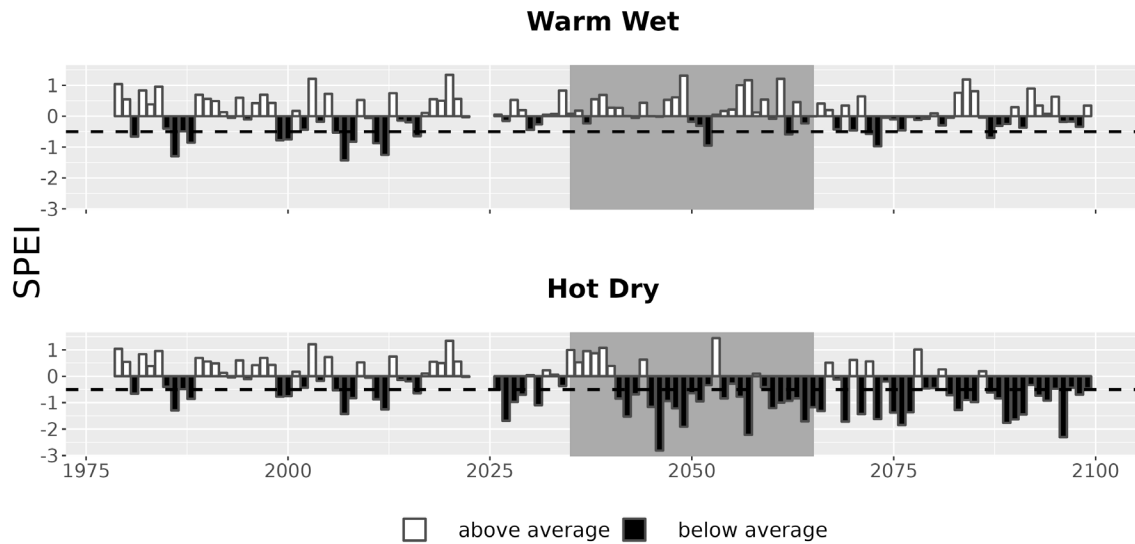
Figure 7. Drought metrics for KEMO. Drought index (SPEI; units = standard deviations from historical) timeseries for each climate future. Below-average SPEI (black bars) indicates dry conditions. The dotted line (SPEI = -0.5) indicates drought conditions.
