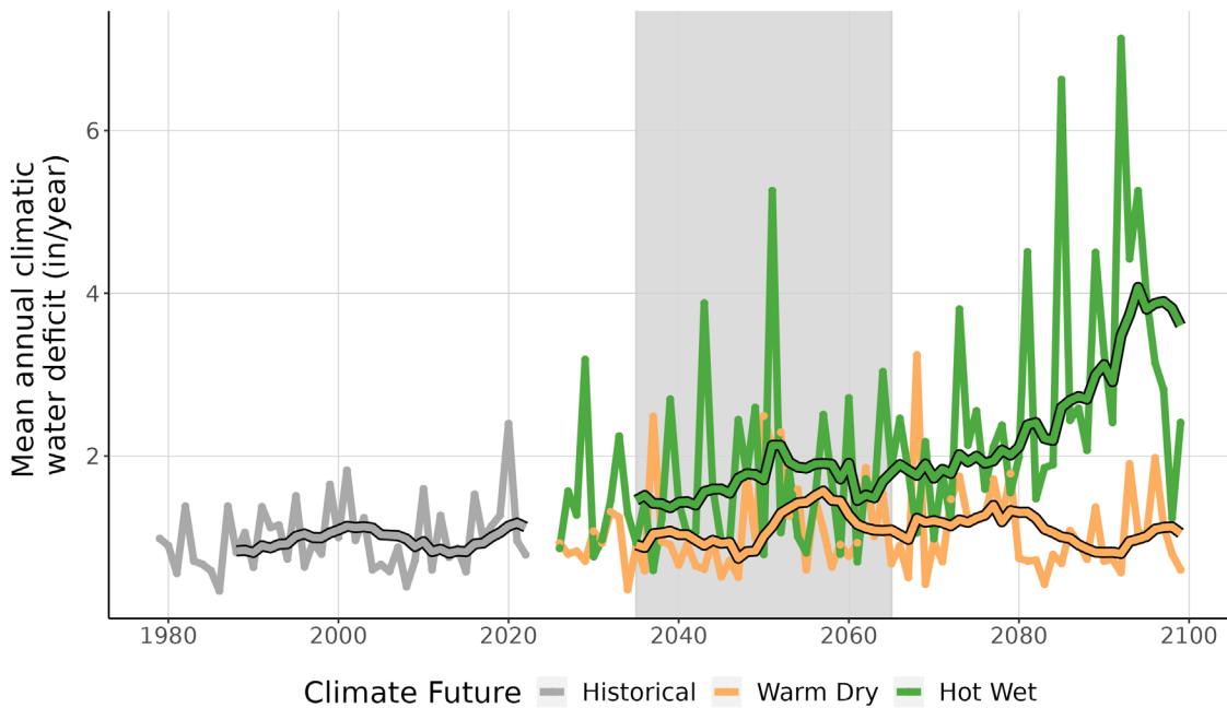
Figure 9. This line graph compares observed climatic water deficit at KAWW (inches/year) (1979-2022) with projected climatic water deficit for the two climate futures over the period 2023-2099. The historical observation data is shown in gray, the Warm Dry climate future in orange, and the Hot Wet climate future in green. The smooth line running through each projection is the 10-year running average for historical observations and future projections. Gray-shaded area represents the time period that was averaged (2035-2065) to summarize future projections for the year 2050.
