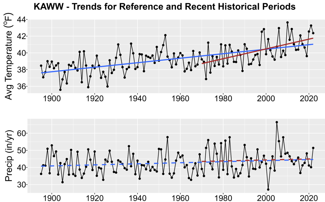
Figure 1. Historical trends in annual average temperature (upper plot) and annual total precipitation (lower plot) for KAWW from 1895-2022. Black points show yearly values while blue lines are linear regressions for the entire period record and red lines for 1970-2022 trends. Solid lines are significant trends (i.e., p < 0.05 ); dashed lines are not statistically significant.
