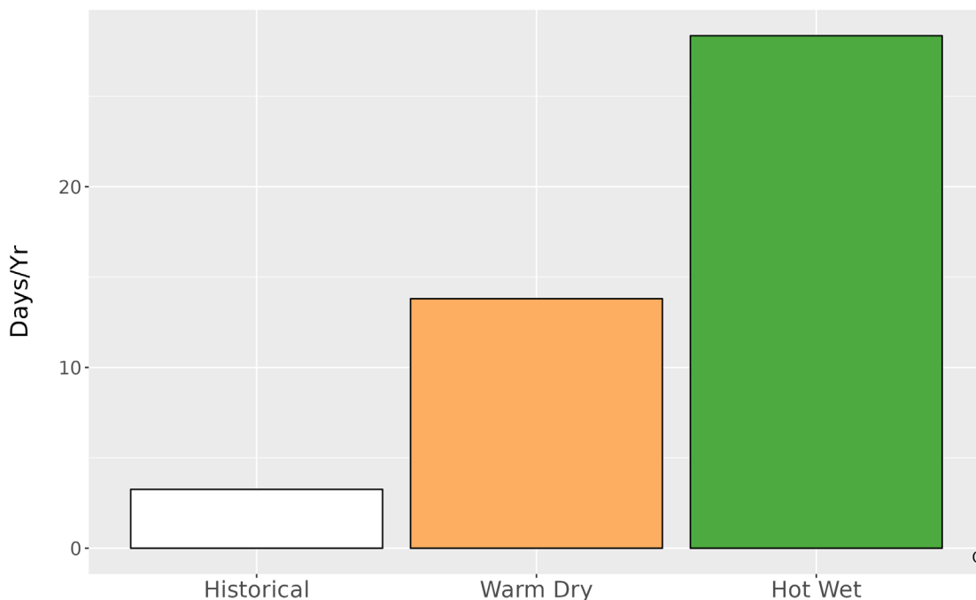
Figure 5. Metrics of extreme temperature at KAWW. The bar graph represents the average number of days annually with temperatures greater than the historical 99th percentile (86.1 °F) historically (1979-2012) and for the two climate futures (2050).
