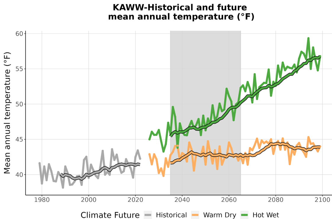
Figure 3. This graph compares observed average annual temperature at KAWW (°F) (1979-2022) with projected average annual temperature for the two climate futures over the period 2023-2099. The historically observed data is shown in gray, the Warm Dry climate future in orange, and the Hot Wet climate future in green. The smooth line
