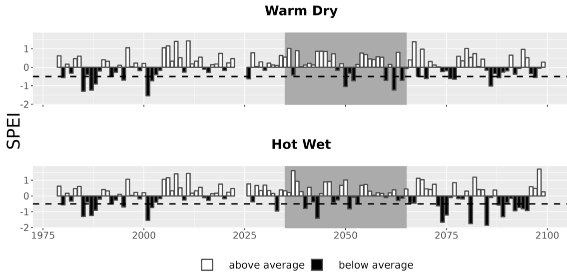
Figure 7. Drought metrics for KAWW. Drought index (SPEI; units = standard deviations from historical) timeseries for each climate future. Below-average SPEI (black bars) indicates dry conditions. The dotted line (SPEI = -0.5) indicates drought conditions.
