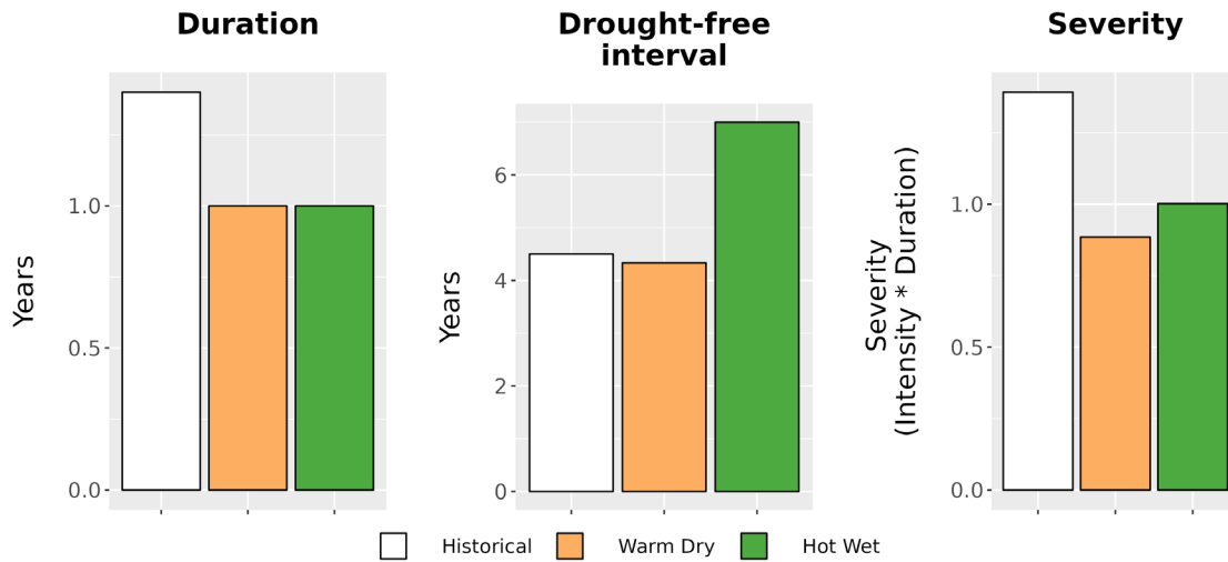
Figure 8. Drought metrics for KAWW. (Left) Average drought duration (years) historically (1979-2012) and under each climate future. (Middle) Average drought return interval (years), indicating the expected amount of time between periods of drought, historically and under each climate future. (Right) Average drought severity, a measure of drought intensity multiplied by duration, historically and under each climate future.
