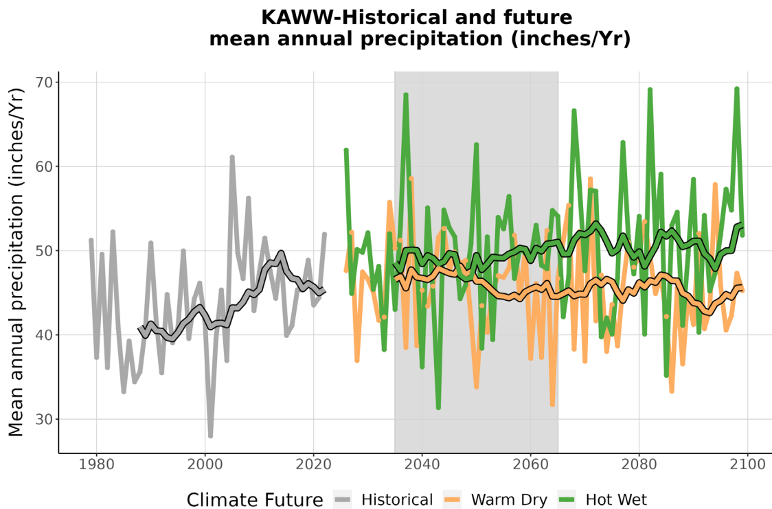
Figure 4. This graph compares observed average annual precipitation at KAWW (inches/year) (1979-2022) with projected average annual precipitation for the two climate futures over the period 2023-2099. The historically observed data is shown in gray, the Warm Dry climate future in orange, and the Hot Wet climate future in green. The smooth line running through each projection is the 10-year running average for historical observations and future projections. The gray-shaded area represents the time period that was averaged (2035-2065) to summarize future projections for the year 2050 (Appendix 1).
