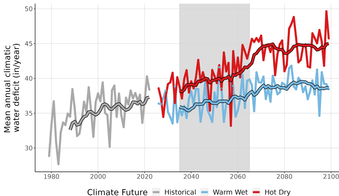
Figure 9. This line graph compares observed climatic water deficit at JOTR (inches/year) (1979-2022) with projected climatic water deficit for the two climate futures over the period 2023-2099. The historical observation data is shown in gray, the Warm Wet climate future in blue, and the Hot Dry climate future in red. The smooth line running through each projection is the 10-year running average for historical observations and future projections. Gray-shaded area represents the time period that was averaged (2035-2065) to summarize future projections for the year 2050.
