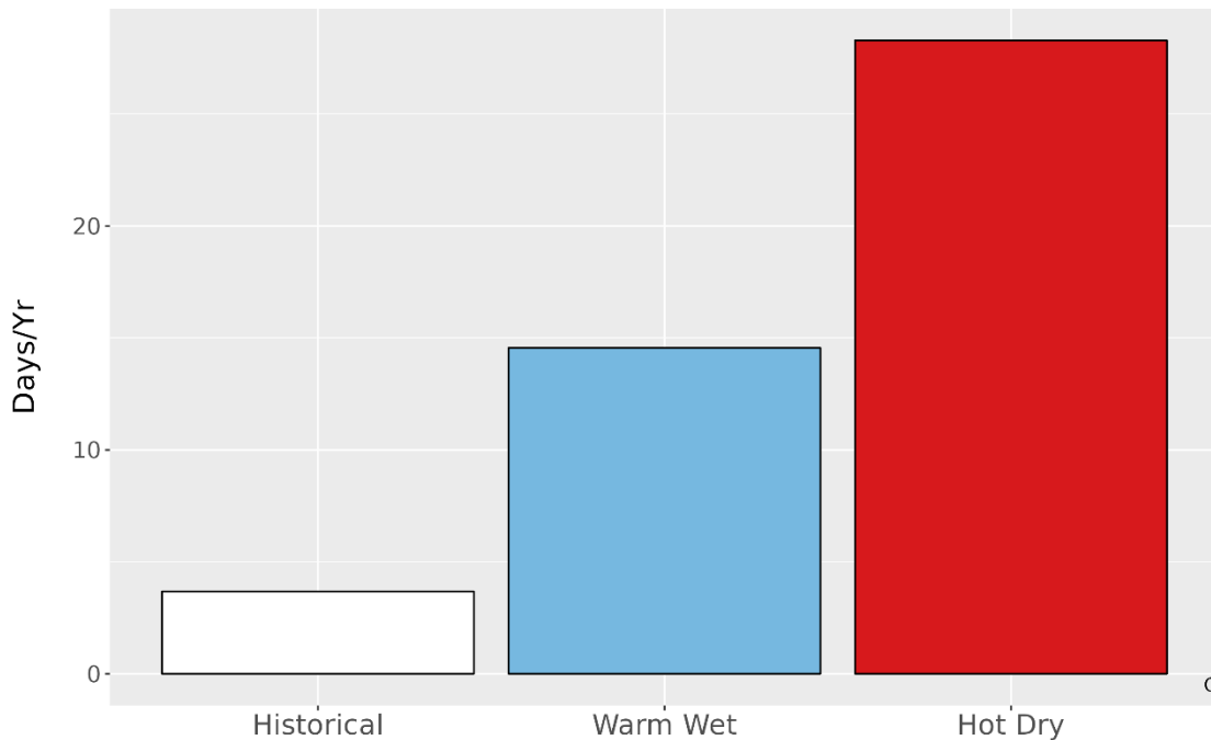
Figure 5. The bar graph represents the average number of days annually with temperatures greater than the historical 99th percentile (102.4 °F) historically (1979-2012) and for the two climate futures (2050).
