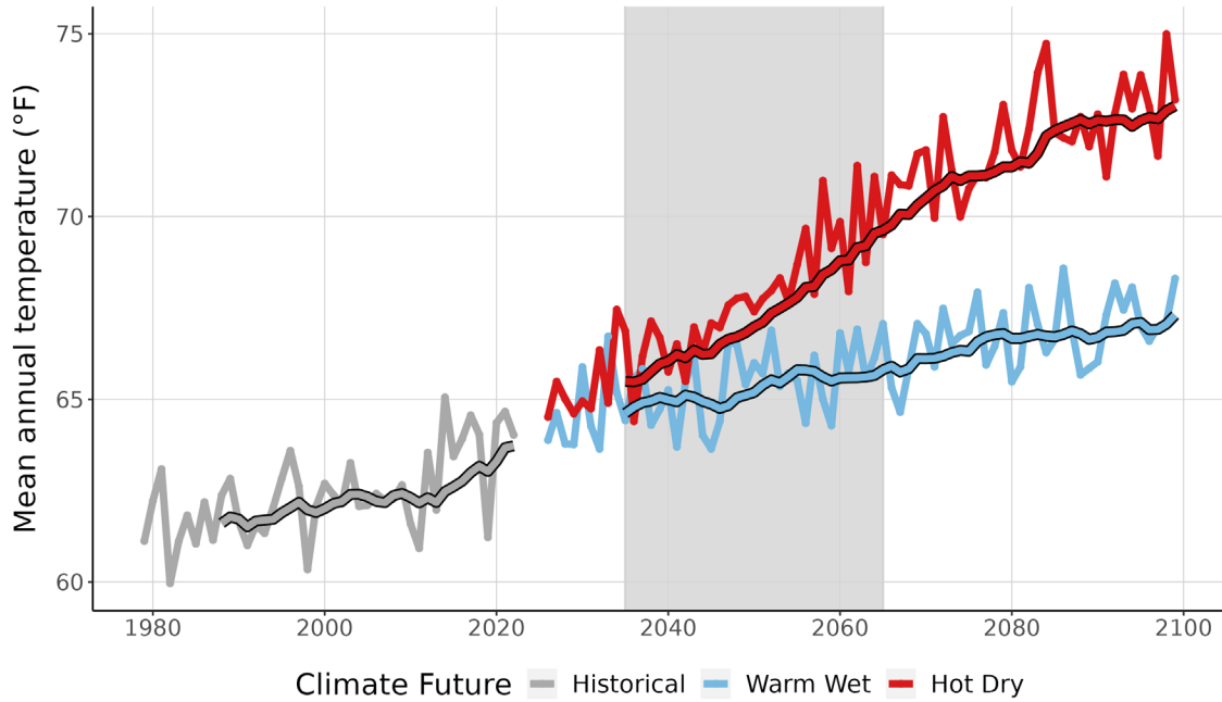
Figure 3. This graph compares observed average annual temperature at JOTR (°F) (1979-2022) with projected average annual temperature for the two climate futures over the period 2023-2099. The historically observed data is shown in gray, the Warm Wet climate future in blue, and the Hot Dry climate future in red. The smooth line running through each projection is the 10-year running average for historical observations and future projections. Gray-shaded area represents the time period that was averaged (2035-2065) to summarize future projections for the year 2050 (Appendix 1).
