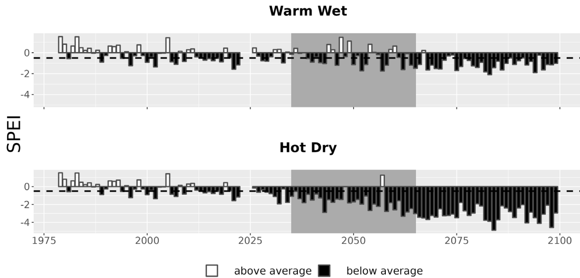
Figure 7. Drought metrics for JOTR. Drought index (SPEI; units = standard deviations from historical) timeseries for each climate future. Below-average SPEI (black bars) indicates dry conditions. The dotted line (SPEI = -0.5) indicates drought conditions.
