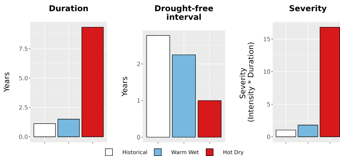
Figure 8. Drought metrics for JOTR. (Left) Average drought duration (years) historically (1979-2012) and under each climate future. (Middle) Average drought return interval (years), indicating the expected amount of time between periods of drought, historically and under each climate future. (Right) Average drought severity, a measure of drought intensity multiplied by duration, historically and under each climate future.
