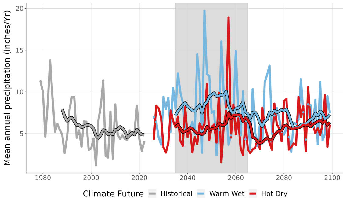
Figure 4. This graph compares observed average annual precipitation at JOTR (inches/year) (1979-2022) with projected average annual precipitation for the two climate futures over the period 2023-2099. The historically observed data is shown in gray, the Warm Wet climate future in blue, and the Hot Dry climate future in red. The smooth line running through each projection is the 10-year running average for historical observations and future projections. The gray-shaded area represents the time period that was averaged (2035-2065) to summarize future projections for the year 2050 (Appendix 1).
