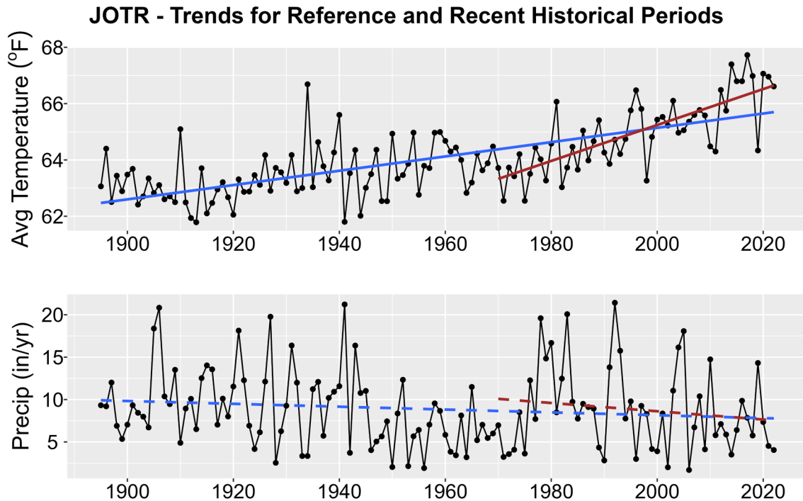
Figure 1. Historical trends in annual average temperature (upper plot) and annual total precipitation (lower plot) for JOTR from 1895-2022. Black points show yearly values while blue lines are linear regressions for the entire period record and red lines for 1970-2022 trends. Solid lines are significant trends (i.e., p < 0.05 ); dashed lines are not statistically significant.
