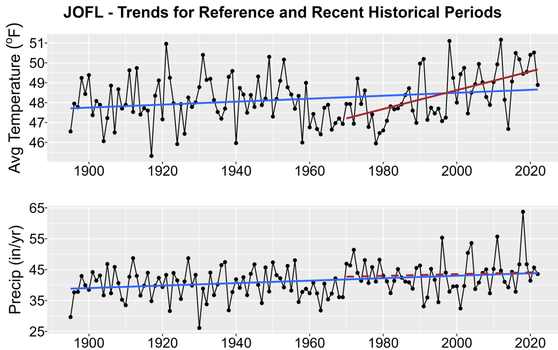
Figure 1. Historical trends in annual average temperature (upper plot) and annual total precipitation (lower plot) for JOFL from 1895-2022. Black points show yearly values while blue lines are linear regressions for the entire period record and red lines for 1970-2022 trends. Solid lines are significant trends (i.e., p < 0.05 ); dashed lines are not statistically significant.
