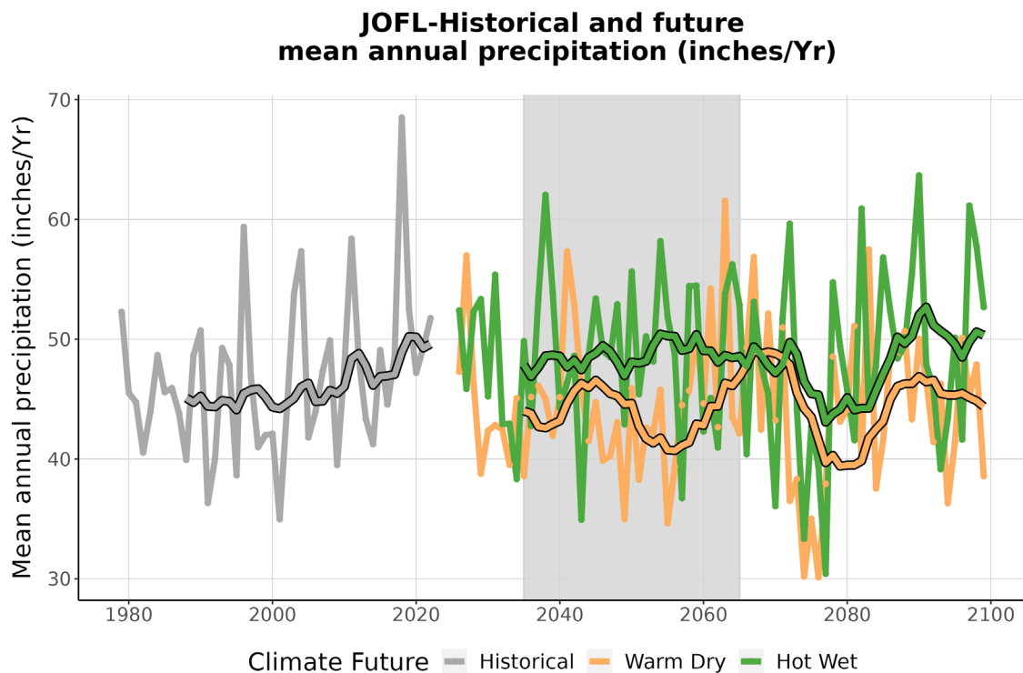
Figure 4. This graph compares observed average annual precipitation at JOFL (inches/year) (1979-2022) with projected average annual precipitation for the two climate futures over the period 2023-2099. The historically observed data is shown in gray, the Warm Dry climate future in orange, and the Hot Wet climate future in green. The smooth line running through each projection is the 10-year running average for historical observations and future projections. The gray-shaded area represents the time period that was averaged (2035-2065) to summarize future projections for the year 2050 (Appendix 1).
