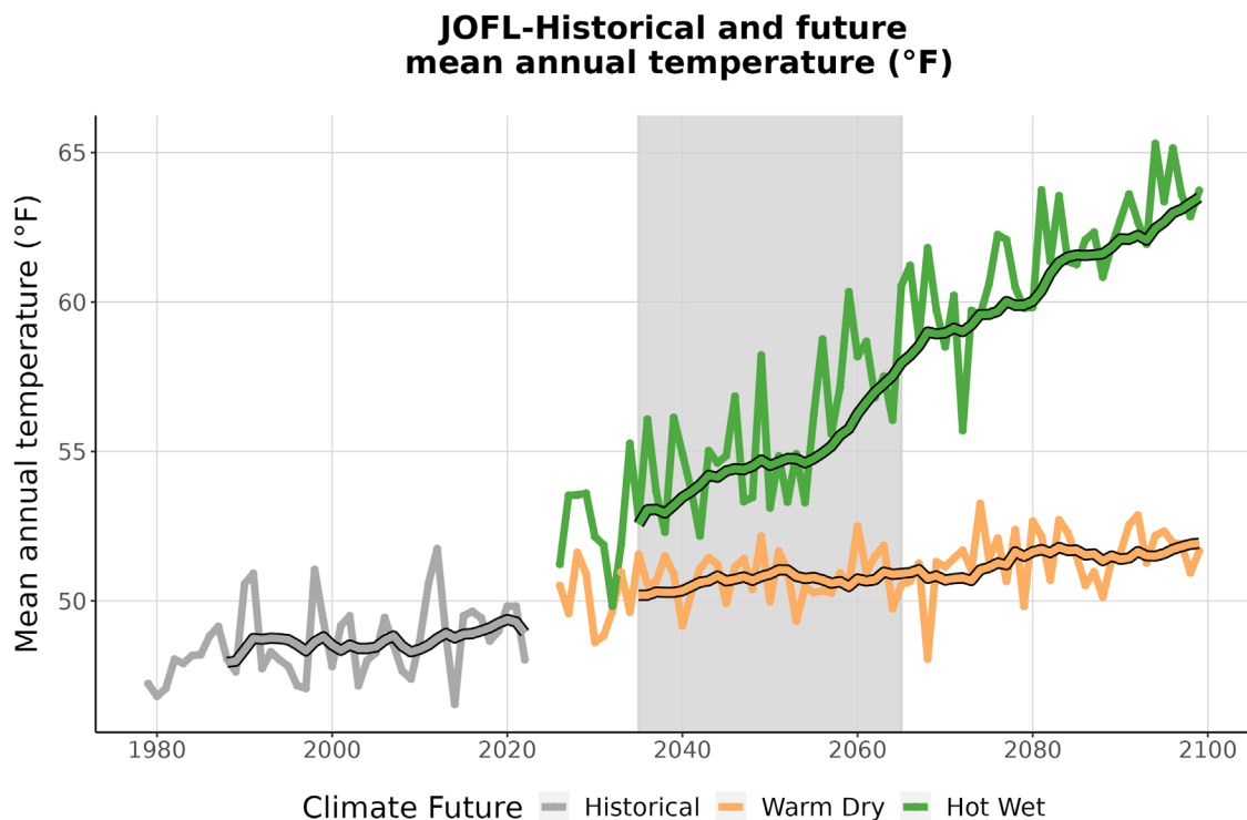
Figure 3. This graph compares observed average annual temperature at JOFL (°F) (1979-2022) with projected average annual temperature for the two climate futures over the period 2023-2099. The historically observed data
