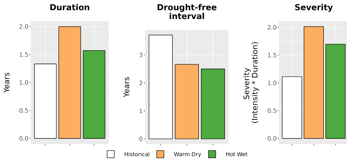
Figure 8. Drought metrics for JOFL. (Left) Average drought duration (years) historically (1979-2012) and under each climate future. (Middle) Average drought return interval (years), indicating the expected amount of time between periods of drought, historically and under each climate future. (Right) Average drought severity, a measure of drought intensity multiplied by duration, historically and under each climate future.
