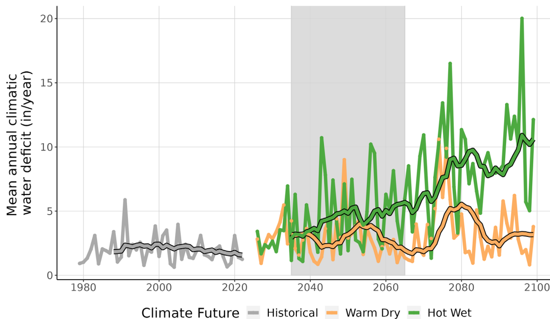
Figure 9. This line graph compares observed climatic water deficit at JOFL (inches/year) (1979-2022) with projected climatic water deficit for the two climate futures over the period 2023-2099. The historical observation data is shown in gray, the Warm Dry climate future in orange, and the Hot Wet climate future in green. The smooth line running through each projection is the 10-year running average for historical observations and future projections. Gray-shaded area represents the time period that was averaged (2035-2065) to summarize future projections for the year 2050.
