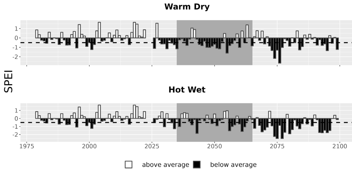
Figure 7. Drought metrics for JOFL. Drought index (SPEI; units = standard deviations from historical) timeseries for each climate future. Below-average SPEI (black bars) indicates dry conditions. The dotted line (SPEI = -0.5) indicates drought conditions.
