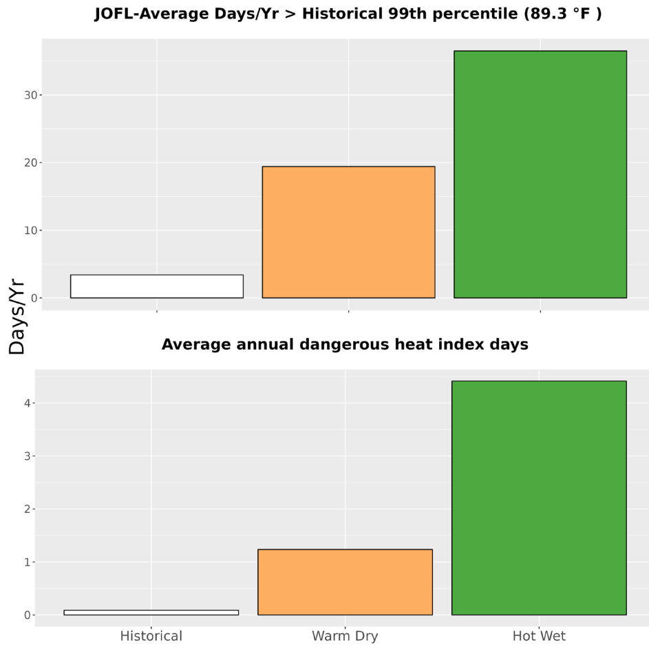
Figure 5. The upper bar graph represents the average number of days annually with temperatures greater than the historical 99th percentile (89.3 °F) historically (1979-2012) and for the two climate futures (2050). The bottom bar graph represents the average annual number of dangerous heat index days historically and for the two climate futures. Dangerous heat index days are days that exceed 105 °F.
