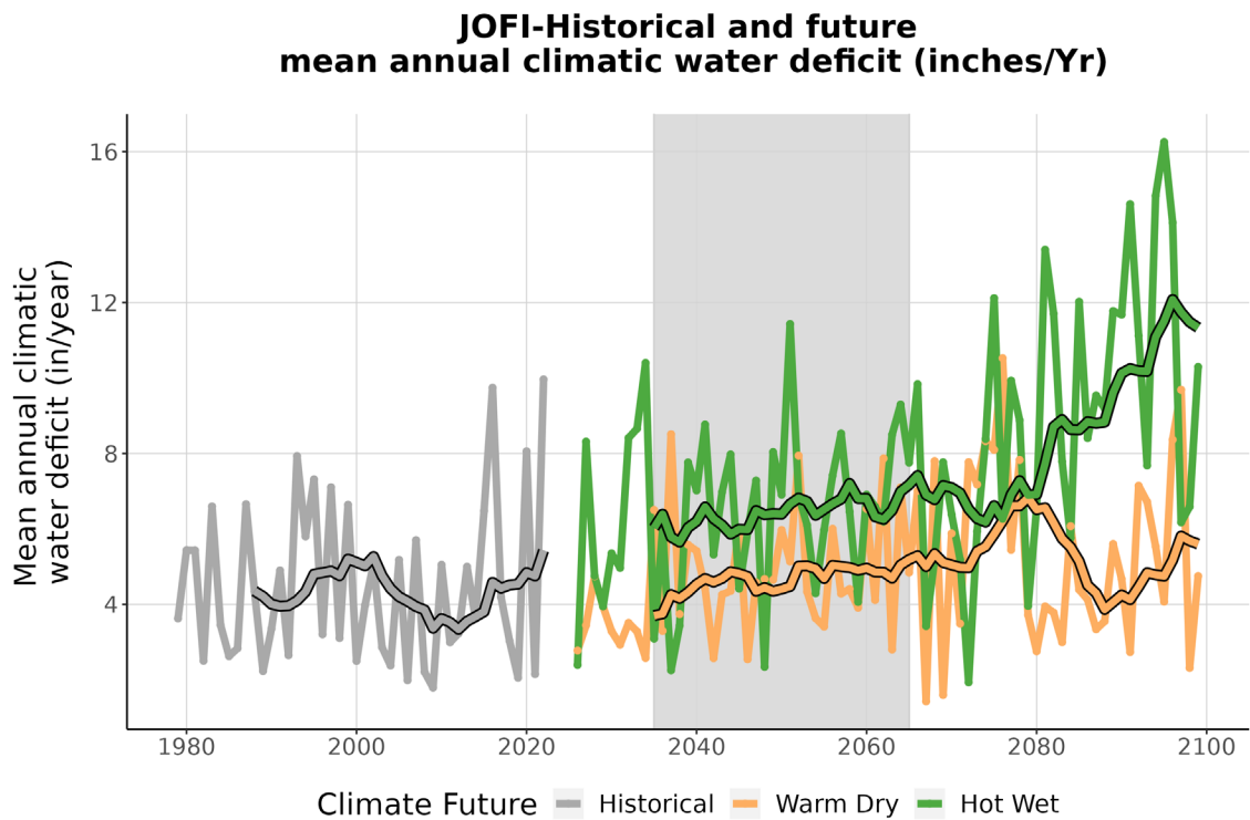
Figure 9. This line graph compares observed climatic water deficit at JOFI (inches/year) (1979-2022) with projected climatic water deficit for the two climate futures over the period 2023-2099. The historical observation data is shown in gray, the Warm Dry climate future in orange, and the Hot Wet climate future in green. The smooth line running through each projection is the 10-year running average for historical observations and future projections. Gray-shaded area represents the time period that was averaged (2035-2065) to summarize future projections for the year 2050.
