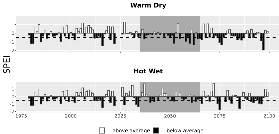
Figure 7. Drought metrics for JOFI. Drought index (SPEI; units = standard deviations from historical) timeseries for each climate future. Below-average SPEI (black bars) indicates dry conditions. The dotted line (SPEI = -0.5) indicates drought conditions.
