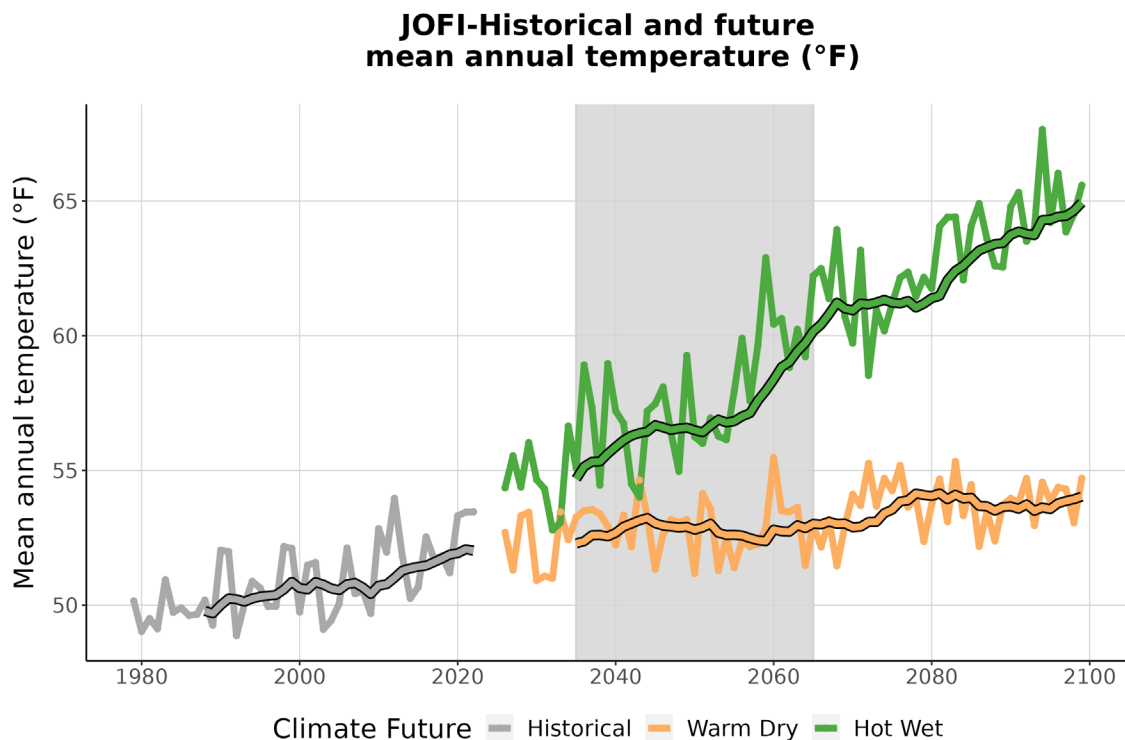
Figure 3. This graph compares observed average annual temperature at JOFI (°F) (1979-2022) with projected average annual temperature for the two climate futures over the period 2023-2099. The historically observed data
