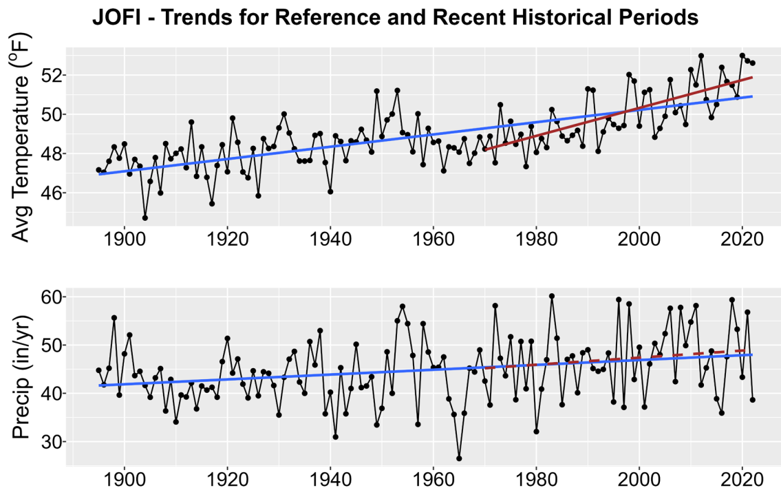
Figure 1. Historical trends in annual average temperature (upper plot) and annual total precipitation (lower plot) for JOFI from 1895-2022. Black points show yearly values while blue lines are linear regressions for the entire period record and red lines for 1970-2022 trends. Solid lines are significant trends (i.e., p < 0.05 ); dashed lines are not statistically significant.
