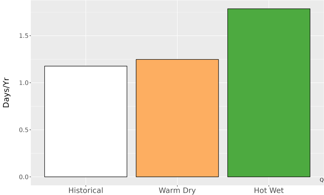
Figure 6. Average number of days annually with precipitation exceeding the 99th percentile (2.3 in.) of precipitation from the historical period 1979-2012 and for each climate future.
