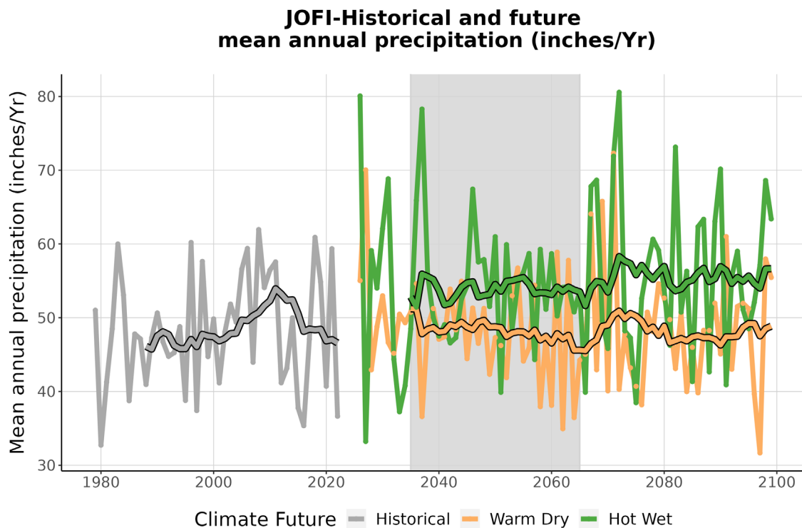
Figure 4. This graph compares observed average annual precipitation at JOFI (inches/year) (1979-2022) with projected average annual precipitation for the two climate futures over the period 2023-2099. The historically observed data is shown in gray, the Warm Dry climate future in orange, and the Hot Wet climate future in green. The smooth line running through each projection is the 10-year running average for historical observations and future projections. The gray-shaded area represents the time period that was averaged (2035-2065) to summarize future projections for the year 2050 (Appendix 1).
