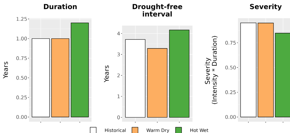
Figure 8. Drought metrics for JOFI. (Left) Average drought duration (years) historically (1979-2012) and under each climate future. (Middle) Average drought return interval (years), indicating the expected amount of time between periods of drought, historically and under each climate future. (Right) Average drought severity, a measure of drought intensity multiplied by duration, historically and under each climate future.
