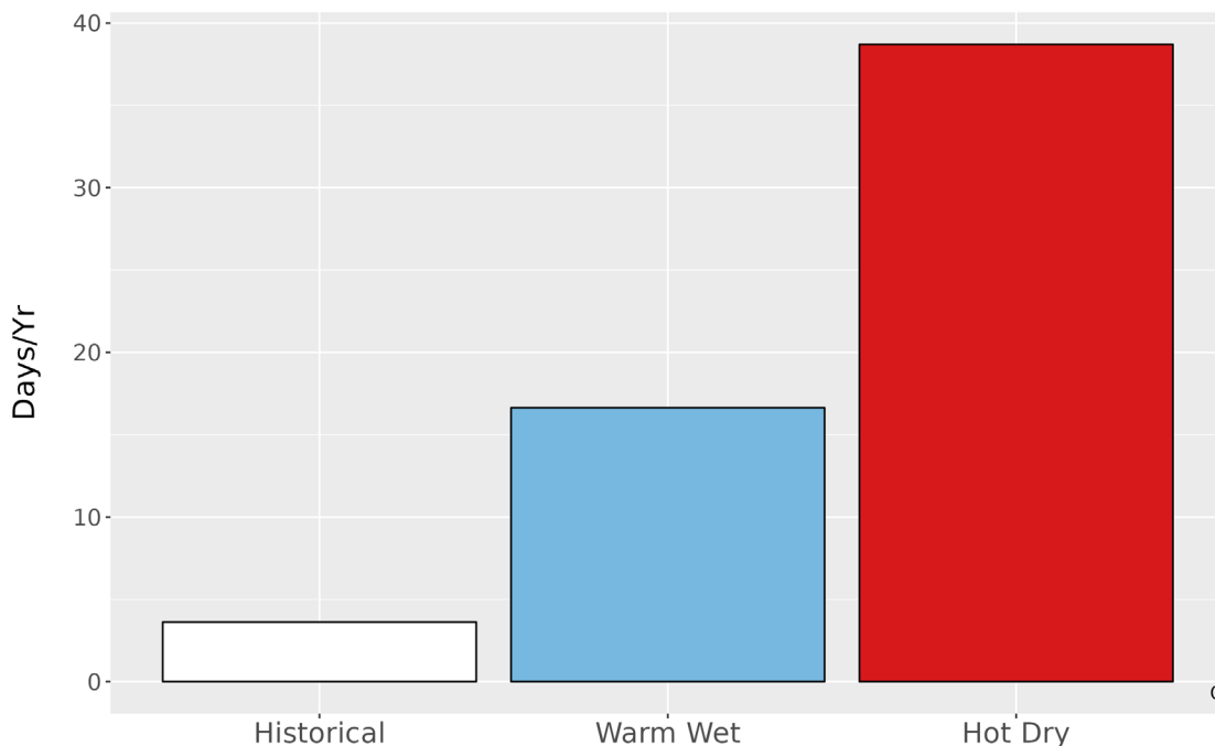
Figure 5. Metrics of extreme temperature at JODR. The bar graph represents the average number of days annually with temperatures greater than the historical 99th percentile (83.6 °F) historically (1979-2012) and for the two climate futures (2050).
