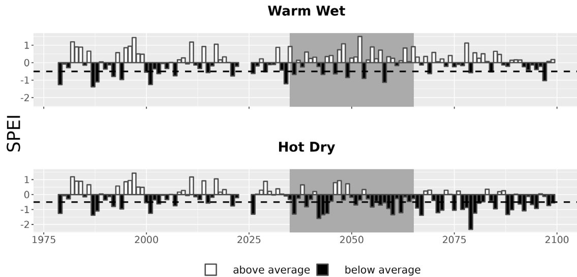
Figure 7. Drought metrics for JODR. Drought index (SPEI; units = standard deviations from historical) timeseries for each climate future. Below-average SPEI (black bars) indicates dry conditions. The dotted line (SPEI = -0.5) indicates drought conditions.
