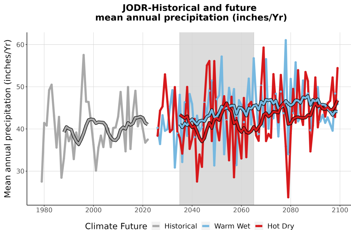
Figure 4. This graph compares observed average annual precipitation at JODR (inches/year) (1979-2022) with projected average annual precipitation for the two climate futures over the period 2023-2099. The historically observed data is shown in gray, the Warm Wet climate future in blue, and the Hot Dry climate future in red. The smooth line running through each projection is the 10-year running average for historical observations and future projections. The gray-shaded area represents the time period that was averaged (2035-2065) to summarize future projections for the year 2050 (Appendix 1).
