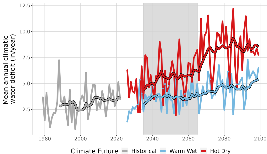
Figure 9. This line graph compares observed climatic water deficit at JODR (inches/year) (1979-2022) with projected climatic water deficit for the two climate futures over the period 2023-2099. The historical observation data is shown in gray, the Warm Wet climate future in blue, and the Hot Dry climate future in red. The smooth line running through each projection is the 10-year running average for historical observations and future projections. Gray-shaded area represents the time period that was averaged (2035-2065) to summarize future projections for the year 2050.
