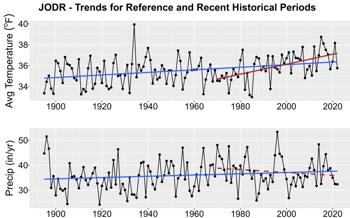
Figure 1. Historical trends in annual average temperature (upper plot) and annual total precipitation (lower plot) for JODR from 1895-2022. Black points show yearly values while blue lines are linear regressions for the entire period record and red lines for 1970-2022 trends. Solid lines are significant trends (i.e., p < 0.05 ); dashed lines are not statistically significant.
