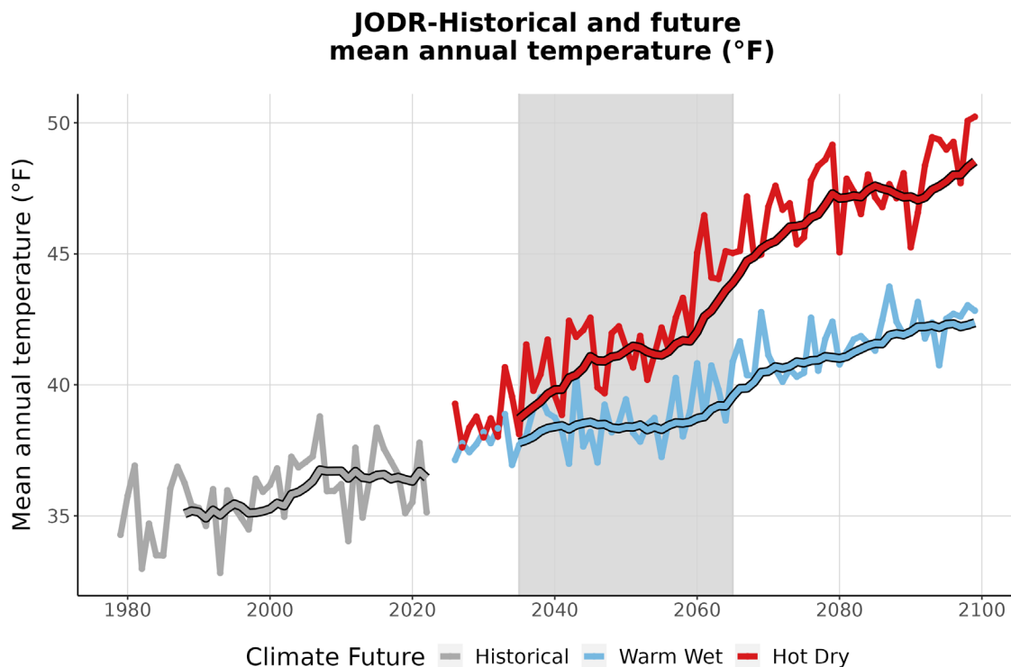
Figure 3. This graph compares observed average annual temperature at JODR (°F) (1979-2022) with projected average annual temperature for the two climate futures over the period 2023-2099. The historically observed data
