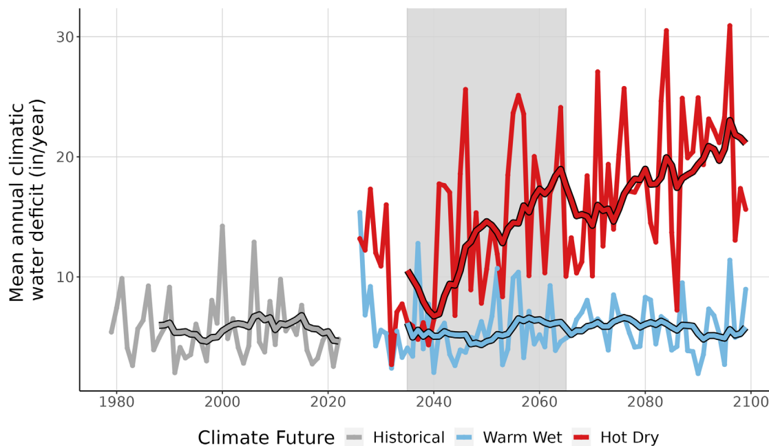
Figure 9. This line graph compares observed climatic water deficit at JELA (inches/year) (1979-2022) with projected climatic water deficit for the two climate futures over the period 2023-2099. The historical observation data is shown in gray, the Warm Wet climate future in blue, and the Hot Dry climate future in red. The smooth line running through each projection is the 10-year running average for historical observations and future projections. Gray-shaded area represents the time period that was averaged (2035-2065) to summarize future projections for the year 2050.
