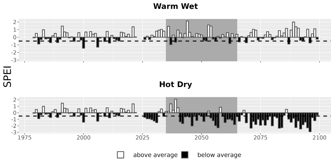
Figure 7. Drought metrics for JELA. Drought index (SPEI; units = standard deviations from historical) timeseries for each climate future. Below-average SPEI (black bars) indicates dry conditions. The dotted line (SPEI = -0.5) indicates drought conditions.
