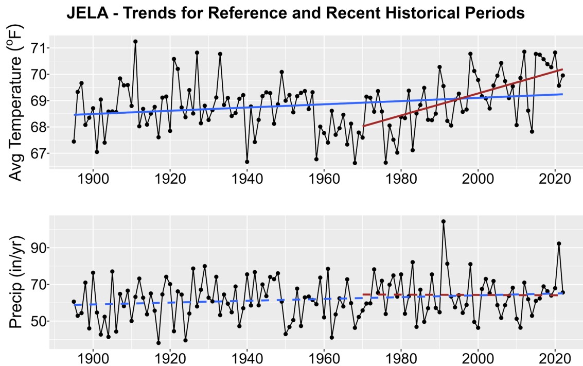
Figure 1. Historical trends in annual average temperature (upper plot) and annual total precipitation (lower plot) for JELA from 1895-2022. Black points show yearly values while blue lines are linear regressions for the entire period record and red lines for 1970-2022 trends. Solid lines are significant trends (i.e., p < 0.05 ); dashed lines are not statistically significant.
