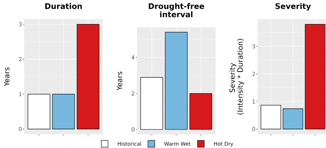
Figure 8. Drought metrics for JELA. (Left) Average drought duration (years) historically (1979-2012) and under each climate future. (Middle) Average drought return interval (years), indicating the expected amount of time between periods of drought, historically and under each climate future. (Right) Average drought severity, a measure of drought intensity multiplied by duration, historically and under each climate future.
