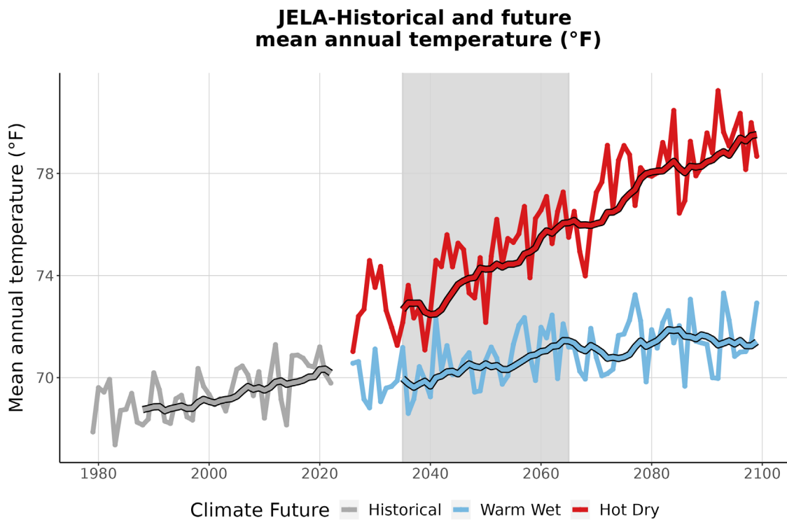
Figure 3. This graph compares observed average annual temperature at JELA (°F) (1979-2022) with projected average annual temperature for the two climate futures over the period 2023-2099. The historically observed data
