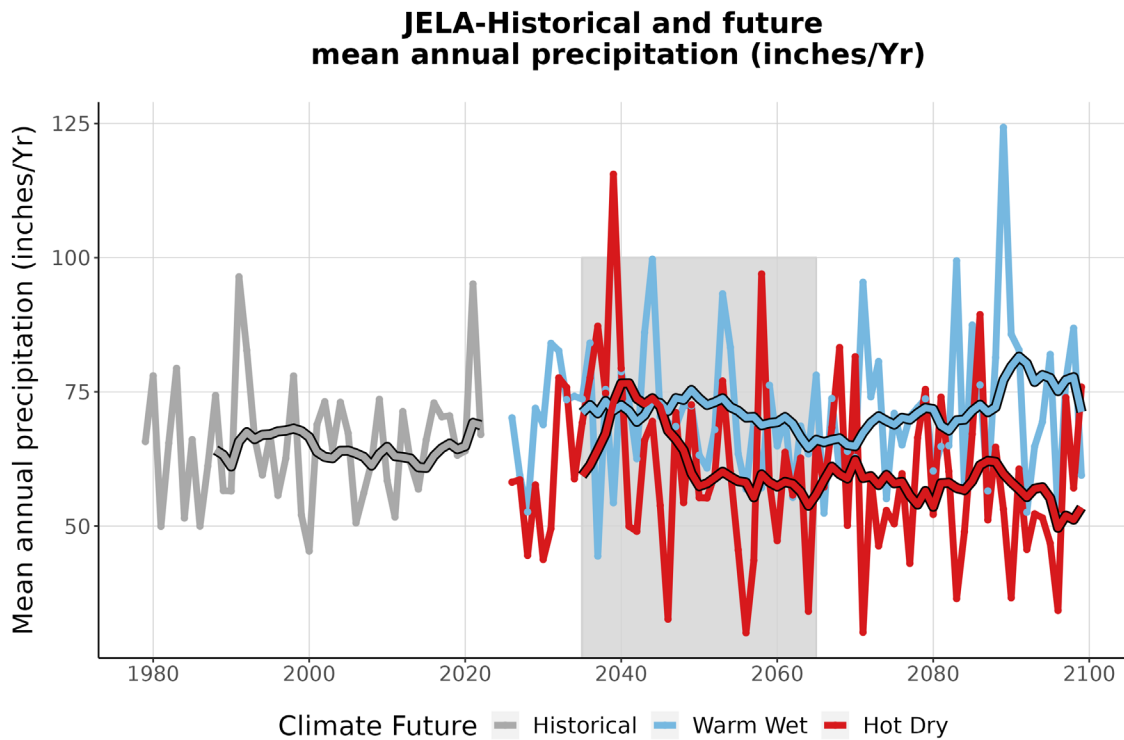
Figure 4. This graph compares observed average annual precipitation at JELA (inches/year) (1979-2022) with projected average annual precipitation for the two climate futures over the period 2023-2099. The historically observed data is shown in gray, the Warm Wet climate future in blue, and the Hot Dry climate future in red. The smooth line running through each projection is the 10-year running average for historical observations and future projections. The gray-shaded area represents the time period that was averaged (2035-2065) to summarize future projections for the year 2050 (Appendix 1).
