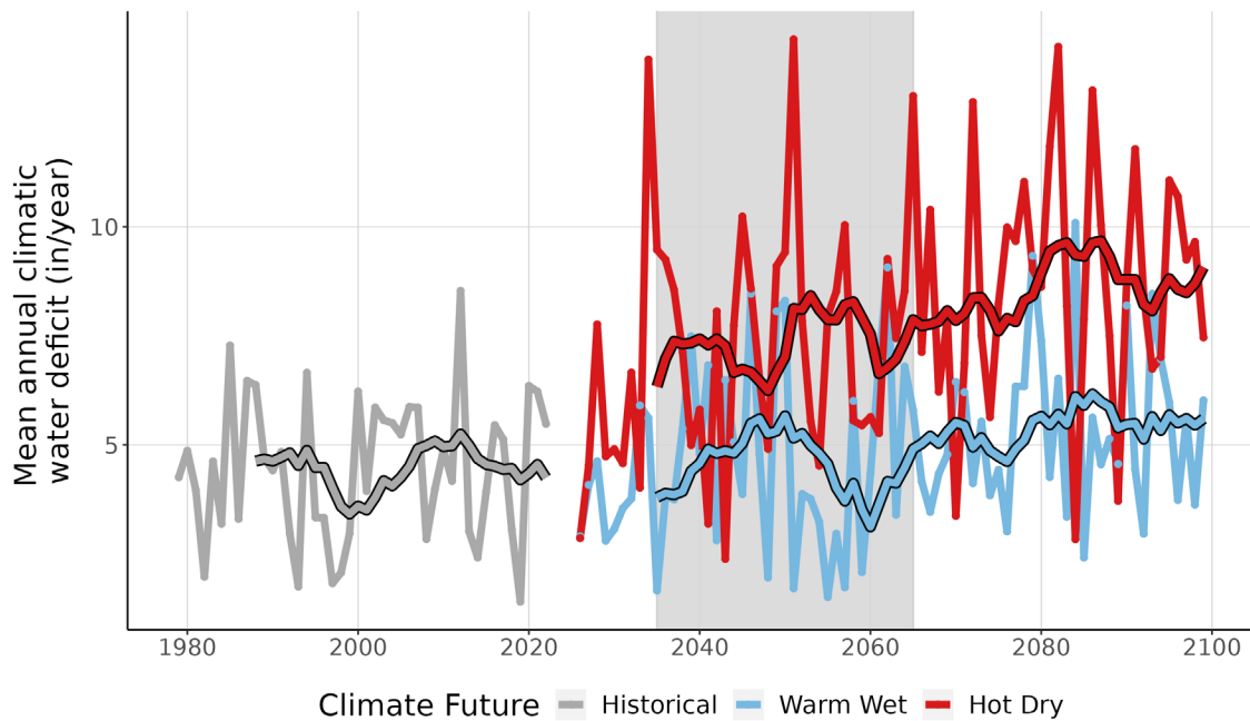
Figure 9. This line graph compares observed climatic water deficit at JECA (inches/year) (1979-2022) with projected climatic water deficit for the two climate futures over the period 2023-2099. The historical observation data is shown in gray, the Warm Wet climate future in blue, and the Hot Dry climate future in red. The smooth line running through each projection is the 10-year running average for historical observations and future projections. Gray-shaded area represents the time period that was averaged (2035-2065) to summarize future projections for the year 2050.
