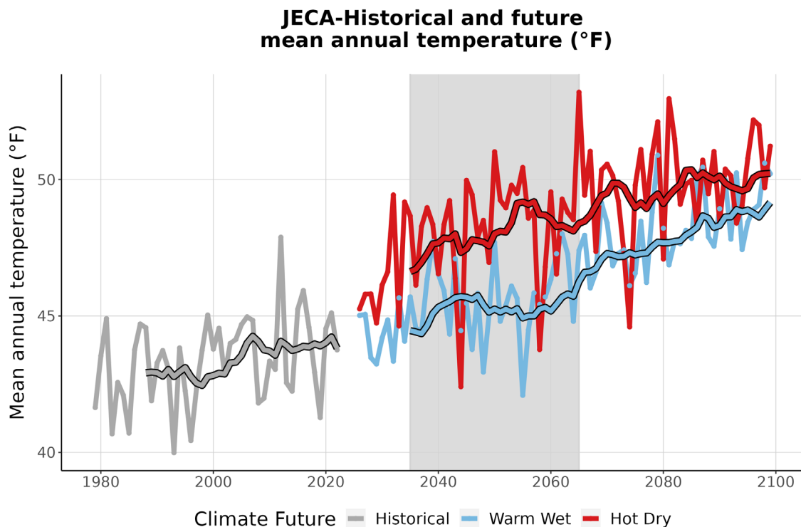
Figure 3. This graph compares observed average annual temperature at JECA (°F) (1979-2022) with projected average annual temperature for the two climate futures over the period 2023-2099. The historically observed data
