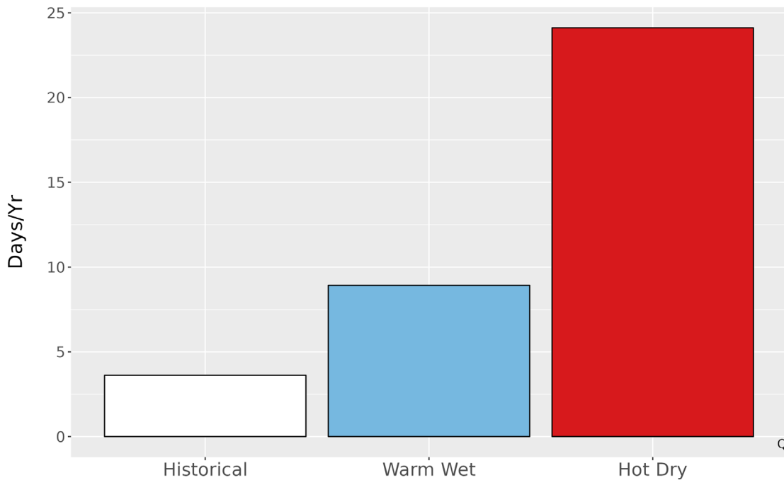
Figure 5. Metrics of extreme temperature at JECA. The bar graph represents the average number of days annually with temperatures greater than the historical 99th percentile (90.6 °F) historically (1979-2012) and for the two climate futures (2050).
