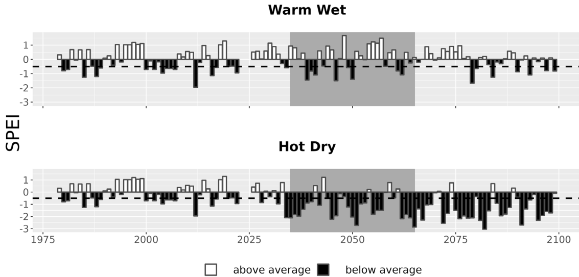
Figure 7. Drought metrics for JECA. Drought index (SPEI; units = standard deviations from historical) timeseries for each climate future. Below-average SPEI (black bars) indicates dry conditions. The dotted line (SPEI = -0.5) indicates drought conditions.
