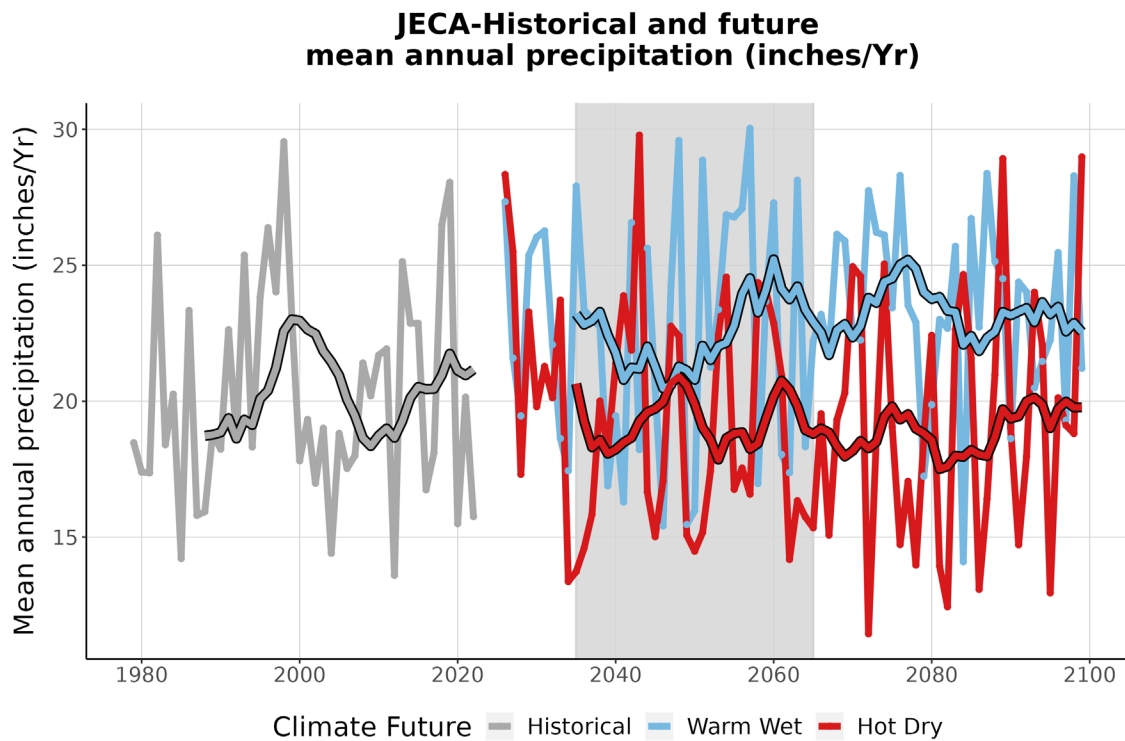
Figure 4. This graph compares observed average annual precipitation at JECA (inches/year) (1979-2022) with projected average annual precipitation for the two climate futures over the period 2023-2099. The historically observed data is shown in gray, the Warm Wet climate future in blue, and the Hot Dry climate future in red. The smooth line running through each projection is the 10-year running average for historical observations and future projections. The gray-shaded area represents the time period that was averaged (2035-2065) to summarize future projections for the year 2050 (Appendix 1).
