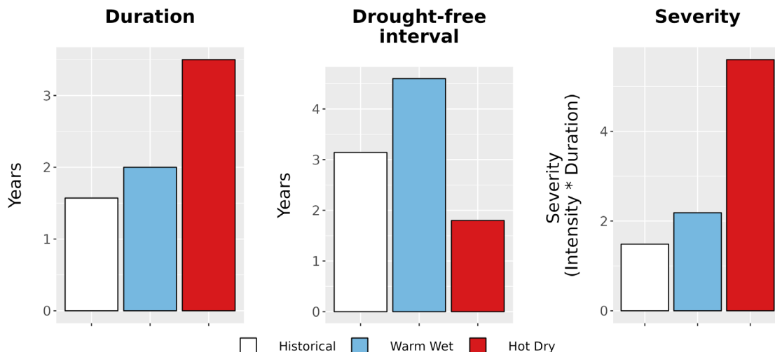
Figure 8. Drought metrics for JECA. (Left) Average drought duration (years) historically (1979-2012) and under each climate future. (Middle) Average drought return interval (years), indicating the expected amount of time between periods of drought, historically and under each climate future. (Right) Average drought severity, a measure of drought intensity multiplied by duration, historically and under each climate future.
