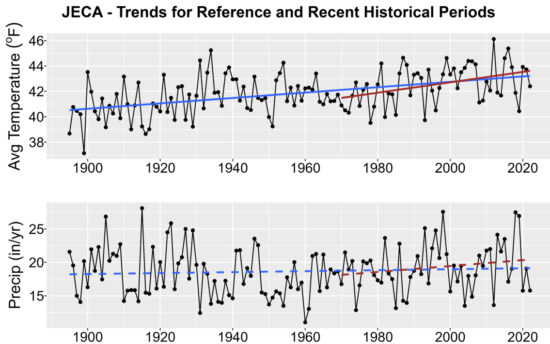
Figure 1. Historical trends in annual average temperature (upper plot) and annual total precipitation (lower plot) for JECA from 1895-2022. Black points show yearly values while blue lines are linear regressions for the entire period record and red lines for 1970-2022 trends. Solid lines are significant trends (i.e., p < 0.05 ); dashed lines are not statistically significant.
