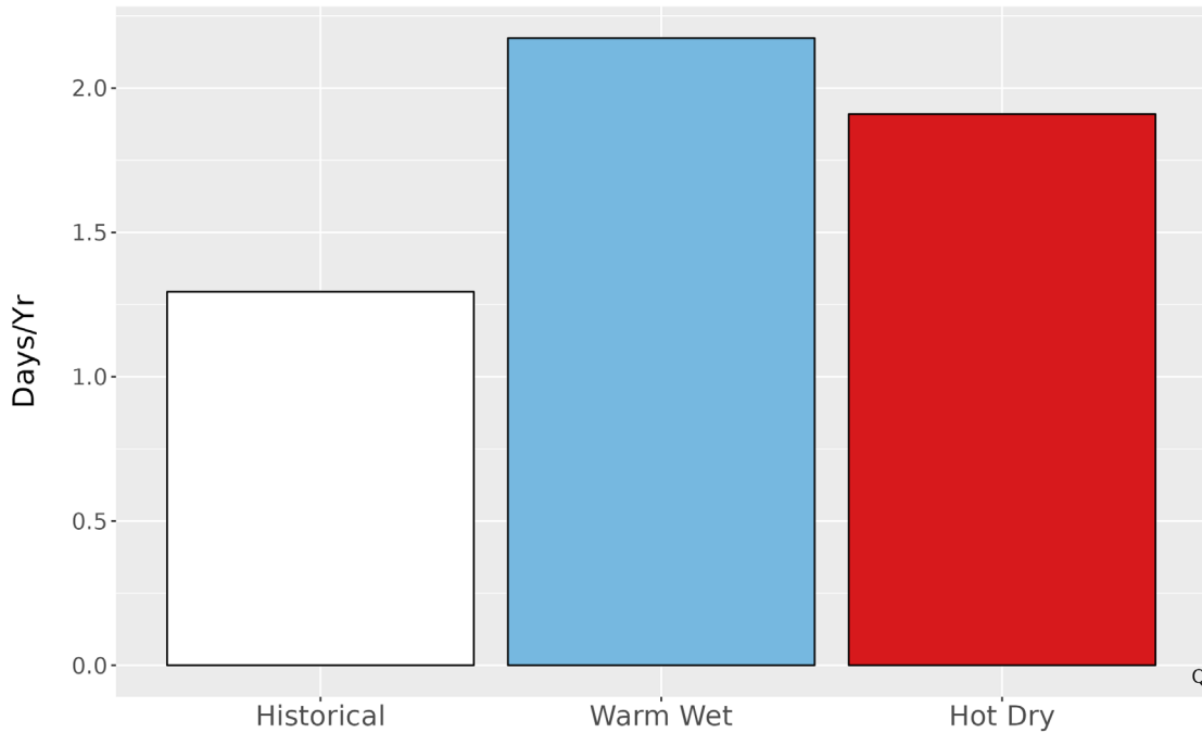
Figure 6. Average number of days annually with precipitation exceeding the 99th percentile (1 in.) of precipitation from the historical period 1979-2012 and for each climate future.
