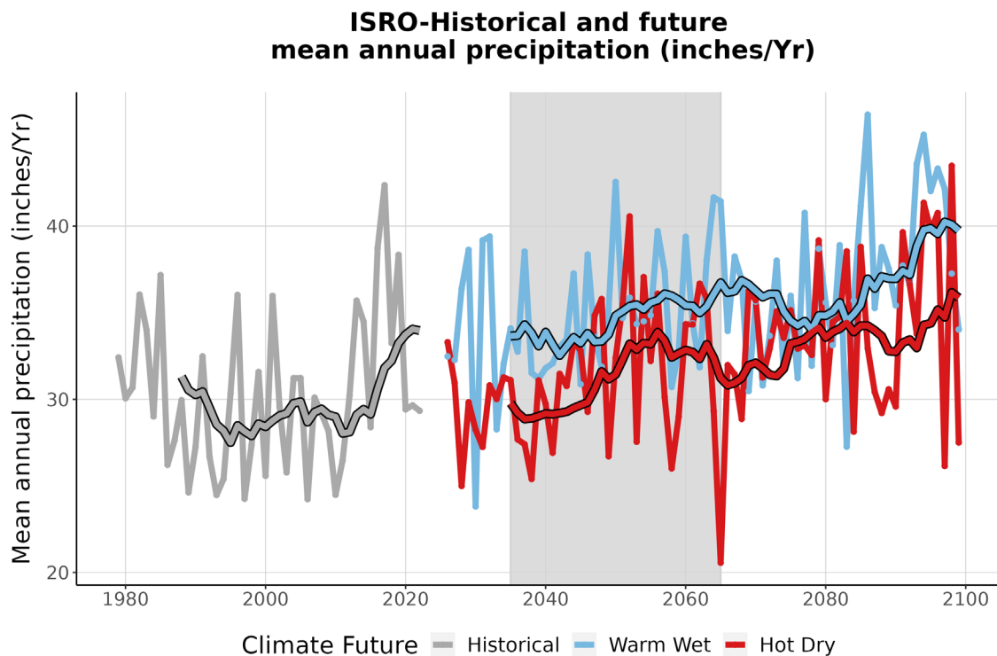
Figure 4. This graph compares observed average annual precipitation at ISRO (inches/year) (1979-2022) with projected average annual precipitation for the two climate futures over the period 2023-2099. The historically observed data is shown in gray, the Warm Wet climate future in blue, and the Hot Dry climate future in red. The smooth line running through each projection is the 10-year running average for historical observations and future projections. The gray-shaded area represents the time period that was averaged (2035-2065) to summarize future projections for the year 2050 (Appendix 1).
