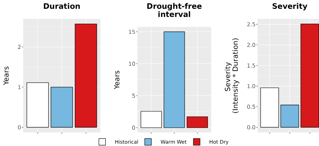
Figure 8. Drought metrics for ISRO. (Left) Average drought duration (years) historically (1979-2012) and under each climate future. (Middle) Average drought return interval (years), indicating the expected amount of time between periods of drought, historically and under each climate future. (Right) Average drought severity, a measure of drought intensity multiplied by duration, historically and under each climate future.
