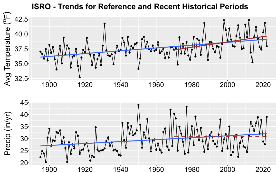
Figure 1. Historical trends in annual average temperature (upper plot) and annual total precipitation (lower plot) for ISRO from 1895-2022. Black points show yearly values while blue lines are linear regressions for the entire period record and red lines for 1970-2022 trends. Solid lines are significant trends (i.e., p < 0.05 ); dashed lines are not statistically significant.
