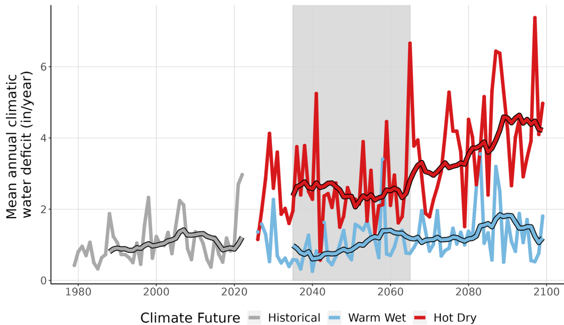
Figure 9. This line graph compares observed climatic water deficit at ISRO (inches/year) (1979-2022) with projected climatic water deficit for the two climate futures over the period 2023-2099. The historical observation data is shown in gray, the Warm Wet climate future in blue, and the Hot Dry climate future in red. The smooth line running through each projection is the 10-year running average for historical observations and future projections. Gray-shaded area represents the time period that was averaged (2035-2065) to summarize future projections for the year 2050.
