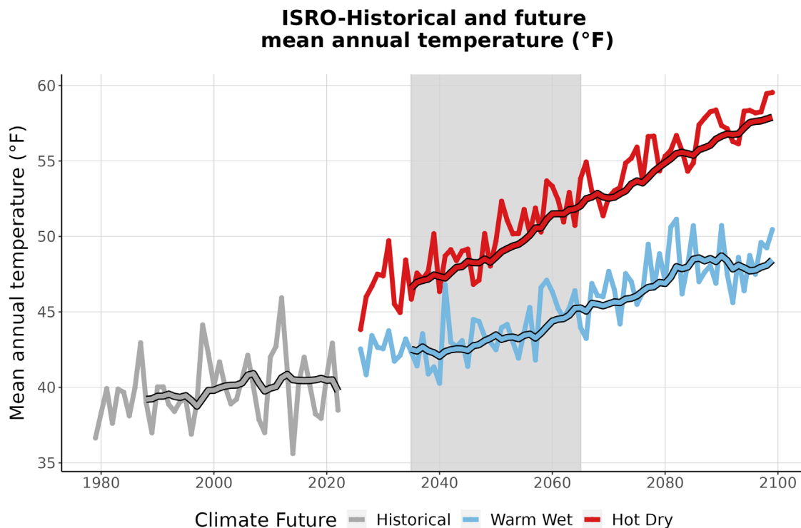
Figure 3. This graph compares observed average annual temperature at ISRO (°F) (1979-2022) with projected average annual temperature for the two climate futures over the period 2023-2099. The historically observed data
