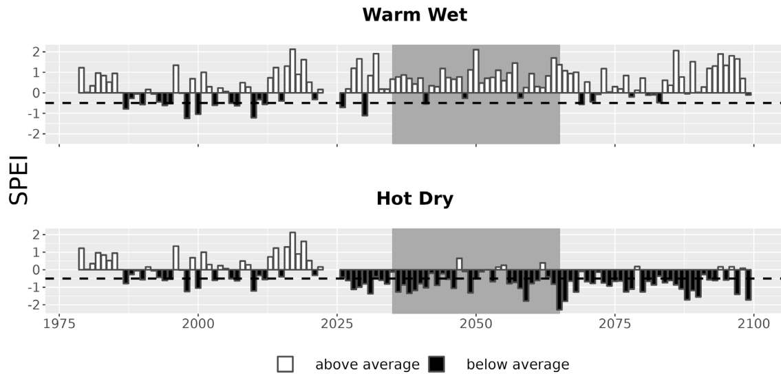
Figure 7. Drought metrics for ISRO. Drought index (SPEI; units = standard deviations from historical) timeseries for each climate future. Below-average SPEI (black bars) indicates dry conditions. The dotted line (SPEI = -0.5) indicates drought conditions.
