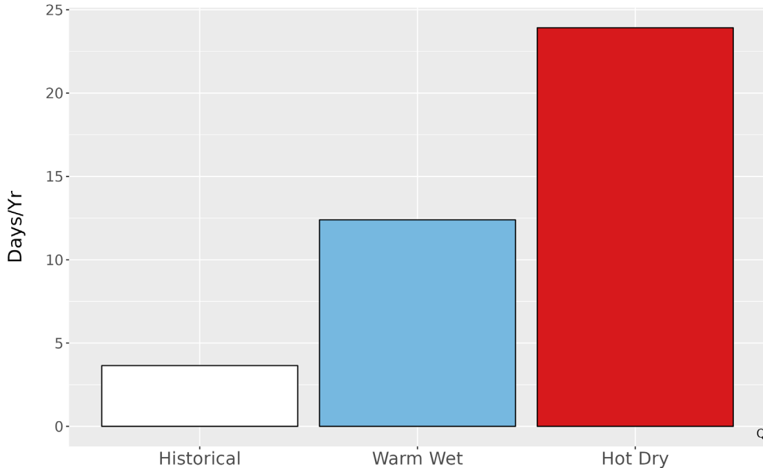
Figure 5. Metrics of extreme temperature at ISRO. The bar graph represents the average number of days annually with temperatures greater than the historical 99th percentile (84.3 °F) historically (1979-2012) and for the two climate futures (2050).
