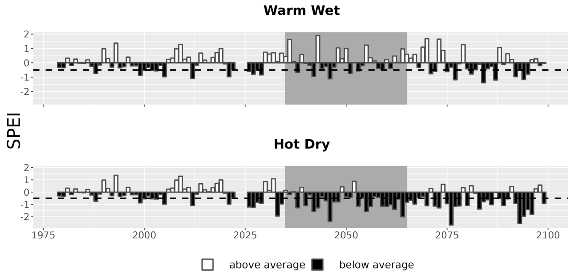
Figure 7. Drought metrics for INDU. Drought index (SPEI; units = standard deviations from historical) timeseries for each climate future. Below-average SPEI (black bars) indicates dry conditions. The dotted line (SPEI = -0.5) indicates drought conditions.
