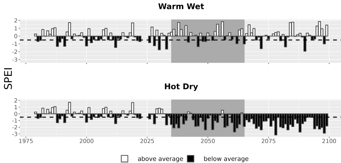
Figure 7. Drought metrics for HOME. Drought index (SPEI; units = standard deviations from historical) timeseries for each climate future. Below-average SPEI (black bars) indicates dry conditions. The dotted line (SPEI = -0.5) indicates drought conditions.
