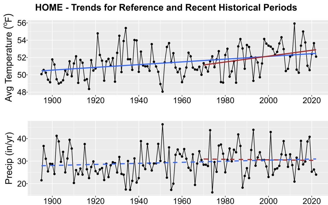
Figure 1. Historical trends in annual average temperature (upper plot) and annual total precipitation (lower plot) for HOME from 1895-2022. Black points show yearly values while blue lines are linear regressions for the entire period record and red lines for 1970-2022 trends. Solid lines are significant trends (i.e., p < 0.05 ); dashed lines are not statistically significant.
