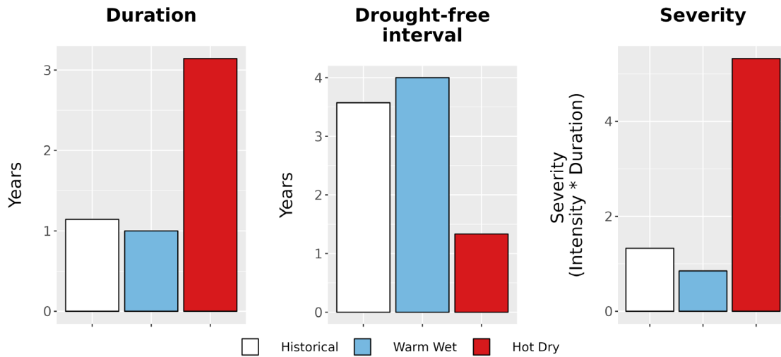
Figure 8. Drought metrics for HOME. (Left) Average drought duration (years) historically (1979-2012) and under each climate future. (Middle) Average drought return interval (years), indicating the expected amount of time between periods of drought, historically and under each climate future. (Right) Average drought severity, a measure of drought intensity multiplied by duration, historically and under each climate future.
