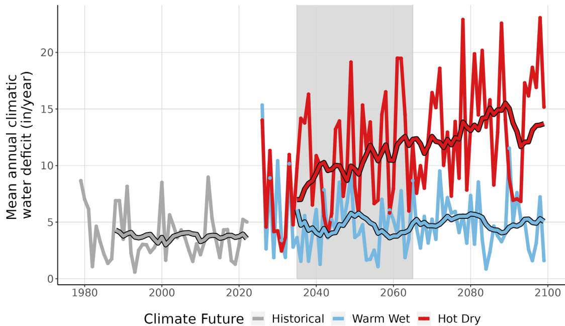
Figure 9. This line graph compares observed climatic water deficit at HOME (inches/year) (1979-2022) with projected climatic water deficit for the two climate futures over the period 2023-2099. The historical observation data is shown in gray, the Warm Wet climate future in blue, and the Hot Dry climate future in red. The smooth line running through each projection is the 10-year running average for historical observations and future projections. Gray-shaded area represents the time period that was averaged (2035-2065) to summarize future projections for the year 2050.
