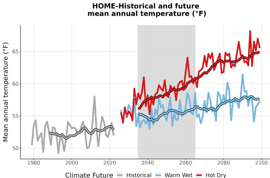
Figure 3. This graph compares observed average annual temperature at HOME (°F) (1979-2022) with projected average annual temperature for the two climate futures over the period 2023-2099. The historically observed data
