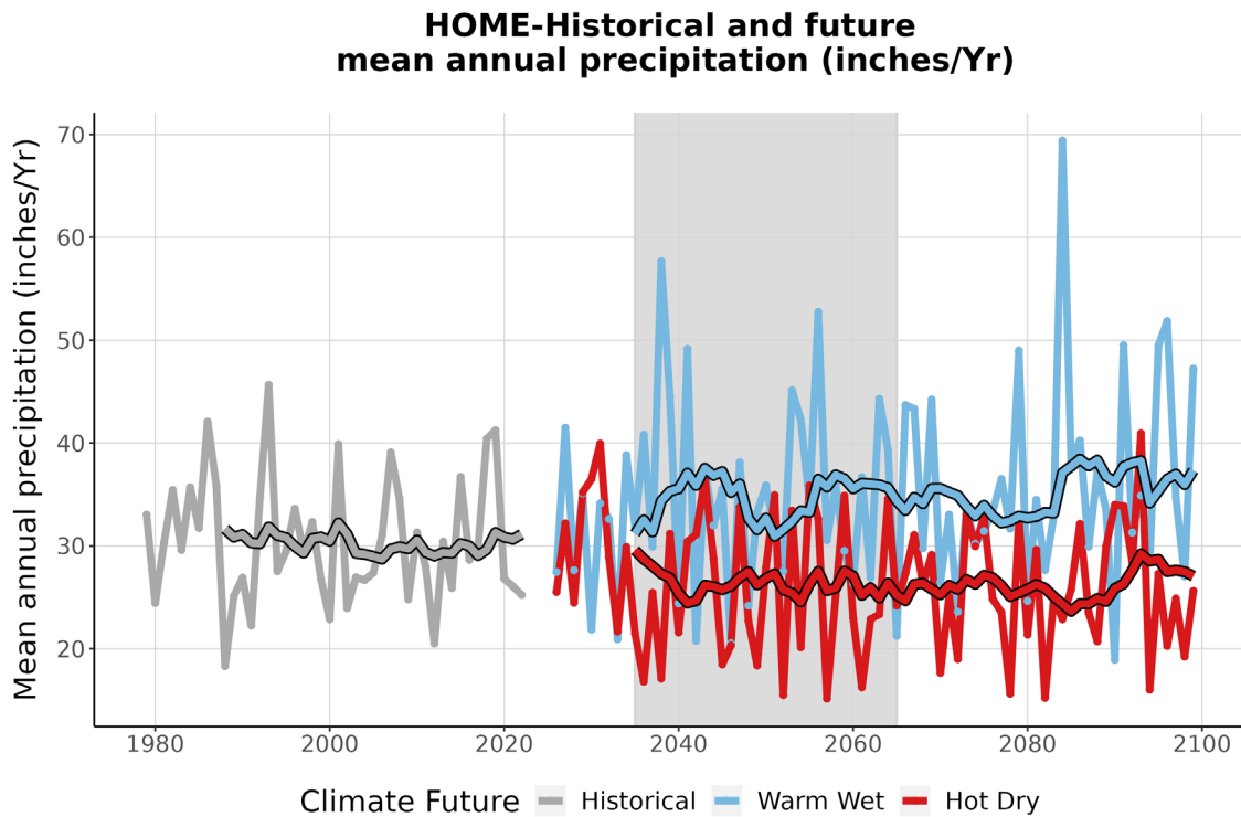
Figure 4. This graph compares observed average annual precipitation at HOME (inches/year) (1979-2022) with projected average annual precipitation for the two climate futures over the period 2023-2099. The historically observed data is shown in gray, the Warm Wet climate future in blue, and the Hot Dry climate future in red. The smooth line running through each projection is the 10-year running average for historical observations and future projections. The gray-shaded area represents the time period that was averaged (2035-2065) to summarize future projections for the year 2050 (Appendix 1).
