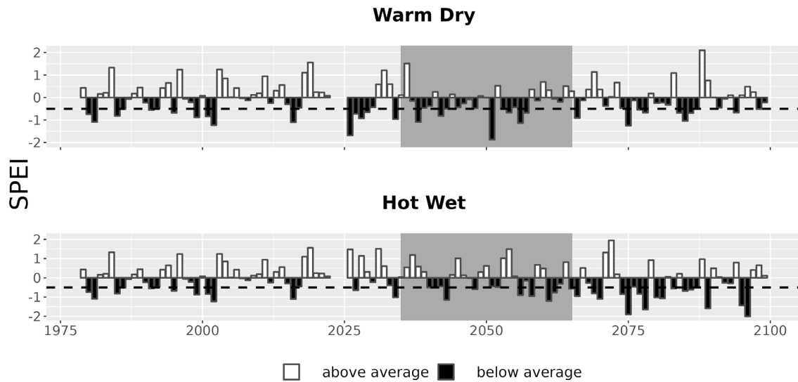
Figure 7. Drought metrics for HOFU. Drought index (SPEI; units = standard deviations from historical) timeseries for each climate future. Below-average SPEI (black bars) indicates dry conditions. The dotted line (SPEI = -0.5) indicates drought conditions.
