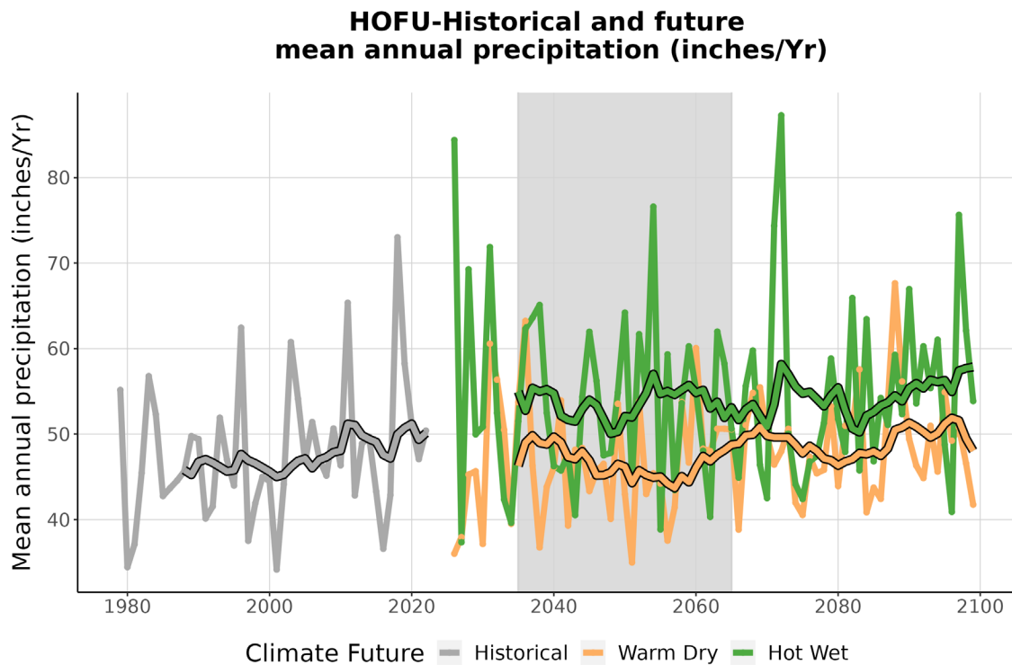
Figure 4. This graph compares observed average annual precipitation at HOFU (inches/year) (1979-2022) with projected average annual precipitation for the two climate futures over the period 2023-2099. The historically observed data is shown in gray, the Warm Dry climate future in orange, and the Hot Wet climate future in green. The smooth line running through each projection is the 10-year running average for historical observations and future projections. The gray-shaded area represents the time period that was averaged (2035-2065) to summarize future projections for the year 2050 (Appendix 1).
