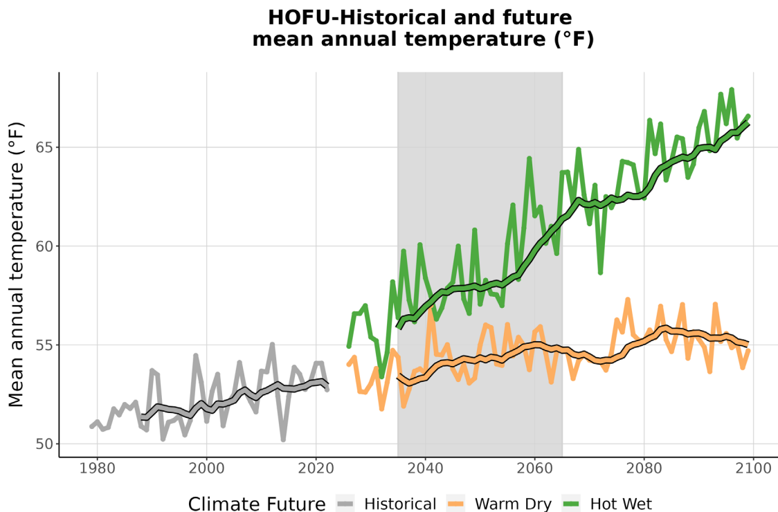
Figure 3. This graph compares observed average annual temperature at HOFU (°F) (1979-2022) with projected average annual temperature for the two climate futures over the period 2023-2099. The historically observed data
