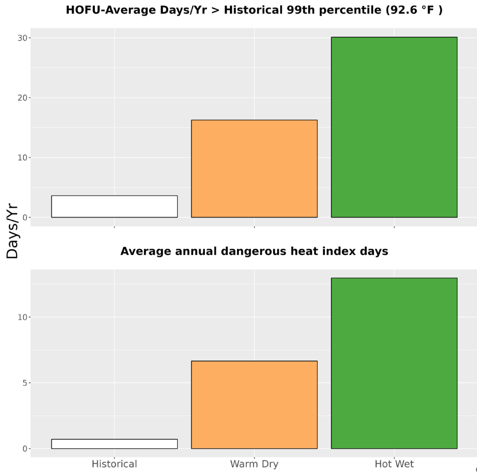
Figure 5. The upper bar graph represents the average number of days annually with temperatures greater than the historical 99th percentile (92.6 °F) historically (1979-2012) and for the two climate futures (2050). The bottom bar graph represents the average annual number of dangerous heat index days historically and for the two climate futures. Dangerous heat index days are days that exceed 105 °F.
