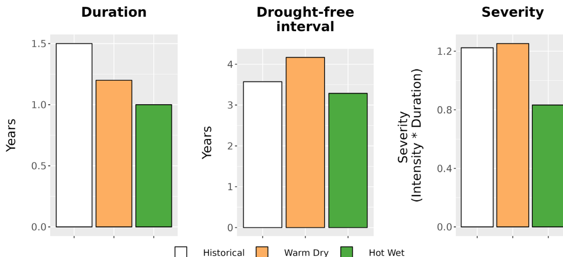
Figure 8. Drought metrics for HOFU. (Left) Average drought duration (years) historically (1979-2012) and under each climate future. (Middle) Average drought return interval (years), indicating the expected amount of time between periods of drought, historically and under each climate future. (Right) Average drought severity, a measure of drought intensity multiplied by duration, historically and under each climate future.
