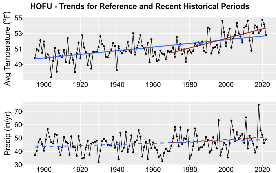
Figure 1. Historical trends in annual average temperature (upper plot) and annual total precipitation (lower plot) for HOFU from 1895-2022. Black points show yearly values while blue lines are linear regressions for the entire period record and red lines for 1970-2022 trends. Solid lines are significant trends (i.e., p < 0.05 ); dashed lines are not statistically significant.
