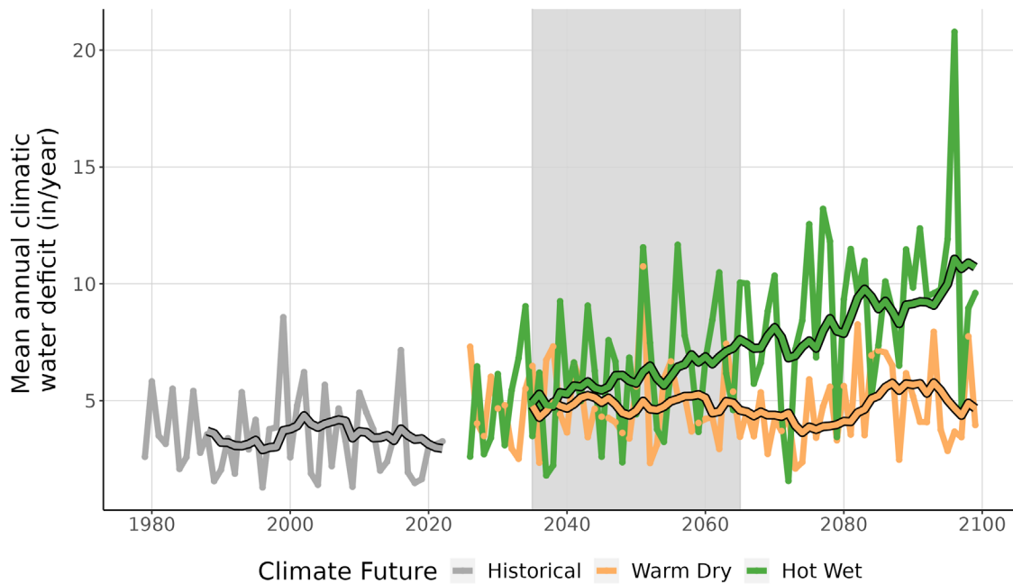
Figure 9. This line graph compares observed climatic water deficit at HOFU (inches/year) (1979-2022) with projected climatic water deficit for the two climate futures over the period 2023-2099. The historical observation data is shown in gray, the Warm Dry climate future in orange, and the Hot Wet climate future in green. The smooth line running through each projection is the 10-year running average for historical observations and future projections. Gray-shaded area represents the time period that was averaged (2035-2065) to summarize future projections for the year 2050.
