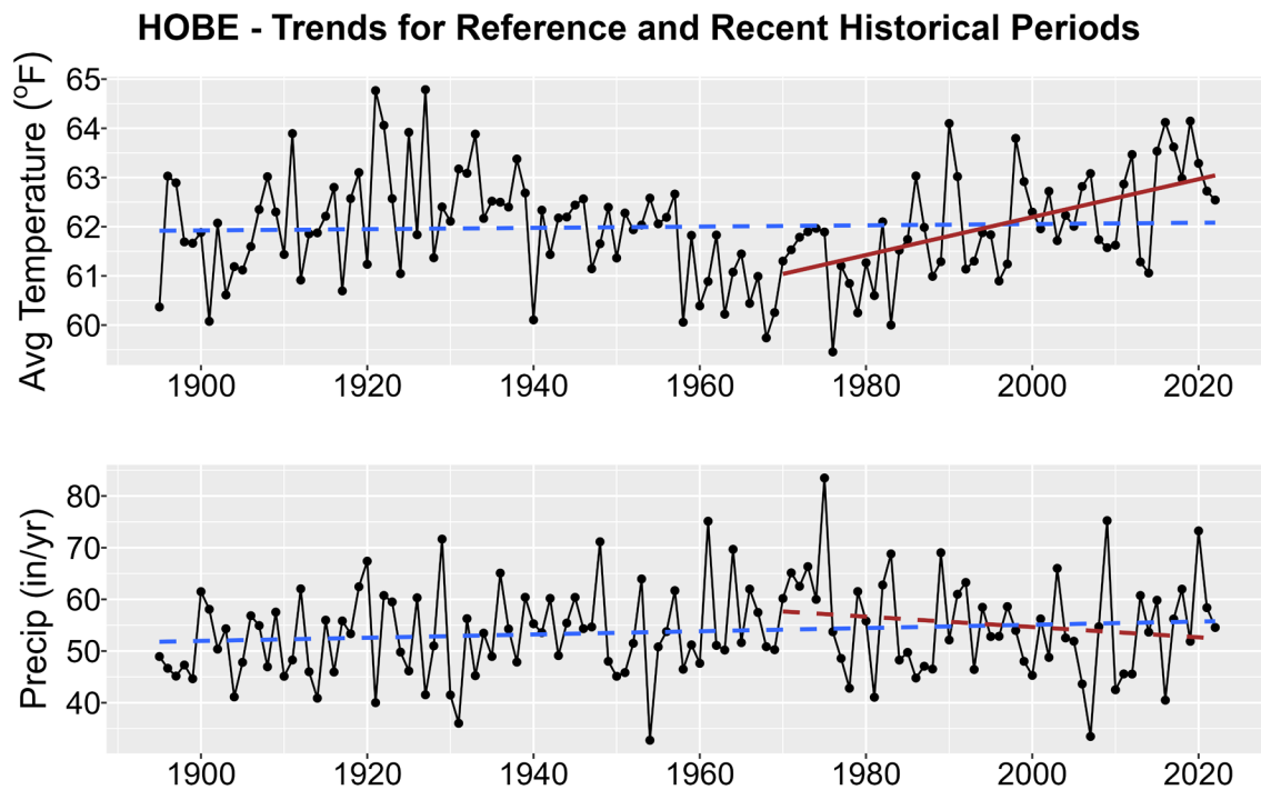
Figure 1. Historical trends in annual average temperature (upper plot) and annual total precipitation (lower plot) for HOBE from 1895-2022. Black points show yearly values while blue lines are linear regressions for the entire period record and red lines for 1970-2022 trends. Solid lines are significant trends (i.e., p < 0.05 ); dashed lines are not statistically significant.
