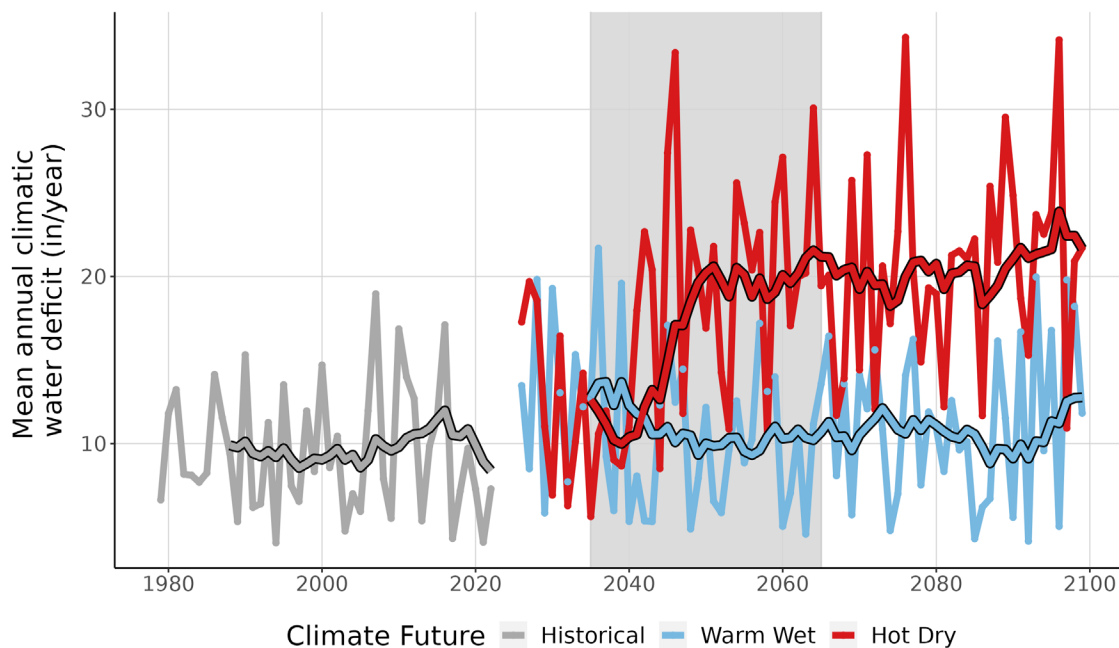
Figure 9. This line graph compares observed climatic water deficit at HOBE (inches/year) (1979-2022) with projected climatic water deficit for the two climate futures over the period 2023-2099. The historical observation data is shown in gray, the Warm Wet climate future in blue, and the Hot Dry climate future in red. The smooth line running through each projection is the 10-year running average for historical observations and future projections. Gray-shaded area represents the time period that was averaged (2035-2065) to summarize future projections for the year 2050.
