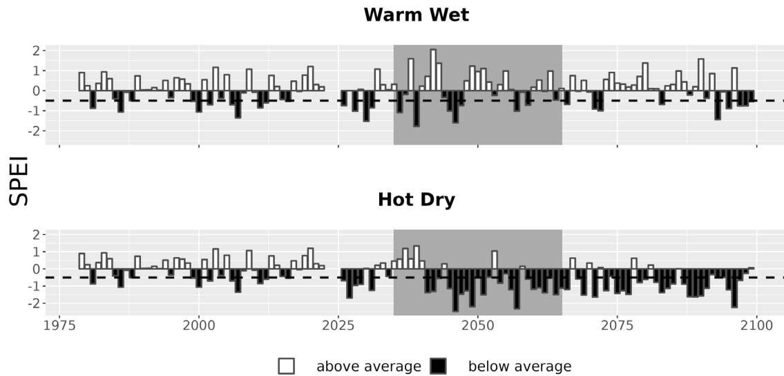
Figure 7. Drought metrics for HOBE. Drought index (SPEI; units = standard deviations from historical) timeseries for each climate future. Below-average SPEI (black bars) indicates dry conditions. The dotted line (SPEI = -0.5) indicates drought conditions.
