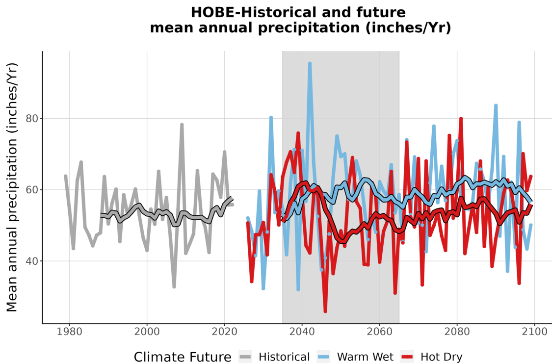
Figure 4. This graph compares observed average annual precipitation at HOBE (inches/year) (1979-2022) with projected average annual precipitation for the two climate futures over the period 2023-2099. The historically observed data is shown in gray, the Warm Wet climate future in blue, and the Hot Dry climate future in red. The smooth line running through each projection is the 10-year running average for historical observations and future projections. The gray-shaded area represents the time period that was averaged (2035-2065) to summarize future projections for the year 2050 (Appendix 1).
