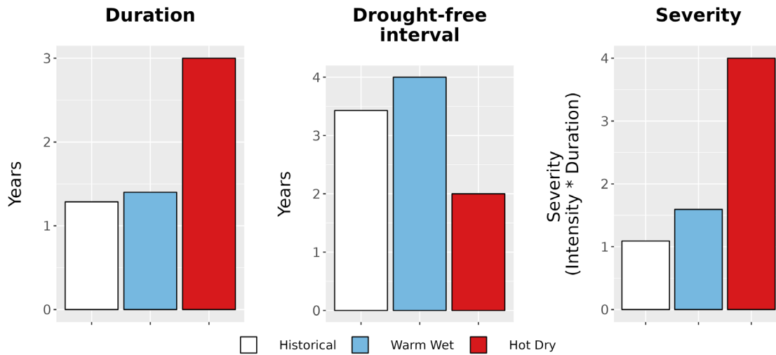
Figure 8. Drought metrics for HOBE. (Left) Average drought duration (years) historically (1979-2012) and under each climate future. (Middle) Average drought return interval (years), indicating the expected amount of time between periods of drought, historically and under each climate future. (Right) Average drought severity, a measure of drought intensity multiplied by duration, historically and under each climate future.
