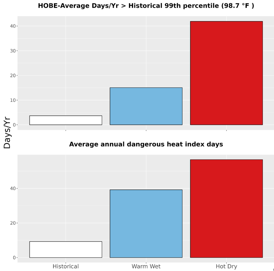
Figure 5. The upper bar graph represents the average number of days annually with temperatures greater than the historical 99th percentile (98.7 °F) historically (1979-2012) and for the two climate futures (2050). The bottom bar graph represents the average annual number of dangerous heat index days historically and for the two climate futures. Dangerous heat index days are days that exceed 105 °F.
