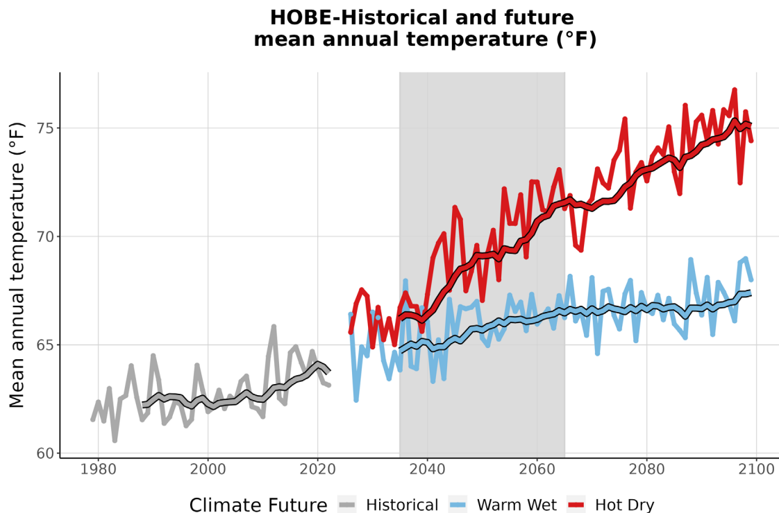
Figure 3. This graph compares observed average annual temperature at HOBE (°F) (1979-2022) with projected average annual temperature for the two climate futures over the period 2023-2099. The historically observed data
