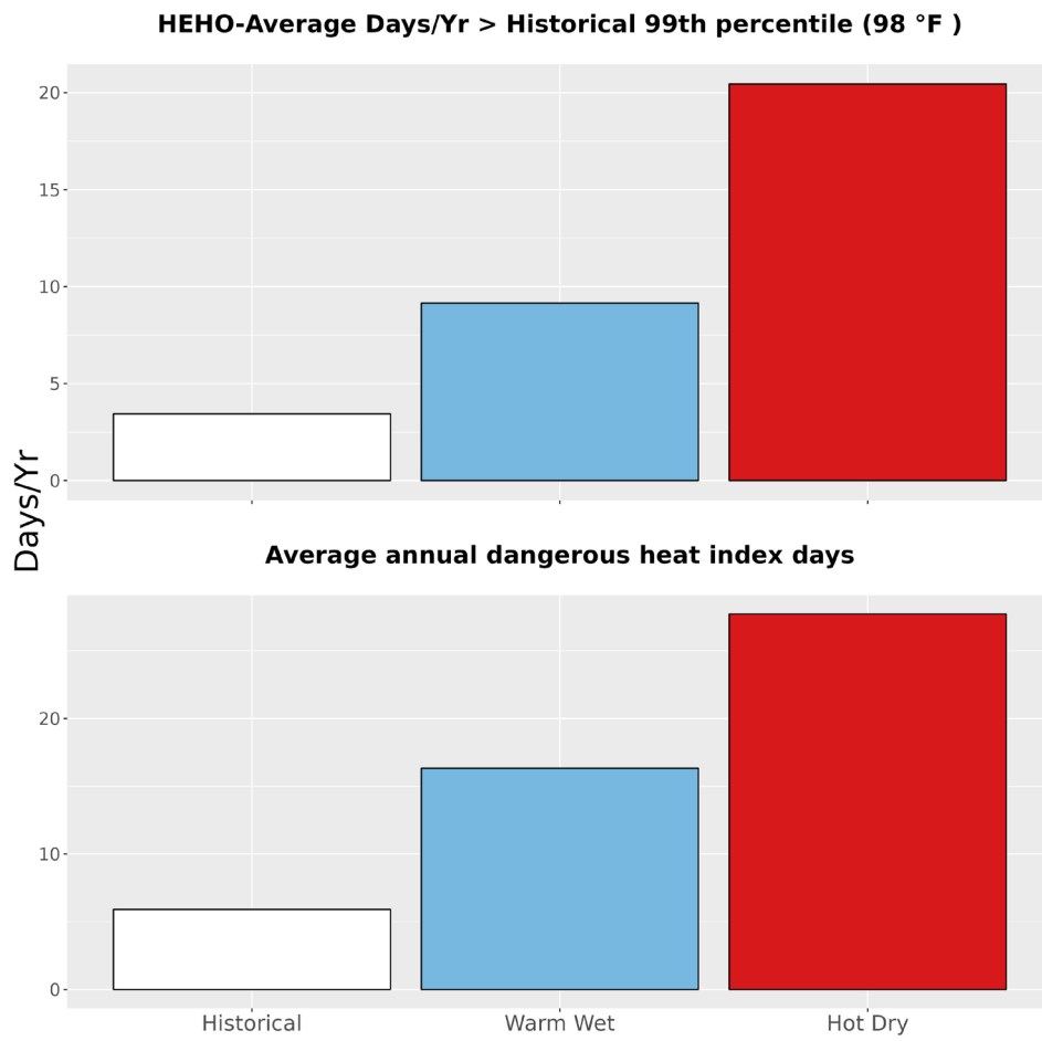
Figure 5. The upper bar graph represents the average number of days annually with temperatures greater than the historical 99th percentile (98 °F) historically (1979-2012) and for the two climate futures (2050). The bottom bar graph represents the average annual number of dangerous heat index days historically and for the two climate futures. Dangerous heat index days are days that exceed 105 °F.
