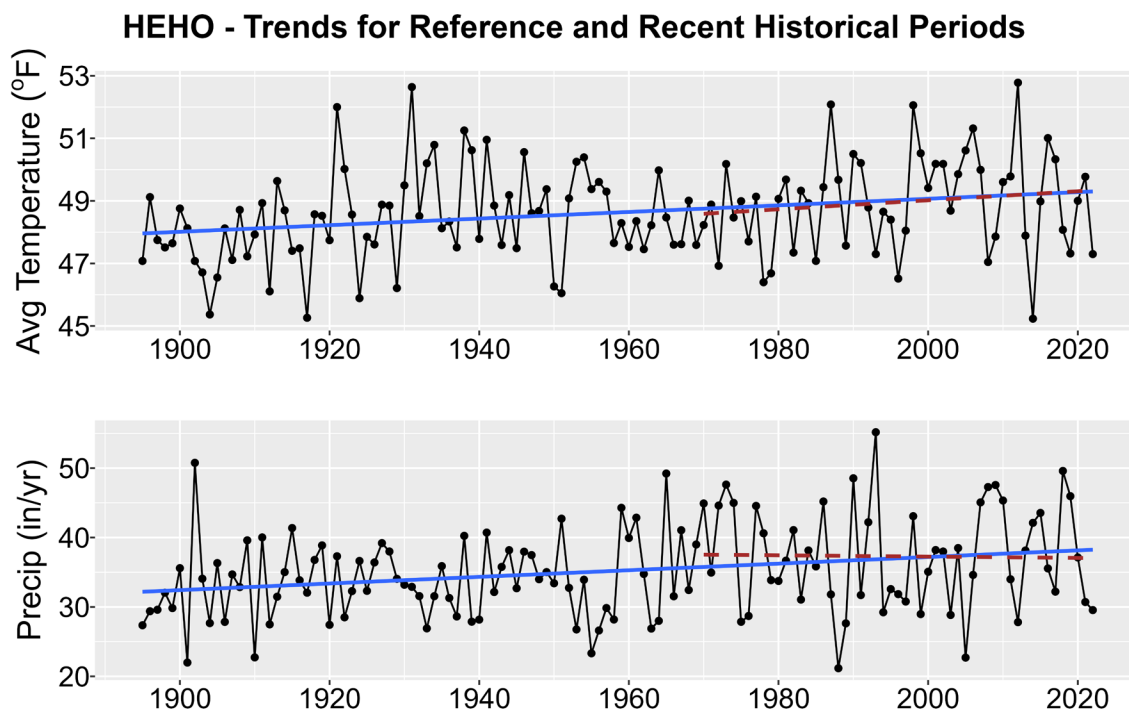
Figure 1. Historical trends in annual average temperature (upper plot) and annual total precipitation (lower plot) for HEHO from 1895-2022. Black points show yearly values while blue lines are linear regressions for the entire period record and red lines for 1970-2022 trends. Solid lines are significant trends (i.e., p < 0.05 ); dashed lines are not statistically significant.
