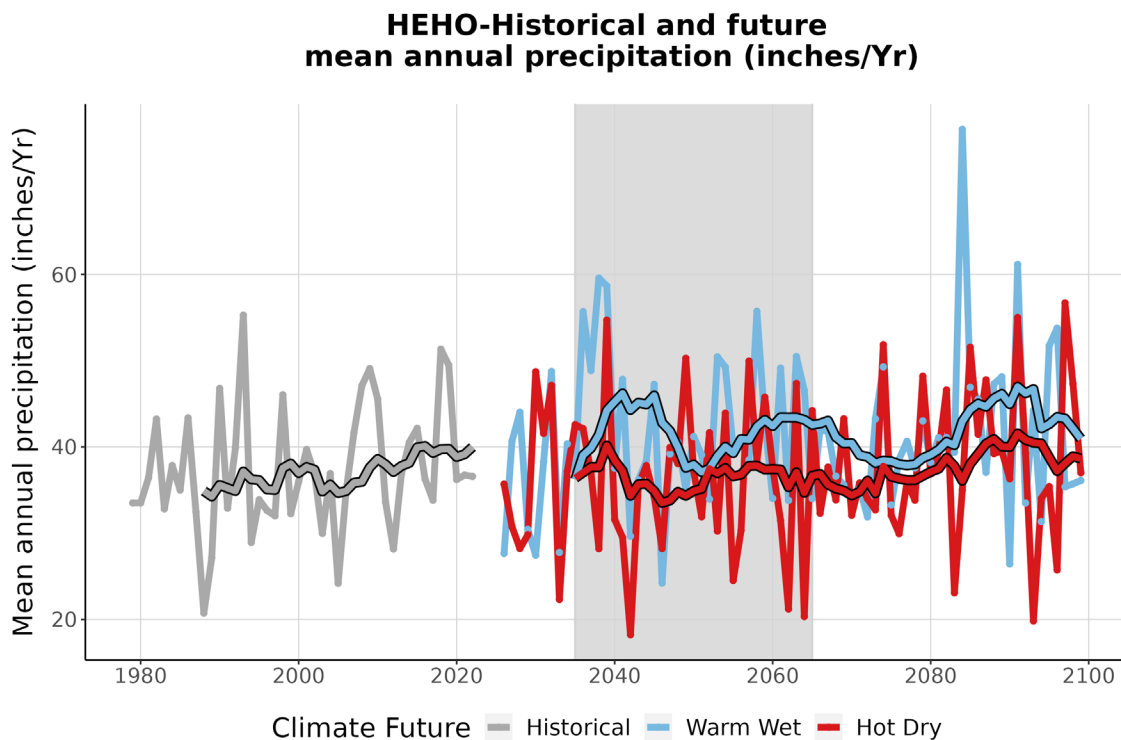
Figure 4. This graph compares observed average annual precipitation at HEHO (inches/year) (1979-2022) with projected average annual precipitation for the two climate futures over the period 2023-2099. The historically observed data is shown in gray, the Warm Wet climate future in blue, and the Hot Dry climate future in red. The smooth line running through each projection is the 10-year running average for historical observations and future projections. The gray-shaded area represents the time period that was averaged (2035-2065) to summarize future projections for the year 2050 (Appendix 1).
