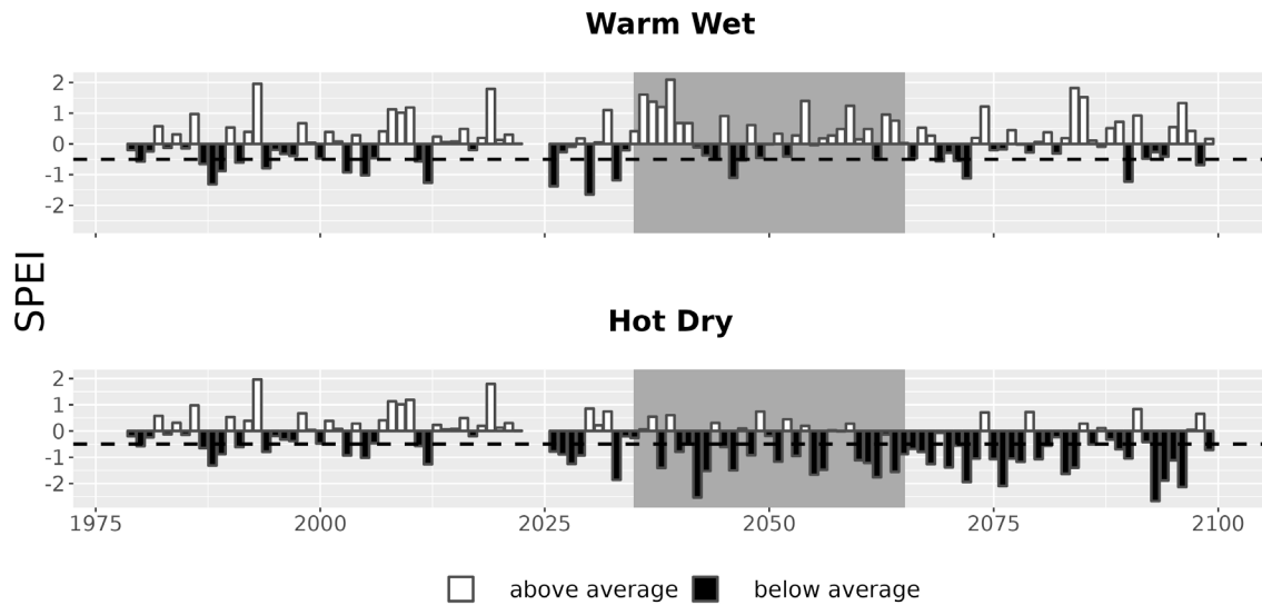
Figure 7. Drought metrics for HEHO. Drought index (SPEI; units = standard deviations from historical) timeseries for each climate future. Below-average SPEI (black bars) indicates dry conditions. The dotted line (SPEI = -0.5) indicates drought conditions.
