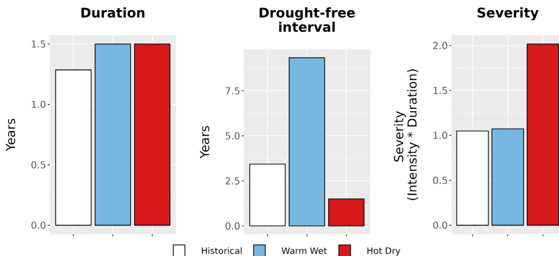
Figure 8. Drought metrics for HEHO. (Left) Average drought duration (years) historically (1979-2012) and under each climate future. (Middle) Average drought return interval (years), indicating the expected amount of time between periods of drought, historically and under each climate future. (Right) Average drought severity, a measure of drought intensity multiplied by duration, historically and under each climate future.
