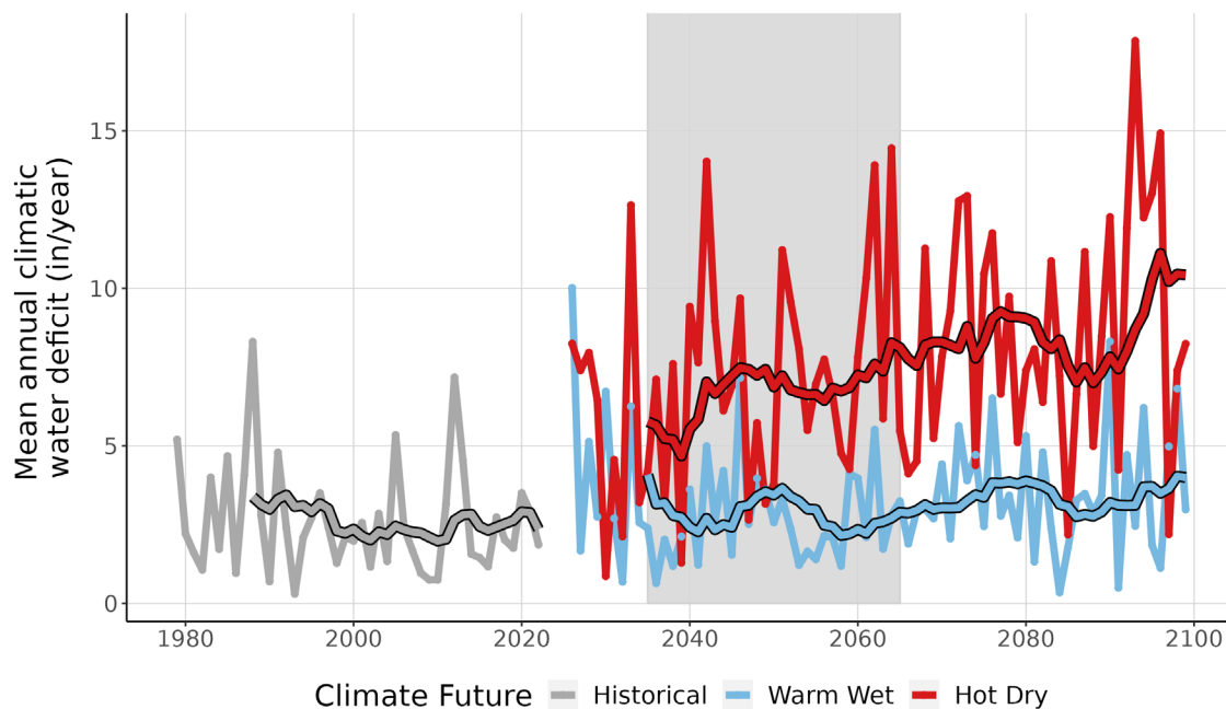
Figure 9. This line graph compares observed climatic water deficit at HEHO (inches/year) (1979-2022) with projected climatic water deficit for the two climate futures over the period 2023-2099. The historical observation data is shown in gray, the Warm Wet climate future in blue, and the Hot Dry climate future in red. The smooth line running through each projection is the 10-year running average for historical observations and future projections. Gray-shaded area represents the time period that was averaged (2035-2065) to summarize future projections for the year 2050.
