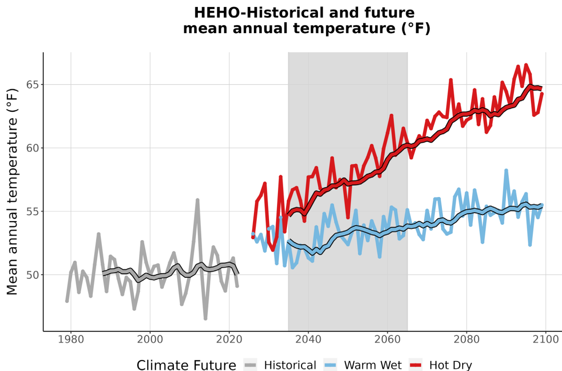
Figure 3. This graph compares observed average annual temperature at HEHO (°F) (1979-2022) with projected average annual temperature for the two climate futures over the period 2023-2099. The historically observed data
