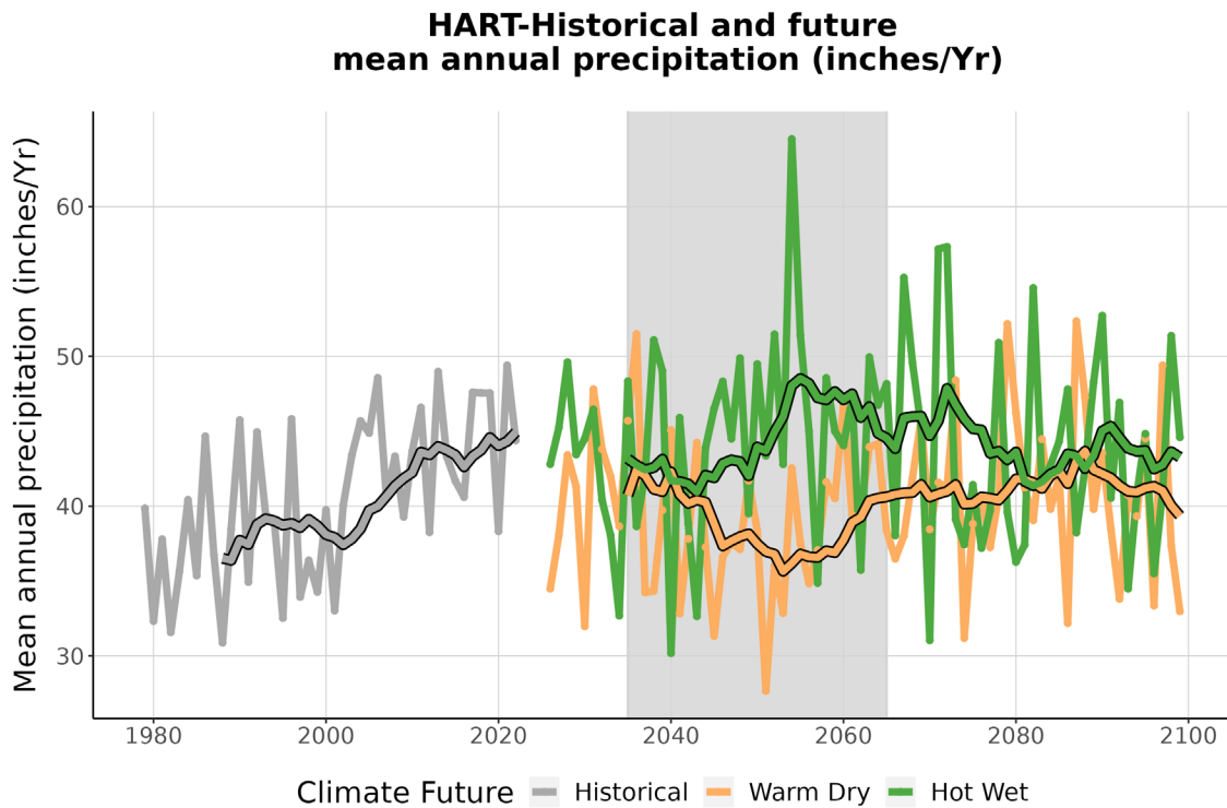
Figure 4. This graph compares observed average annual precipitation at HART (inches/year) (1979-2022) with projected average annual precipitation for the two climate futures over the period 2023-2099. The historically observed data is shown in gray, the Warm Dry climate future in orange, and the Hot Wet climate future in green. The smooth line running through each projection is the 10-year running average for historical observations and future projections. The gray-shaded area represents the time period that was averaged (2035-2065) to summarize future projections for the year 2050 (Appendix 1).
