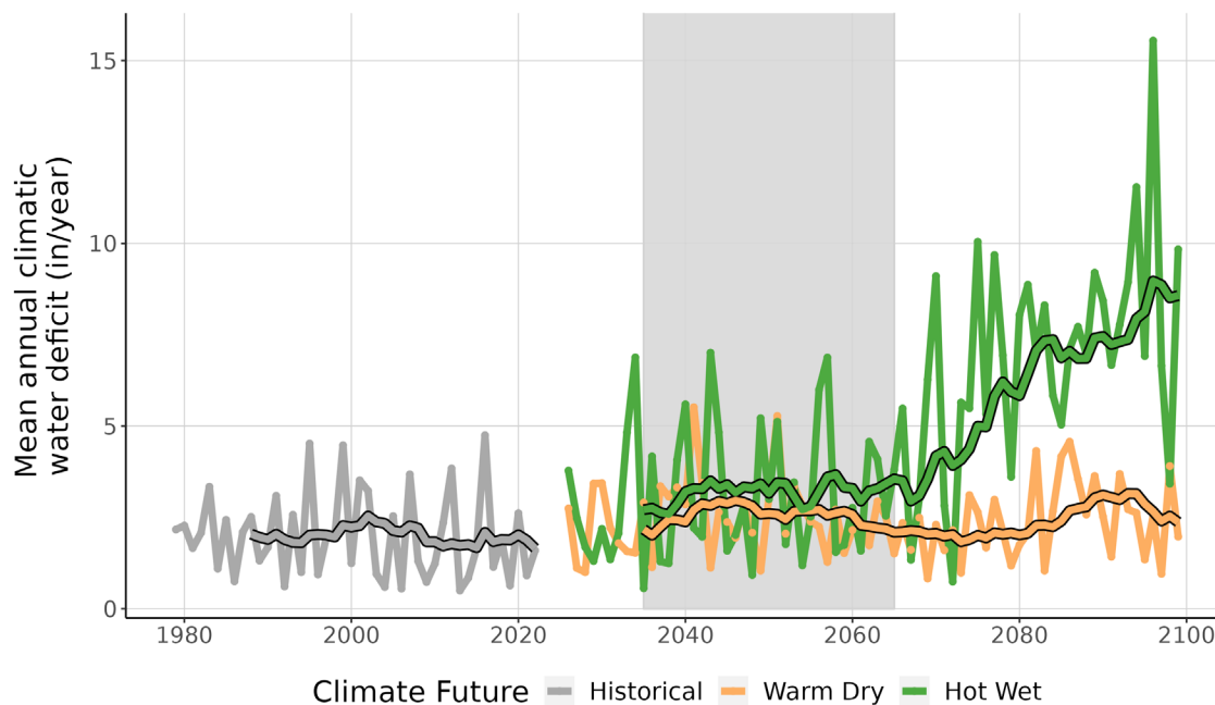
Figure 9. This line graph compares observed climatic water deficit at HART (inches/year) (1979-2022) with projected climatic water deficit for the two climate futures over the period 2023-2099. The historical observation data is shown in gray, the Warm Dry climate future in orange, and the Hot Wet climate future in green. The smooth line running through each projection is the 10-year running average for historical observations and future projections. Gray-shaded area represents the time period that was averaged (2035-2065) to summarize future projections for the year 2050.
