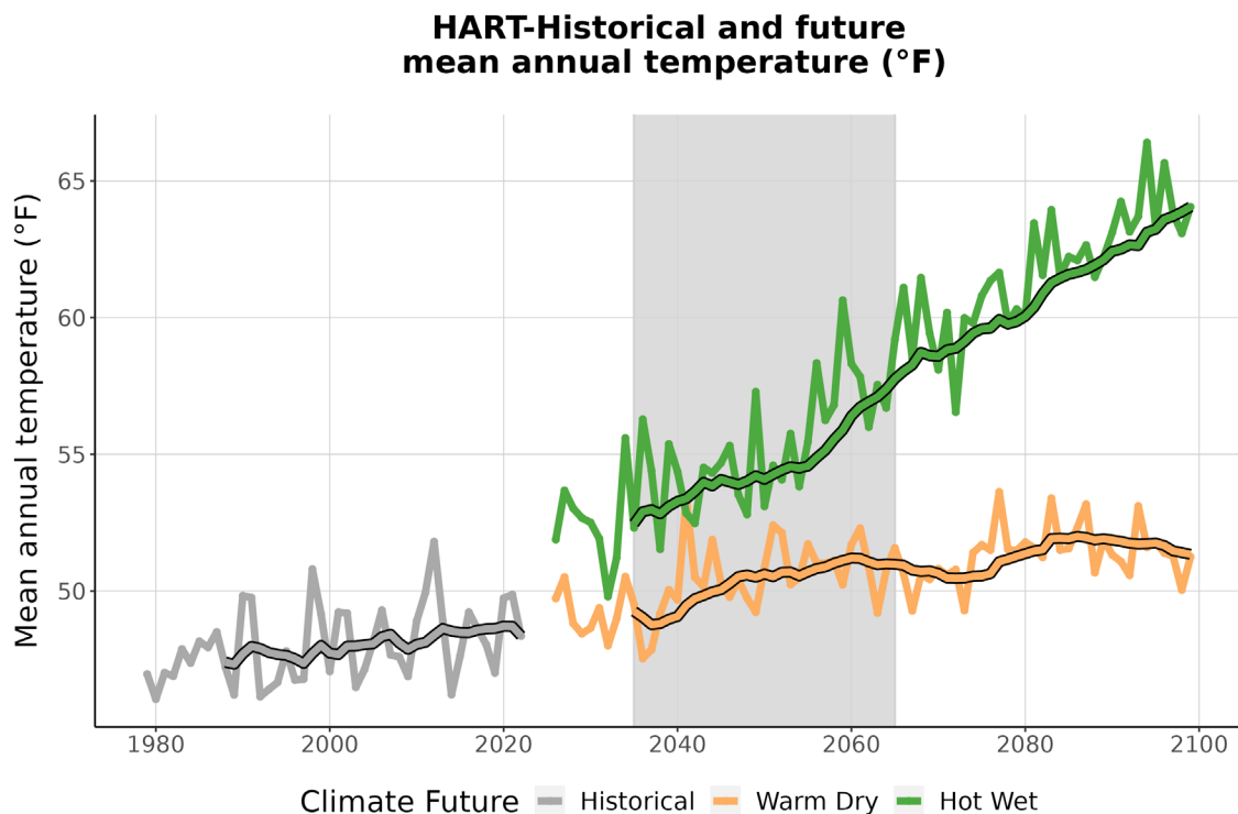
Figure 3. This graph compares observed average annual temperature at HART (°F) (1979-2022) with projected average annual temperature for the two climate futures over the period 2023-2099. The historically observed data
