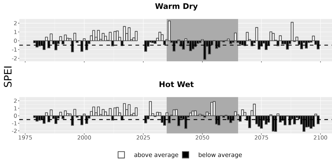
Figure 7. Drought metrics for HART. Drought index (SPEI; units = standard deviations from historical) timeseries for each climate future. Below-average SPEI (black bars) indicates dry conditions. The dotted line (SPEI = -0.5) indicates drought conditions.
