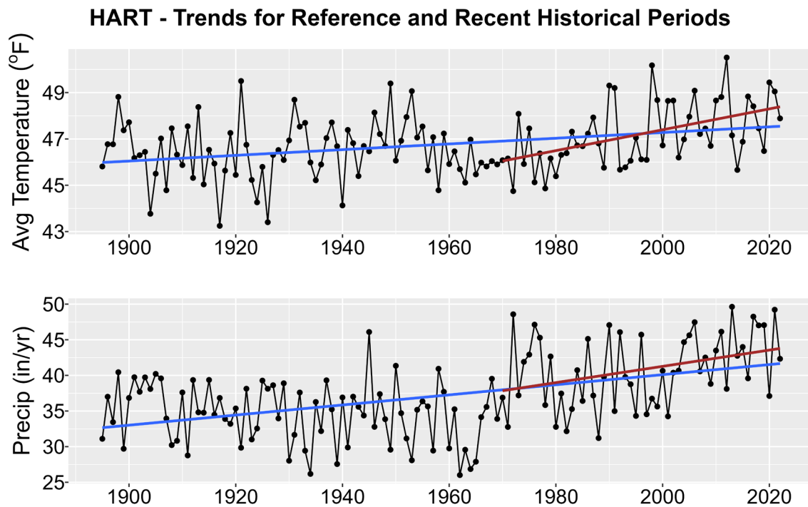
Figure 1. Historical trends in annual average temperature (upper plot) and annual total precipitation (lower plot) for HART from 1895-2022. Black points show yearly values while blue lines are linear regressions for the entire period record and red lines for 1970-2022 trends. Solid lines are significant trends (i.e., p < 0.05 ); dashed lines are not statistically significant.
