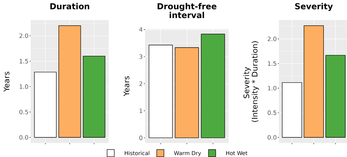
Figure 8. Drought metrics for HART. (Left) Average drought duration (years) historically (1979-2012) and under each climate future. (Middle) Average drought return interval (years), indicating the expected amount of time between periods of drought, historically and under each climate future. (Right) Average drought severity, a measure of drought intensity multiplied by duration, historically and under each climate future.
