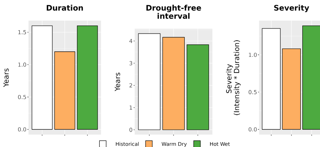
Figure 8. Drought metrics for HAMP. (Left) Average drought duration (years) historically (1979-2012) and under each climate future. (Middle) Average drought return interval (years), indicating the expected amount of time between periods of drought, historically and under each climate future. (Right) Average drought severity, a measure of drought intensity multiplied by duration, historically and under each climate future.
