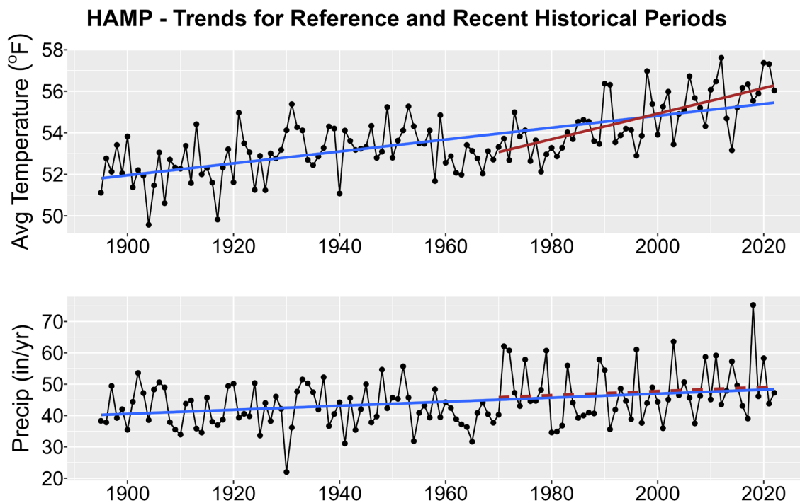
Figure 1. Historical trends in annual average temperature (upper plot) and annual total precipitation (lower plot) for HAMP from 1895-2022. Black points show yearly values while blue lines are linear regressions for the entire period record and red lines for 1970-2022 trends. Solid lines are significant trends (i.e., p < 0.05 ); dashed lines are not statistically significant.
