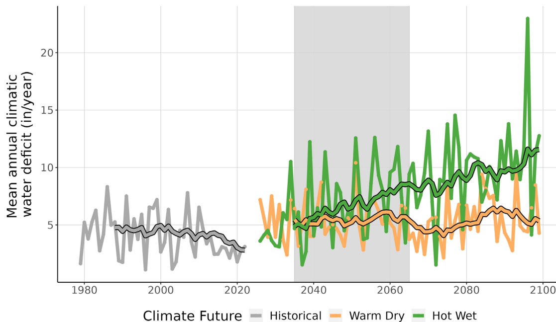
Figure 9. This line graph compares observed climatic water deficit at HAMP (inches/year) (1979-2022) with projected climatic water deficit for the two climate futures over the period 2023-2099. The historical observation data is shown in gray, the Warm Dry climate future in orange, and the Hot Wet climate future in green. The smooth line running through each projection is the 10-year running average for historical observations and future projections. Gray-shaded area represents the time period that was averaged (2035-2065) to summarize future projections for the year 2050.
