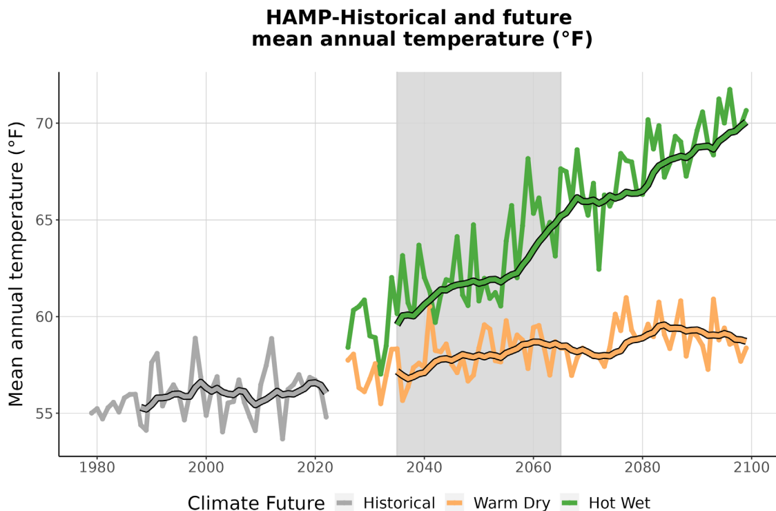
Figure 3. This graph compares observed average annual temperature at HAMP (°F) (1979-2022) with projected average annual temperature for the two climate futures over the period 2023-2099. The historically observed data
