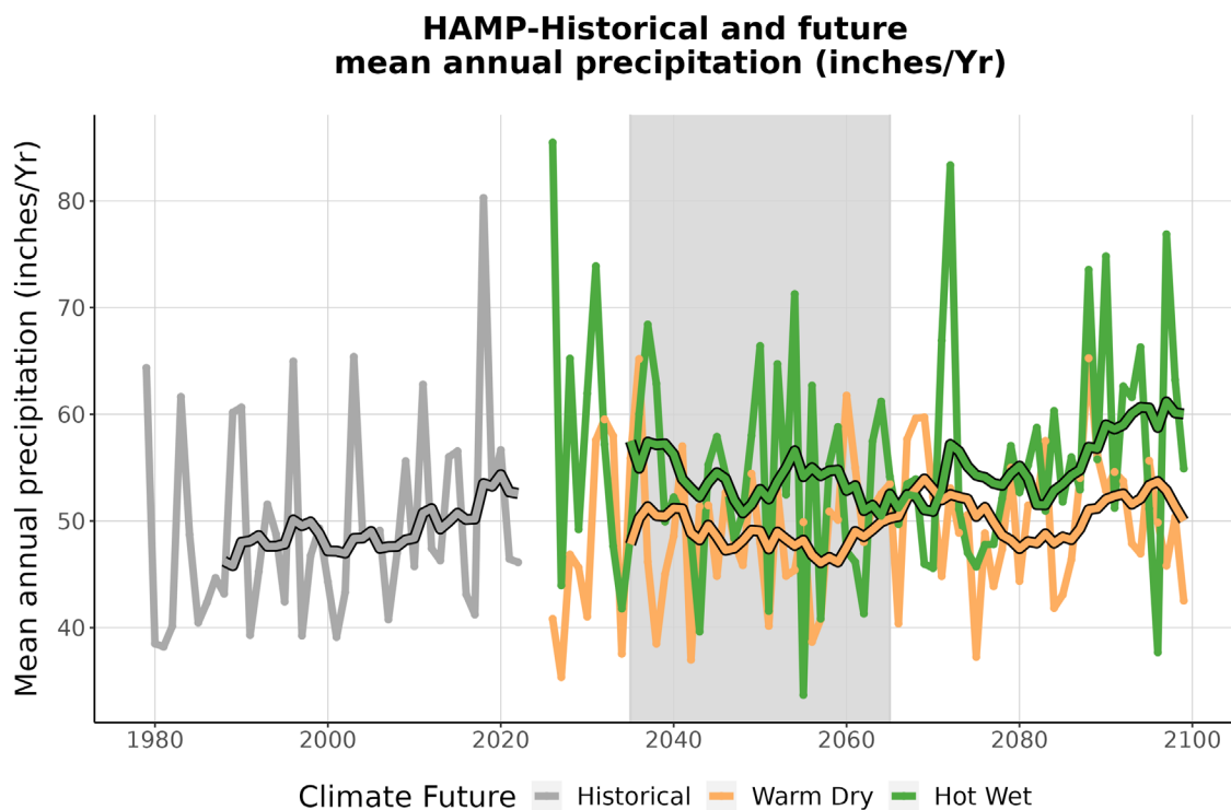
Figure 4. This graph compares observed average annual precipitation at HAMP (inches/year) (1979-2022) with projected average annual precipitation for the two climate futures over the period 2023-2099. The historically observed data is shown in gray, the Warm Dry climate future in orange, and the Hot Wet climate future in green. The smooth line running through each projection is the 10-year running average for historical observations and future projections. The gray-shaded area represents the time period that was averaged (2035-2065) to summarize future projections for the year 2050 (Appendix 1).
