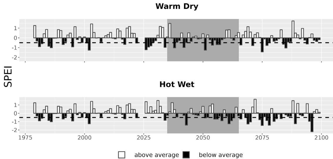
Figure 7. Drought metrics for HAMP. Drought index (SPEI; units = standard deviations from historical) timeseries for each climate future. Below-average SPEI (black bars) indicates dry conditions. The dotted line (SPEI = -0.5) indicates drought conditions.
