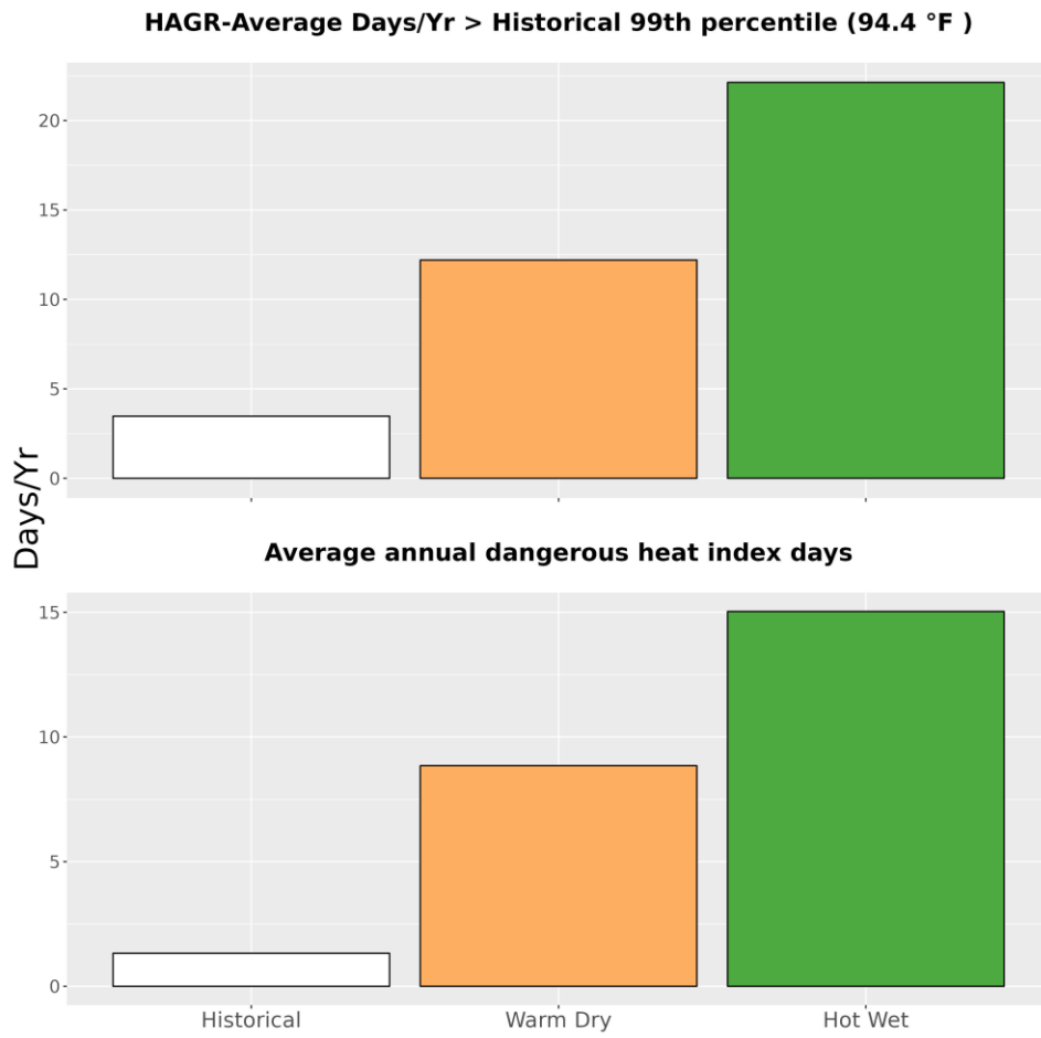
Figure 5. The upper bar graph represents the average number of days annually with temperatures greater than the historical 99th percentile (94.4 °F) historically (1979-2012) and for the two climate futures (2050). The bottom bar graph represents the average annual number of dangerous heat index days historically and for the two climate futures. Dangerous heat index days are days that exceed 105 °F.
