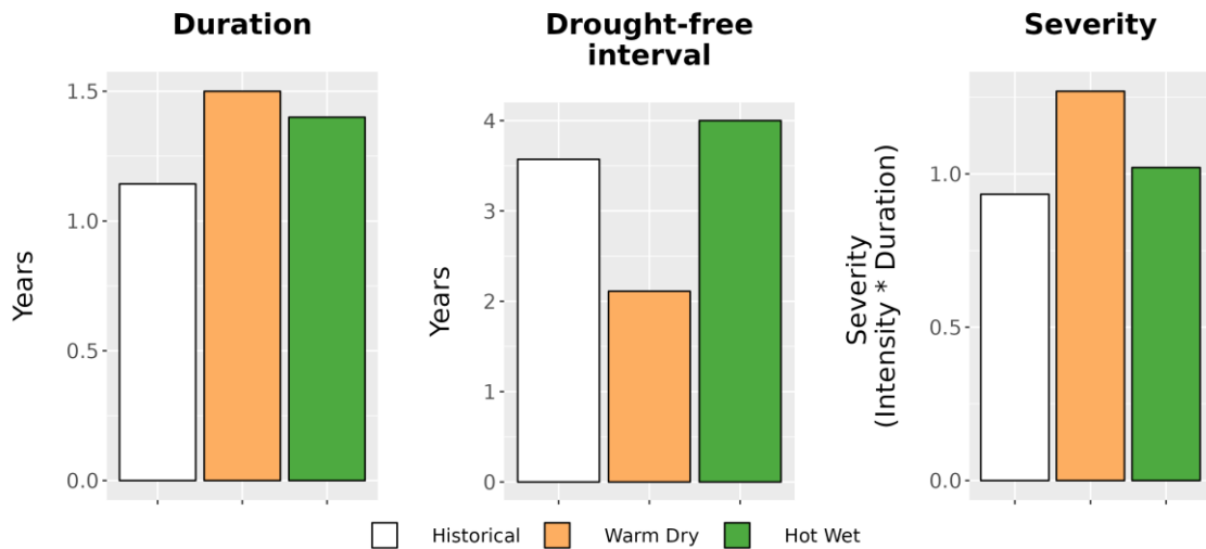
Figure 8. Drought metrics for HAGR. (Left) Average drought duration (years) historically (1979-2012) and under each climate future. (Middle) Average drought return interval (years), indicating the expected amount of time between periods of drought, historically and under each climate future. (Right) Average drought severity, a measure of drought intensity multiplied by duration, historically and under each climate future.
