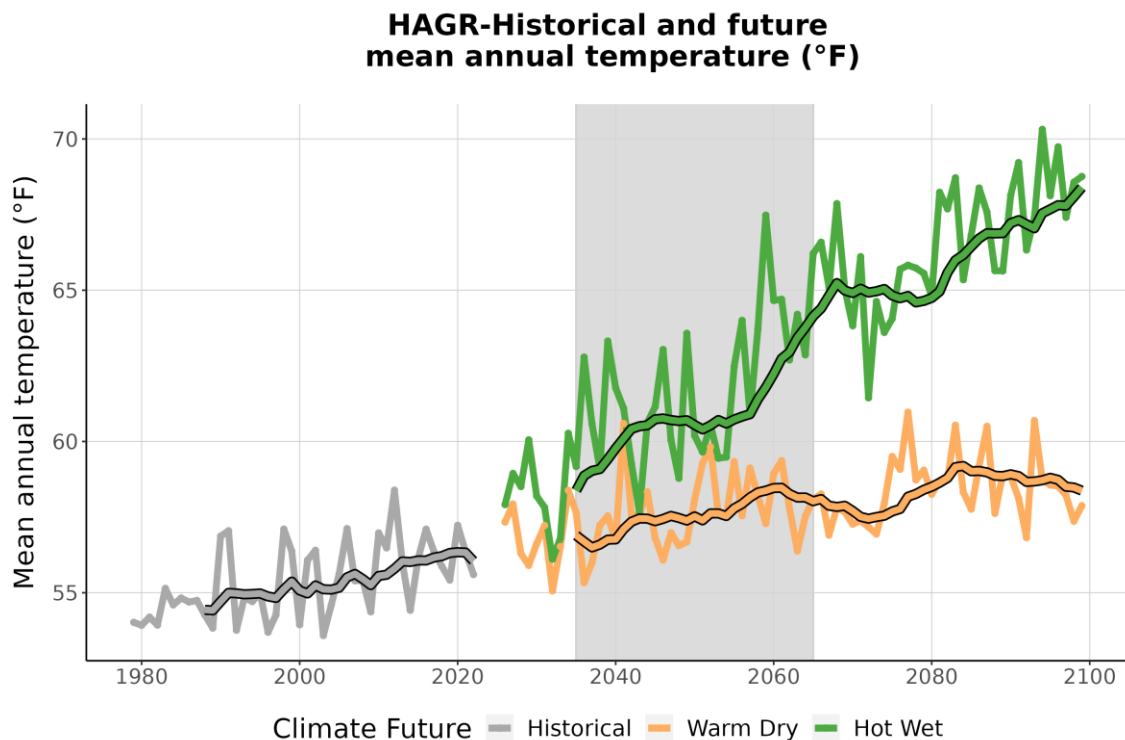
Figure 3. This graph compares observed average annual temperature at HAGR (°F) (1979-2022) with projected average annual temperature for the two climate futures over the period 2023-2099. The historically observed data
