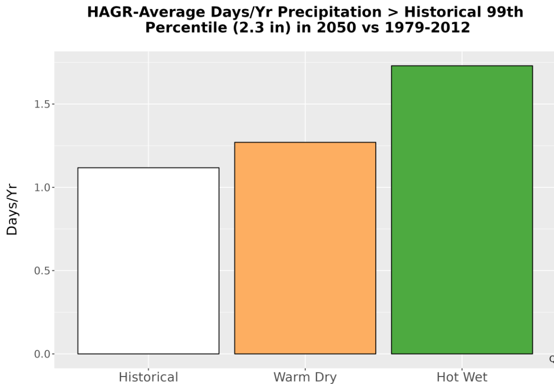
Figure 6. Average number of days annually with precipitation exceeding the 99th percentile (2.3 in.) of precipitation from the historical period 1979-2012 and for each climate future.
