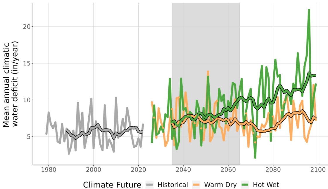
Figure 9. This line graph compares observed climatic water deficit at HAGR (inches/year) (1979-2022) with projected climatic water deficit for the two climate futures over the period 2023-2099. The historical observation data is shown in gray, the Warm Dry climate future in orange, and the Hot Wet climate future in green. The smooth line running through each projection is the 10-year running average for historical observations and future projections. Gray-shaded area represents the time period that was averaged (2035-2065) to summarize future projections for the year 2050.
