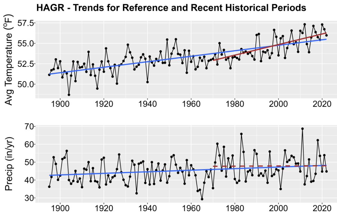
Figure 1. Historical trends in annual average temperature (upper plot) and annual total precipitation (lower plot) for HAGR from 1895-2022. Black points show yearly values while blue lines are linear regressions for the entire period record and red lines for 1970-2022 trends. Solid lines are significant trends (i.e., p < 0.05 ); dashed lines are not statistically significant.
