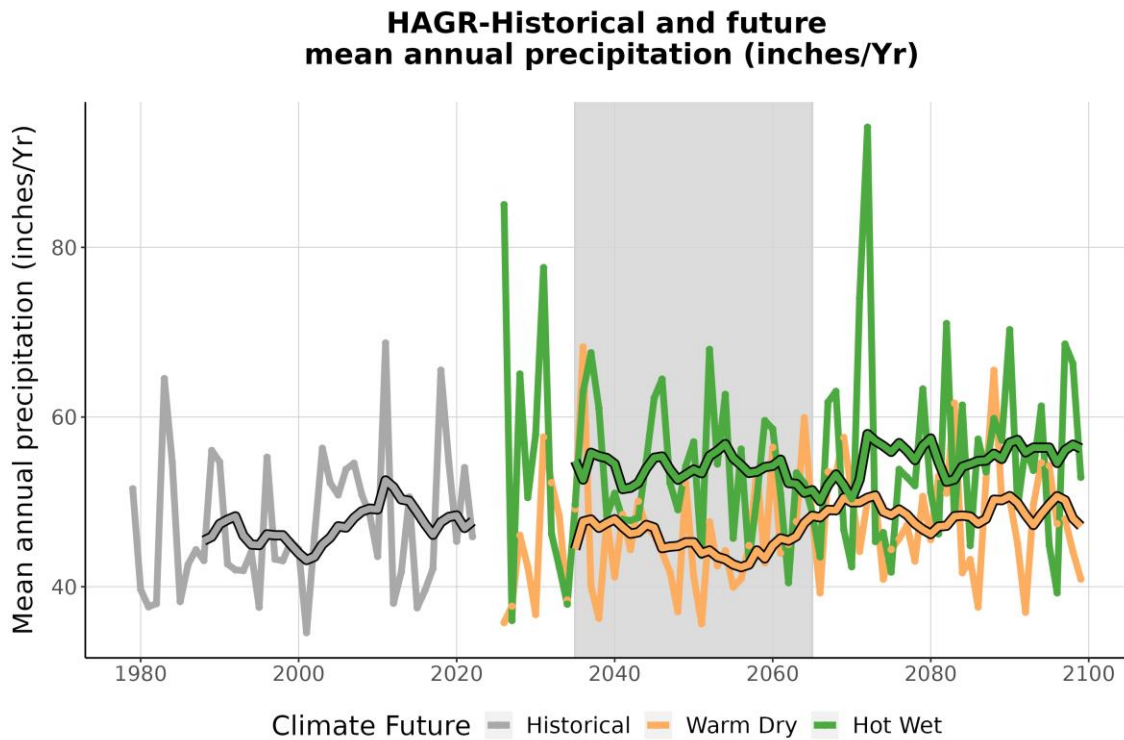
Figure 4. This graph compares observed average annual precipitation at HAGR (inches/year) (1979-2022) with projected average annual precipitation for the two climate futures over the period 2023-2099. The historically observed data is shown in gray, the Warm Dry climate future in orange, and the Hot Wet climate future in green. The smooth line running through each projection is the 10-year running average for historical observations and future projections. The gray-shaded area represents the time period that was averaged (2035-2065) to summarize future projections for the year 2050 (Appendix 1).
