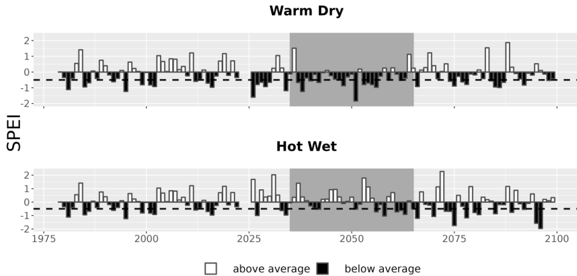
Figure 7. Drought metrics for HAGR. Drought index (SPEI; units = standard deviations from historical) timeseries for each climate future. Below-average SPEI (black bars) indicates dry conditions. The dotted line (SPEI = -0.5) indicates drought conditions.
