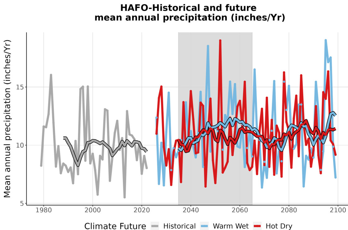
Figure 4. This graph compares observed average annual precipitation at HAFO (inches/year) (1979-2022) with projected average annual precipitation for the two climate futures over the period 2023-2099. The historically observed data is shown in gray, the Warm Wet climate future in blue, and the Hot Dry climate future in red. The smooth line running through each projection is the 10-year running average for historical observations and future projections. The gray-shaded area represents the time period that was averaged (2035-2065) to summarize future projections for the year 2050 (Appendix 1).
