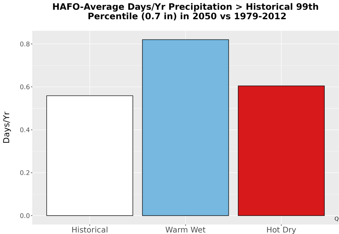
Figure 6. Average number of days annually with precipitation exceeding the 99th percentile (0.7 in.) of precipitation from the historical period 1979-2012 and for each climate future.
