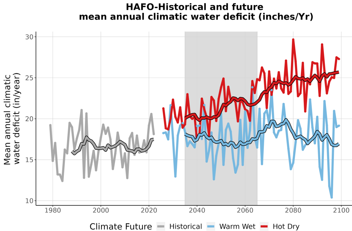
Figure 9. This line graph compares observed climatic water deficit at HAFO (inches/year) (1979-2022) with projected climatic water deficit for the two climate futures over the period 2023-2099. The historical observation data is shown in gray, the Warm Wet climate future in blue, and the Hot Dry climate future in red. The smooth line running through each projection is the 10-year running average for historical observations and future projections. Gray-shaded area represents the time period that was averaged (2035-2065) to summarize future projections for the year 2050.
