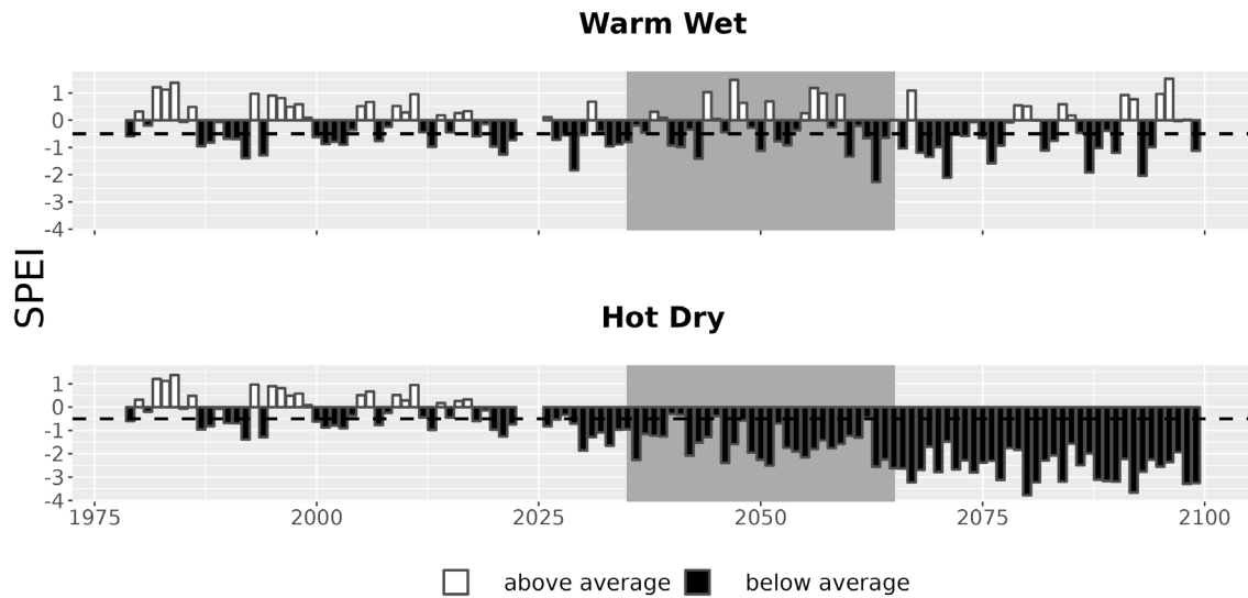
Figure 7. Drought metrics for HAFO. Drought index (SPEI; units = standard deviations from historical) timeseries for each climate future. Below-average SPEI (black bars) indicates dry conditions. The dotted line (SPEI = -0.5) indicates drought conditions.
