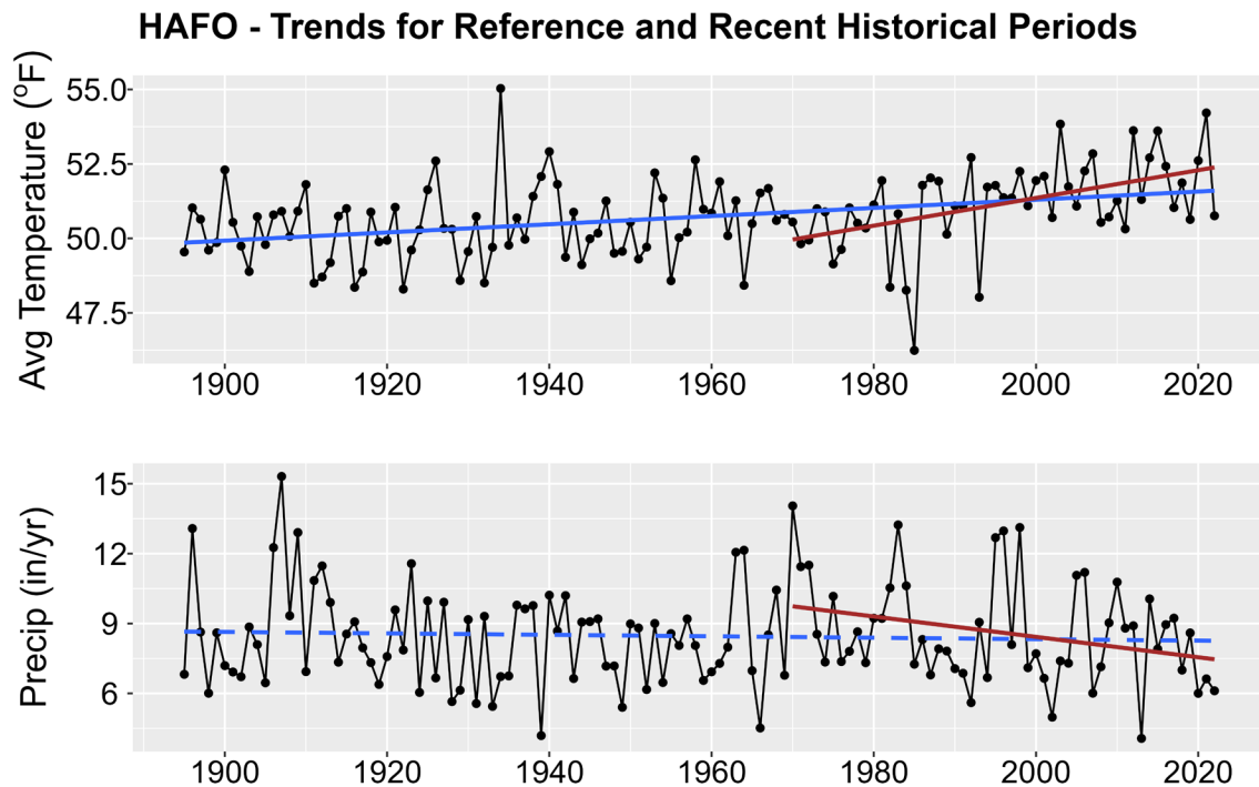
Figure 1. Historical trends in annual average temperature (upper plot) and annual total precipitation (lower plot) for HAFO from 1895-2022. Black points show yearly values while blue lines are linear regressions for the entire period record and red lines for 1970-2022 trends. Solid lines are significant trends (i.e., p < 0.05 ); dashed lines are not statistically significant.
