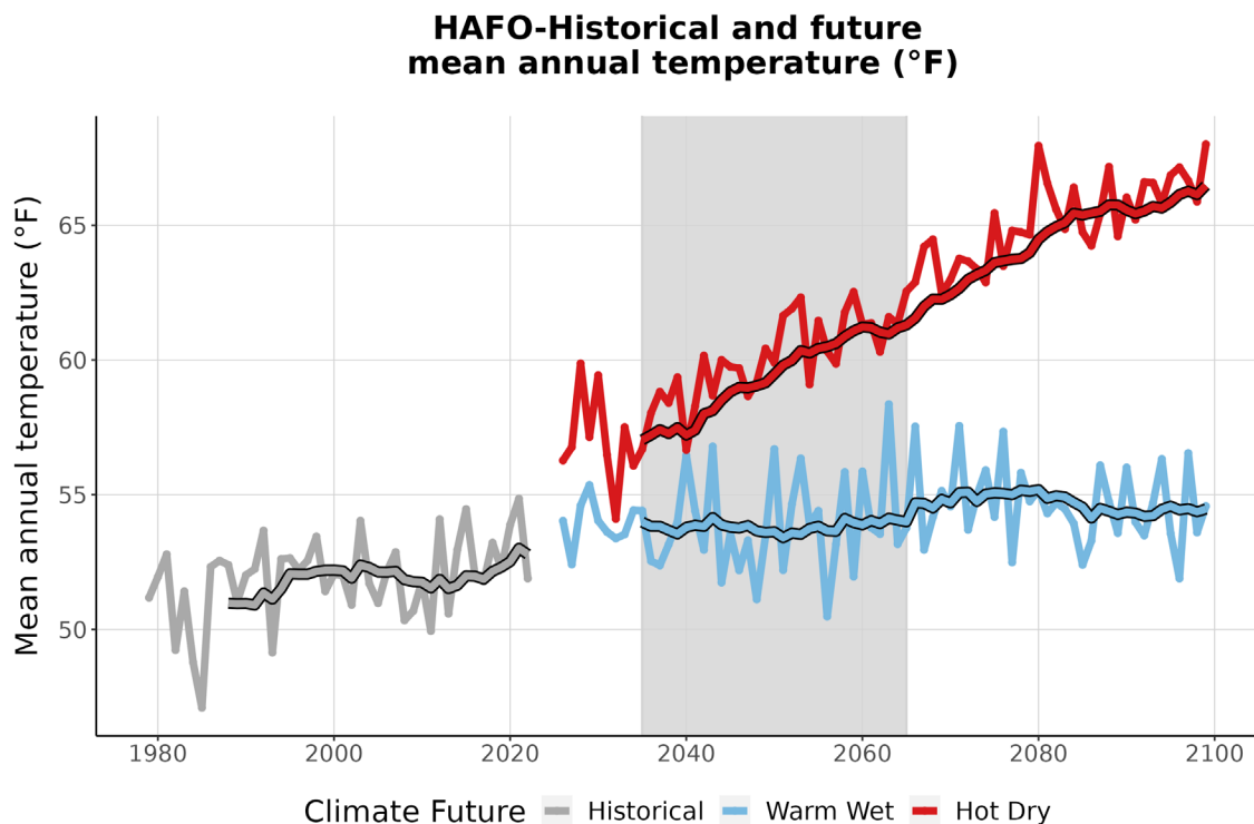
Figure 3. This graph compares observed average annual temperature at HAFO (°F) (1979-2022) with projected average annual temperature for the two climate futures over the period 2023-2099. The historically observed data
