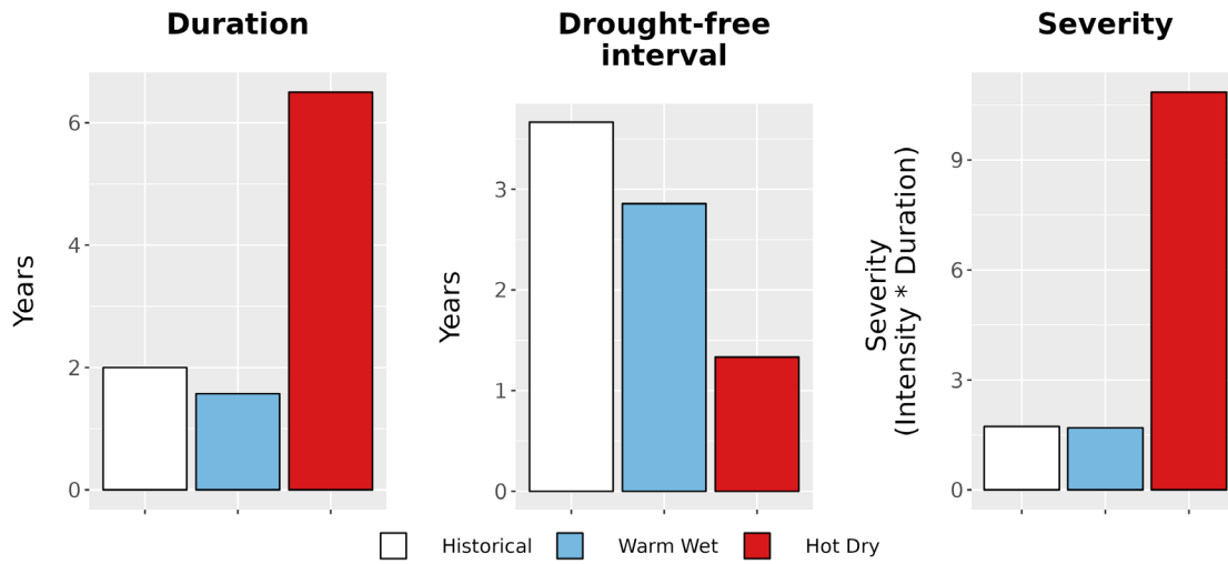
Figure 8. Drought metrics for HAFO. (Left) Average drought duration (years) historically (1979-2012) and under each climate future. (Middle) Average drought return interval (years), indicating the expected amount of time between periods of drought, historically and under each climate future. (Right) Average drought severity, a measure of drought intensity multiplied by duration, historically and under each climate future.
