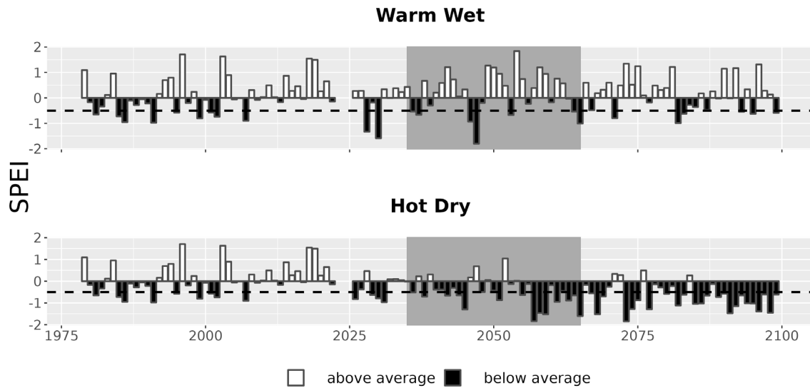
Figure 7. Drought metrics for HAFE. Drought index (SPEI; units = standard deviations from historical) timeseries for each climate future. Below-average SPEI (black bars) indicates dry conditions. The dotted line (SPEI = -0.5) indicates drought conditions.
