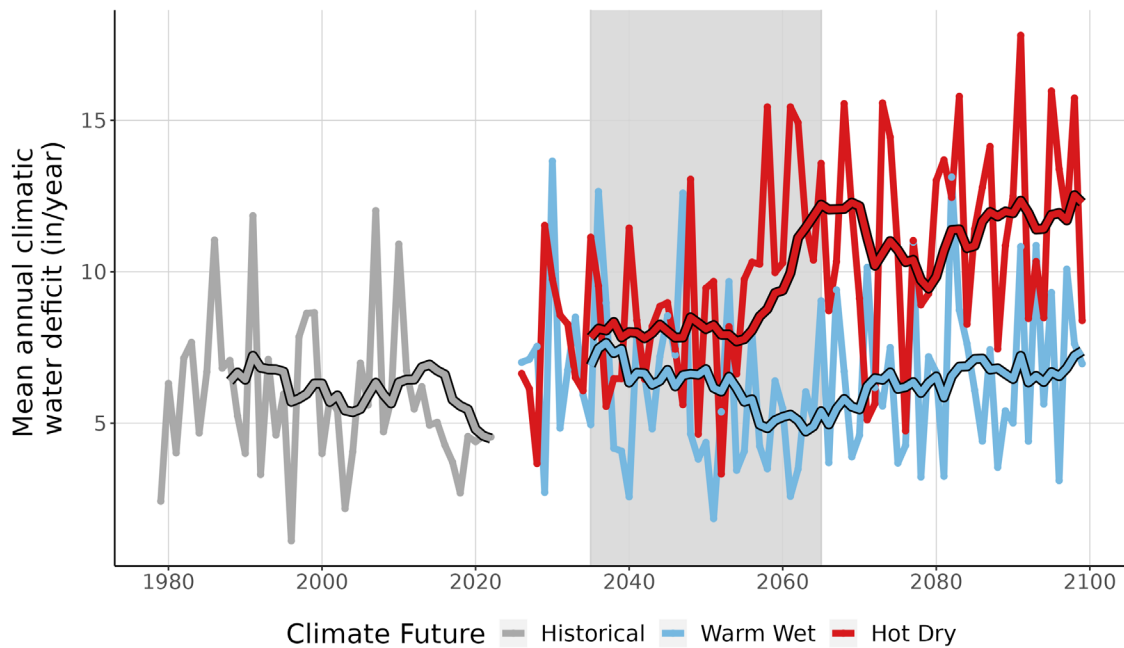
Figure 9. This line graph compares observed climatic water deficit at HAFE (inches/year) (1979-2022) with projected climatic water deficit for the two climate futures over the period 2023-2099. The historical observation data is shown in gray, the Warm Wet climate future in blue, and the Hot Dry climate future in red. The smooth line running through each projection is the 10-year running average for historical observations and future projections. Gray-shaded area represents the time period that was averaged (2035-2065) to summarize future projections for the year 2050.
