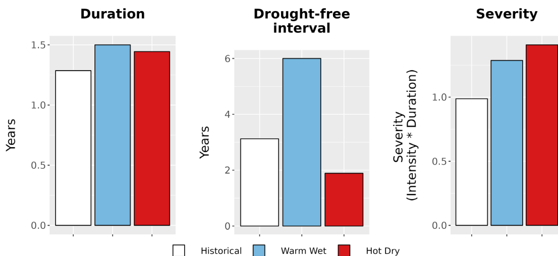
Figure 8. Drought metrics for HAFE. (Left) Average drought duration (years) historically (1979-2012) and under each climate future. (Middle) Average drought return interval (years), indicating the expected amount of time between periods of drought, historically and under each climate future. (Right) Average drought severity, a measure of drought intensity multiplied by duration, historically and under each climate future.
