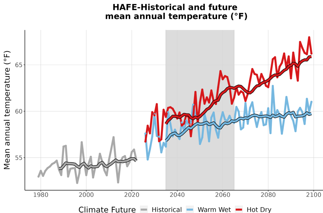
Figure 3. This graph compares observed average annual temperature at HAFE (°F) (1979-2022) with projected average annual temperature for the two climate futures over the period 2023-2099. The historically observed data
