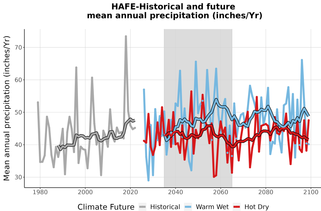
Figure 4. This graph compares observed average annual precipitation at HAFE (inches/year) (1979-2022) with projected average annual precipitation for the two climate futures over the period 2023-2099. The historically observed data is shown in gray, the Warm Wet climate future in blue, and the Hot Dry climate future in red. The smooth line running through each projection is the 10-year running average for historical observations and future projections. The gray-shaded area represents the time period that was averaged (2035-2065) to summarize future projections for the year 2050 (Appendix 1).
