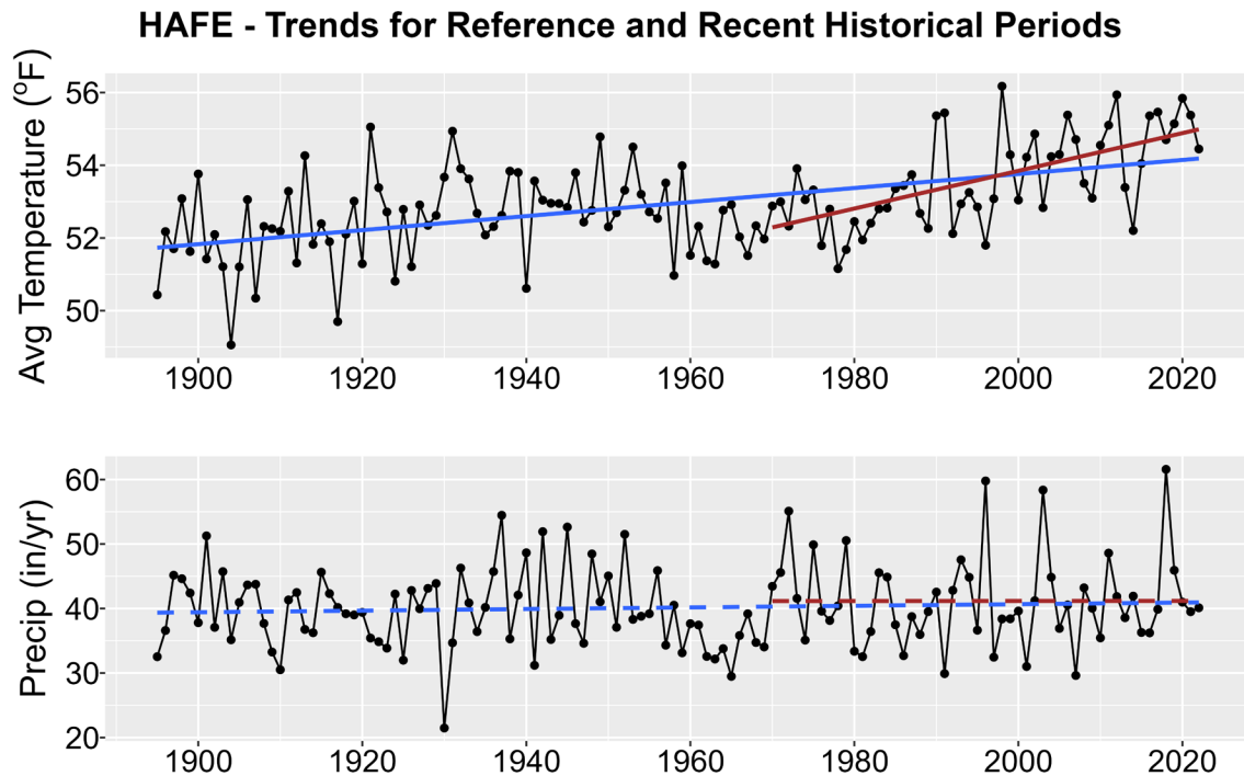
Figure 1. Historical trends in annual average temperature (upper plot) and annual total precipitation (lower plot) for HAFE from 1895-2022. Black points show yearly values while blue lines are linear regressions for the entire period record and red lines for 1970-2022 trends. Solid lines are significant trends (i.e., p < 0.05 ); dashed lines are not statistically significant.
