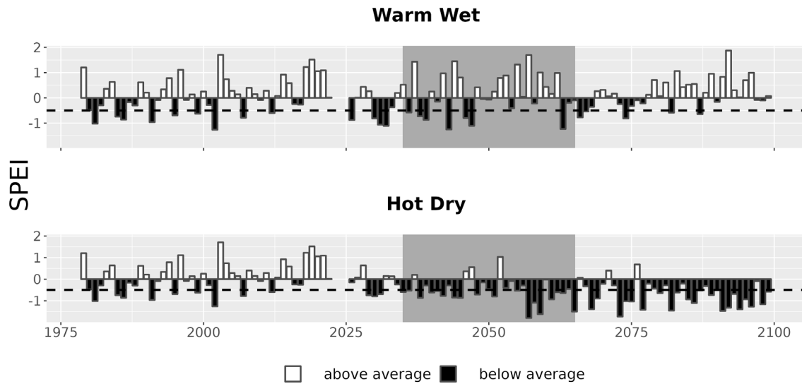
Figure 7. Drought metrics for GWMP. Drought index (SPEI; units = standard deviations from historical) timeseries for each climate future. Below-average SPEI (black bars) indicates dry conditions. The dotted line (SPEI = -0.5) indicates drought conditions.
