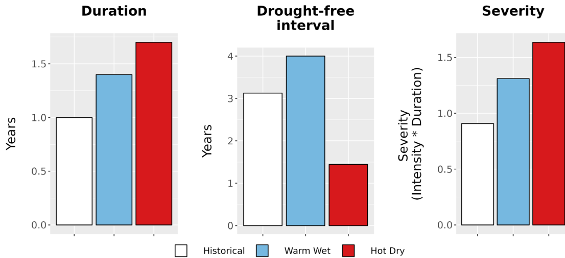
Figure 8. Drought metrics for GWMP. (Left) Average drought duration (years) historically (1979-2012) and under each climate future. (Middle) Average drought return interval (years), indicating the expected amount of time between periods of drought, historically and under each climate future. (Right) Average drought severity, a measure of drought intensity multiplied by duration, historically and under each climate future.
