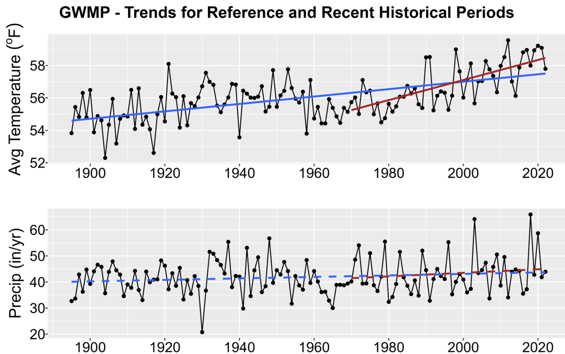
Figure 1. Historical trends in annual average temperature (upper plot) and annual total precipitation (lower plot) for GWMP from 1895-2022. Black points show yearly values while blue lines are linear regressions for the entire period record and red lines for 1970-2022 trends. Solid lines are significant trends (i.e., p < 0.05 ); dashed lines are not statistically significant.
