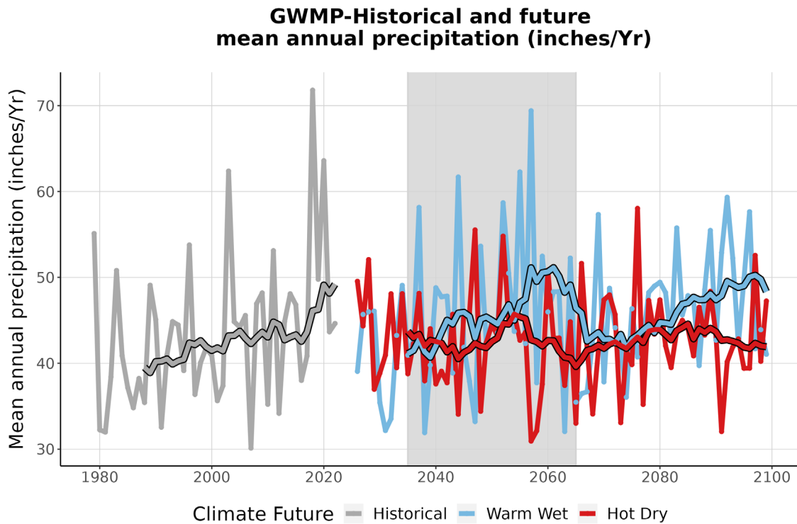
Figure 4. This graph compares observed average annual precipitation at GWMP (inches/year) (1979-2022) with projected average annual precipitation for the two climate futures over the period 2023-2099. The historically observed data is shown in gray, the Warm Wet climate future in blue, and the Hot Dry climate future in red. The smooth line running through each projection is the 10-year running average for historical observations and future projections. The gray-shaded area represents the time period that was averaged (2035-2065) to summarize future projections for the year 2050 (Appendix 1).
