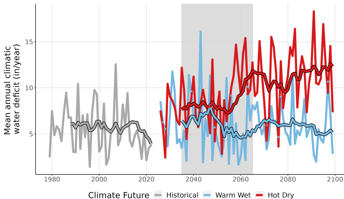
Figure 9. This line graph compares observed climatic water deficit at GWMP (inches/year) (1979-2022) with projected climatic water deficit for the two climate futures over the period 2023-2099. The historical observation data is shown in gray, the Warm Wet climate future in blue, and the Hot Dry climate future in red. The smooth line running through each projection is the 10-year running average for historical observations and future projections. Gray-shaded area represents the time period that was averaged (2035-2065) to summarize future projections for the year 2050.
