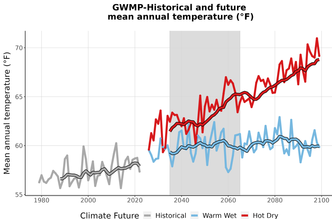
Figure 3. This graph compares observed average annual temperature at GWMP (°F) (1979-2022) with projected average annual temperature for the two climate futures over the period 2023-2099. The historically observed data
