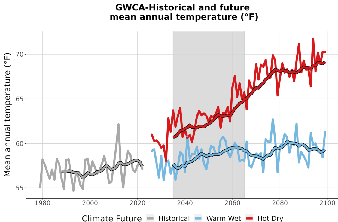
Figure 3. This graph compares observed average annual temperature at GWCA (°F) (1979-2022) with projected average annual temperature for the two climate futures over the period 2023-2099. The historically observed data
