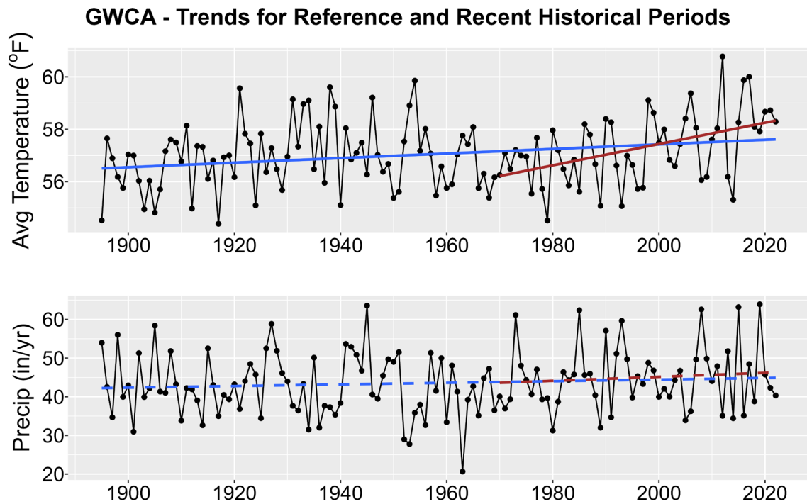
Figure 1. Historical trends in annual average temperature (upper plot) and annual total precipitation (lower plot) for GWCA from 1895-2022. Black points show yearly values while blue lines are linear regressions for the entire period record and red lines for 1970-2022 trends. Solid lines are significant trends (i.e., p < 0.05 ); dashed lines are not statistically significant.
