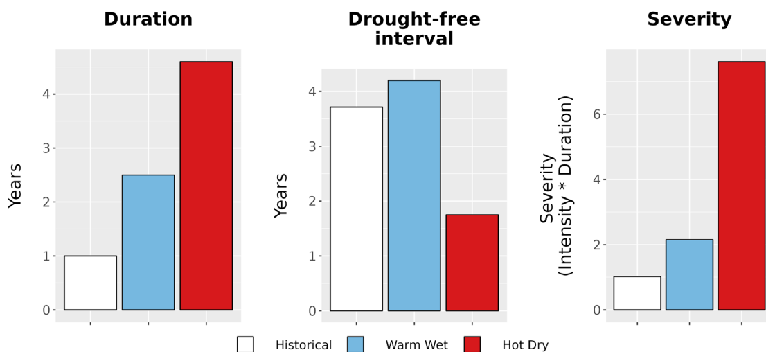
Figure 8. Drought metrics for GWCA. (Left) Average drought duration (years) historically (1979-2012) and under each climate future. (Middle) Average drought return interval (years), indicating the expected amount of time between periods of drought, historically and under each climate future. (Right) Average drought severity, a measure of drought intensity multiplied by duration, historically and under each climate future.
