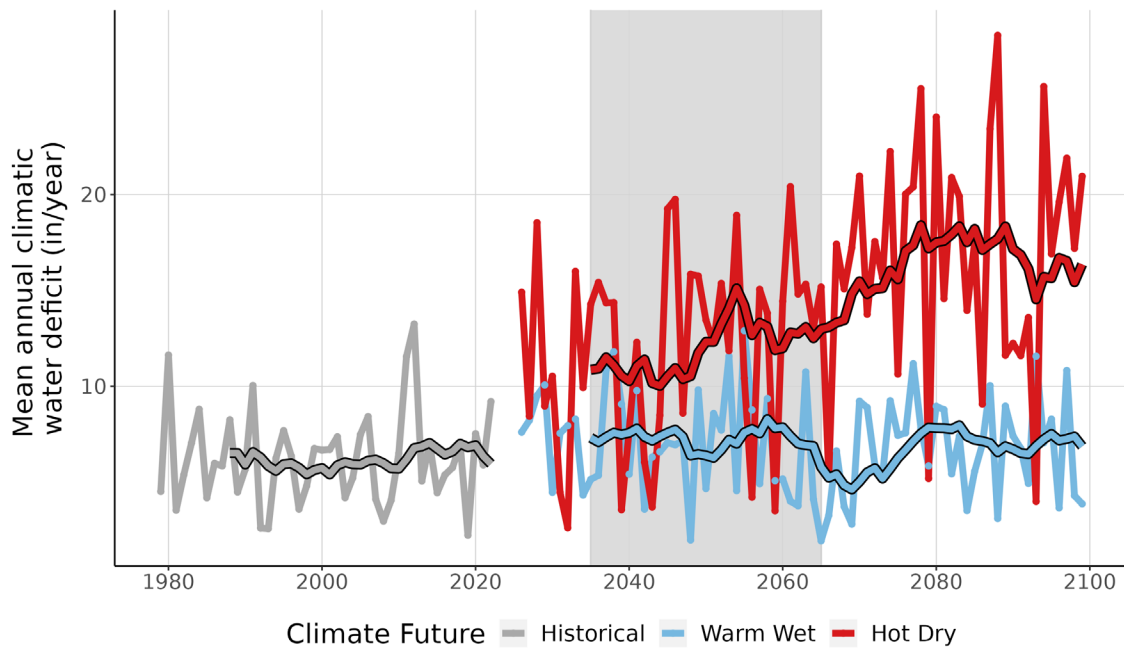
Figure 9. This line graph compares observed climatic water deficit at GWCA (inches/year) (1979-2022) with projected climatic water deficit for the two climate futures over the period 2023-2099. The historical observation data is shown in gray, the Warm Wet climate future in blue, and the Hot Dry climate future in red. The smooth line running through each projection is the 10-year running average for historical observations and future projections. Gray-shaded area represents the time period that was averaged (2035-2065) to summarize future projections for the year 2050.
