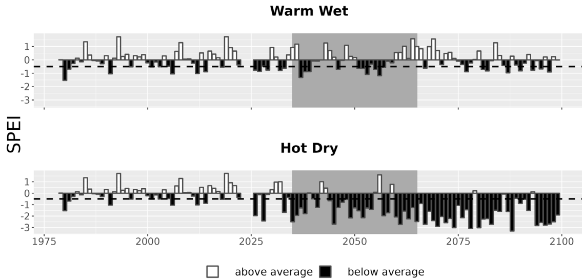
Figure 7. Drought metrics for GWCA. Drought index (SPEI; units = standard deviations from historical) timeseries for each climate future. Below-average SPEI (black bars) indicates dry conditions. The dotted line (SPEI = -0.5) indicates drought conditions.
