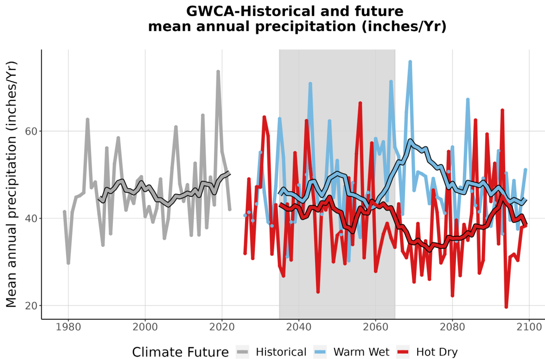
Figure 4. This graph compares observed average annual precipitation at GWCA (inches/year) (1979-2022) with projected average annual precipitation for the two climate futures over the period 2023-2099. The historically observed data is shown in gray, the Warm Wet climate future in blue, and the Hot Dry climate future in red. The smooth line running through each projection is the 10-year running average for historical observations and future projections. The gray-shaded area represents the time period that was averaged (2035-2065) to summarize future projections for the year 2050 (Appendix 1).
