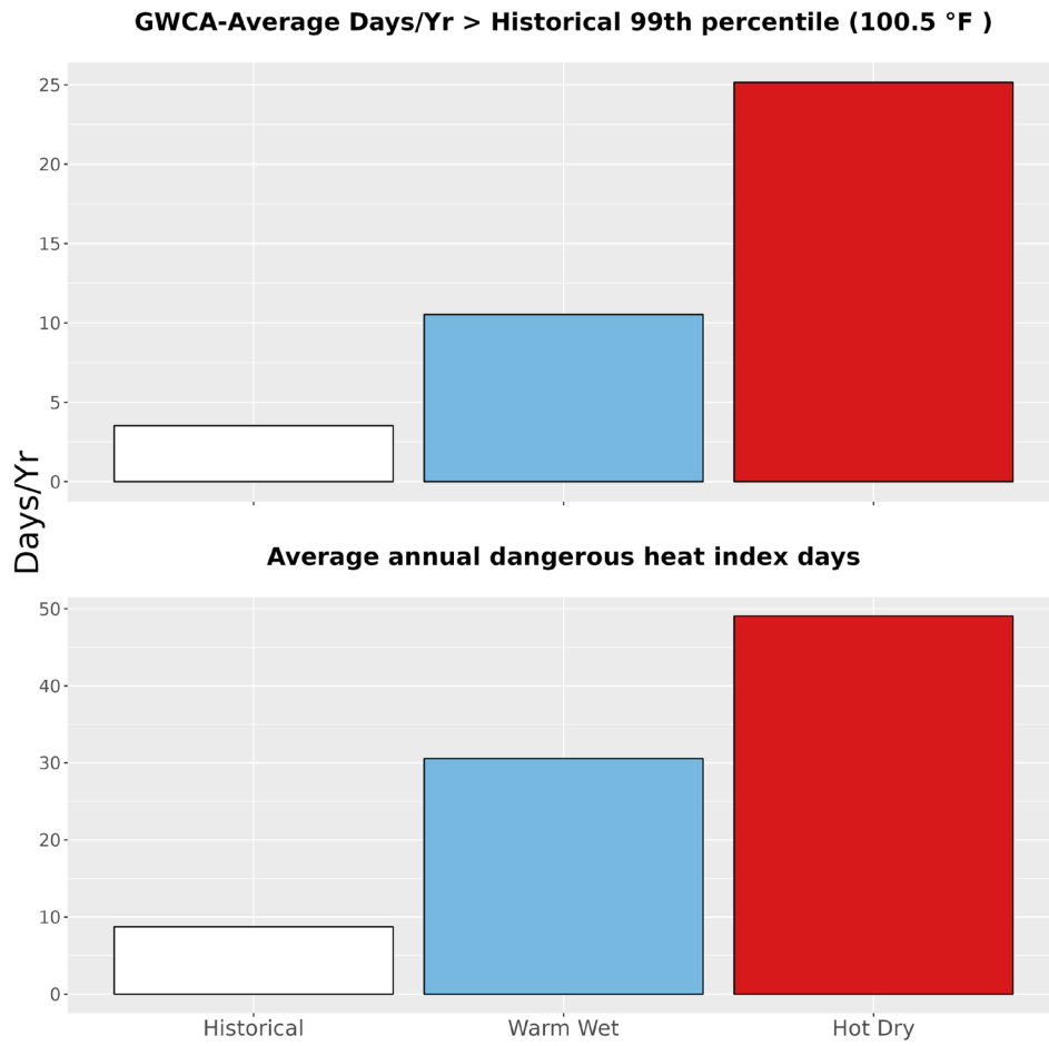
Figure 5. The upper bar graph represents the average number of days annually with temperatures greater than the historical 99th percentile (100.5 °F) historically (1979-2012) and for the two climate futures (2050). The bottom bar graph represents the average annual number of dangerous heat index days historically and for the two climate futures. Dangerous heat index days are days that exceed 105 °F.
