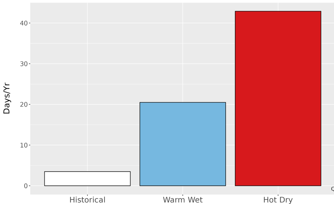
Figure 5. Metrics of extreme temperature at GRTE. The bar graph represents the average number of days annually with temperatures greater than the historical 99th percentile (84.8 °F) historically (1979-2012) and for the two climate futures (2050).
