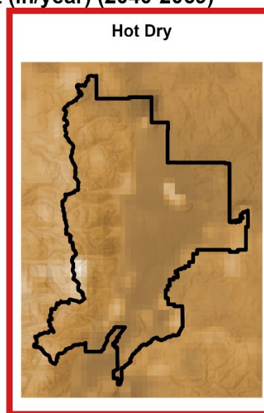
Figure A3. (Top) Map showing average annual climatic water deficit for the historical period (inches/year) and (bottom) change in average annual climatic water deficit for the two climate futures. Legends are located below each set of maps as a continuous color gradient. Gridded data is extracted from 30-year summary GIS layers for CONUS water balance model (Tercek et al 2021, 2023). ( http://screenedcleanedsummaries.s3-website-us-west-2.amazonaws.com/ ) accessed on 6/3/2024.
