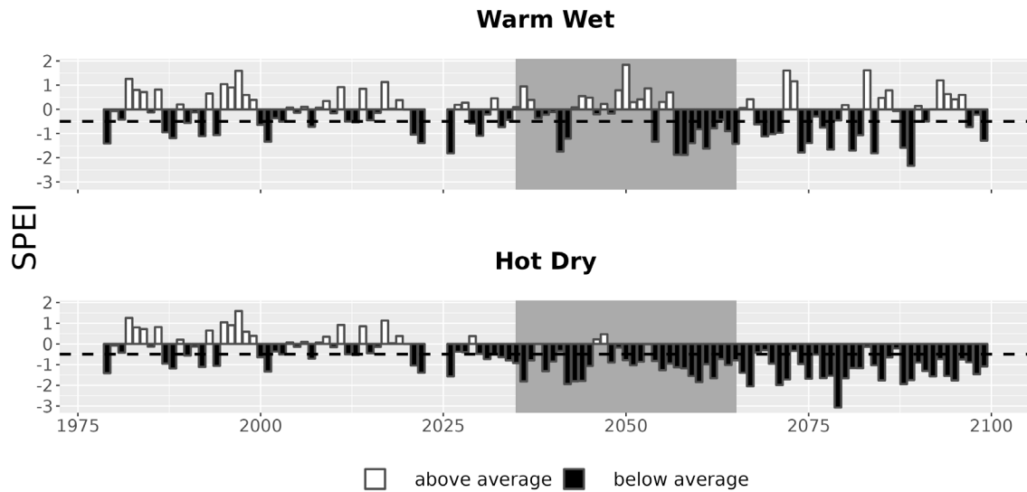
Figure 7. Drought metrics for GRTE. Drought index (SPEI; units = standard deviations from historical) timeseries for each climate future. Below-average SPEI (black bars) indicates dry conditions. The dotted line (SPEI = -0.5) indicates drought conditions.
