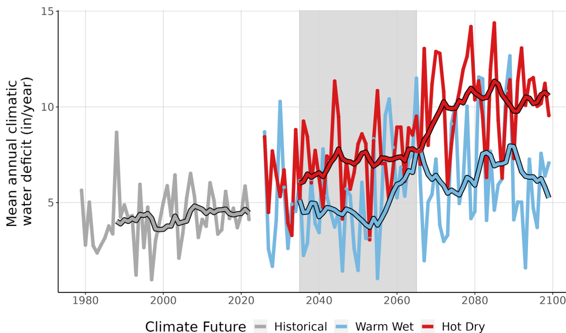
Figure 9. This line graph compares observed climatic water deficit at GRTE (inches/year) (1979-2022) with projected climatic water deficit for the two climate futures over the period 2023-2099. The historical observation data is shown in gray, the Warm Wet climate future in blue, and the Hot Dry climate future in red. The smooth line running through each projection is the 10-year running average for historical observations and future projections. Gray-shaded area represents the time period that was averaged (2035-2065) to summarize future projections for the year 2050.
