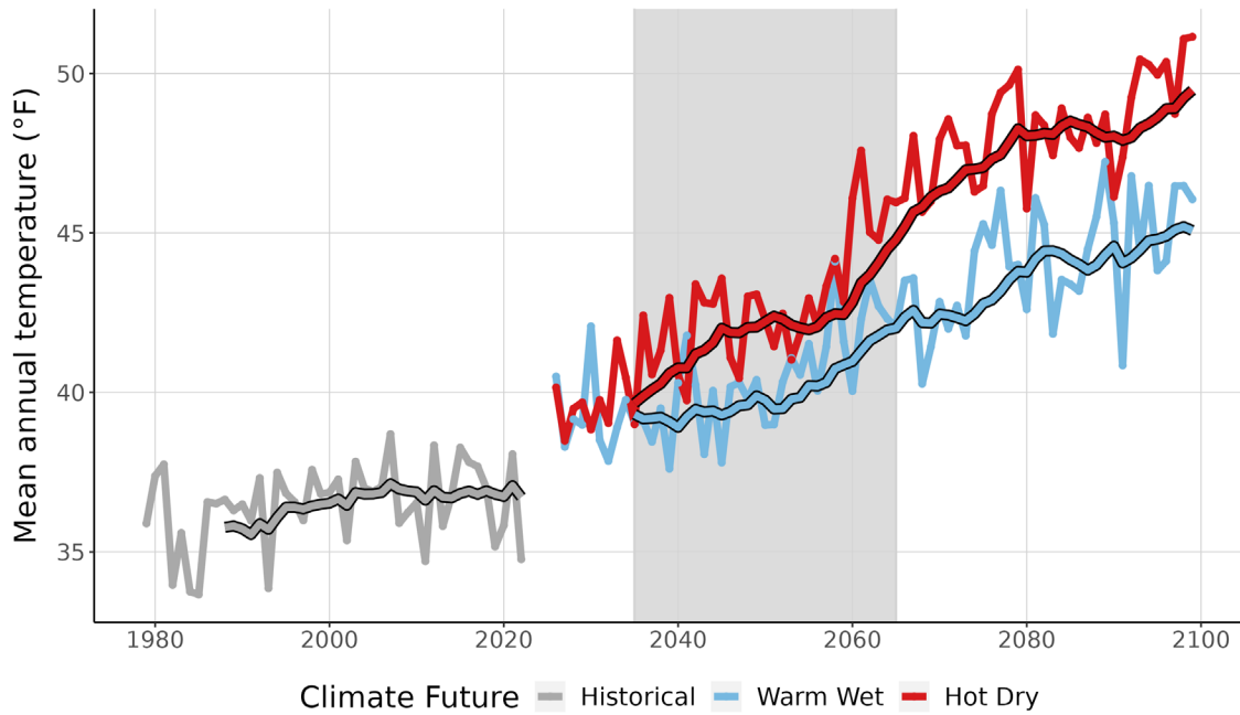
Figure 3. This graph compares observed average annual temperature at GRTE (°F) (1979-2022) with projected average annual temperature for the two climate futures over the period 2023-2099. The historically observed data is shown in gray, the Warm Wet climate future in blue, and the Hot Dry climate future in red. The smooth line running through each projection is the 10-year running average for historical observations and future projections. Gray-shaded area represents the time period that was averaged (2035-2065) to summarize future projections for the year 2050 (Appendix 1).
