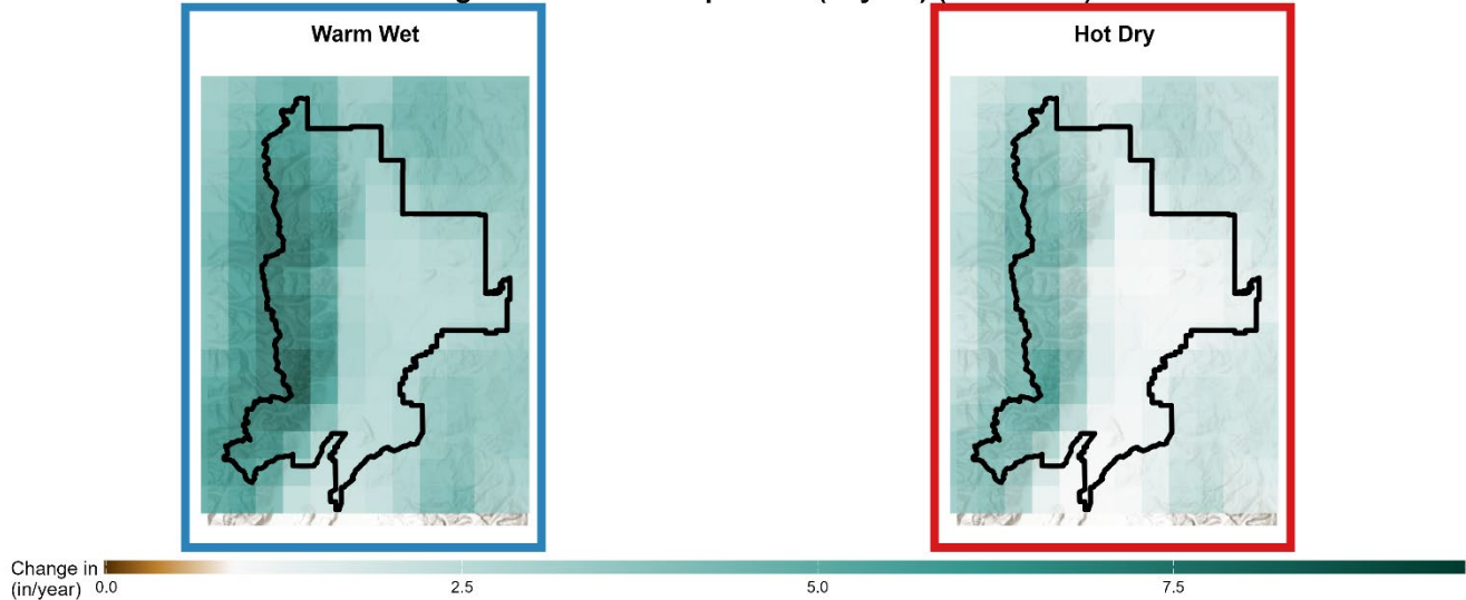
Figure A2. (Top) Map showing average annual precipitation for the historical period (inches/year) and (bottom) change in average annual precipitation for the two climate futures. Legends are located below each set of maps as a continuous color gradient. Gridded data is extracted from Hegewisch, K.C. and J.T. Abatzoglou, 'Climate Mapper' web tool. Climate Toolbox ( https://climatetoolbox.org/ ) accessed on 6/3/2024.
