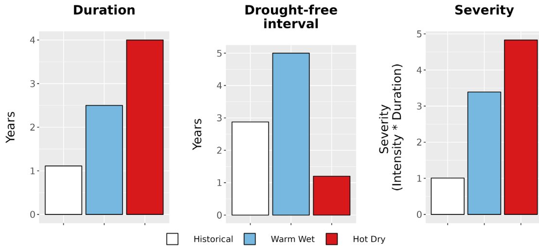
Figure 8. Drought metrics for GRTE. (Left) Average drought duration (years) historically (1979-2012) and under each climate future. (Middle) Average drought return interval (years), indicating the expected amount of time between periods of drought, historically and under each climate future. (Right) Average drought severity, a measure of drought intensity multiplied by duration, historically and under each climate future.
