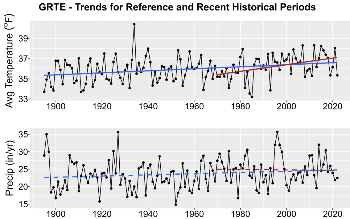
Figure 1. Historical trends in annual average temperature (upper plot) and annual total precipitation (lower plot) for GRTE from 1895-2022. Black points show yearly values while blue lines are linear regressions for the entire period record and red lines for 1970-2022 trends. Solid lines are significant trends (i.e., p < 0.05 ); dashed lines are not statistically significant.
