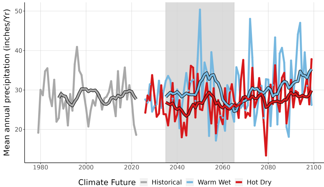
Figure 4. This graph compares observed average annual precipitation at GRTE (inches/year) (1979-2022) with projected average annual precipitation for the two climate futures over the period 2023-2099. The historically observed data is shown in gray, the Warm Wet climate future in blue, and the Hot Dry climate future in red. The smooth line running through each projection is the 10-year running average for historical observations and future projections. The gray-shaded area represents the time period that was averaged (2035-2065) to summarize future projections for the year 2050 (Appendix 1).
