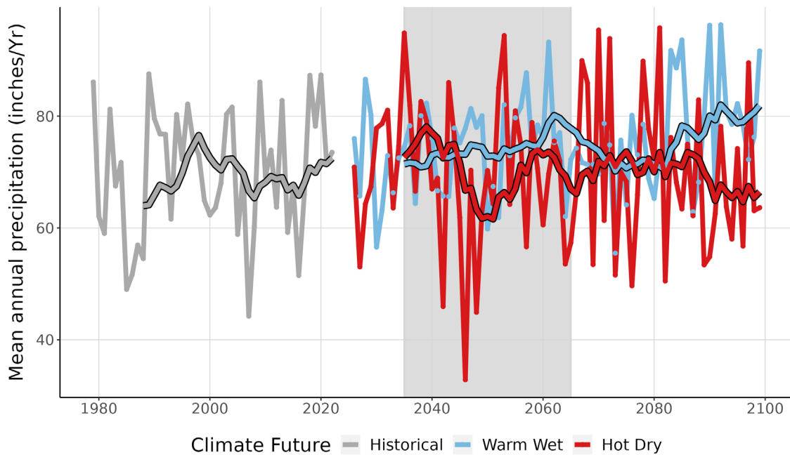
Figure 4. This graph compares observed average annual precipitation at GRSM (inches/year) (1979-2022) with projected average annual precipitation for the two climate futures over the period 2023-2099. The historically observed data is shown in gray, the Warm Wet climate future in blue, and the Hot Dry climate future in red. The smooth line running through each projection is the 10-year running average for historical observations and future projections. The gray-shaded area represents the time period that was averaged (2035-2065) to summarize future projections for the year 2050 (Appendix 1).
