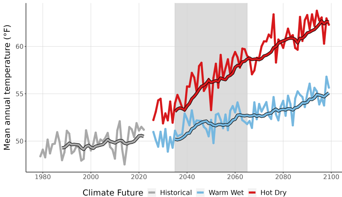
Figure 3. This graph compares observed average annual temperature at GRSM (°F) (1979-2022) with projected average annual temperature for the two climate futures over the period 2023-2099. The historically observed data is shown in gray, the Warm Wet climate future in blue, and the Hot Dry climate future in red. The smooth line running through each projection is the 10-year running average for historical observations and future projections. Gray-shaded area represents the time period that was averaged (2035-2065) to summarize future projections for the year 2050 (Appendix 1).
