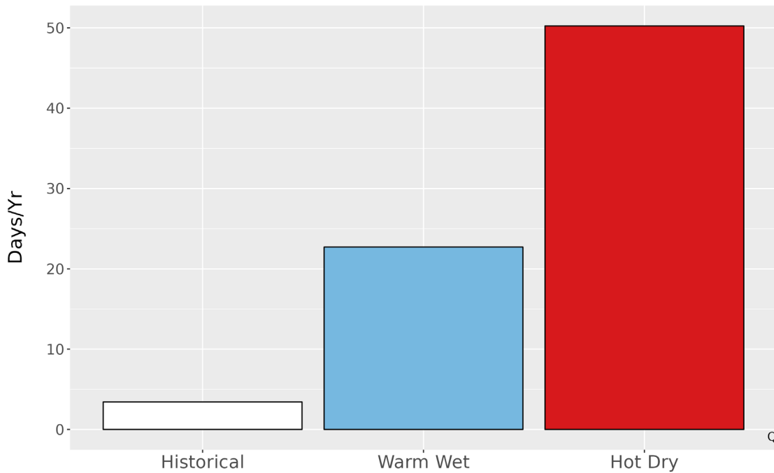
Figure 5. Metrics of extreme temperature at GRSM. The bar graph represents the average number of days annually with temperatures greater than the historical 99th percentile (83.4 °F) historically (1979-2012) and for the two climate futures (2050).
