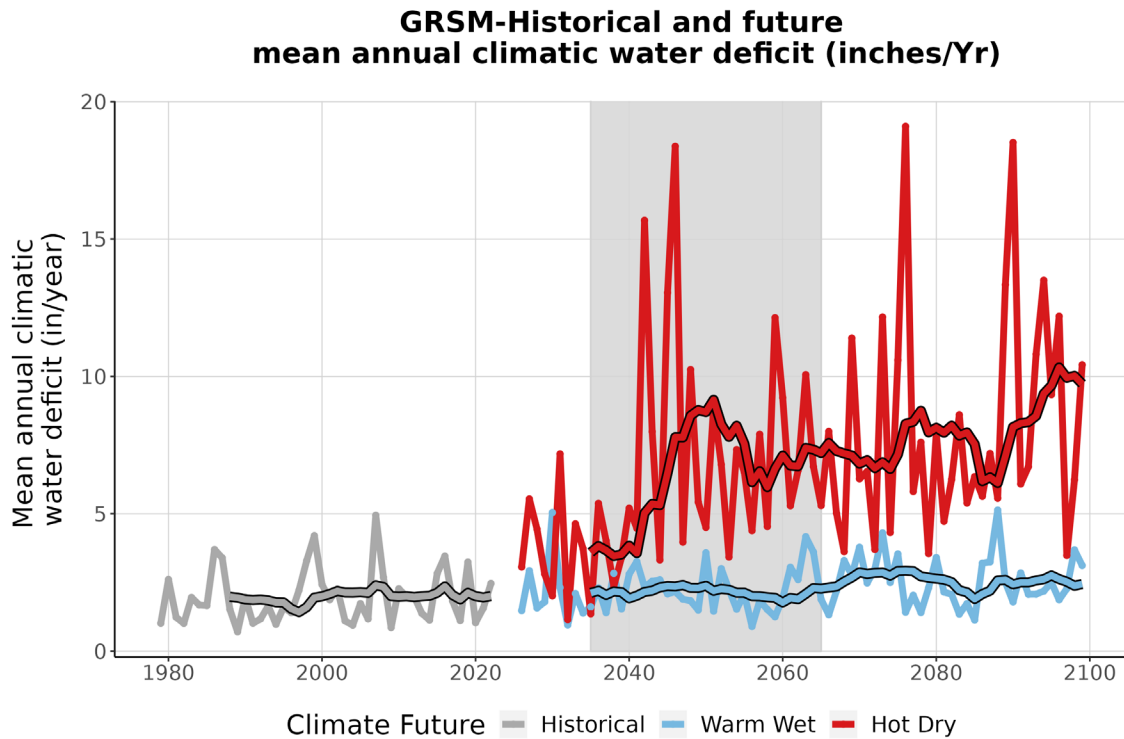
Figure 9. This line graph compares observed climatic water deficit at GRSM (inches/year) (1979-2022) with projected climatic water deficit for the two climate futures over the period 2023-2099. The historical observation data is shown in gray, the Warm Wet climate future in blue, and the Hot Dry climate future in red. The smooth line running through each projection is the 10-year running average for historical observations and future projections. Gray-shaded area represents the time period that was averaged (2035-2065) to summarize future projections for the year 2050.
