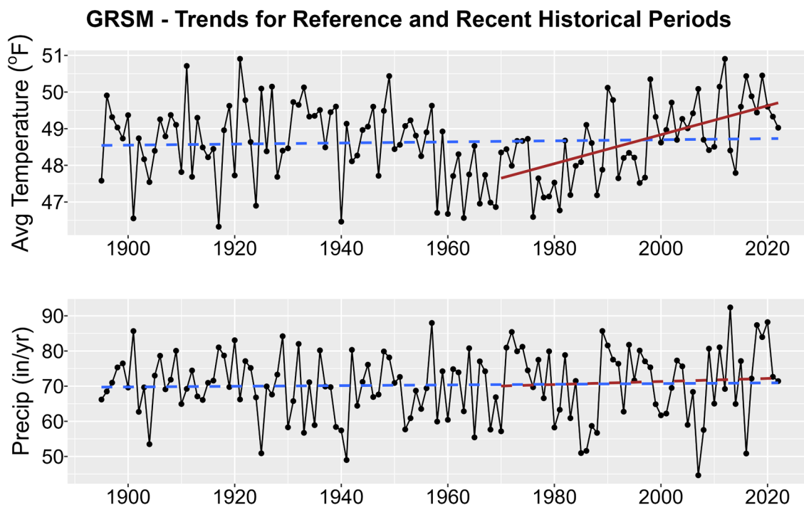
Figure 1. Historical trends in annual average temperature (upper plot) and annual total precipitation (lower plot) for GRSM from 1895-2022. Black points show yearly values while blue lines are linear regressions for the entire period record and red lines for 1970-2022 trends. Solid lines are significant trends (i.e., p < 0.05 ); dashed lines are not statistically significant.
