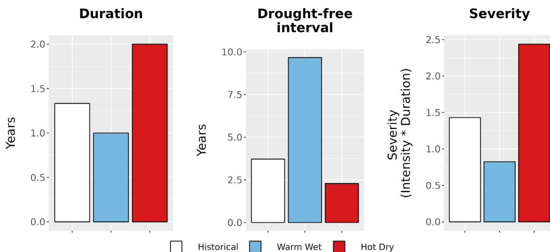
Figure 8. Drought metrics for GRSM. (Left) Average drought duration (years) historically (1979-2012) and under each climate future. (Middle) Average drought return interval (years), indicating the expected amount of time between periods of drought, historically and under each climate future. (Right) Average drought severity, a measure of drought intensity multiplied by duration, historically and under each climate future.
