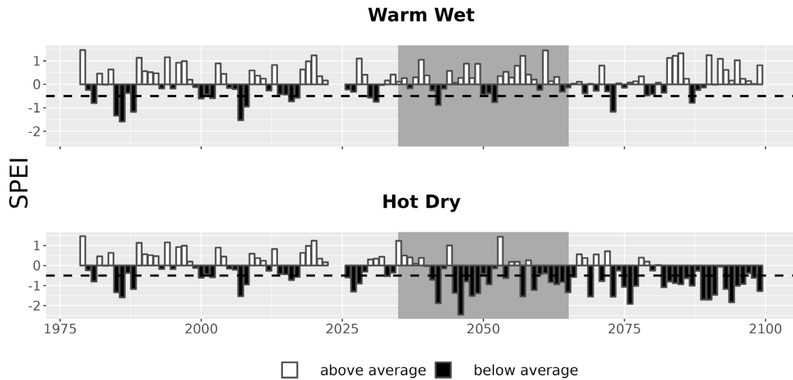
Figure 7. Drought metrics for GRSM. Drought index (SPEI; units = standard deviations from historical) timeseries for each climate future. Below-average SPEI (black bars) indicates dry conditions. The dotted line (SPEI = -0.5) indicates drought conditions.
