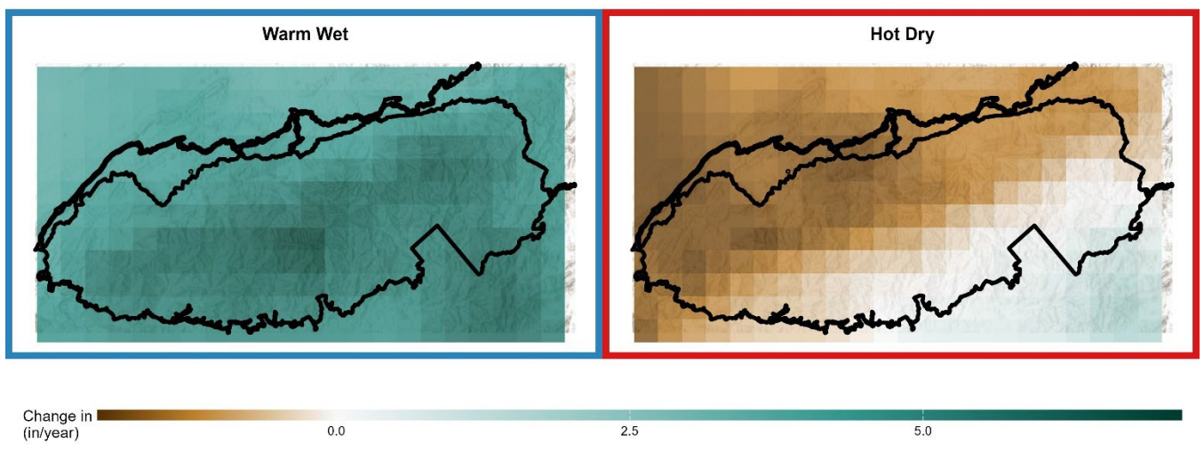
Figure A2. (Top) Map showing average annual precipitation for the historical period (inches/year) and (bottom) change in average annual precipitation for the two climate futures. Legends are located below each set of maps as a continuous color gradient. Gridded data is extracted from Hegewisch, K.C. and J.T. Abatzoglou, 'Climate Mapper' web tool. Climate Toolbox ( https://climatetoolbox.org/ ) accessed on 6/3/2024.
