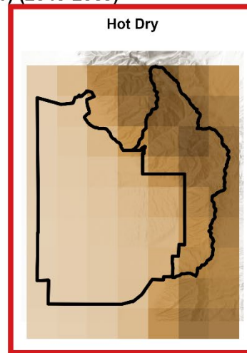
Figure A2. (Top) Map showing average annual precipitation for the historical period (inches/year) and (bottom) change in average annual precipitation for the two climate futures. Legends are located below each set of maps as a continuous color gradient. Gridded data is extracted from Hegewisch, K.C. and J.T. Abatzoglou, 'Climate Mapper' web tool. Climate Toolbox ( https://climatetoolbox.org/ ) accessed on 6/3/2024.
