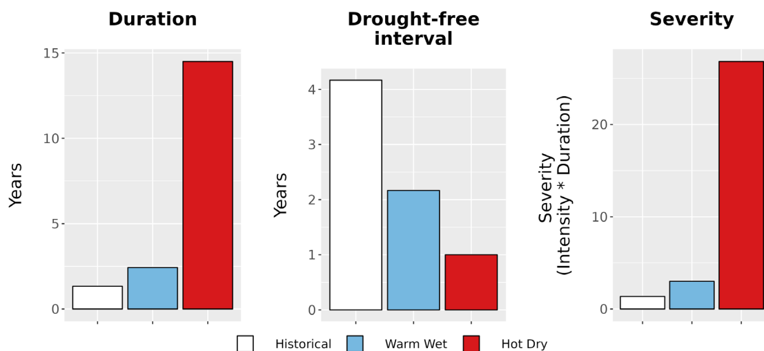
Figure 8. Drought metrics for GRSA. (Left) Average drought duration (years) historically (1979-2012) and under each climate future. (Middle) Average drought return interval (years), indicating the expected amount of time between periods of drought, historically and under each climate future. (Right) Average drought severity, a measure of drought intensity multiplied by duration, historically and under each climate future.
