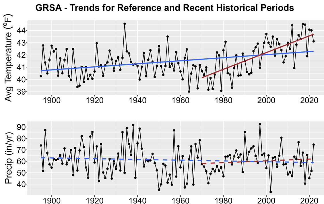
Figure 1. Historical trends in annual average temperature (upper plot) and annual total precipitation (lower plot) for GRSA from 1895-2022. Black points show yearly values while blue lines are linear regressions for the entire period record and red lines for 1970-2022 trends. Solid lines are significant trends (i.e., p < 0.05 ); dashed lines are not statistically significant.
