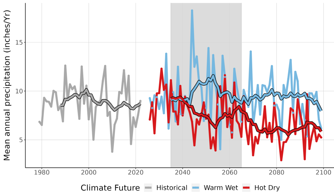
Figure 4. This graph compares observed average annual precipitation at GRSA (inches/year) (1979-2022) with projected average annual precipitation for the two climate futures over the period 2023-2099. The historically observed data is shown in gray, the Warm Wet climate future in blue, and the Hot Dry climate future in red. The smooth line running through each projection is the 10-year running average for historical observations and future projections. The gray-shaded area represents the time period that was averaged (2035-2065) to summarize future projections for the year 2050 (Appendix 1).
