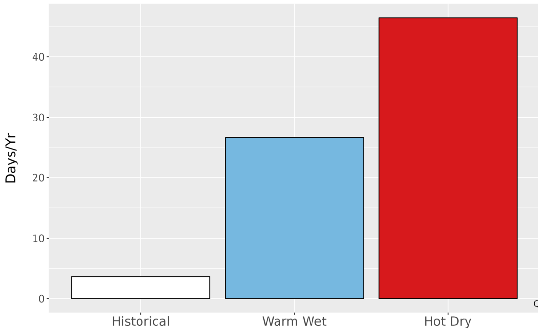
Figure 5. Metrics of extreme temperature at GRSA. The bar graph represents the average number of days annually with temperatures greater than the historical 99th percentile (87.3 °F) historically (1979-2012) and for the two climate futures (2050).
