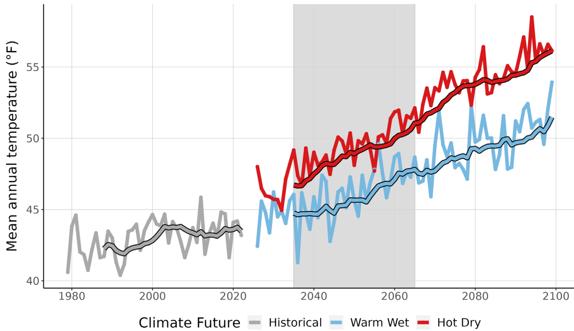
Figure 3. This graph compares observed average annual temperature at GRSA (°F) (1979-2022) with projected average annual temperature for the two climate futures over the period 2023-2099. The historically observed data is shown in gray, the Warm Wet climate future in blue, and the Hot Dry climate future in red. The smooth line running through each projection is the 10-year running average for historical observations and future projections. Gray-shaded area represents the time period that was averaged (2035-2065) to summarize future projections for the year 2050 (Appendix 1).
