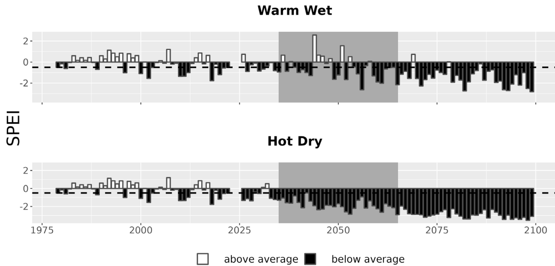
Figure 7. Drought metrics for GRSA. Drought index (SPEI; units = standard deviations from historical) timeseries for each climate future. Below-average SPEI (black bars) indicates dry conditions. The dotted line (SPEI = -0.5) indicates drought conditions.
