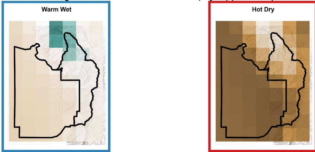
Figure A3. (Top) Map showing average annual climatic water deficit for the historical period (inches/year) and (bottom) change in average annual climatic water deficit for the two climate futures. Legends are located below each set of maps as a continuous color gradient. Gridded data is extracted from Hegewisch, K.C. and J.T. Abatzoglou, 'Climate Mapper' web tool. Climate Toolbox ( https://climatetoolbox.org/ ) accessed on 6/3/2024.
