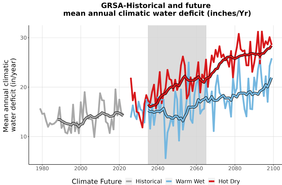
Figure 9. This line graph compares observed climatic water deficit at GRSA (inches/year) (1979-2022) with projected climatic water deficit for the two climate futures over the period 2023-2099. The historical observation data is shown in gray, the Warm Wet climate future in blue, and the Hot Dry climate future in red. The smooth line running through each projection is the 10-year running average for historical observations and future projections. Gray-shaded area represents the time period that was averaged (2035-2065) to summarize future projections for the year 2050.
