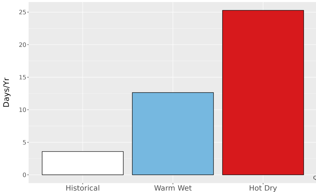
Figure 5. Metrics of extreme temperature at GRPO. The bar graph represents the average number of days annually with temperatures greater than the historical 99th percentile (85.2 °F) historically (1979-2012) and for the two climate futures (2050).
