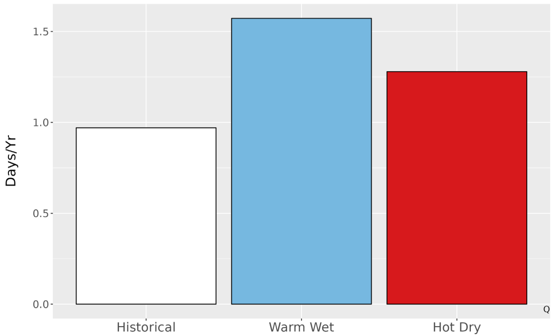
Figure 6. Average number of days annually with precipitation exceeding the 99th percentile (1.6 in.) of precipitation from the historical period 1979-2012 and for each climate future.
