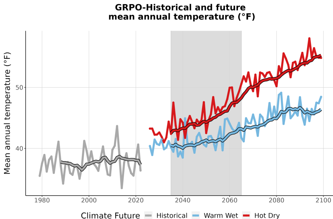
Figure 3. This graph compares observed average annual temperature at GRPO (°F) (1979-2022) with projected average annual temperature for the two climate futures over the period 2023-2099. The historically observed data
