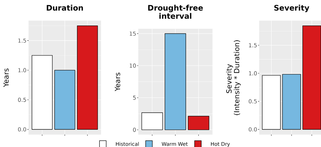
Figure 8. Drought metrics for GRPO. (Left) Average drought duration (years) historically (1979-2012) and under each climate future. (Middle) Average drought return interval (years), indicating the expected amount of time between periods of drought, historically and under each climate future. (Right) Average drought severity, a measure of drought intensity multiplied by duration, historically and under each climate future.
