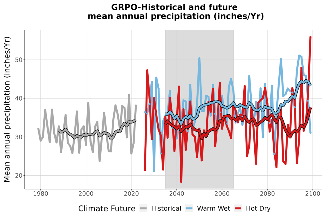
Figure 4. This graph compares observed average annual precipitation at GRPO (inches/year) (1979-2022) with projected average annual precipitation for the two climate futures over the period 2023-2099. The historically observed data is shown in gray, the Warm Wet climate future in blue, and the Hot Dry climate future in red. The smooth line running through each projection is the 10-year running average for historical observations and future projections. The gray-shaded area represents the time period that was averaged (2035-2065) to summarize future projections for the year 2050 (Appendix 1).
