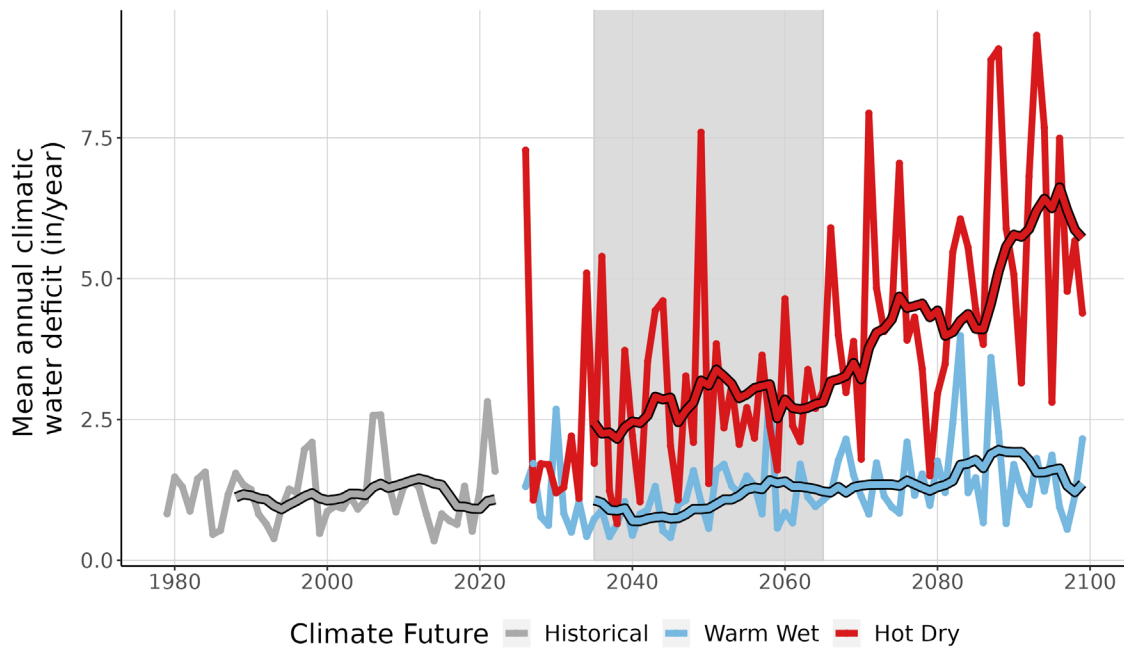
Figure 9. This line graph compares observed climatic water deficit at GRPO (inches/year) (1979-2022) with projected climatic water deficit for the two climate futures over the period 2023-2099. The historical observation data is shown in gray, the Warm Wet climate future in blue, and the Hot Dry climate future in red. The smooth line running through each projection is the 10-year running average for historical observations and future projections. Gray-shaded area represents the time period that was averaged (2035-2065) to summarize future projections for the year 2050.
