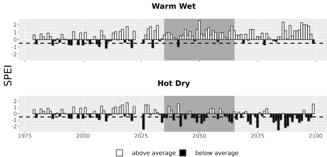
Figure 7. Drought metrics for GRPO. Drought index (SPEI; units = standard deviations from historical) timeseries for each climate future. Below-average SPEI (black bars) indicates dry conditions. The dotted line (SPEI = -0.5) indicates drought conditions.
