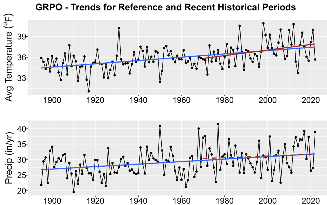
Figure 1. Historical trends in annual average temperature (upper plot) and annual total precipitation (lower plot) for GRPO from 1895-2022. Black points show yearly values while blue lines are linear regressions for the entire period record and red lines for 1970-2022 trends. Solid lines are significant trends (i.e., p < 0.05 ); dashed lines are not statistically significant.
