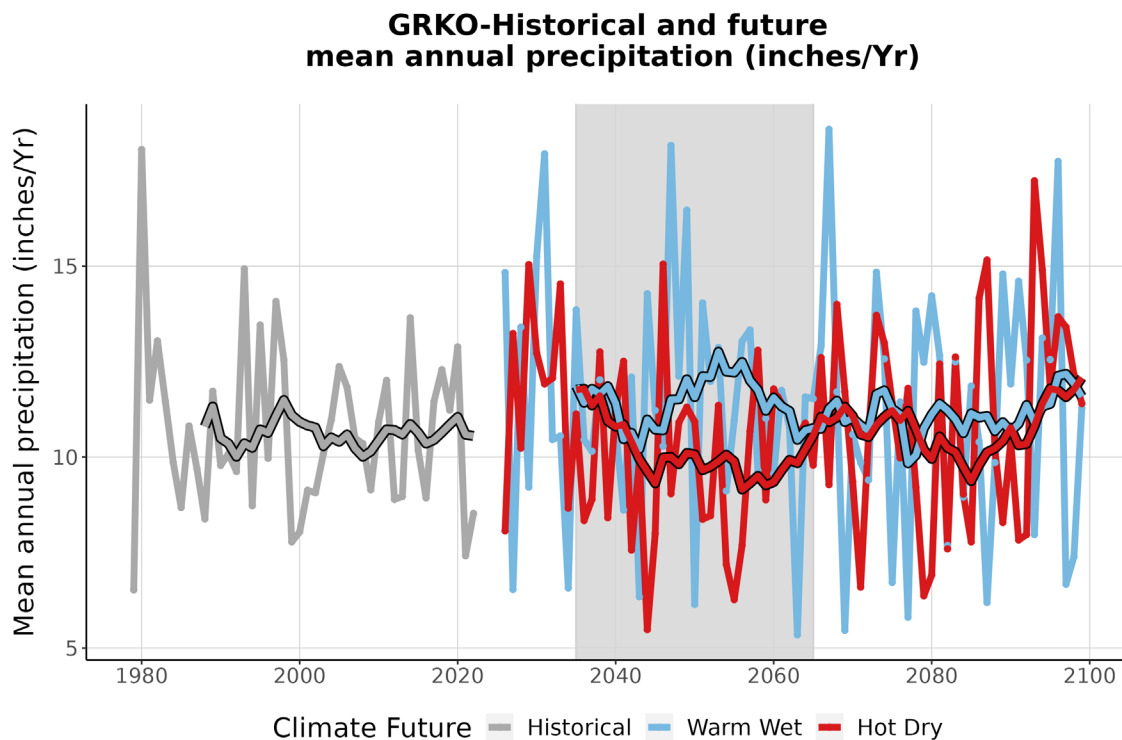
Figure 4. This graph compares observed average annual precipitation at GRKO (inches/year) (1979-2022) with projected average annual precipitation for the two climate futures over the period 2023-2099. The historically observed data is shown in gray, the Warm Wet climate future in blue, and the Hot Dry climate future in red. The smooth line running through each projection is the 10-year running average for historical observations and future projections. The gray-shaded area represents the time period that was averaged (2035-2065) to summarize future projections for the year 2050 (Appendix 1).
