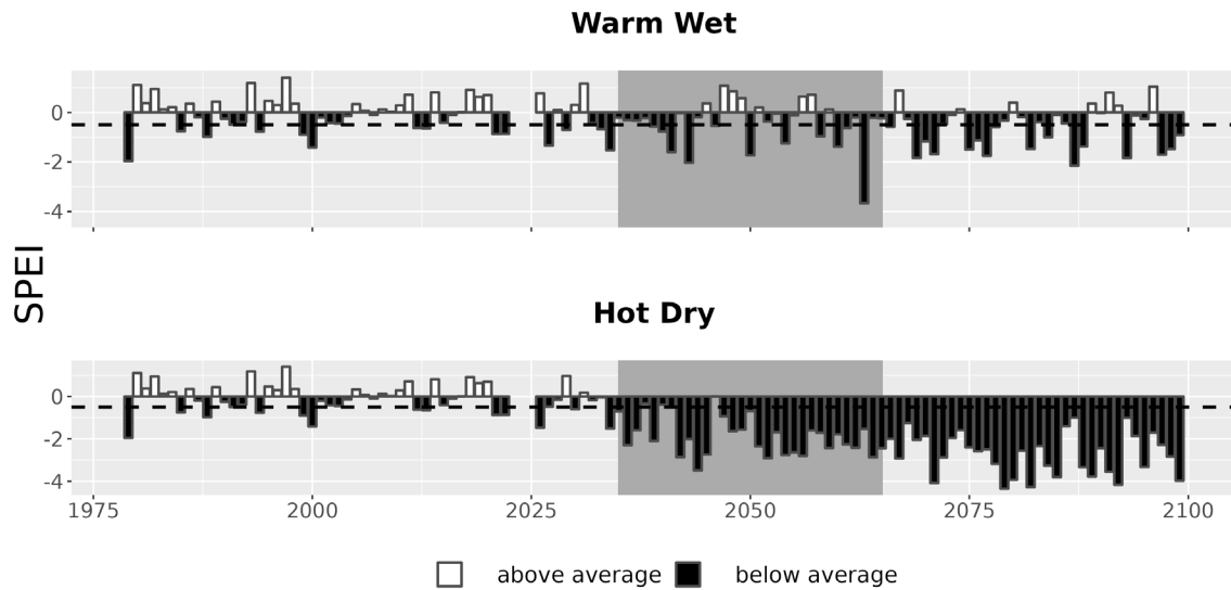
Figure 7. Drought metrics for GRKO. Drought index (SPEI; units = standard deviations from historical) timeseries for each climate future. Below-average SPEI (black bars) indicates dry conditions. The dotted line (SPEI = -0.5) indicates drought conditions.
