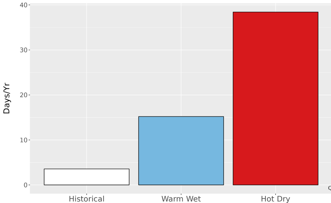
Figure 5. Metrics of extreme temperature at GRKO. The bar graph represents the average number of days annually with temperatures greater than the historical 99th percentile (90.9 °F) historically (1979-2012) and for the two climate futures (2050).
