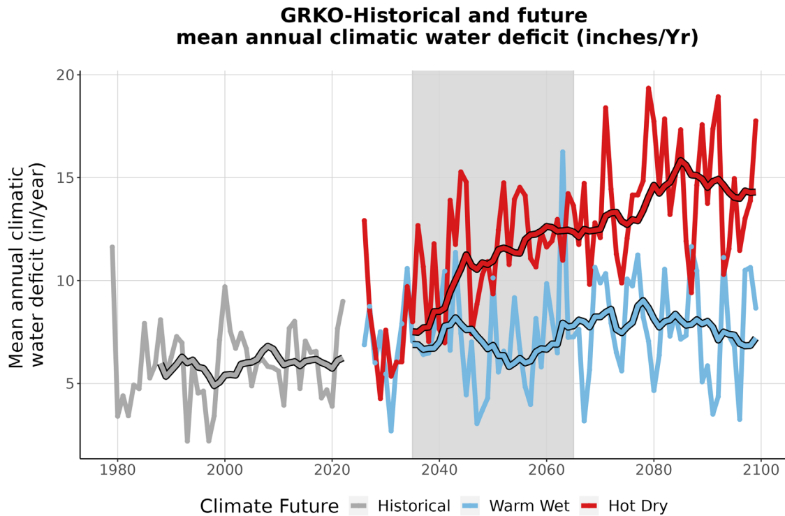
Figure 9. This line graph compares observed climatic water deficit at GRKO (inches/year) (1979-2022) with projected climatic water deficit for the two climate futures over the period 2023-2099. The historical observation data is shown in gray, the Warm Wet climate future in blue, and the Hot Dry climate future in red. The smooth line running through each projection is the 10-year running average for historical observations and future projections. Gray-shaded area represents the time period that was averaged (2035-2065) to summarize future projections for the year 2050.
