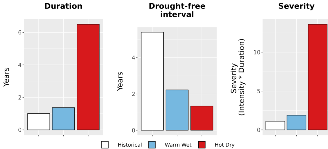
Figure 8. Drought metrics for GRKO. (Left) Average drought duration (years) historically (1979-2012) and under each climate future. (Middle) Average drought return interval (years), indicating the expected amount of time between periods of drought, historically and under each climate future. (Right) Average drought severity, a measure of drought intensity multiplied by duration, historically and under each climate future.
