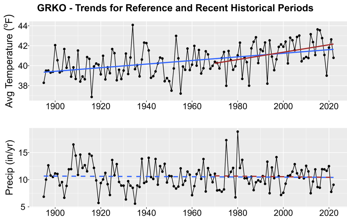
Figure 1. Historical trends in annual average temperature (upper plot) and annual total precipitation (lower plot) for GRKO from 1895-2022. Black points show yearly values while blue lines are linear regressions for the entire period record and red lines for 1970-2022 trends. Solid lines are significant trends (i.e., p < 0.05 ); dashed lines are not statistically significant.
