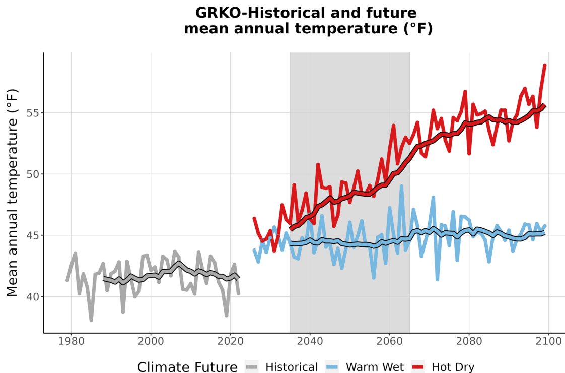
Figure 3. This graph compares observed average annual temperature at GRKO (°F) (1979-2022) with projected average annual temperature for the two climate futures over the period 2023-2099. The historically observed data
