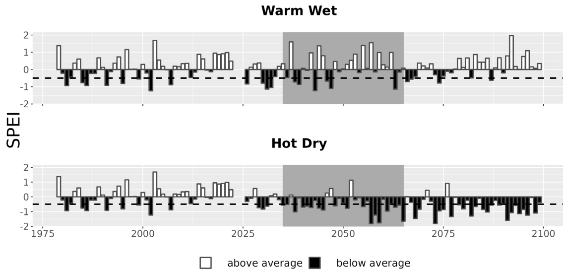
Figure 7. Drought metrics for GREE. Drought index (SPEI; units = standard deviations from historical) timeseries for each climate future. Below-average SPEI (black bars) indicates dry conditions. The dotted line (SPEI = -0.5) indicates drought conditions.
