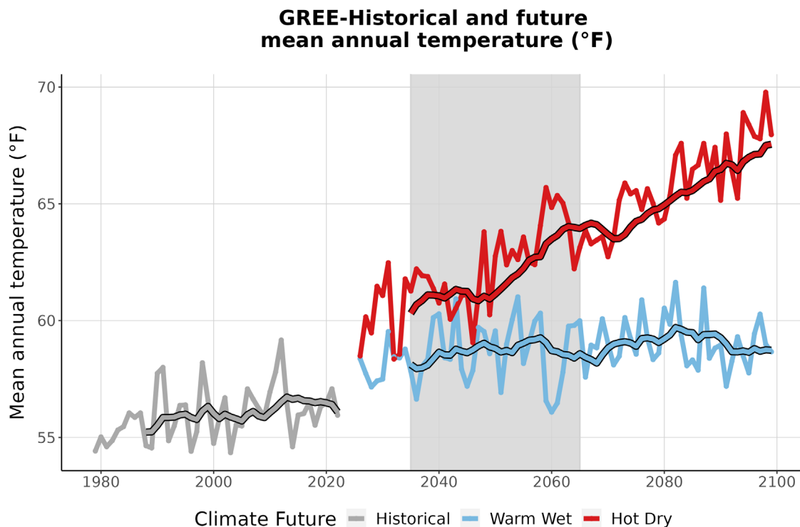
Figure 3. This graph compares observed average annual temperature at GREE (°F) (1979-2022) with projected average annual temperature for the two climate futures over the period 2023-2099. The historically observed data
