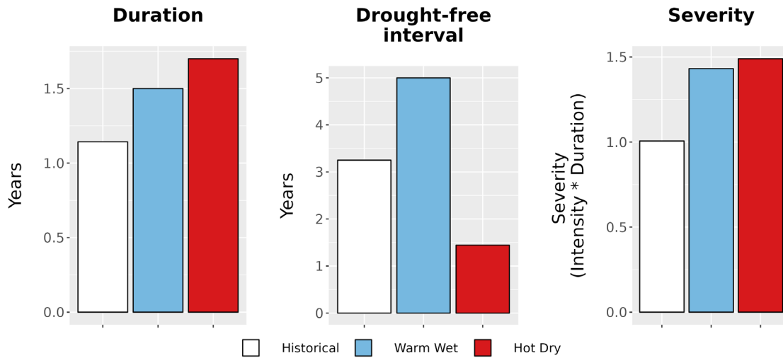
Figure 8. Drought metrics for GREE. (Left) Average drought duration (years) historically (1979-2012) and under each climate future. (Middle) Average drought return interval (years), indicating the expected amount of time between periods of drought, historically and under each climate future. (Right) Average drought severity, a measure of drought intensity multiplied by duration, historically and under each climate future.
