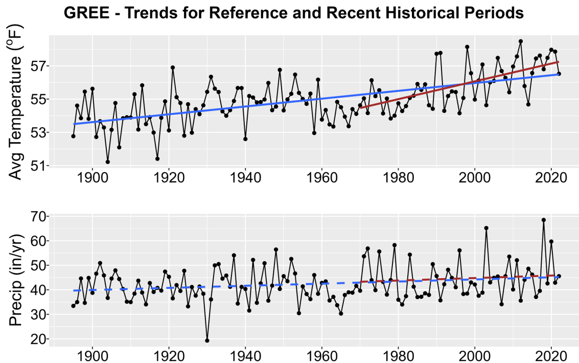
Figure 1. Historical trends in annual average temperature (upper plot) and annual total precipitation (lower plot) for GREE from 1895-2022. Black points show yearly values while blue lines are linear regressions for the entire period record and red lines for 1970-2022 trends. Solid lines are significant trends (i.e., p < 0.05 ); dashed lines are not statistically significant.
