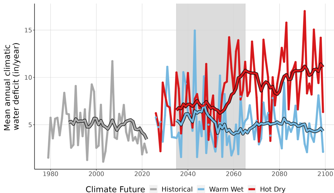
Figure 9. This line graph compares observed climatic water deficit at GREE (inches/year) (1979-2022) with projected climatic water deficit for the two climate futures over the period 2023-2099. The historical observation data is shown in gray, the Warm Wet climate future in blue, and the Hot Dry climate future in red. The smooth line running through each projection is the 10-year running average for historical observations and future projections. Gray-shaded area represents the time period that was averaged (2035-2065) to summarize future projections for the year 2050.
