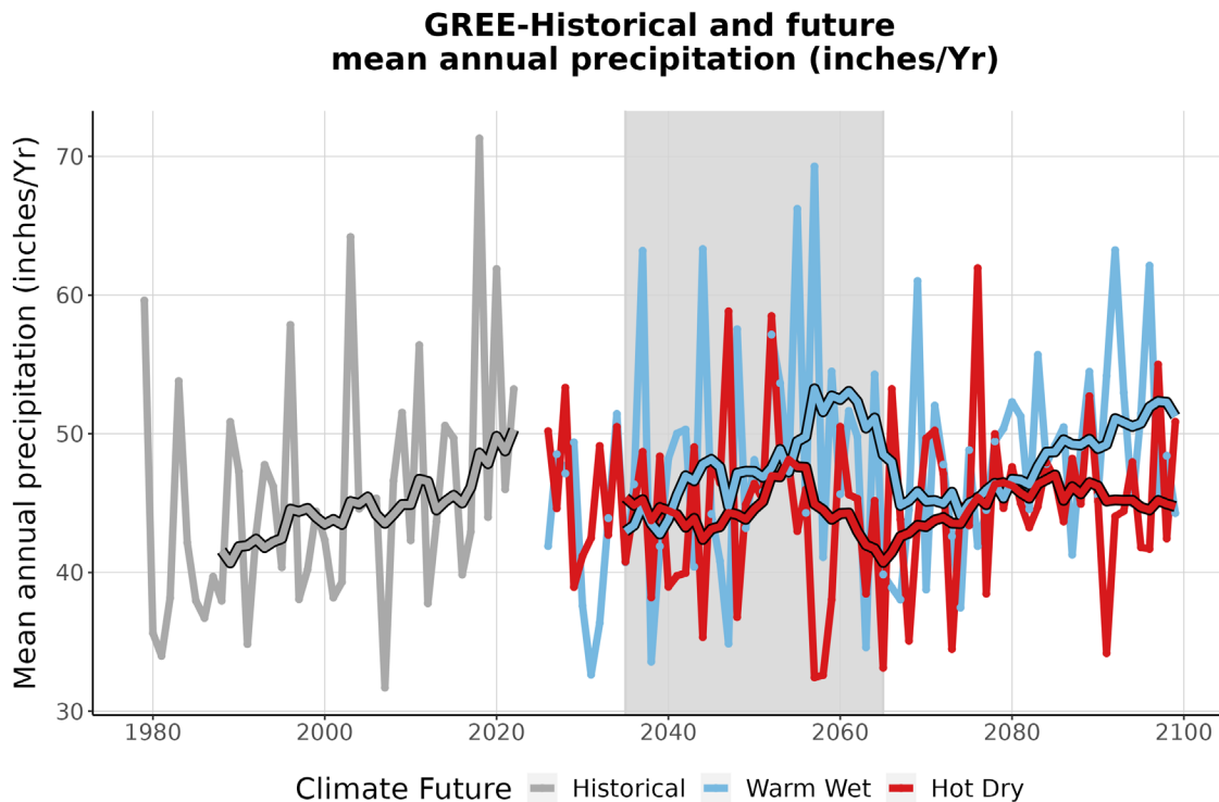
Figure 4. This graph compares observed average annual precipitation at GREE (inches/year) (1979-2022) with projected average annual precipitation for the two climate futures over the period 2023-2099. The historically observed data is shown in gray, the Warm Wet climate future in blue, and the Hot Dry climate future in red. The smooth line running through each projection is the 10-year running average for historical observations and future projections. The gray-shaded area represents the time period that was averaged (2035-2065) to summarize future projections for the year 2050 (Appendix 1).
