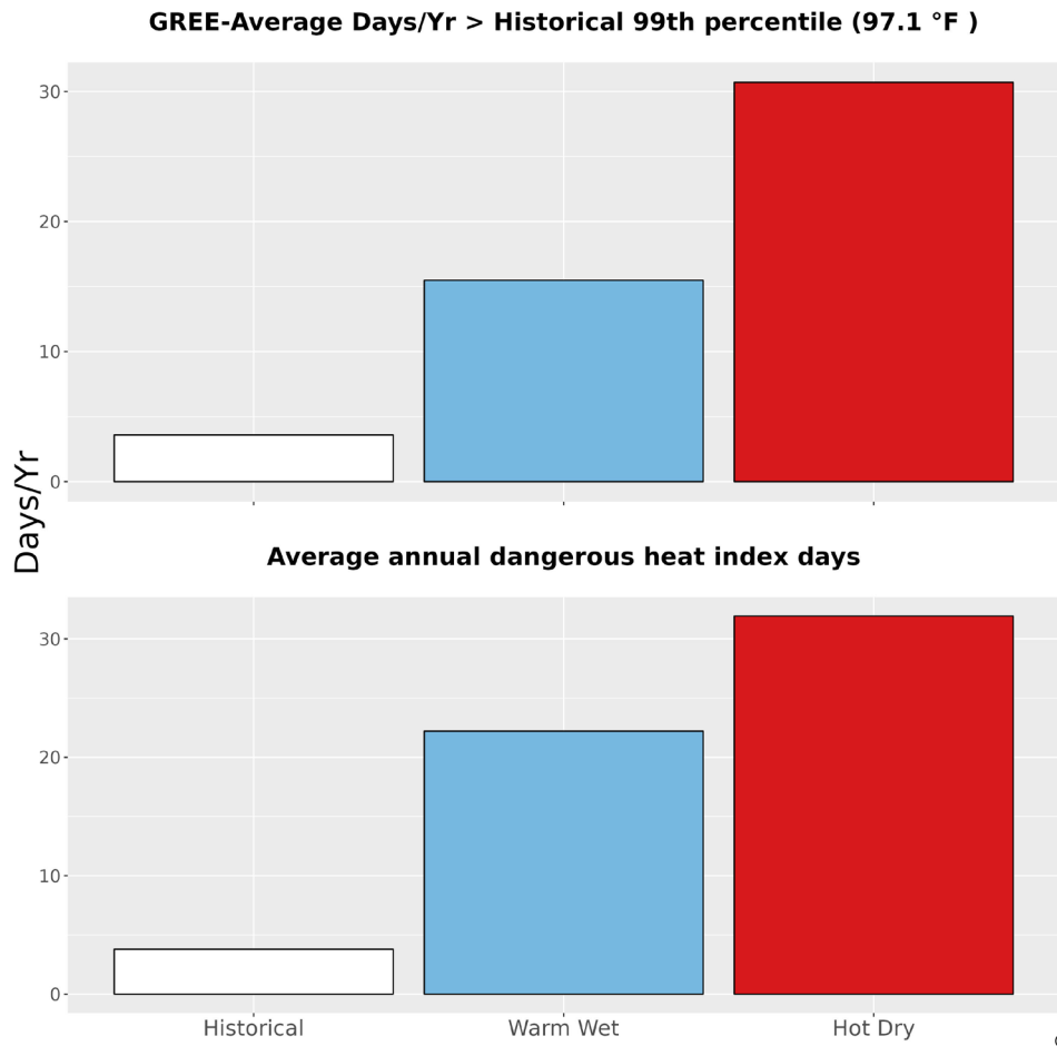
Figure 5. The upper bar graph represents the average number of days annually with temperatures greater than the historical 99th percentile (97.1 °F) historically (1979-2012) and for the two climate futures (2050). The bottom bar graph represents the average annual number of dangerous heat index days historically and for the two climate futures. Dangerous heat index days are days that exceed 105 °F.
