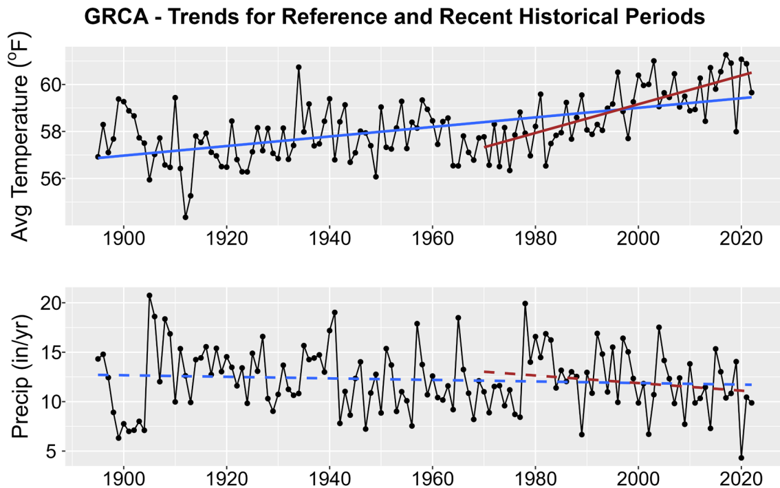
Figure 1. Historical trends in annual average temperature (upper plot) and annual total precipitation (lower plot) for GRCA from 1895-2022. Black points show yearly values while blue lines are linear regressions for the entire period record and red lines for 1970-2022 trends. Solid lines are significant trends (i.e., p < 0.05 ); dashed lines are not statistically significant.
