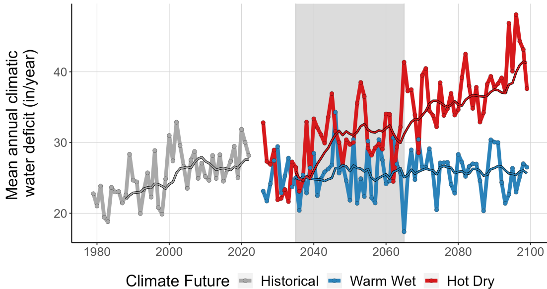
Figure 9. This line graph compares observed climatic water deficit at GRCA (inches/year) (1979-2022) with projected climatic water deficit for the two climate futures over the period 2023-2099. The historical observation data is shown in gray, the Warm Wet climate future in blue, and the Hot Dry climate future in red. The smooth line running through each projection is the 10-year running average for historical observations and future projections. Gray-shaded area represents the time period that was averaged (2035-2065) to summarize future projections for the year 2050.
