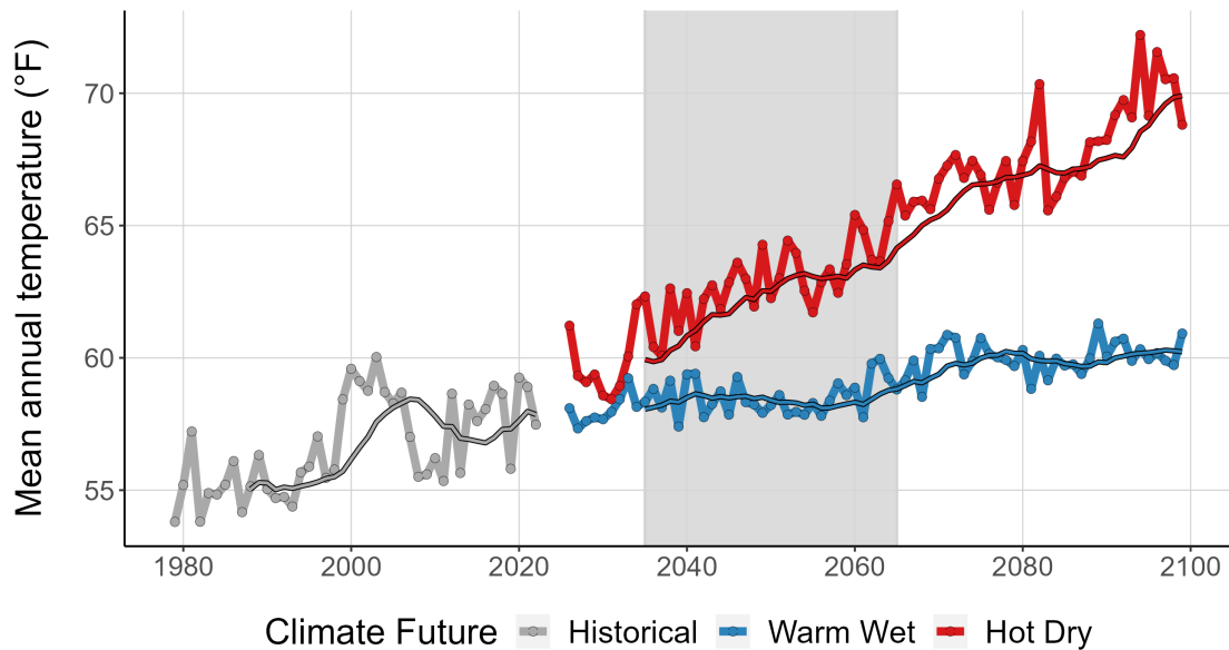
Figure 3. This graph compares observed average annual temperature at GRCA (°F) (1979-2022) with projected average annual temperature for the two climate futures over the period 2023-2099. The historically observed data is shown in gray, the Warm Wet climate future in blue, and the Hot Dry climate future in red. The smooth line running through each projection is the 10-year running average for historical observations and future projections. Gray-shaded area represents the time period that was averaged (2035-2065) to summarize future projections for the year 2050 (Appendix 1).
