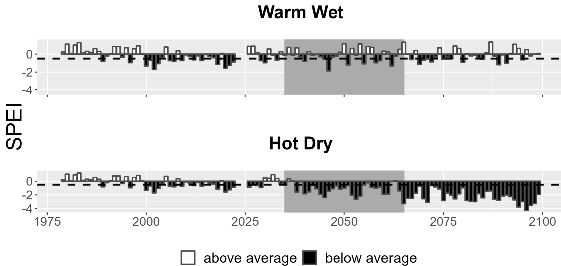
Figure 7. Drought metrics for GRCA. Drought index (SPEI; units = standard deviations from historical) timeseries for each climate future. Below-average SPEI (black bars) indicates dry conditions. The dotted line (SPEI = -0.5) indicates drought conditions.
