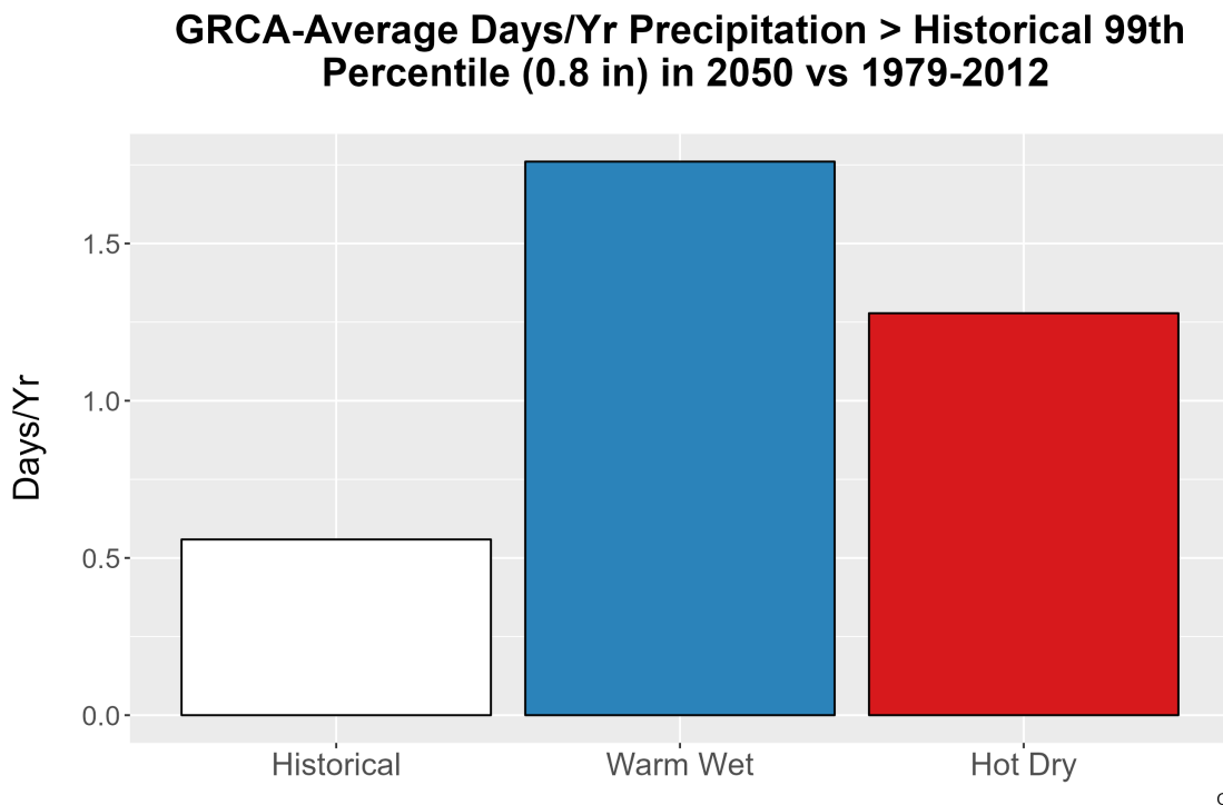
Figure 6. Average number of days annually with precipitation exceeding the 99th percentile (0.8 in.) of precipitation from the historical period 1979-2012 and for each climate future.
