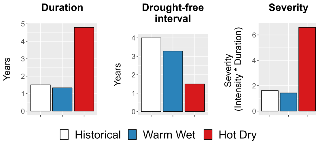
Figure 8. Drought metrics for GRCA. (Left) Average drought duration (years) historically (1979-2012) and under each climate future. (Middle) Average drought return interval (years), indicating the expected amount of time between periods of drought, historically and under each climate future. (Right) Average drought severity, a measure of drought intensity multiplied by duration, historically and under each climate future.
