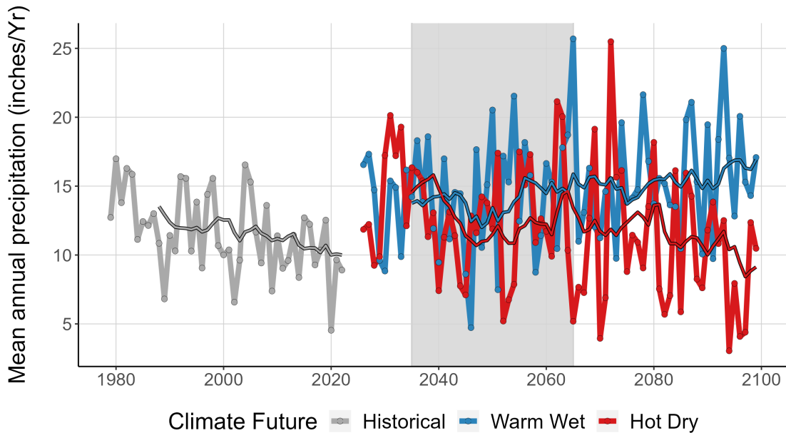
Figure 4. This graph compares observed average annual precipitation at GRCA (inches/year) (1979-2022) with projected average annual precipitation for the two climate futures over the period 2023-2099. The historically observed data is shown in gray, the Warm Wet climate future in blue, and the Hot Dry climate future in red. The smooth line running through each projection is the 10-year running average for historical observations and future projections. The gray-shaded area represents the time period that was averaged (2035-2065) to summarize future projections for the year 2050 (Appendix 1).
