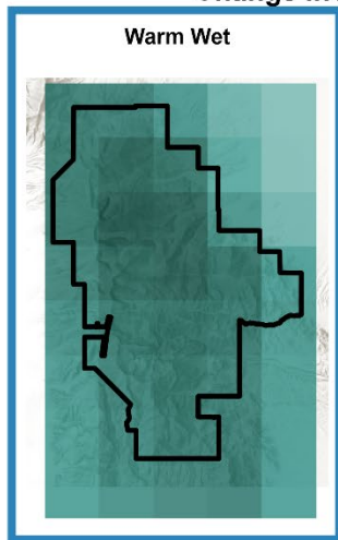
Figure A2. (Top) Map showing average annual precipitation for the historical period (inches/year) and (bottom) change in average annual precipitation for the two climate futures. Legends are located below each set of maps as a continuous color gradient. Gridded data is extracted from Hegewisch, K.C. and J.T. Abatzoglou, 'Climate Mapper' web tool. Climate Toolbox ( https://climatetoolbox.org/ ) accessed on 6/3/2024.
