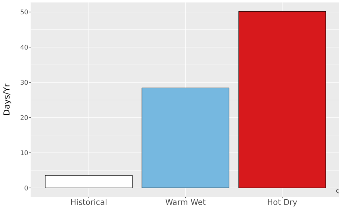
Figure 5. Metrics of extreme temperature at GRBA. The bar graph represents the average number of days annually with temperatures greater than the historical 99th percentile (80.3 °F) historically (1979-2012) and for the two climate futures (2050).
