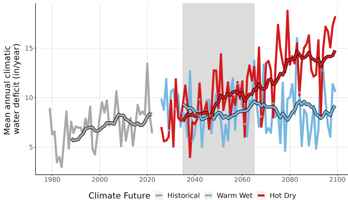
Figure 9. This line graph compares observed climatic water deficit at GRBA (inches/year) (1979-2022) with projected climatic water deficit for the two climate futures over the period 2023-2099. The historical observation data is shown in gray, the Warm Wet climate future in blue, and the Hot Dry climate future in red. The smooth line running through each projection is the 10-year running average for historical observations and future projections. Gray-shaded area represents the time period that was averaged (2035-2065) to summarize future projections for the year 2050.
