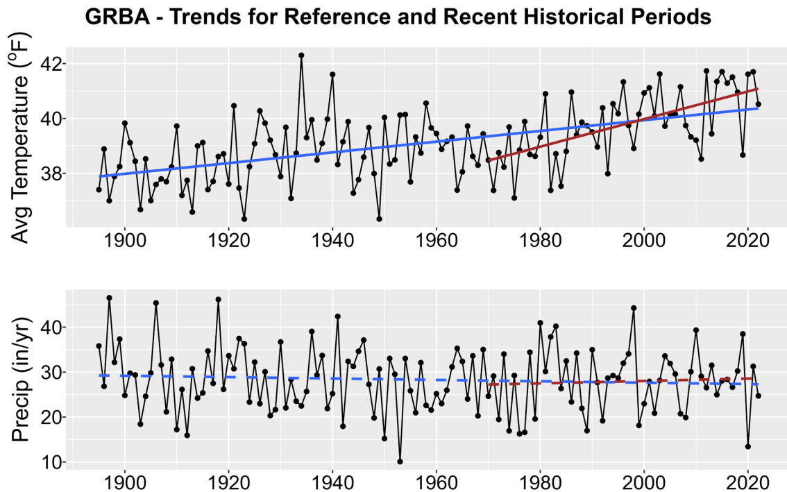
Figure 1. Historical trends in annual average temperature (upper plot) and annual total precipitation (lower plot) for GRBA from 1895-2022. Black points show yearly values while blue lines are linear regressions for the entire period record and red lines for 1970-2022 trends. Solid lines are significant trends (i.e., p < 0.05 ); dashed lines are not statistically significant.
