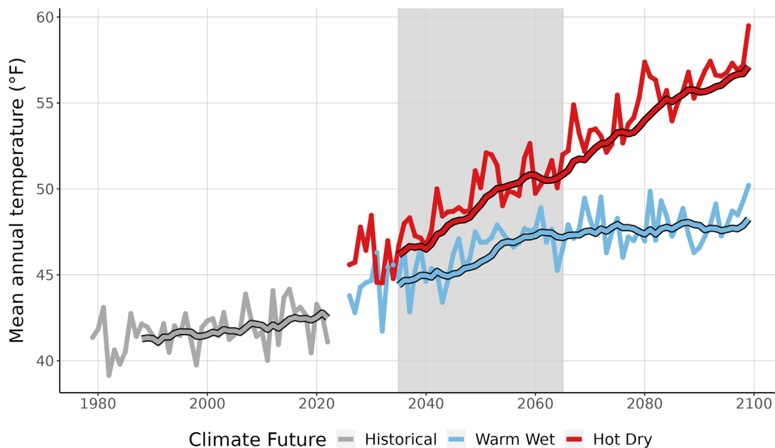
Figure 3. This graph compares observed average annual temperature at GRBA (°F) (1979-2022) with projected average annual temperature for the two climate futures over the period 2023-2099. The historically observed data is shown in gray, the Warm Wet climate future in blue, and the Hot Dry climate future in red. The smooth line running through each projection is the 10-year running average for historical observations and future projections. Gray-shaded area represents the time period that was averaged (2035-2065) to summarize future projections for the year 2050 (Appendix 1).
