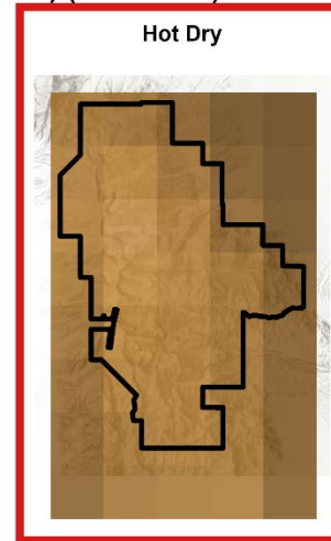
Figure A3. (Top) Map showing average annual climatic water deficit for the historical period (inches/year) and (bottom) change in average annual climatic water deficit for the two climate futures. Legends are located below each set of maps as a continuous color gradient. Gridded data is extracted from Hegewisch, K.C. and J.T. Abatzoglou, 'Climate Mapper' web tool. Climate Toolbox ( https://climatetoolbox.org/ ) accessed on 6/3/2024.
