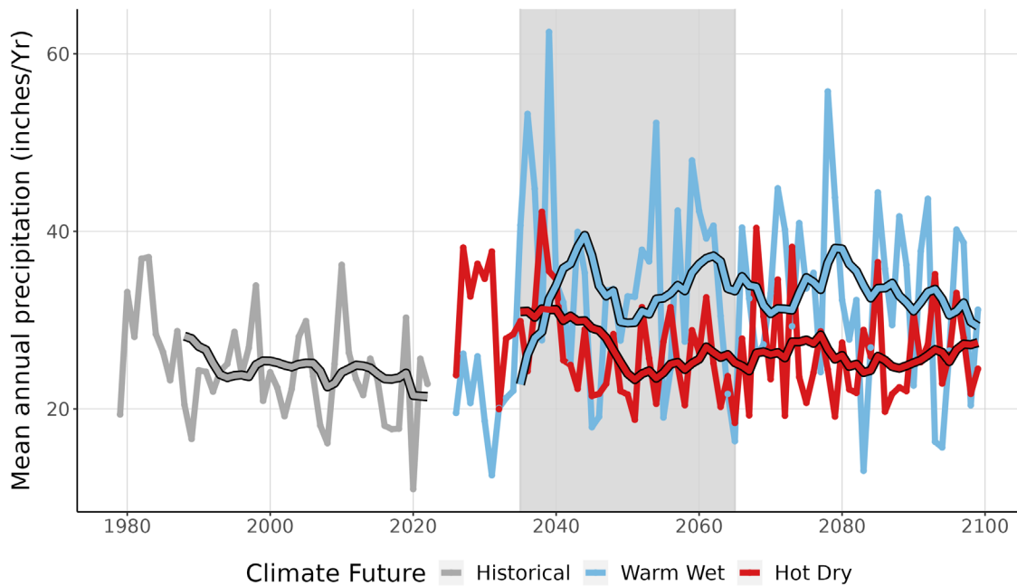
Figure 4. This graph compares observed average annual precipitation at GRBA (inches/year) (1979-2022) with projected average annual precipitation for the two climate futures over the period 2023-2099. The historically observed data is shown in gray, the Warm Wet climate future in blue, and the Hot Dry climate future in red. The smooth line running through each projection is the 10-year running average for historical observations and future projections. The gray-shaded area represents the time period that was averaged (2035-2065) to summarize future projections for the year 2050 (Appendix 1).
