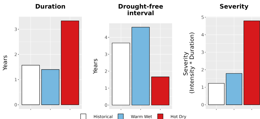
Figure 8. Drought metrics for GRBA. (Left) Average drought duration (years) historically (1979-2012) and under each climate future. (Middle) Average drought return interval (years), indicating the expected amount of time between periods of drought, historically and under each climate future. (Right) Average drought severity, a measure of drought intensity multiplied by duration, historically and under each climate future.
