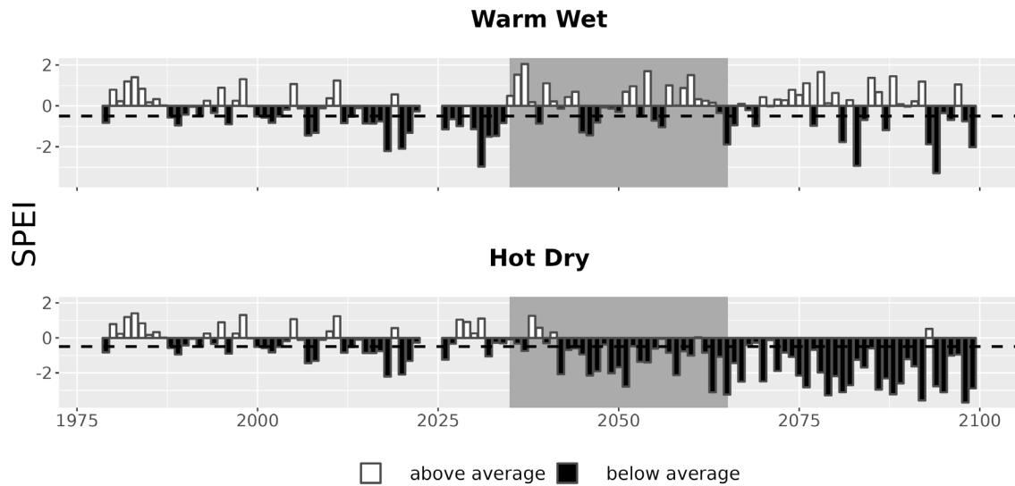
Figure 7. Drought metrics for GRBA. Drought index (SPEI; units = standard deviations from historical) timeseries for each climate future. Below-average SPEI (black bars) indicates dry conditions. The dotted line (SPEI = -0.5) indicates drought conditions.
