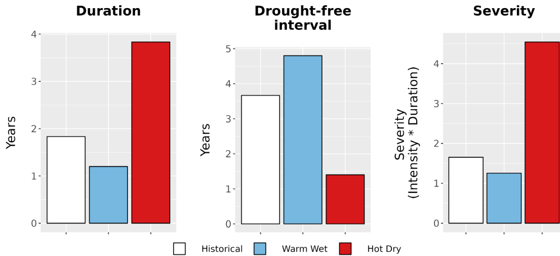
Figure 8. Drought metrics for GOSP. (Left) Average drought duration (years) historically (1979-2012) and under each climate future. (Middle) Average drought return interval (years), indicating the expected amount of time between periods of drought, historically and under each climate future. (Right) Average drought severity, a measure of drought intensity multiplied by duration, historically and under each climate future.
