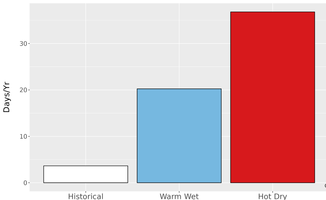
Figure 5. Metrics of extreme temperature at GOSP. The bar graph represents the average number of days annually with temperatures greater than the historical 99th percentile (98.1 °F) historically (1979-2012) and for the two climate futures (2050).
