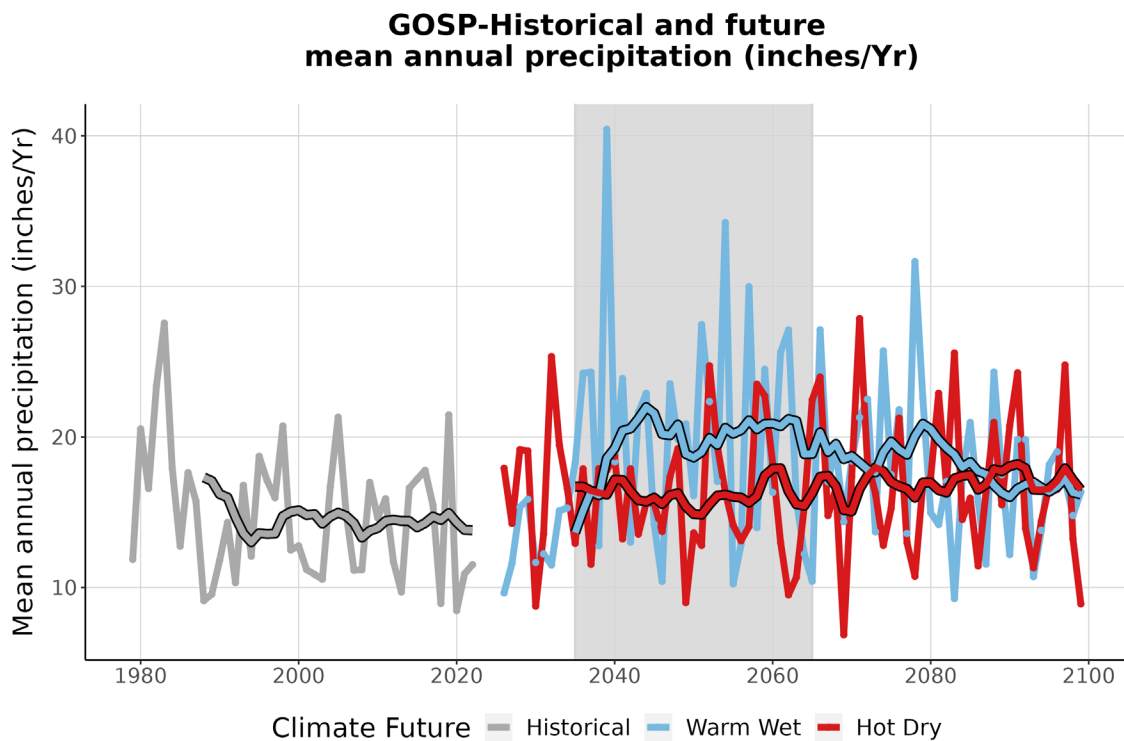
Figure 4. This graph compares observed average annual precipitation at GOSP (inches/year) (1979-2022) with projected average annual precipitation for the two climate futures over the period 2023-2099. The historically observed data is shown in gray, the Warm Wet climate future in blue, and the Hot Dry climate future in red. The smooth line running through each projection is the 10-year running average for historical observations and future projections. The gray-shaded area represents the time period that was averaged (2035-2065) to summarize future projections for the year 2050 (Appendix 1).
