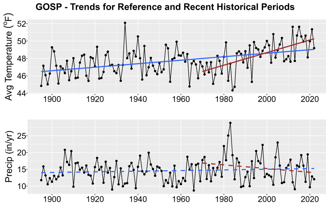
Figure 1. Historical trends in annual average temperature (upper plot) and annual total precipitation (lower plot) for GOSP from 1895-2022. Black points show yearly values while blue lines are linear regressions for the entire period record and red lines for 1970-2022 trends. Solid lines are significant trends (i.e., p < 0.05 ); dashed lines are not statistically significant.
