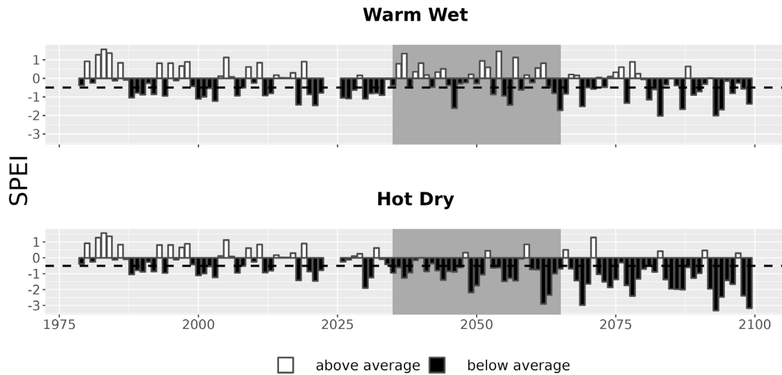
Figure 7. Drought metrics for GOSP. Drought index (SPEI; units = standard deviations from historical) timeseries for each climate future. Below-average SPEI (black bars) indicates dry conditions. The dotted line (SPEI = -0.5) indicates drought conditions.
