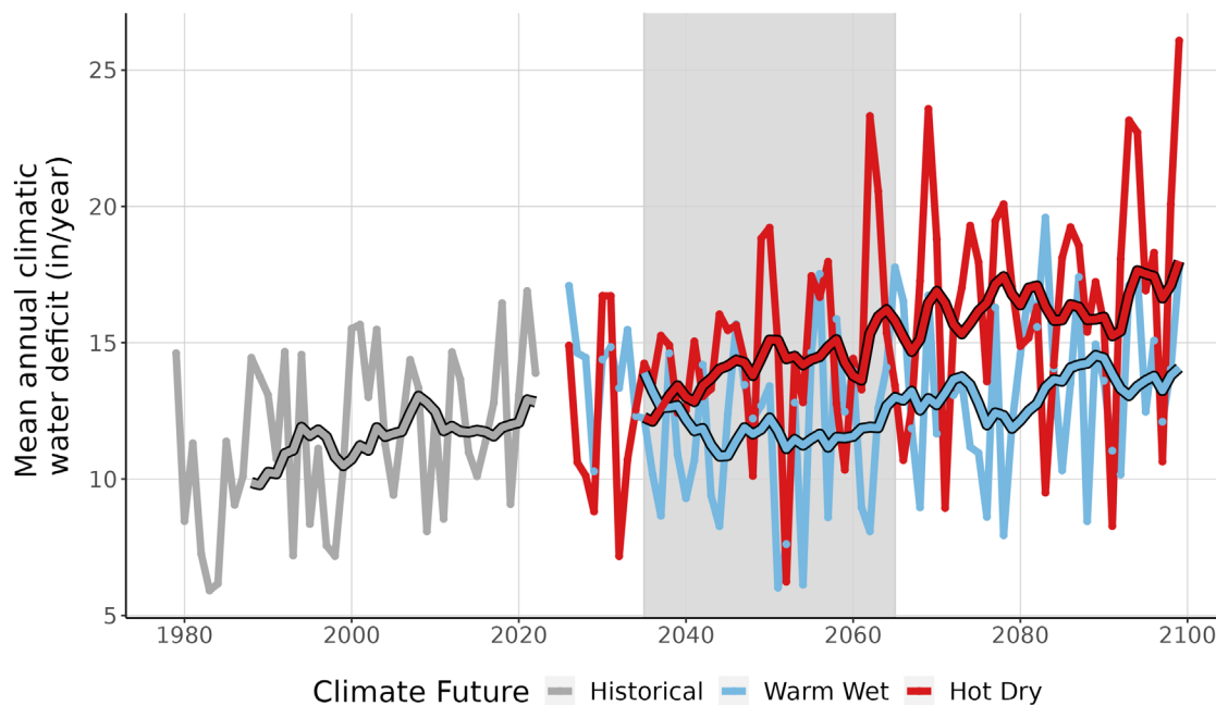
Figure 9. This line graph compares observed climatic water deficit at GOSP (inches/year) (1979-2022) with projected climatic water deficit for the two climate futures over the period 2023-2099. The historical observation data is shown in gray, the Warm Wet climate future in blue, and the Hot Dry climate future in red. The smooth line running through each projection is the 10-year running average for historical observations and future projections. Gray-shaded area represents the time period that was averaged (2035-2065) to summarize future projections for the year 2050.
