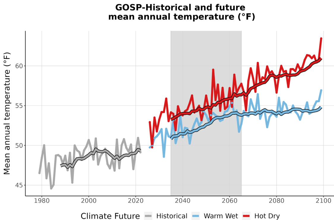
Figure 3. This graph compares observed average annual temperature at GOSP (°F) (1979-2022) with projected average annual temperature for the two climate futures over the period 2023-2099. The historically observed data is shown in gray, the Warm Wet climate future in blue, and the Hot Dry climate future in red. The smooth line
