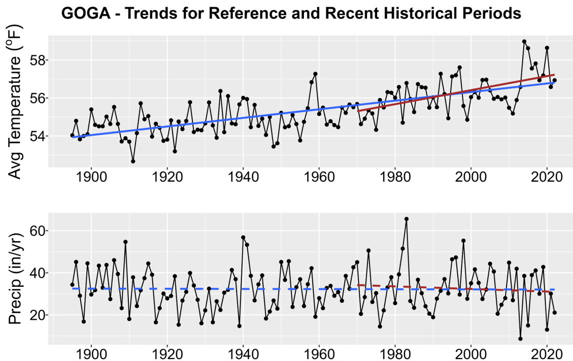
Figure 1. Historical trends in annual average temperature (upper plot) and annual total precipitation (lower plot) for GOGA from 1895-2022. Black points show yearly values while blue lines are linear regressions for the entire period record and red lines for 1970-2022 trends. Solid lines are significant trends (i.e., p < 0.05 ); dashed lines are not statistically significant.
