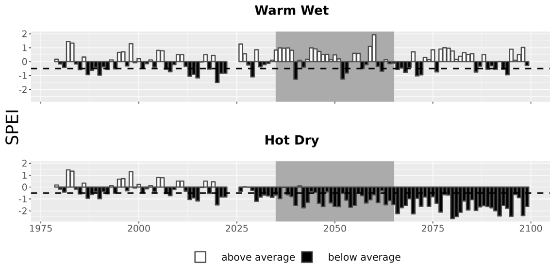
Figure 7. Drought metrics for GOGA. Drought index (SPEI; units = standard deviations from historical) timeseries for each climate future. Below-average SPEI (black bars) indicates dry conditions. The dotted line (SPEI = -0.5) indicates drought conditions.
