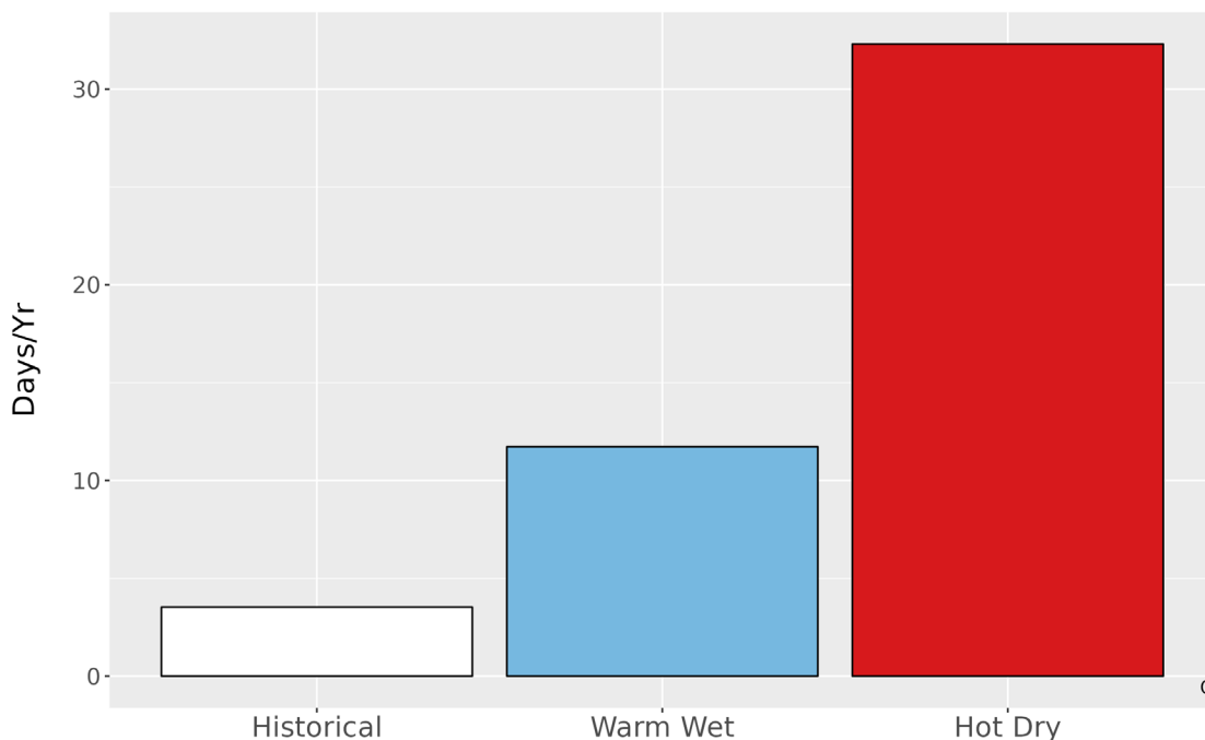
Figure 5. Metrics of extreme temperature at GOGA. The bar graph represents the average number of days annually with temperatures greater than the historical 99th percentile (76.4 °F) historically (1979-2012) and for the two climate futures (2050).
