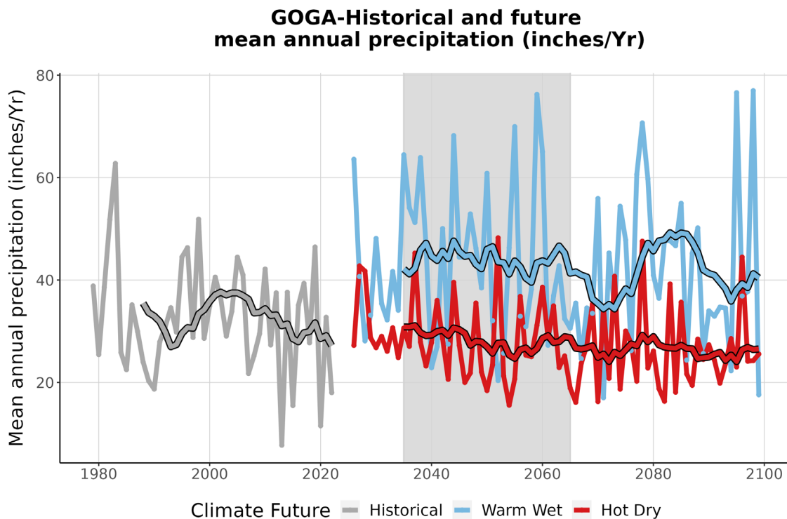
Figure 4. This graph compares observed average annual precipitation at GOGA (inches/year) (1979-2022) with projected average annual precipitation for the two climate futures over the period 2023-2099. The historically observed data is shown in gray, the Warm Wet climate future in blue, and the Hot Dry climate future in red. The smooth line running through each projection is the 10-year running average for historical observations and future projections. The gray-shaded area represents the time period that was averaged (2035-2065) to summarize future projections for the year 2050 (Appendix 1).
