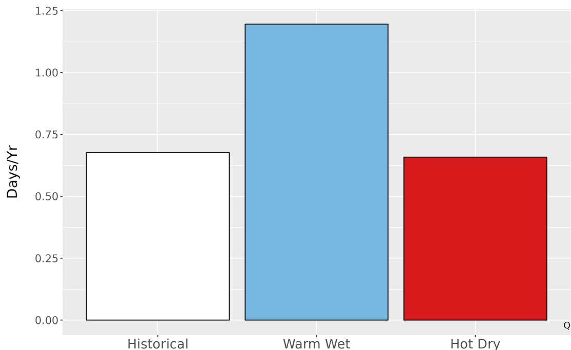
Figure 6. Average number of days annually with precipitation exceeding the 99th percentile (2.5 in.) of precipitation from the historical period 1979-2012 and for each climate future.
