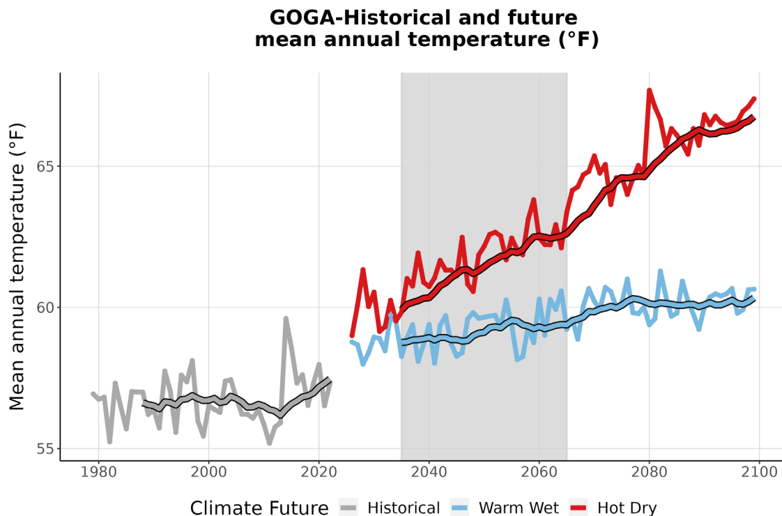
Figure 3. This graph compares observed average annual temperature at GOGA (°F) (1979-2022) with projected average annual temperature for the two climate futures over the period 2023-2099. The historically observed data
