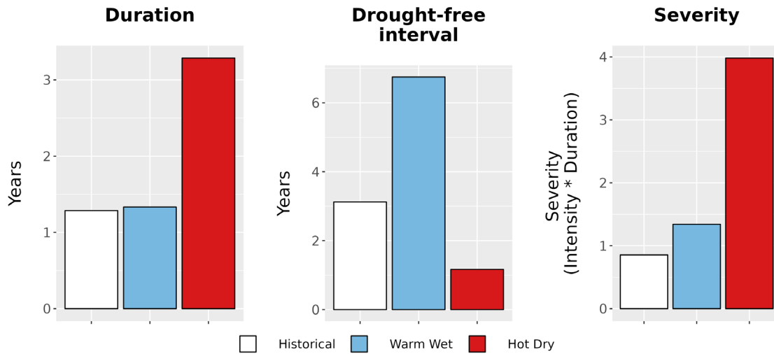
Figure 8. Drought metrics for GOGA. (Left) Average drought duration (years) historically (1979-2012) and under each climate future. (Middle) Average drought return interval (years), indicating the expected amount of time between periods of drought, historically and under each climate future. (Right) Average drought severity, a measure of drought intensity multiplied by duration, historically and under each climate future.
