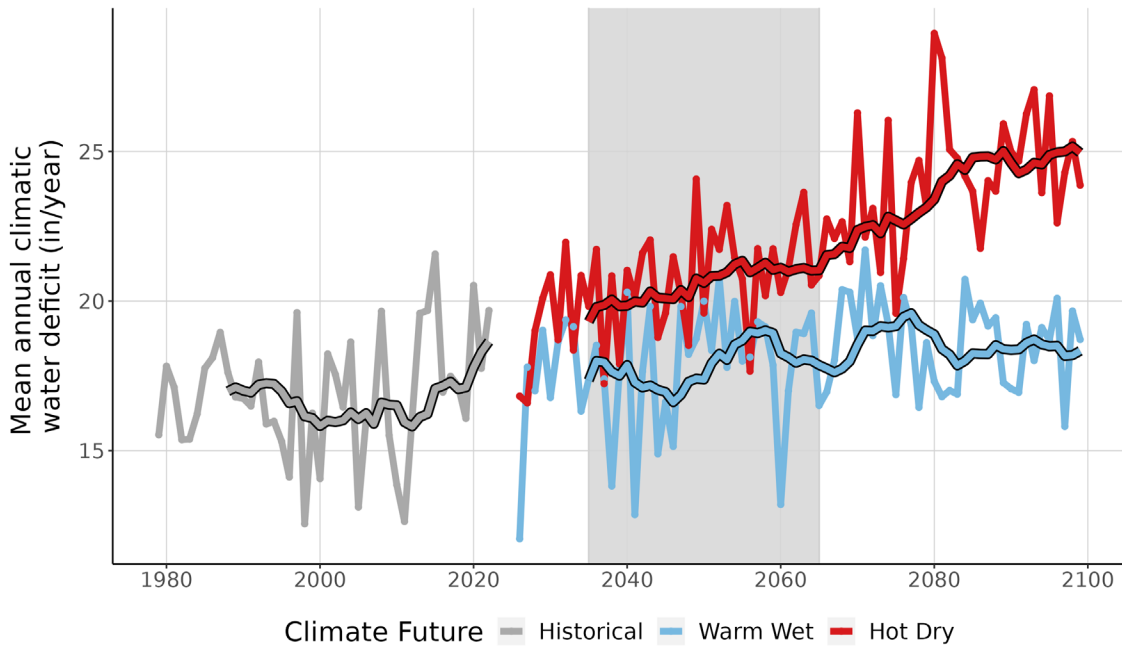
Figure 9. This line graph compares observed climatic water deficit at GOGA (inches/year) (1979-2022) with projected climatic water deficit for the two climate futures over the period 2023-2099. The historical observation data is shown in gray, the Warm Wet climate future in blue, and the Hot Dry climate future in red. The smooth line running through each projection is the 10-year running average for historical observations and future projections. Gray-shaded area represents the time period that was averaged (2035-2065) to summarize future projections for the year 2050.
