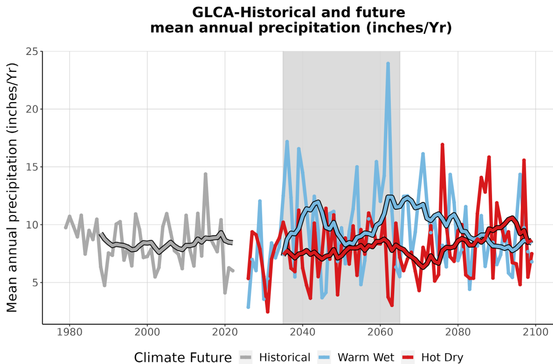
Figure 4. This graph compares observed average annual precipitation at GLCA (inches/year) (1979-2022) with projected average annual precipitation for the two climate futures over the period 2023-2099. The historically observed data is shown in gray, the Warm Wet climate future in blue, and the Hot Dry climate future in red. The smooth line running through each projection is the 10-year running average for historical observations and future projections. The gray-shaded area represents the time period that was averaged (2035-2065) to summarize future projections for the year 2050 (Appendix 1).
