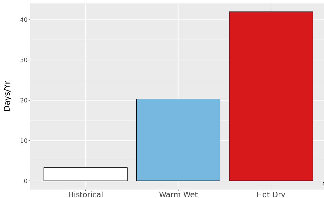
Figure 5. Metrics of extreme temperature at GLCA. The bar graph represents the average number of days annually with temperatures greater than the historical 99th percentile (99.8 °F) historically (1979-2012) and for the two climate futures (2050).
