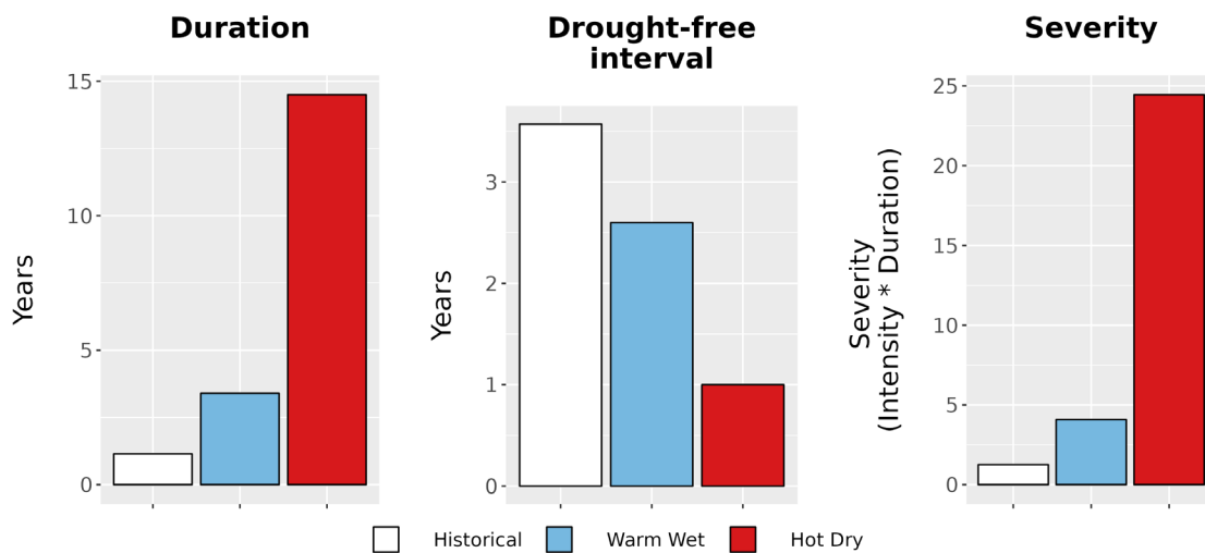
Figure 8. Drought metrics for GLCA. (Left) Average drought duration (years) historically (1979-2012) and under each climate future. (Middle) Average drought return interval (years), indicating the expected amount of time between periods of drought, historically and under each climate future. (Right) Average drought severity, a measure of drought intensity multiplied by duration, historically and under each climate future.
