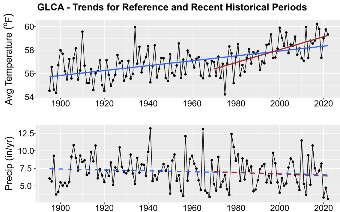
Figure 1. Historical trends in annual average temperature (upper plot) and annual total precipitation (lower plot) for GLCA from 1895-2022. Black points show yearly values while blue lines are linear regressions for the entire period record and red lines for 1970-2022 trends. Solid lines are significant trends (i.e., p < 0.05 ); dashed lines are not statistically significant.
