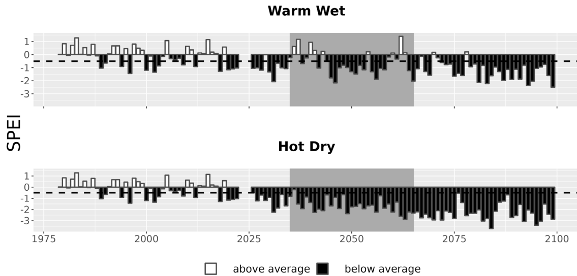
Figure 7. Drought metrics for GLCA. Drought index (SPEI; units = standard deviations from historical) timeseries for each climate future. Below-average SPEI (black bars) indicates dry conditions. The dotted line (SPEI = -0.5) indicates drought conditions.
