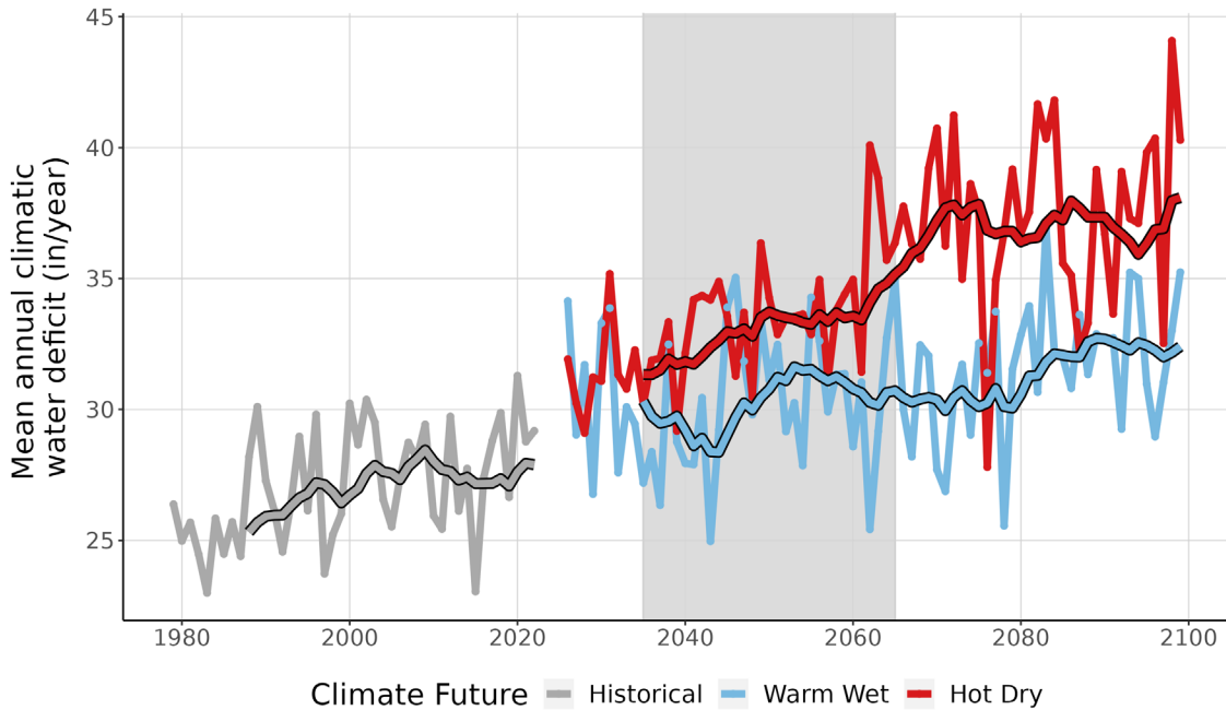
Figure 9. This line graph compares observed climatic water deficit at GLCA (inches/year) (1979-2022) with projected climatic water deficit for the two climate futures over the period 2023-2099. The historical observation data is shown in gray, the Warm Wet climate future in blue, and the Hot Dry climate future in red. The smooth line running through each projection is the 10-year running average for historical observations and future projections. Gray-shaded area represents the time period that was averaged (2035-2065) to summarize future projections for the year 2050.
