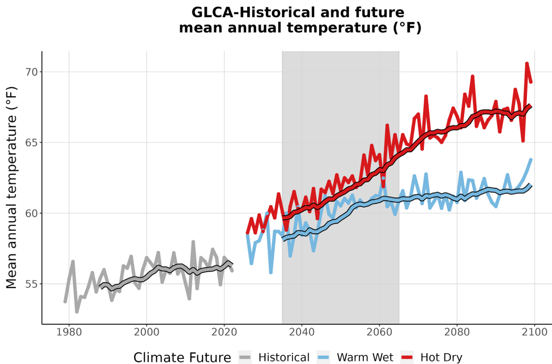
Figure 3. This graph compares observed average annual temperature at GLCA (°F) (1979-2022) with projected average annual temperature for the two climate futures over the period 2023-2099. The historically observed data is shown in gray, the Warm Wet climate future in blue, and the Hot Dry climate future in red. The smooth line
