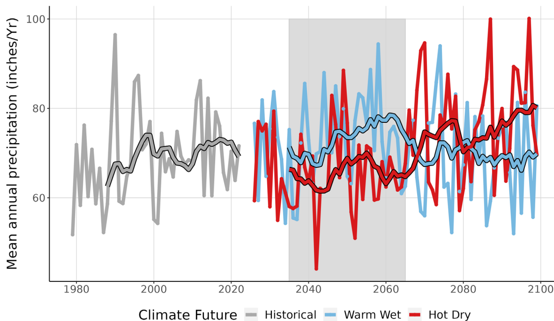
Figure 4. This graph compares observed average annual precipitation at GLAC (inches/year) (1979-2022) with projected average annual precipitation for the two climate futures over the period 2023-2099. The historically observed data is shown in gray, the Warm Wet climate future in blue, and the Hot Dry climate future in red. The smooth line running through each projection is the 10-year running average for historical observations and future projections. The gray-shaded area represents the time period that was averaged (2035-2065) to summarize future projections for the year 2050 (Appendix 1).
