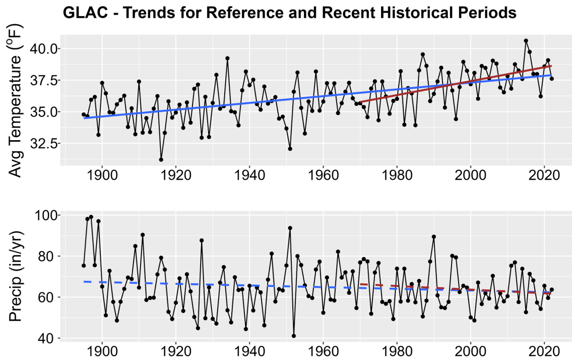
Figure 1. Historical trends in annual average temperature (upper plot) and annual total precipitation (lower plot) for GLAC from 1895-2022. Black points show yearly values while blue lines are linear regressions for the entire period record and red lines for 1970-2022 trends. Solid lines are significant trends (i.e., p < 0.05 ); dashed lines are not statistically significant.
