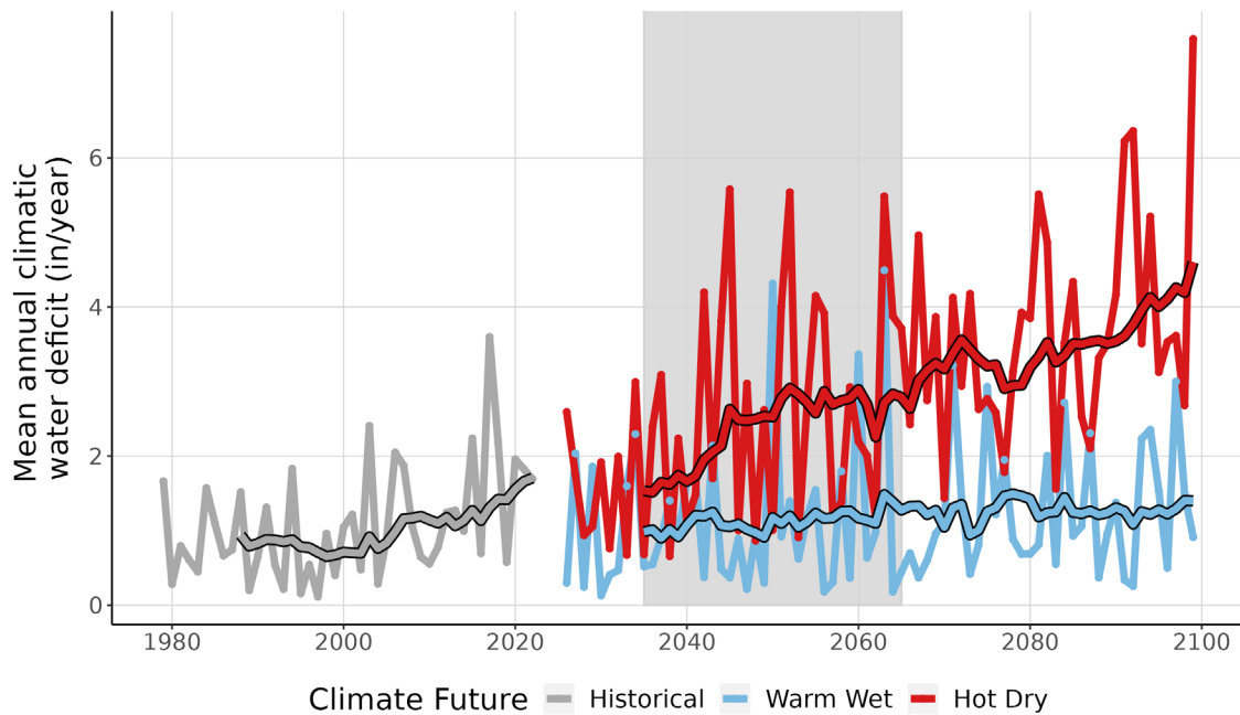
Figure 9. This line graph compares observed climatic water deficit at GLAC (inches/year) (1979-2022) with projected climatic water deficit for the two climate futures over the period 2023-2099. The historical observation data is shown in gray, the Warm Wet climate future in blue, and the Hot Dry climate future in red. The smooth line running through each projection is the 10-year running average for historical observations and future projections. Gray-shaded area represents the time period that was averaged (2035-2065) to summarize future projections for the year 2050.
