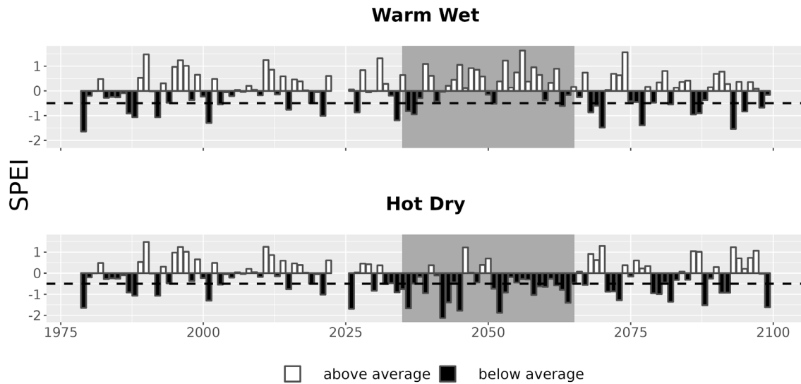
Figure 7. Drought metrics for GLAC. Drought index (SPEI; units = standard deviations from historical) timeseries for each climate future. Below-average SPEI (black bars) indicates dry conditions. The dotted line (SPEI = -0.5) indicates drought conditions.
