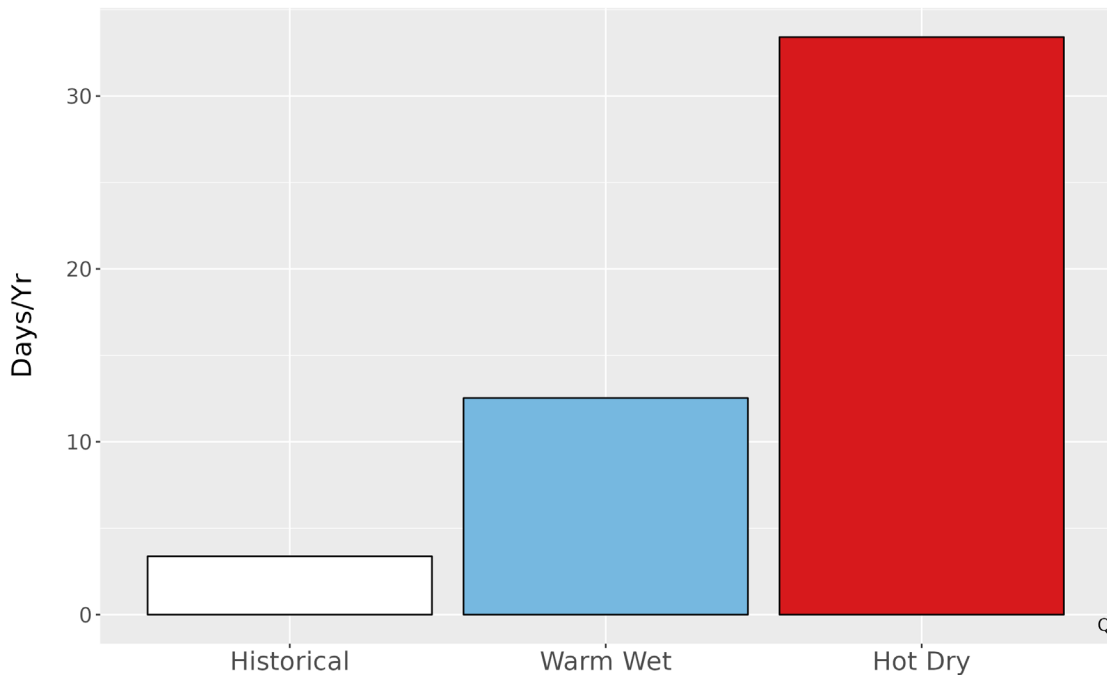
Figure 5. Metrics of extreme temperature at GLAC. The bar graph represents the average number of days annually with temperatures greater than the historical 99th percentile (78.2 °F) historically (1979-2012) and for the two climate futures (2050).
