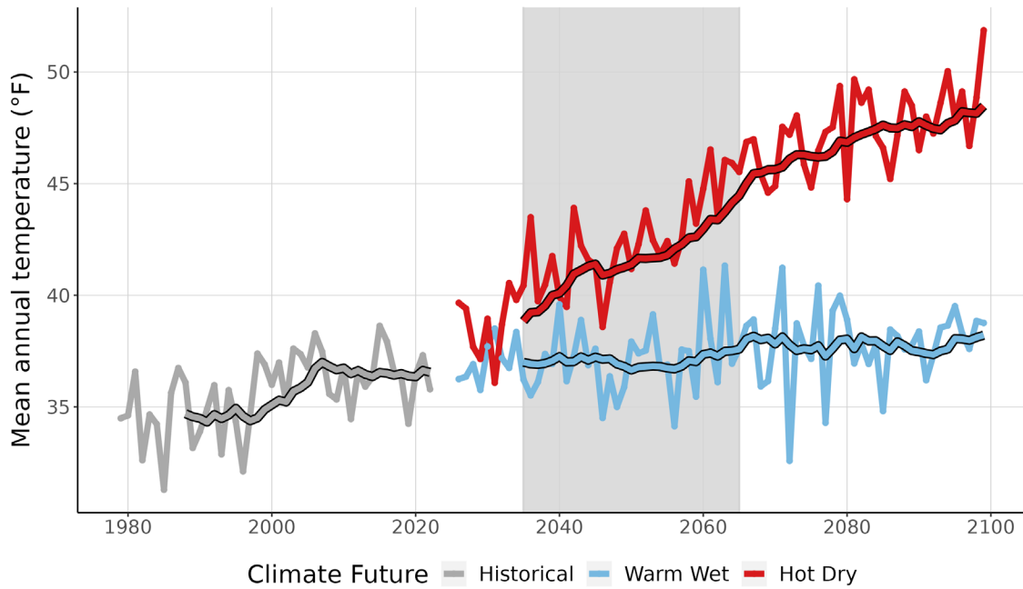
Figure 3. This graph compares observed average annual temperature at GLAC (°F) (1979-2022) with projected average annual temperature for the two climate futures over the period 2023-2099. The historically observed data is shown in gray, the Warm Wet climate future in blue, and the Hot Dry climate future in red. The smooth line running through each projection is the 10-year running average for historical observations and future projections. Gray-shaded area represents the time period that was averaged (2035-2065) to summarize future projections for the year 2050 (Appendix 1).
