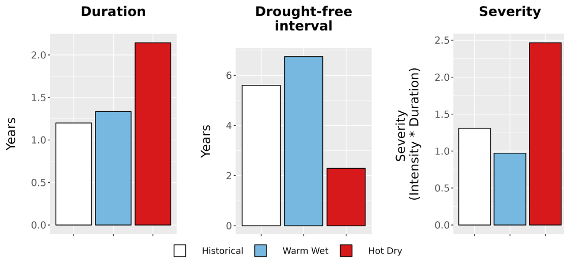
Figure 8. Drought metrics for GLAC. (Left) Average drought duration (years) historically (1979-2012) and under each climate future. (Middle) Average drought return interval (years), indicating the expected amount of time between periods of drought, historically and under each climate future. (Right) Average drought severity, a measure of drought intensity multiplied by duration, historically and under each climate future.
