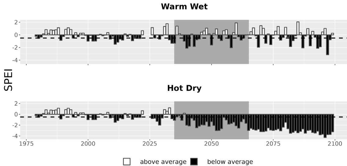
Figure 7. Drought metrics for GICL. Drought index (SPEI; units = standard deviations from historical) timeseries for each climate future. Below-average SPEI (black bars) indicates dry conditions. The dotted line (SPEI = -0.5) indicates drought conditions.
