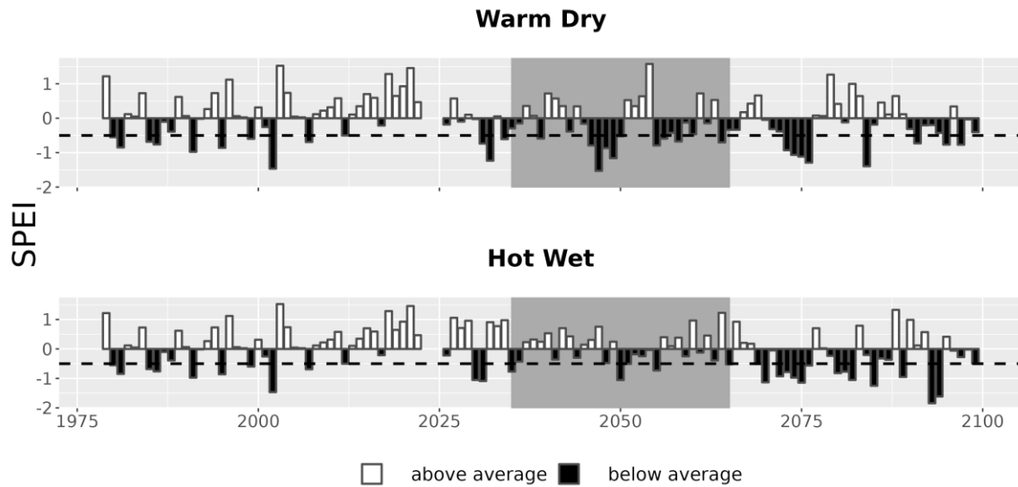
Figure 7. Drought metrics for GEWA. Drought index (SPEI; units = standard deviations from historical) timeseries for each climate future. Below-average SPEI (black bars) indicates dry conditions. The dotted line (SPEI = -0.5) indicates drought conditions.
