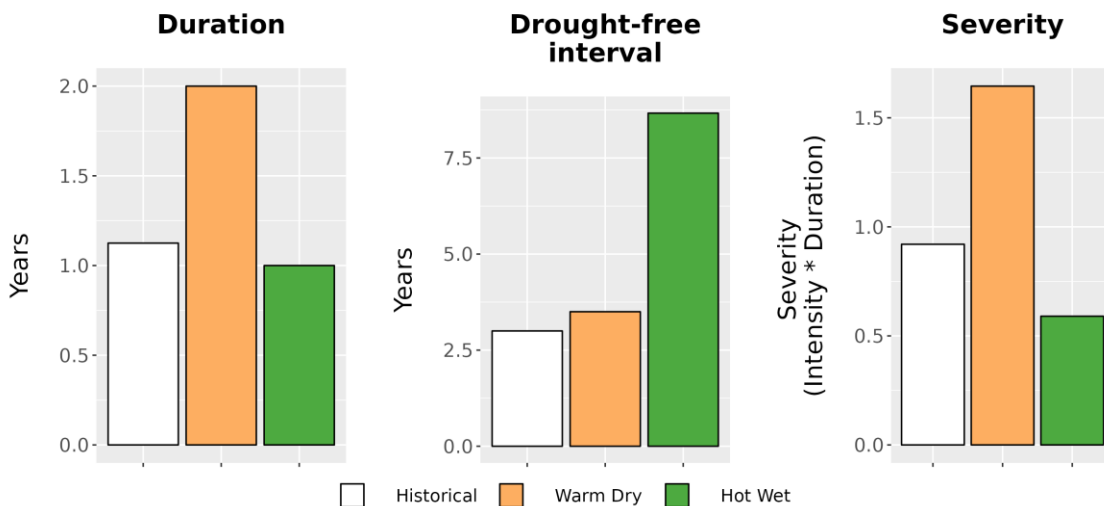
Figure 8. Drought metrics for GEWA. (Left) Average drought duration (years) historically (1979-2012) and under each climate future. (Middle) Average drought return interval (years), indicating the expected amount of time between periods of drought, historically and under each climate future. (Right) Average drought severity, a measure of drought intensity multiplied by duration, historically and under each climate future.
