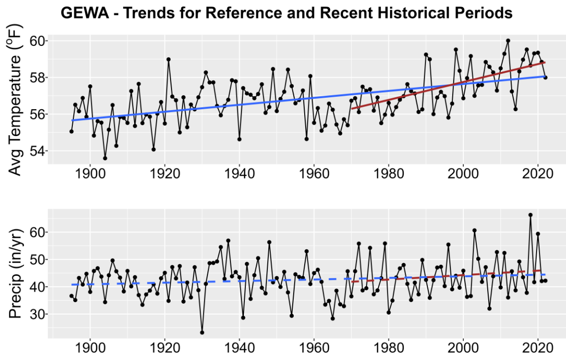
Figure 1. Historical trends in annual average temperature (upper plot) and annual total precipitation (lower plot) for GEWA from 1895-2022. Black points show yearly values while blue lines are linear regressions for the entire period record and red lines for 1970-2022 trends. Solid lines are significant trends (i.e., p < 0.05 ); dashed lines are not statistically significant.
