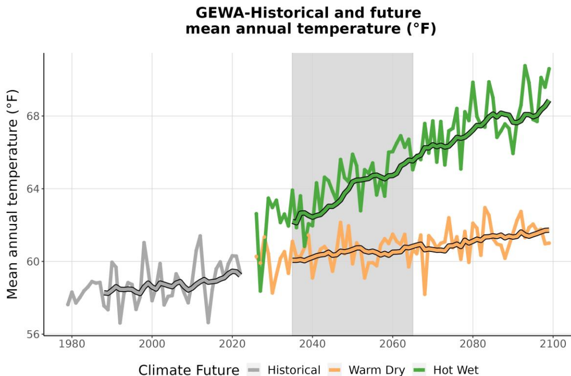
Figure 3. This graph compares observed average annual temperature at GEWA (°F) (1979-2022) with projected average annual temperature for the two climate futures over the period 2023-2099. The historically observed data
