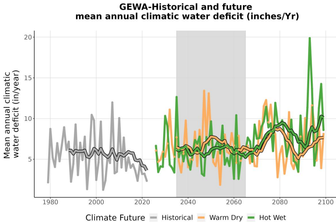
Figure 9. This line graph compares observed climatic water deficit at GEWA (inches/year) (1979-2022) with projected climatic water deficit for the two climate futures over the period 2023-2099. The historical observation data is shown in gray, the Warm Dry climate future in orange, and the Hot Wet climate future in green. The smooth line running through each projection is the 10-year running average for historical observations and future projections. Gray-shaded area represents the time period that was averaged (2035-2065) to summarize future projections for the year 2050.
