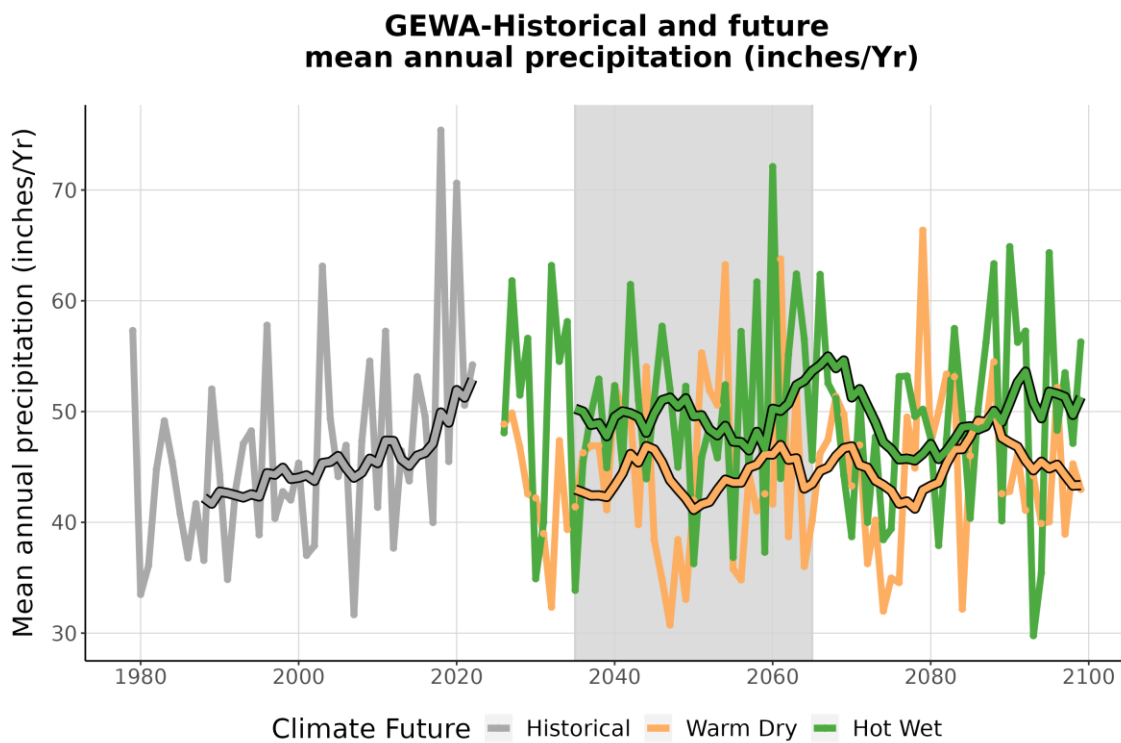
Figure 4. This graph compares observed average annual precipitation at GEWA (inches/year) (1979-2022) with projected average annual precipitation for the two climate futures over the period 2023-2099. The historically observed data is shown in gray, the Warm Dry climate future in orange, and the Hot Wet climate future in green. The smooth line running through each projection is the 10-year running average for historical observations and future projections. The gray-shaded area represents the time period that was averaged (2035-2065) to summarize future projections for the year 2050 (Appendix 1).
