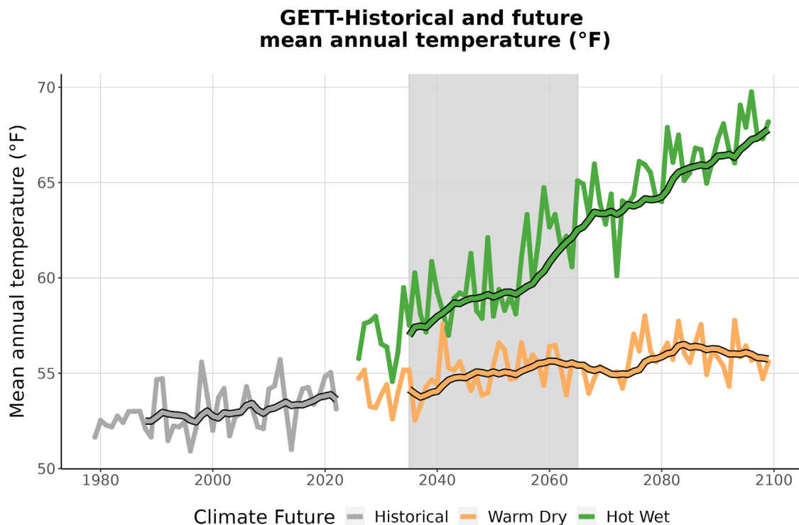
Figure 3. This graph compares observed average annual temperature at GETT (°F) (1979-2022) with projected average annual temperature for the two climate futures over the period 2023-2099. The historically observed data
