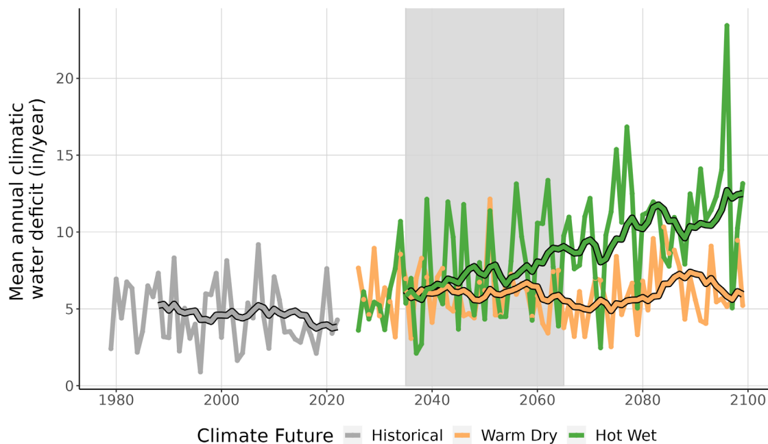
Figure 9. This line graph compares observed climatic water deficit at GETT (inches/year) (1979-2022) with projected climatic water deficit for the two climate futures over the period 2023-2099. The historical observation data is shown in gray, the Warm Dry climate future in orange, and the Hot Wet climate future in green. The smooth line running through each projection is the 10-year running average for historical observations and future projections. Gray-shaded area represents the time period that was averaged (2035-2065) to summarize future projections for the year 2050.
