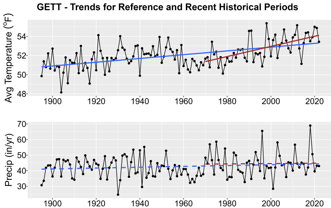
Figure 1. Historical trends in annual average temperature (upper plot) and annual total precipitation (lower plot) for GETT from 1895-2022. Black points show yearly values while blue lines are linear regressions for the entire period record and red lines for 1970-2022 trends. Solid lines are significant trends (i.e., p < 0.05 ); dashed lines are not statistically significant.
