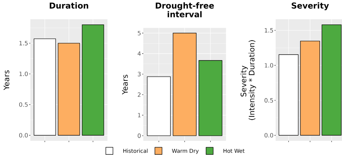
Figure 8. Drought metrics for GETT. (Left) Average drought duration (years) historically (1979-2012) and under each climate future. (Middle) Average drought return interval (years), indicating the expected amount of time between periods of drought, historically and under each climate future. (Right) Average drought severity, a measure of drought intensity multiplied by duration, historically and under each climate future.
