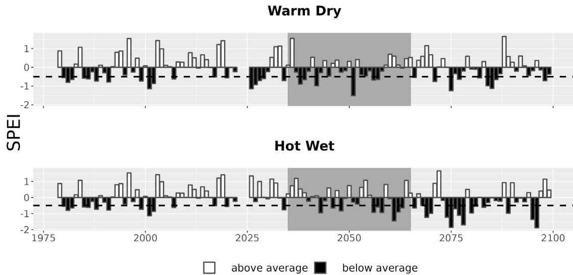
Figure 7. Drought metrics for GETT. Drought index (SPEI; units = standard deviations from historical) timeseries for each climate future. Below-average SPEI (black bars) indicates dry conditions. The dotted line (SPEI = -0.5) indicates drought conditions.
