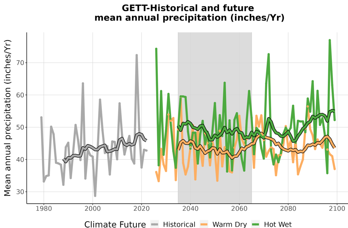
Figure 4. This graph compares observed average annual precipitation at GETT (inches/year) (1979-2022) with projected average annual precipitation for the two climate futures over the period 2023-2099. The historically observed data is shown in gray, the Warm Dry climate future in orange, and the Hot Wet climate future in green. The smooth line running through each projection is the 10-year running average for historical observations and future projections. The gray-shaded area represents the time period that was averaged (2035-2065) to summarize future projections for the year 2050 (Appendix 1).
