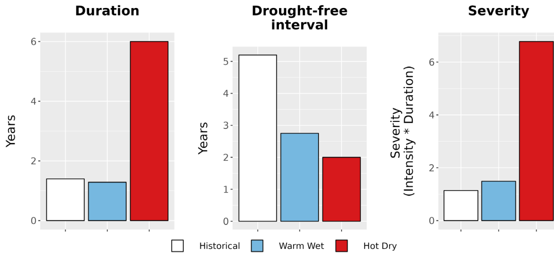
Figure 8. Drought metrics for GERO. (Left) Average drought duration (years) historically (1979-2012) and under each climate future. (Middle) Average drought return interval (years), indicating the expected amount of time between periods of drought, historically and under each climate future. (Right) Average drought severity, a measure of drought intensity multiplied by duration, historically and under each climate future.
