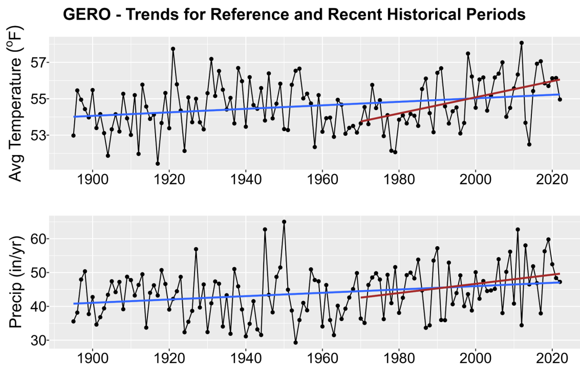
Figure 1. Historical trends in annual average temperature (upper plot) and annual total precipitation (lower plot) for GERO from 1895-2022. Black points show yearly values while blue lines are linear regressions for the entire period record and red lines for 1970-2022 trends. Solid lines are significant trends (i.e., p < 0.05 ); dashed lines are not statistically significant.
