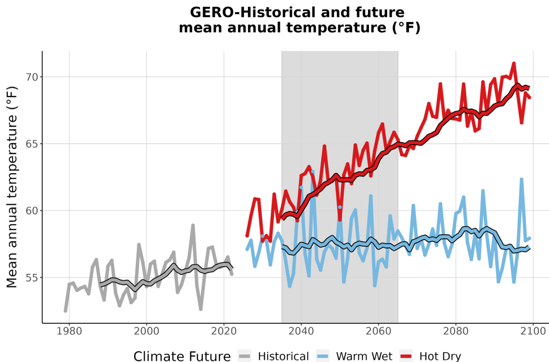
Figure 3. This graph compares observed average annual temperature at GERO (°F) (1979-2022) with projected average annual temperature for the two climate futures over the period 2023-2099. The historically observed data
