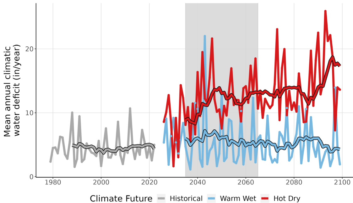
Figure 9. This line graph compares observed climatic water deficit at GERO (inches/year) (1979-2022) with projected climatic water deficit for the two climate futures over the period 2023-2099. The historical observation data is shown in gray, the Warm Wet climate future in blue, and the Hot Dry climate future in red. The smooth line running through each projection is the 10-year running average for historical observations and future projections. Gray-shaded area represents the time period that was averaged (2035-2065) to summarize future projections for the year 2050.
