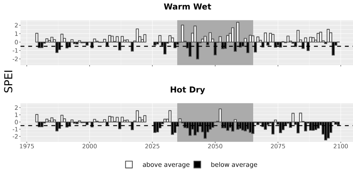
Figure 7. Drought metrics for GERO. Drought index (SPEI; units = standard deviations from historical) timeseries for each climate future. Below-average SPEI (black bars) indicates dry conditions. The dotted line (SPEI = -0.5) indicates drought conditions.
