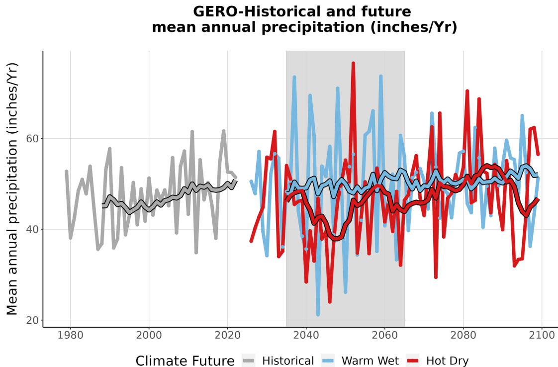
Figure 4. This graph compares observed average annual precipitation at GERO (inches/year) (1979-2022) with projected average annual precipitation for the two climate futures over the period 2023-2099. The historically observed data is shown in gray, the Warm Wet climate future in blue, and the Hot Dry climate future in red. The smooth line running through each projection is the 10-year running average for historical observations and future projections. The gray-shaded area represents the time period that was averaged (2035-2065) to summarize future projections for the year 2050 (Appendix 1).
