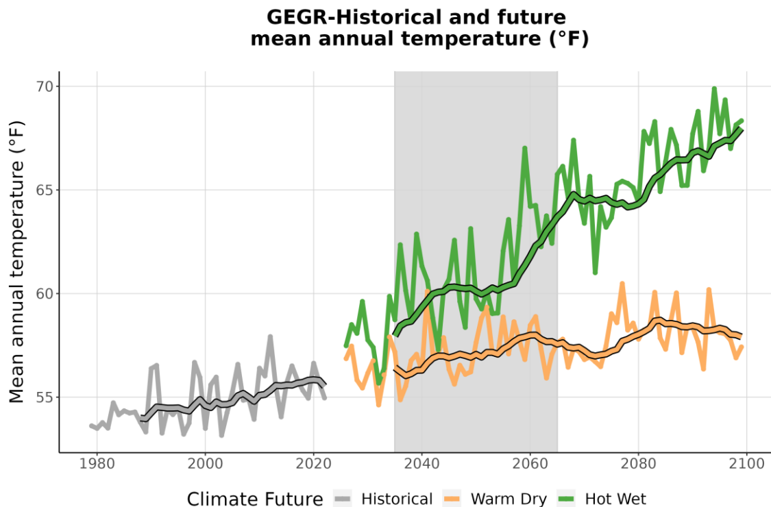
Figure 3. This graph compares observed average annual temperature at GEGR (°F) (1979-2022) with projected average annual temperature for the two climate futures over the period 2023-2099. The historically observed data
