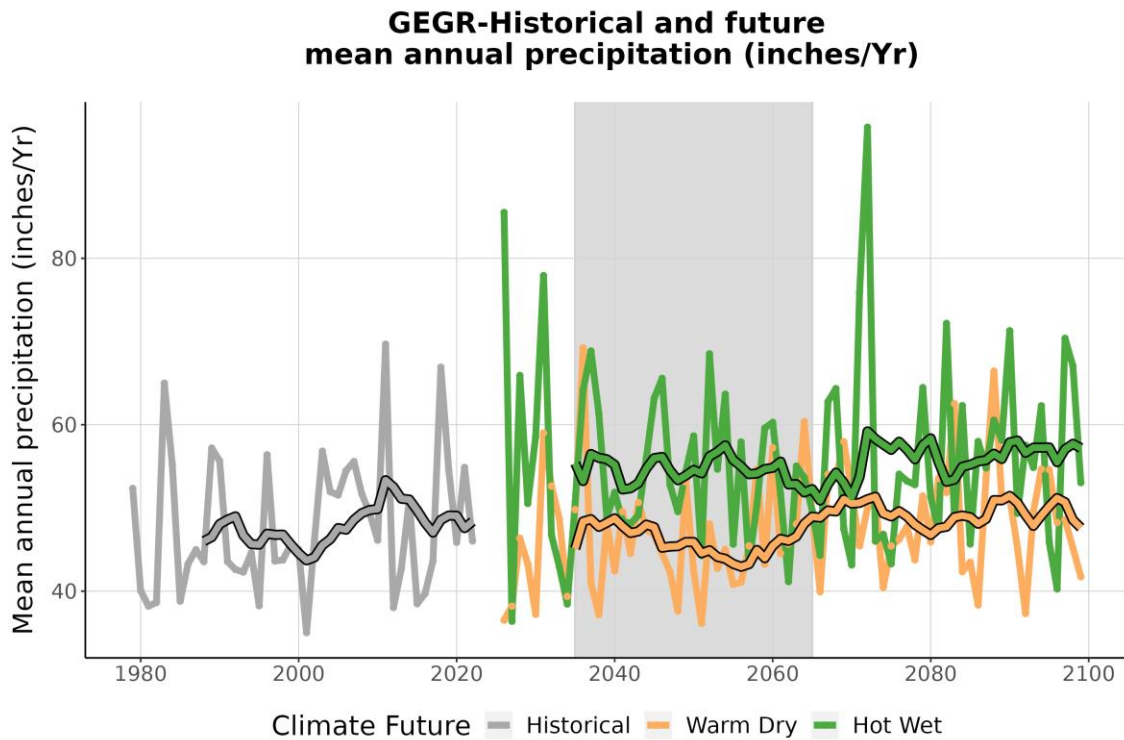
Figure 4. This graph compares observed average annual precipitation at GEGR (inches/year) (1979-2022) with projected average annual precipitation for the two climate futures over the period 2023-2099. The historically observed data is shown in gray, the Warm Dry climate future in orange, and the Hot Wet climate future in green. The smooth line running through each projection is the 10-year running average for historical observations and future projections. The gray-shaded area represents the time period that was averaged (2035-2065) to summarize future projections for the year 2050 (Appendix 1).
