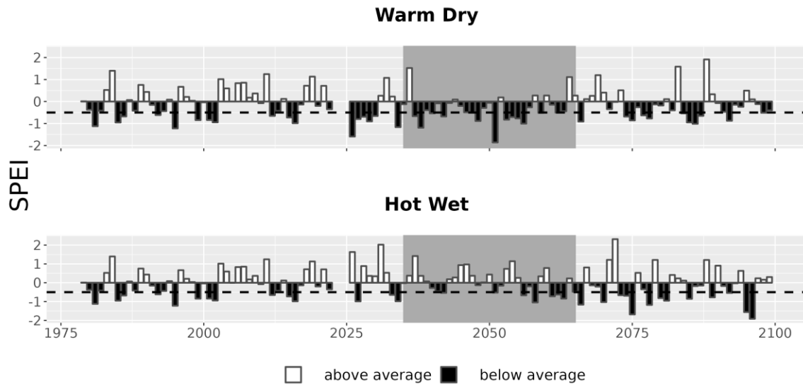
Figure 7. Drought metrics for GEGR. Drought index (SPEI; units = standard deviations from historical) timeseries for each climate future. Below-average SPEI (black bars) indicates dry conditions. The dotted line (SPEI = -0.5) indicates drought conditions.
