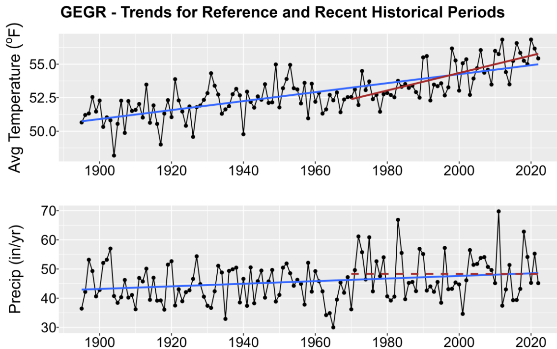
Figure 1. Historical trends in annual average temperature (upper plot) and annual total precipitation (lower plot) for GEGR from 1895-2022. Black points show yearly values while blue lines are linear regressions for the entire period record and red lines for 1970-2022 trends. Solid lines are significant trends (i.e., p < 0.05 ); dashed lines are not statistically significant.
