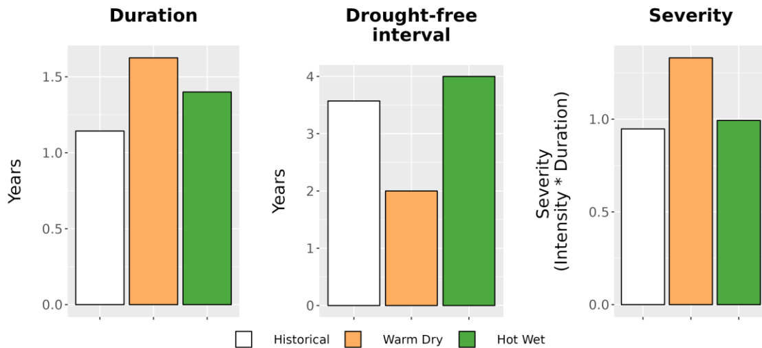
Figure 8. Drought metrics for GEGR. (Left) Average drought duration (years) historically (1979-2012) and under each climate future. (Middle) Average drought return interval (years), indicating the expected amount of time between periods of drought, historically and under each climate future. (Right) Average drought severity, a measure of drought intensity multiplied by duration, historically and under each climate future.
