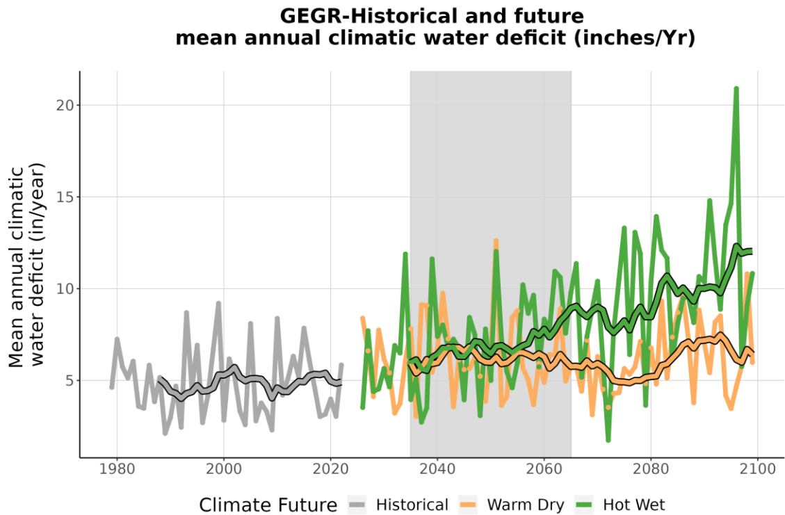
Figure 9. This line graph compares observed climatic water deficit at GEGR (inches/year) (1979-2022) with projected climatic water deficit for the two climate futures over the period 2023-2099. The historical observation data is shown in gray, the Warm Dry climate future in orange, and the Hot Wet climate future in green. The smooth line running through each projection is the 10-year running average for historical observations and future projections. Gray-shaded area represents the time period that was averaged (2035-2065) to summarize future projections for the year 2050.
