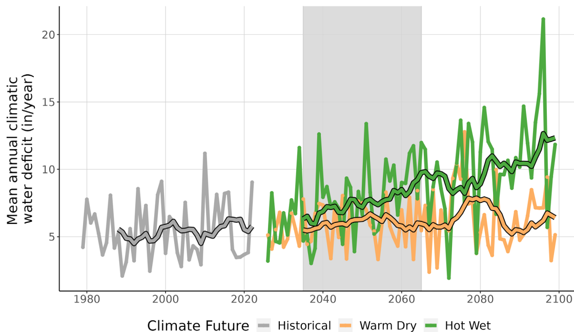
Figure 9. This line graph compares observed climatic water deficit at GATE (inches/year) (1979-2022) with projected climatic water deficit for the two climate futures over the period 2023-2099. The historical observation data is shown in gray, the Warm Dry climate future in orange, and the Hot Wet climate future in green. The smooth line running through each projection is the 10-year running average for historical observations and future projections. Gray-shaded area represents the time period that was averaged (2035-2065) to summarize future projections for the year 2050.
