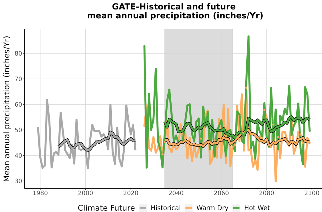
Figure 4. This graph compares observed average annual precipitation at GATE (inches/year) (1979-2022) with projected average annual precipitation for the two climate futures over the period 2023-2099. The historically observed data is shown in gray, the Warm Dry climate future in orange, and the Hot Wet climate future in green. The smooth line running through each projection is the 10-year running average for historical observations and future projections. The gray-shaded area represents the time period that was averaged (2035-2065) to summarize future projections for the year 2050 (Appendix 1).
