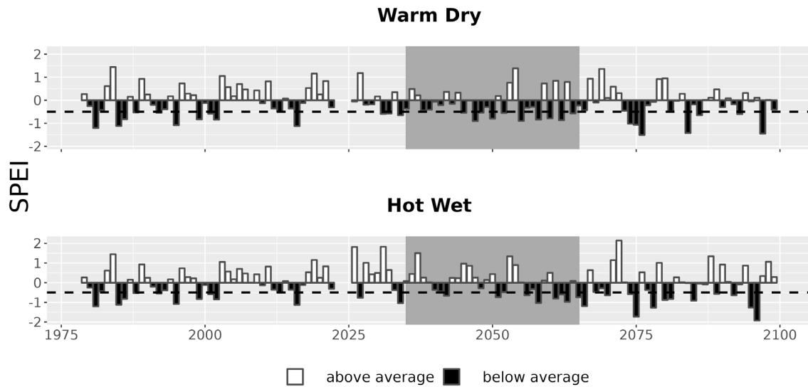
Figure 7. Drought metrics for GATE. Drought index (SPEI; units = standard deviations from historical) timeseries for each climate future. Below-average SPEI (black bars) indicates dry conditions. The dotted line (SPEI = -0.5) indicates drought conditions.
