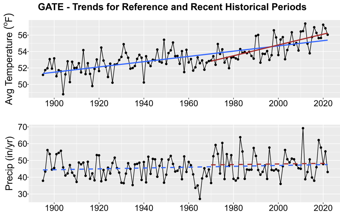
Figure 1. Historical trends in annual average temperature (upper plot) and annual total precipitation (lower plot) for GATE from 1895-2022. Black points show yearly values while blue lines are linear regressions for the entire period record and red lines for 1970-2022 trends. Solid lines are significant trends (i.e., p < 0.05 ); dashed lines are not statistically significant.
