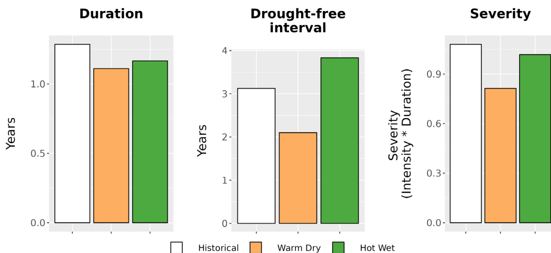
Figure 8. Drought metrics for GATE. (Left) Average drought duration (years) historically (1979-2012) and under each climate future. (Middle) Average drought return interval (years), indicating the expected amount of time between periods of drought, historically and under each climate future. (Right) Average drought severity, a measure of drought intensity multiplied by duration, historically and under each climate future.
