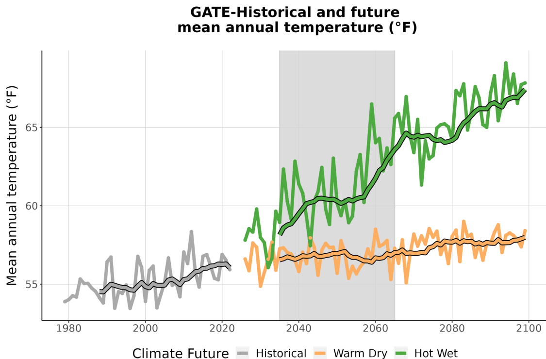
Figure 3. This graph compares observed average annual temperature at GATE (°F) (1979-2022) with projected average annual temperature for the two climate futures over the period 2023-2099. The historically observed data
