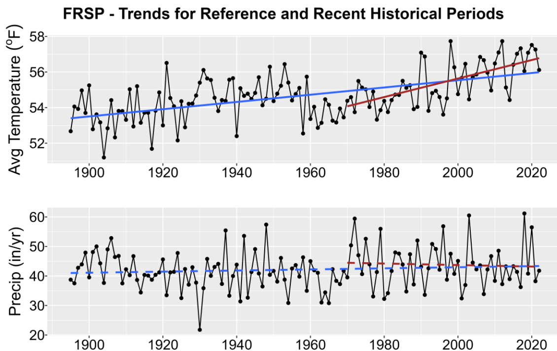
Figure 1. Historical trends in annual average temperature (upper plot) and annual total precipitation (lower plot) for FRSP from 1895-2022. Black points show yearly values while blue lines are linear regressions for the entire period record and red lines for 1970-2022 trends. Solid lines are significant trends (i.e., p < 0.05 ); dashed lines are not statistically significant.
