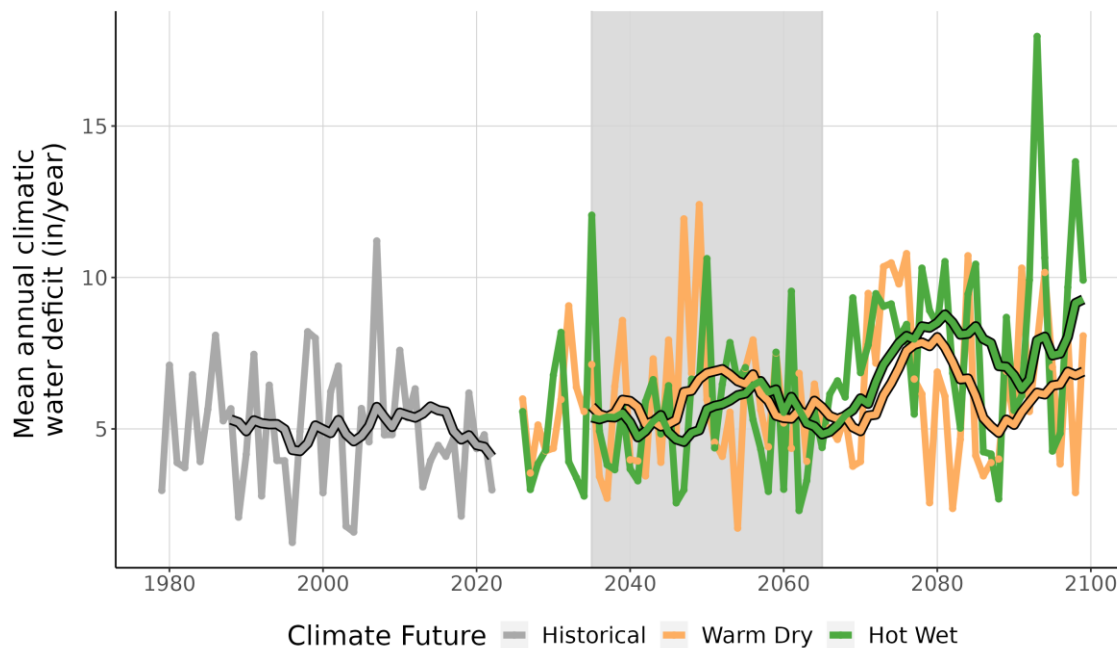
Figure 9. This line graph compares observed climatic water deficit at FRSP (inches/year) (1979-2022) with projected climatic water deficit for the two climate futures over the period 2023-2099. The historical observation data is shown in gray, the Warm Dry climate future in orange, and the Hot Wet climate future in green. The smooth line running through each projection is the 10-year running average for historical observations and future projections. Gray-shaded area represents the time period that was averaged (2035-2065) to summarize future projections for the year 2050.
