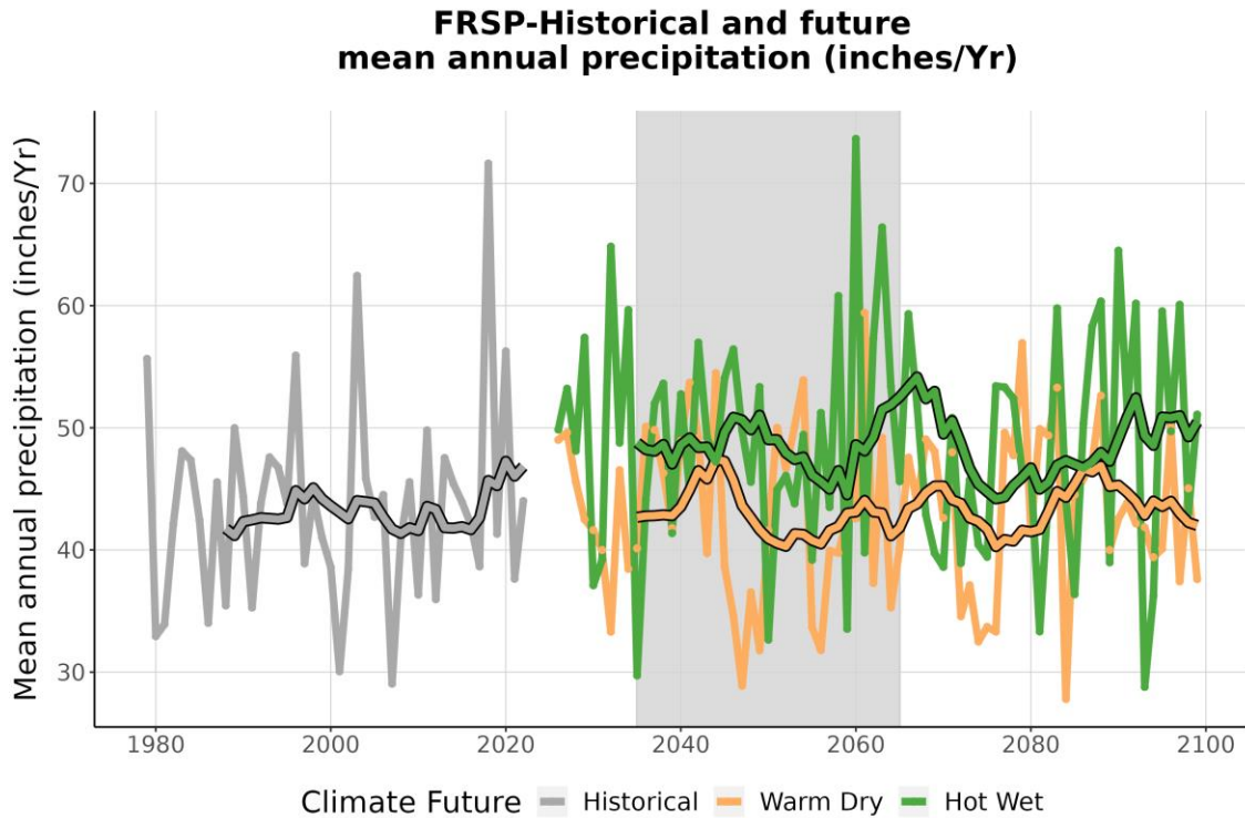
Figure 4. This graph compares observed average annual precipitation at FRSP (inches/year) (1979-2022) with projected average annual precipitation for the two climate futures over the period 2023-2099. The historically observed data is shown in gray, the Warm Dry climate future in orange, and the Hot Wet climate future in green. The smooth line running through each projection is the 10-year running average for historical observations and future projections. The gray-shaded area represents the time period that was averaged (2035-2065) to summarize future projections for the year 2050 (Appendix 1).
