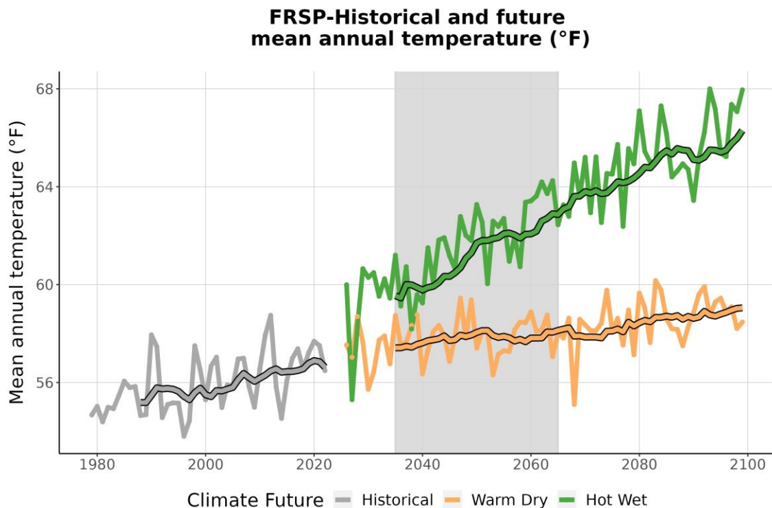
Figure 3. This graph compares observed average annual temperature at FRSP (°F) (1979-2022) with projected average annual temperature for the two climate futures over the period 2023-2099. The historically observed data
