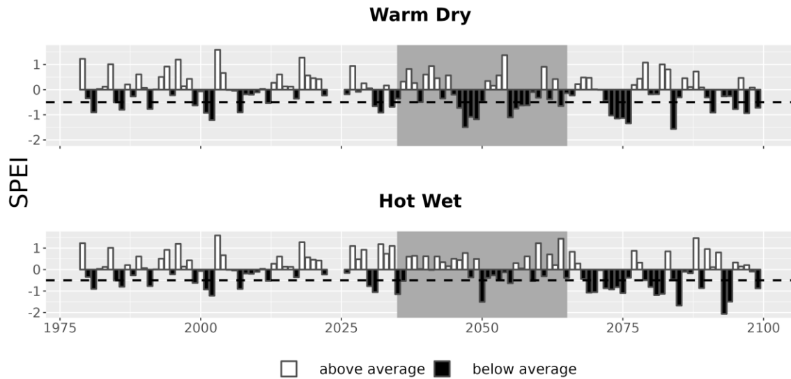
Figure 7. Drought metrics for FRSP. Drought index (SPEI; units = standard deviations from historical) timeseries for each climate future. Below-average SPEI (black bars) indicates dry conditions. The dotted line (SPEI = -0.5) indicates drought conditions.
