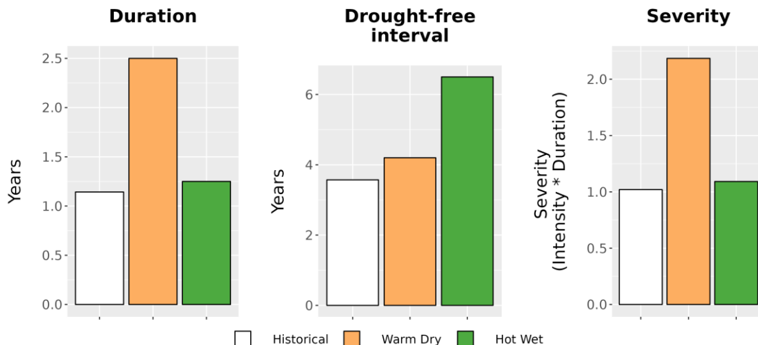
Figure 8. Drought metrics for FRSP. (Left) Average drought duration (years) historically (1979-2012) and under each climate future. (Middle) Average drought return interval (years), indicating the expected amount of time between periods of drought, historically and under each climate future. (Right) Average drought severity, a measure of drought intensity multiplied by duration, historically and under each climate future.
